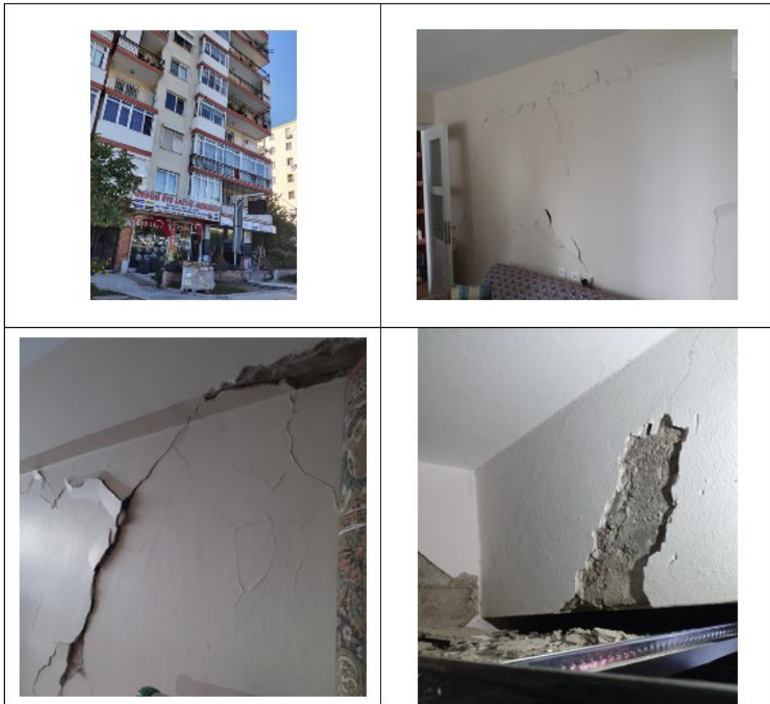
Figure 6.17. Photographs of Building #9
