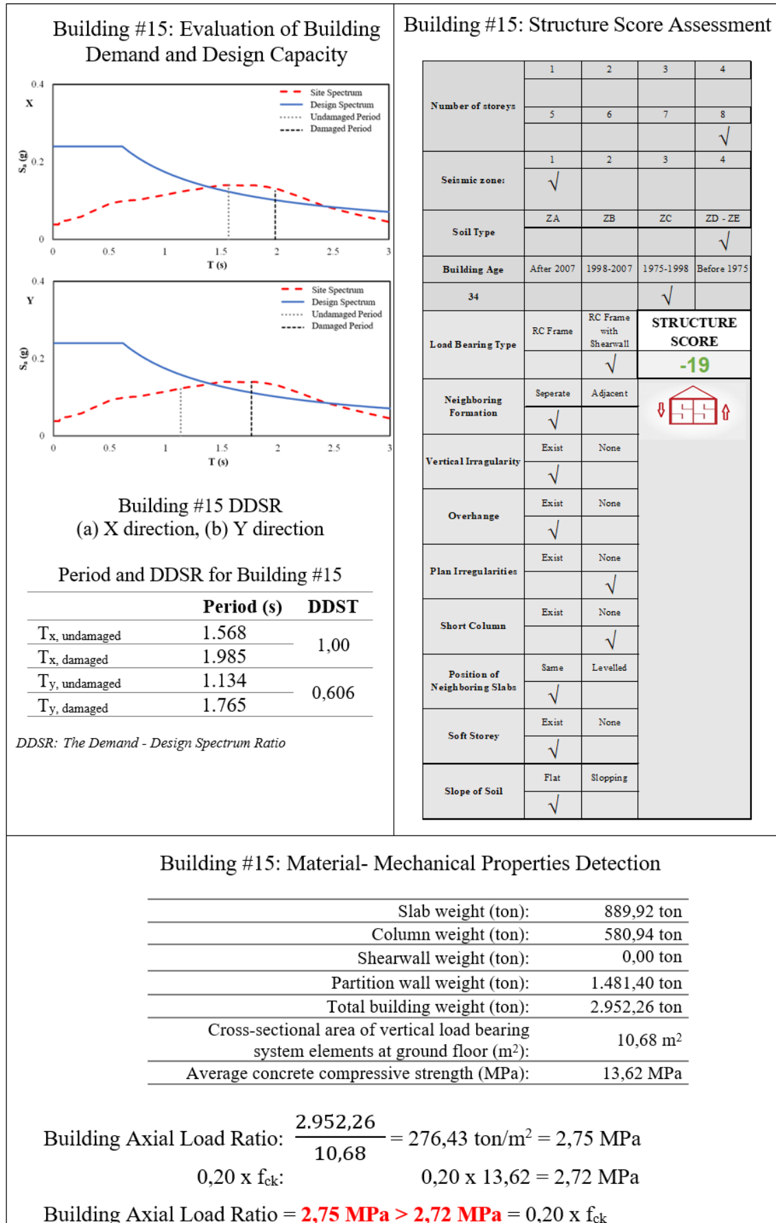
Figure 6.30. Calculation of three-stage evaluation score for Building #15
