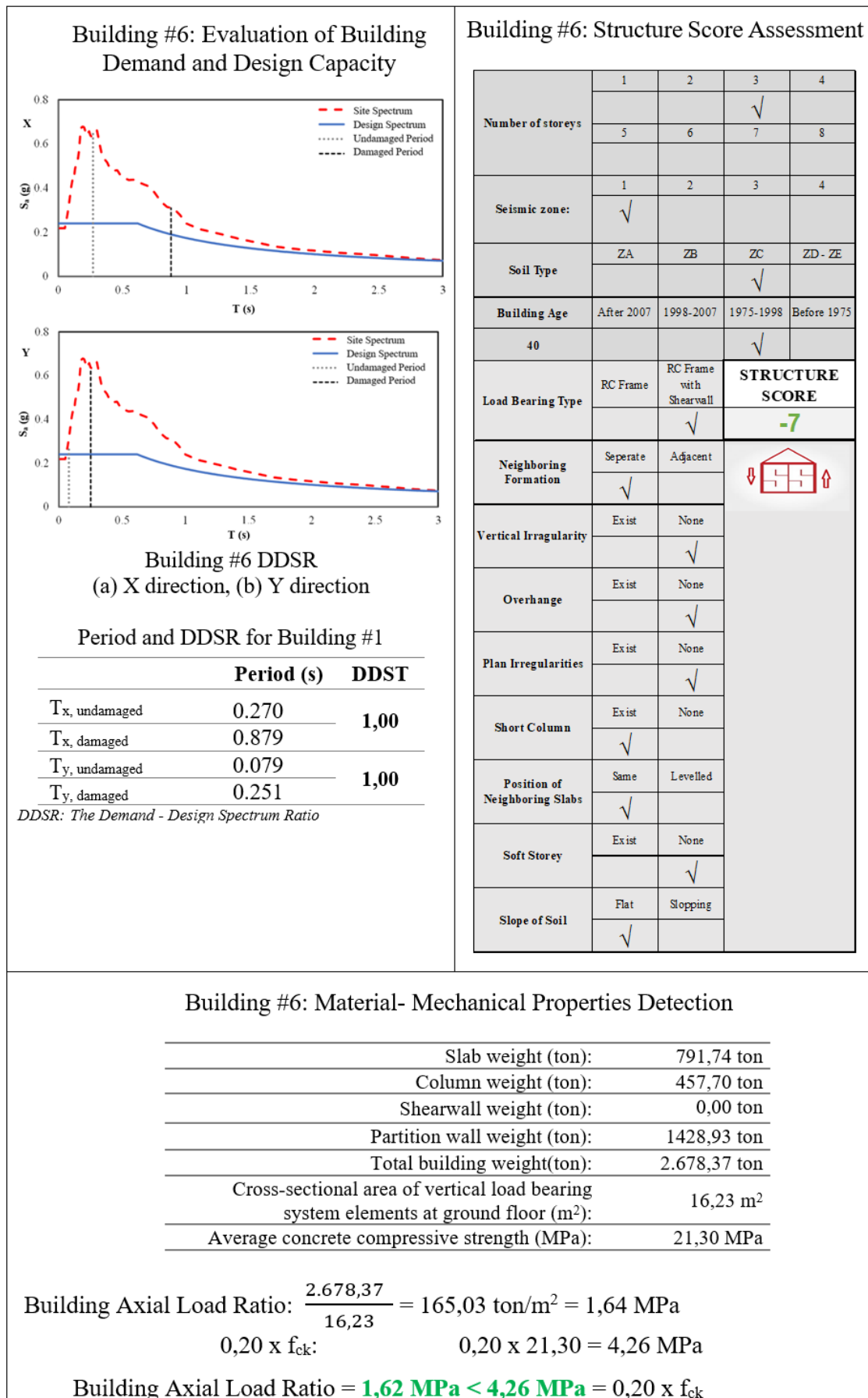
Figure 6.12. Calculation of three-stage evaluation score for Building #6
