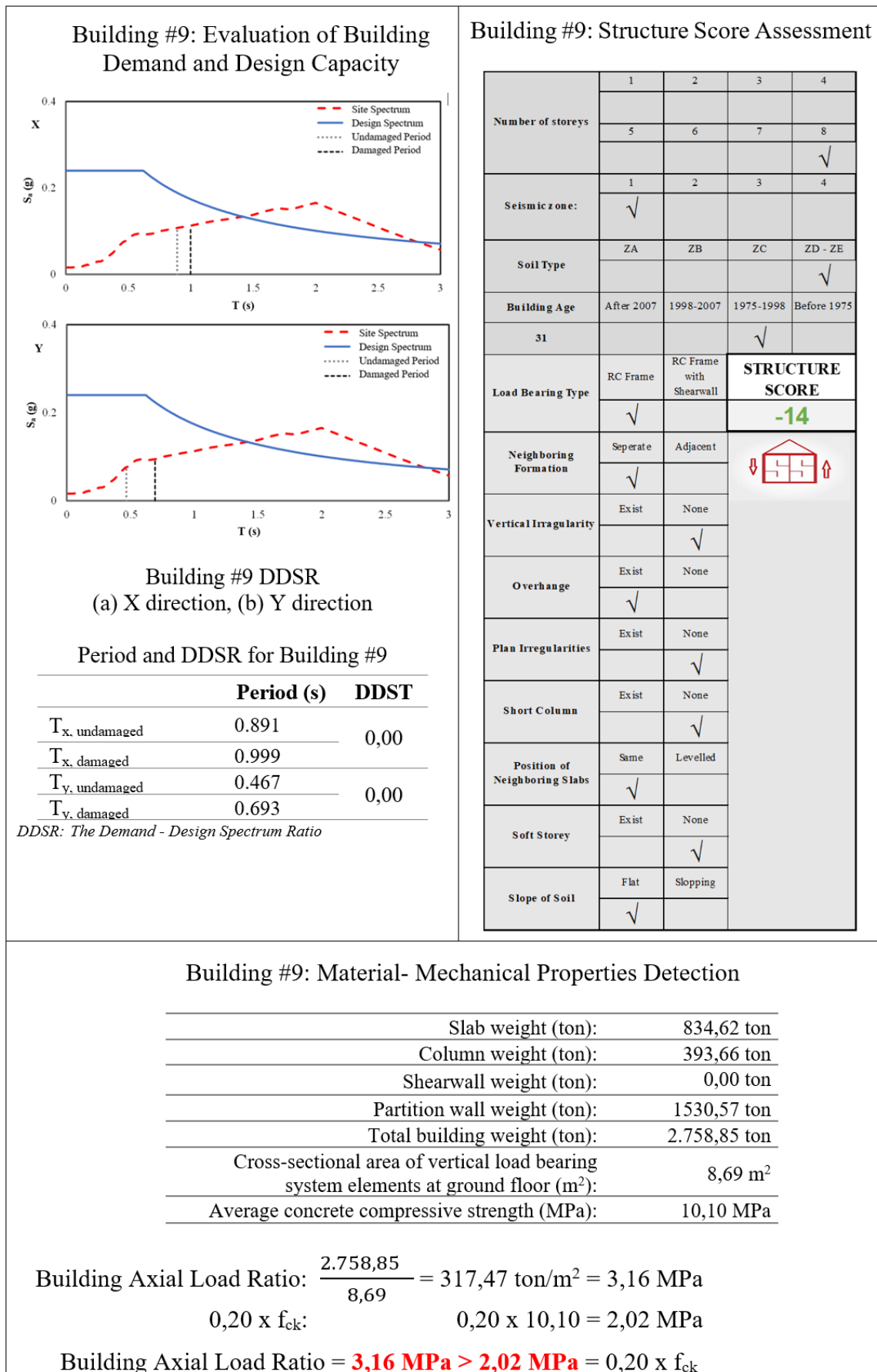
Figure 6.18. Calculation of three-stage evaluation score for Building #9
