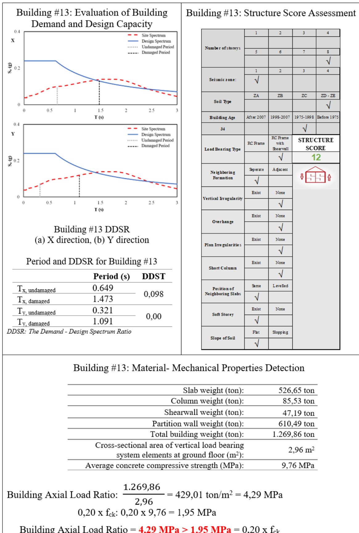
Figure 6.26. Calculation of three-stage evaluation score for Building #13
