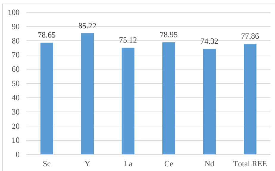
Figure 4.11 Recoveries of Sc, Y, La, Ce, Nd, and Total REE of Asphaltite Fly Ash subjected to 10% Sulfuric Acid leaching in 90°C for 24 h
