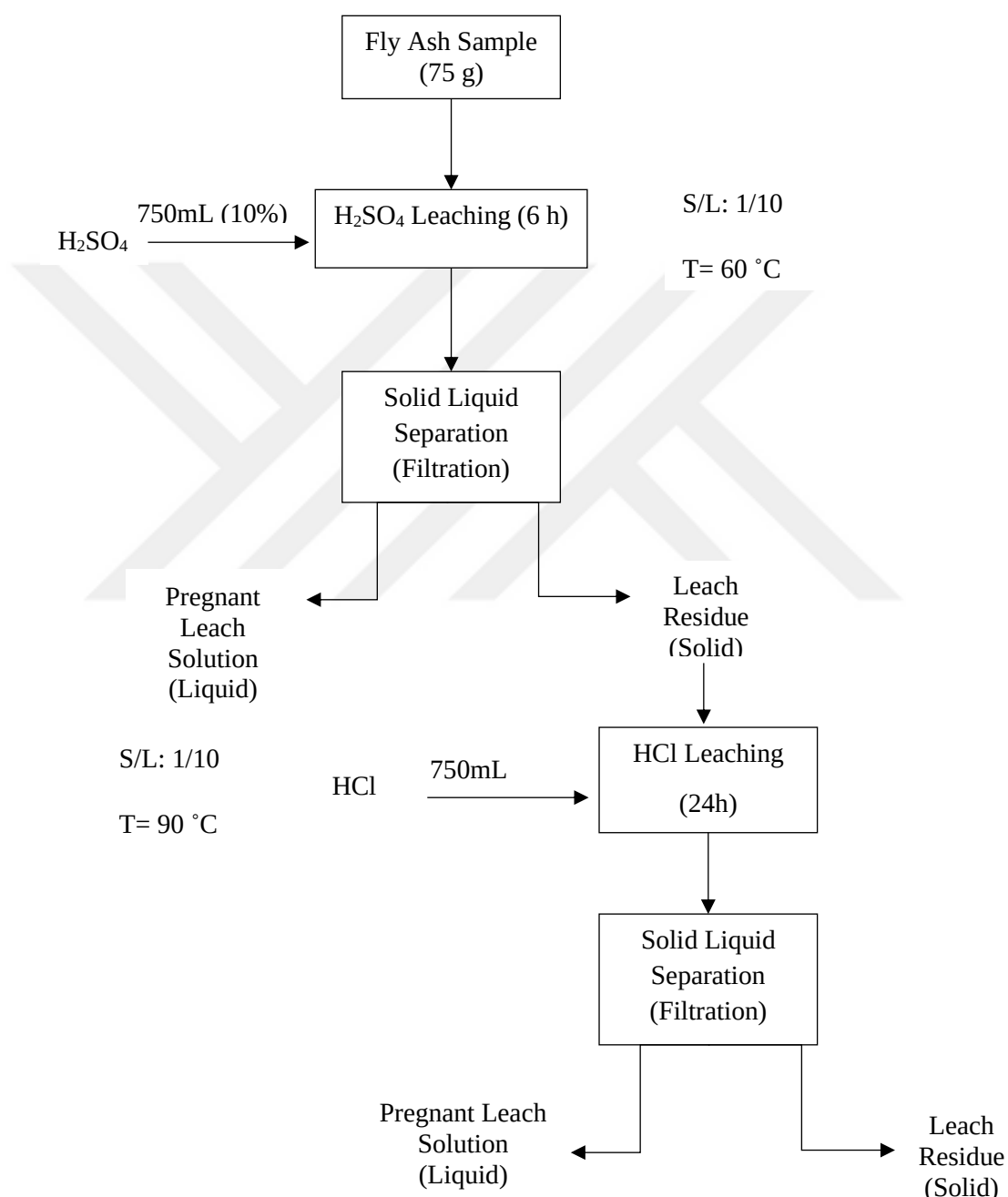
Figure 3.22 Flowsheet of Sequential Leaching
