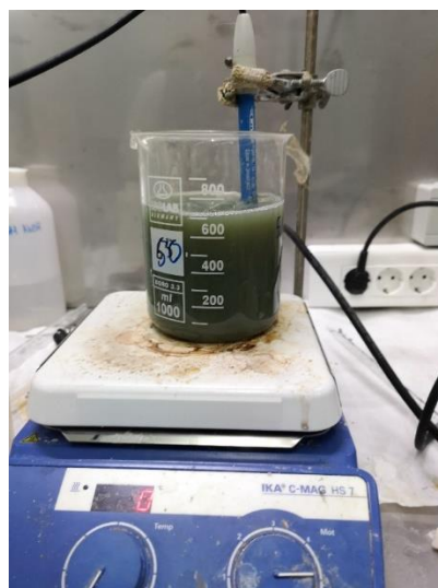
Figure 3.23 Neutralization - Selective Precipitation Tests Experimental Setup
