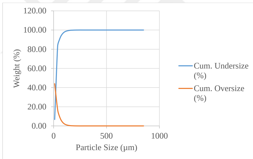
Figure 3.13 Particle size distribution of Asphaltite Fly Ash
