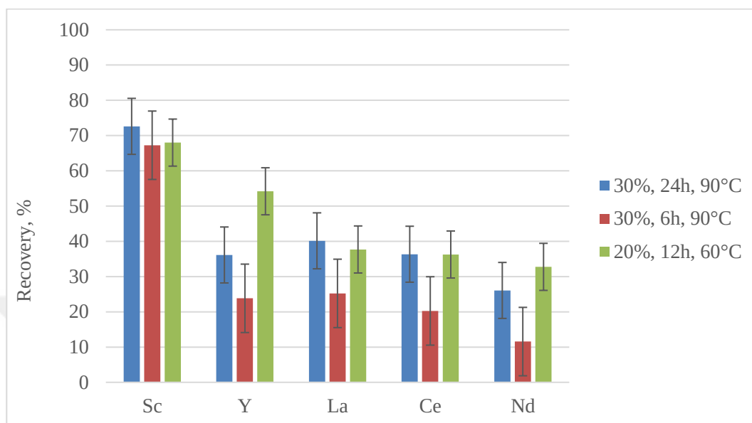
Figure 4.1 Recoveries of Sc, Y, La, Ce, Nd of Lignite Fly Ash after Sulfuric Acid Leaching Experiments
