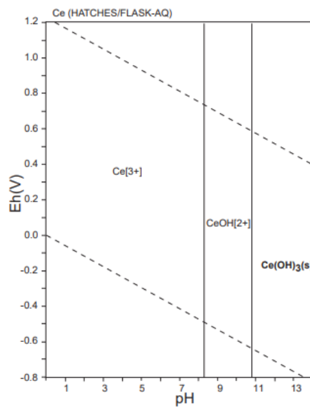
Figure 4.63. Eh-pH diagram of the system Ce-O-H. \text{Ce} = 10^{-10} , 298.15K, 10^5 Pa. (Takeno, 2005)
