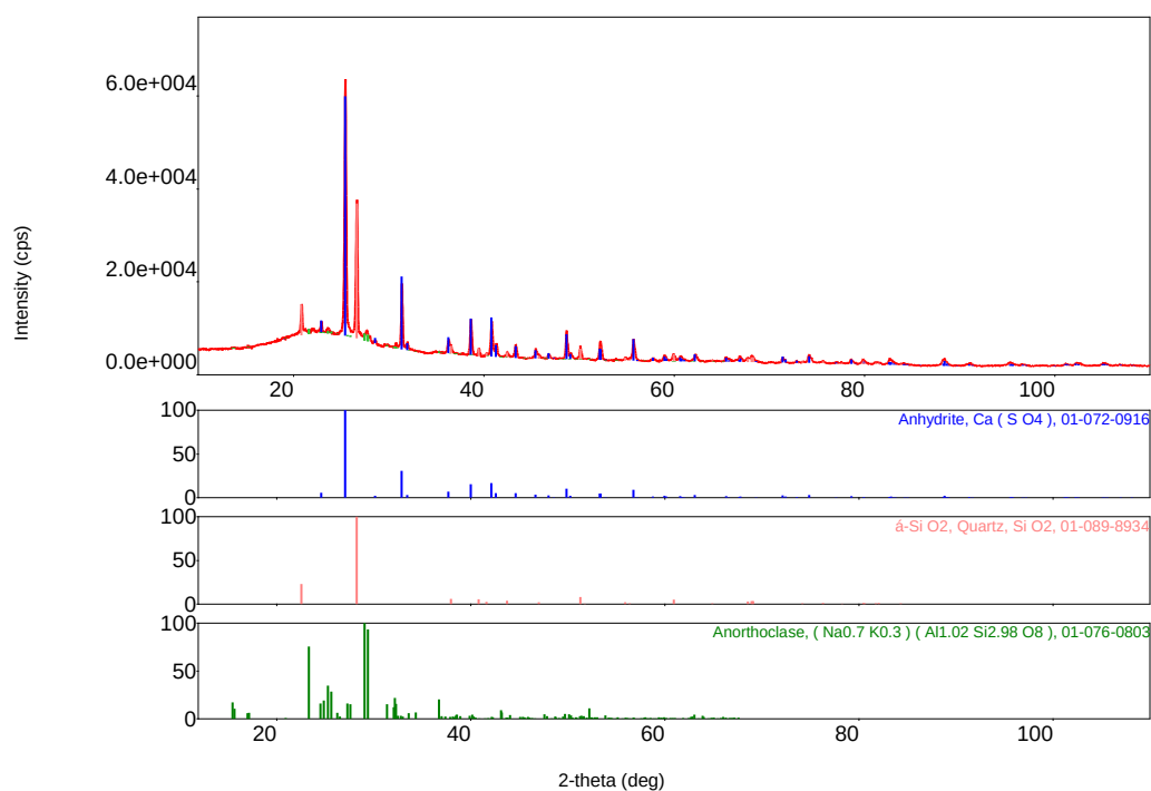
Figure 4.35 XRD Result of Lignite Fly Ash after Sequential Leaching Experiments
