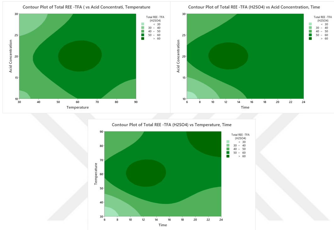
Figure 4.18 Contour Graphs of Hard Coal Fly Ash after Sulfuric Acid Leaching Experiments (Minitab Software)
