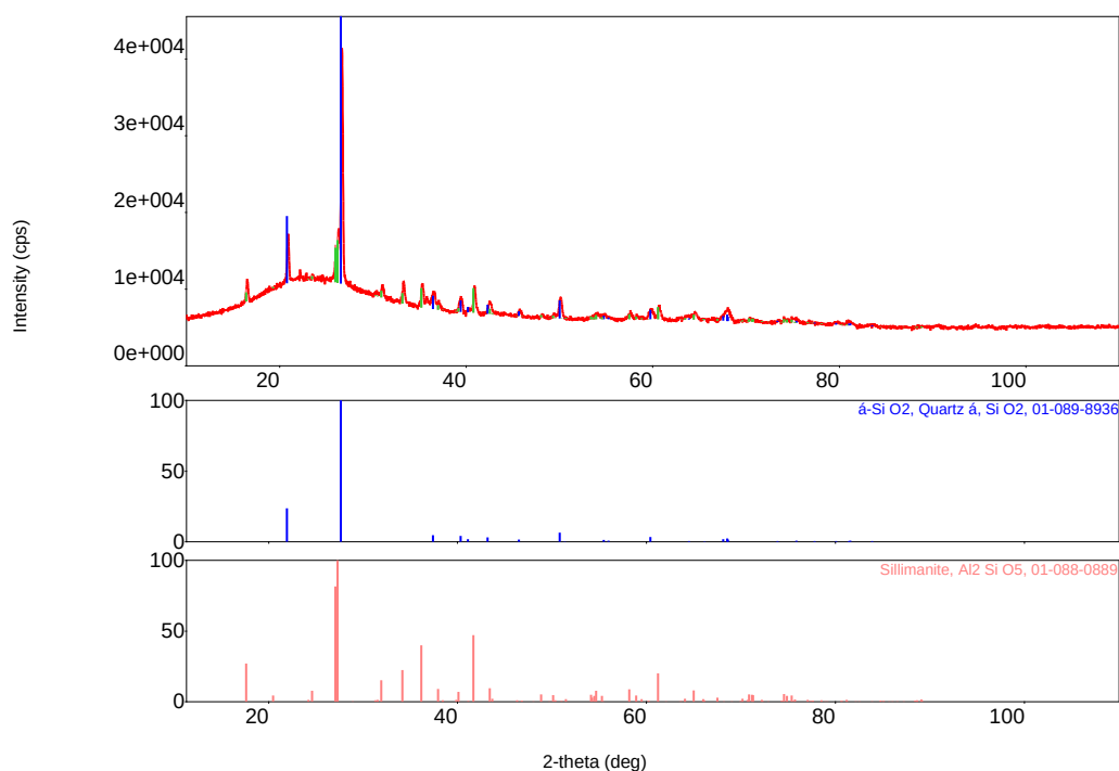
Figure 4.33 XRD Results of Hard Coal Fly Ash after Citric Acid Leaching Experiments
