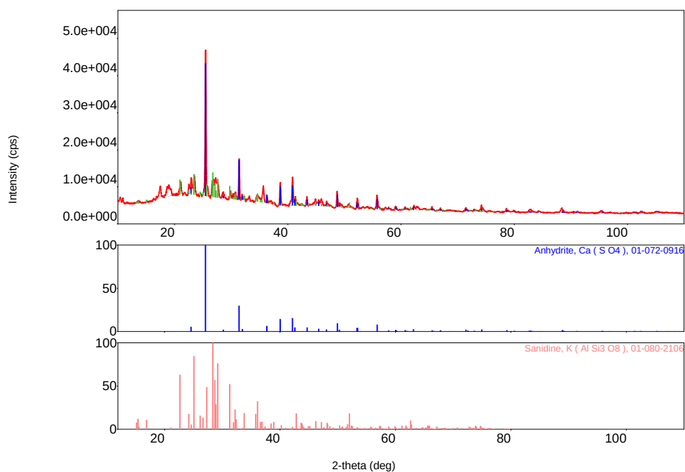
Figure 4.30 XRD Results of Asphaltite Fly Ash after Citric Acid Leaching Experiments
