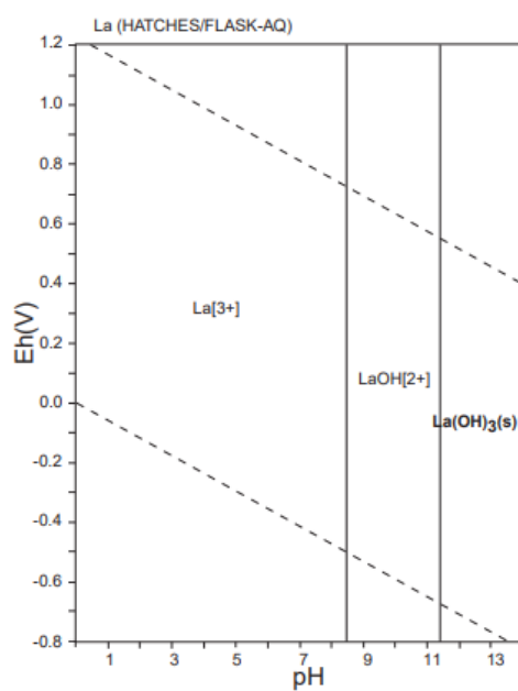
Figure 4.64. Eh-pH diagram of the system La-O-H. \text{La} = 10^{-10} , 298.15K, 10^5 Pa. (Takeno, 2005)
