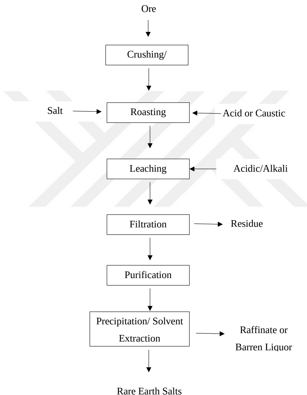
Figure 2.3 Flowsheet of a rare earth element processing (Kumari, et al., 2015)
