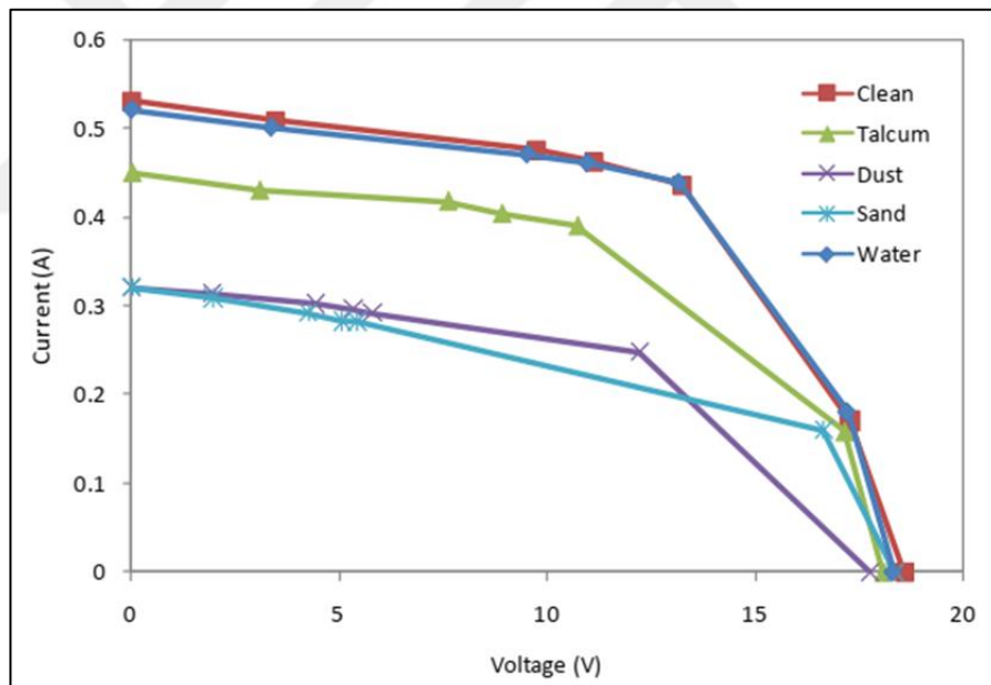
Figure 5.17. I-V characteristic at radiation intensity of 250 W/m² [69].
