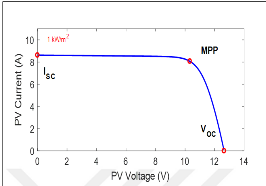
Figure 3.6. PV cell I-V curve ( G = 1000 \text{ W/m}^2 and T = 25^\circ\text{C} ).
