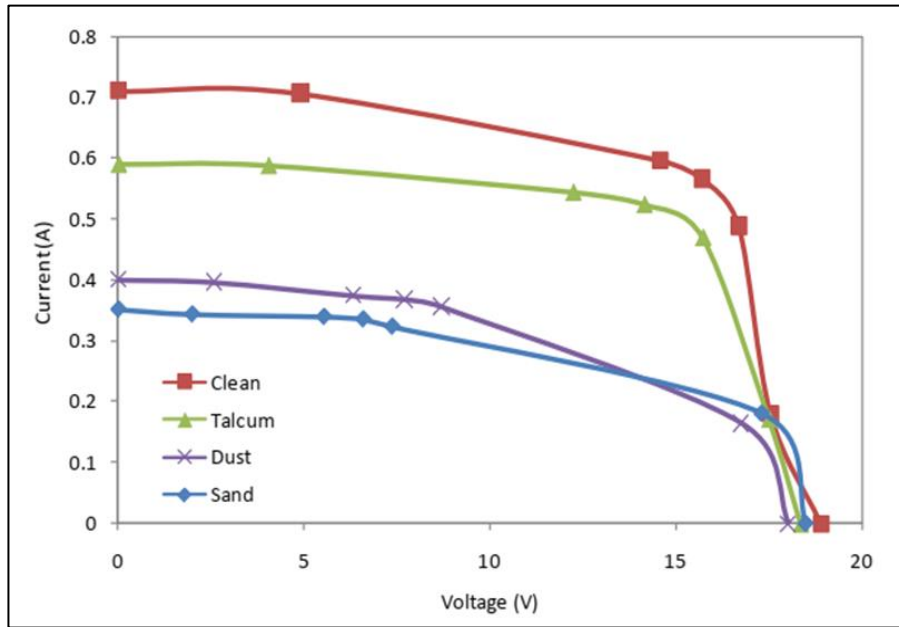
Figure 5.16. I-V characteristic at radiation intensity of 310 W/m² [69].
