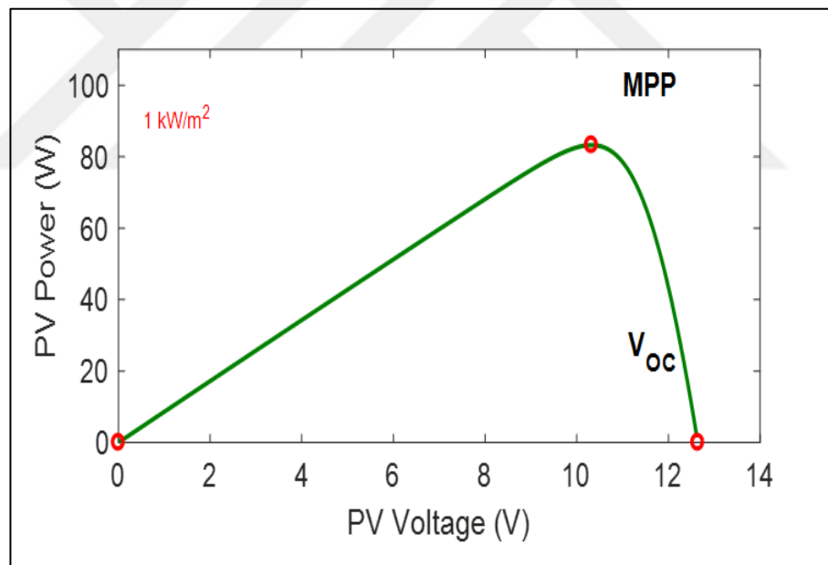
Figure 3.7. The PV cell's power-voltage graph with a fixed temperature and irradiance of T = 25^\circ\text{C} and G = 1000 \text{ W/m}^2 .
