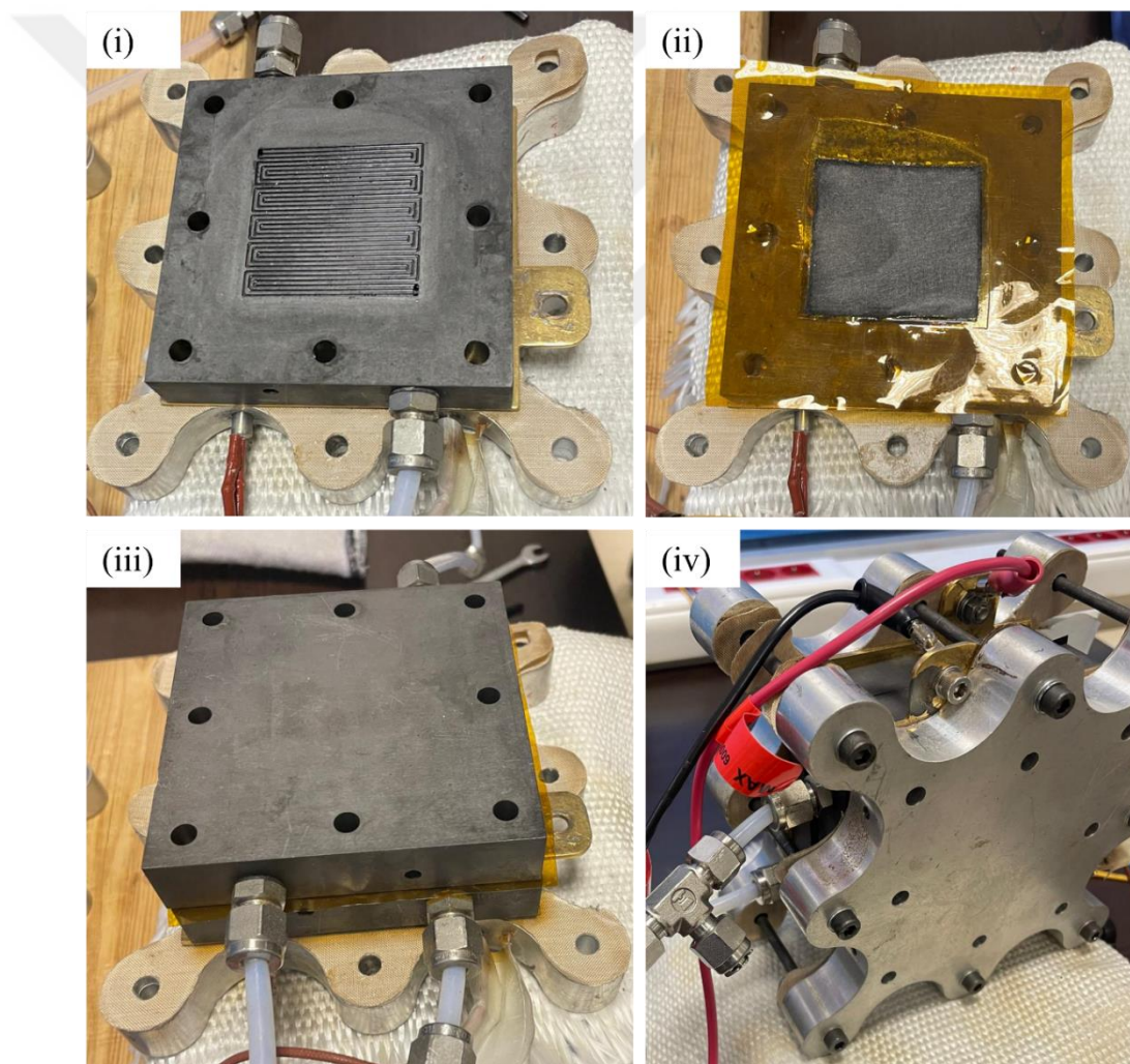
Figure 4.3 HT-ECHP test cell preparation
