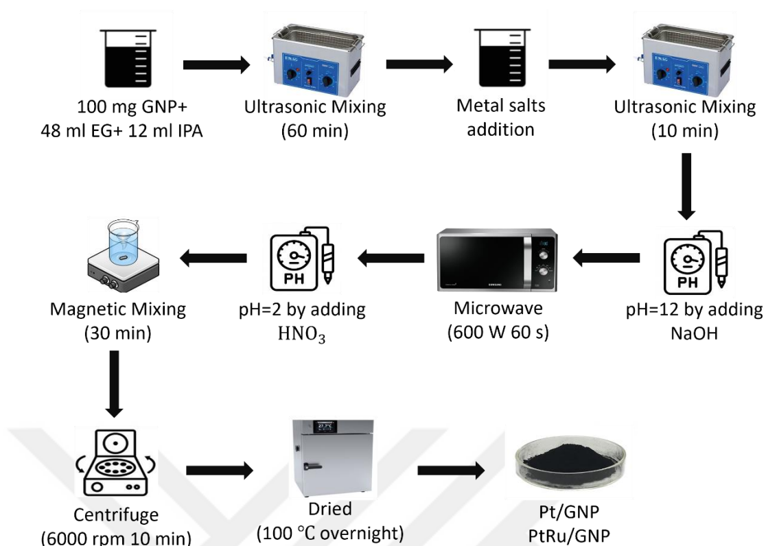
Figure 4.1 Catalyst synthesis steps
