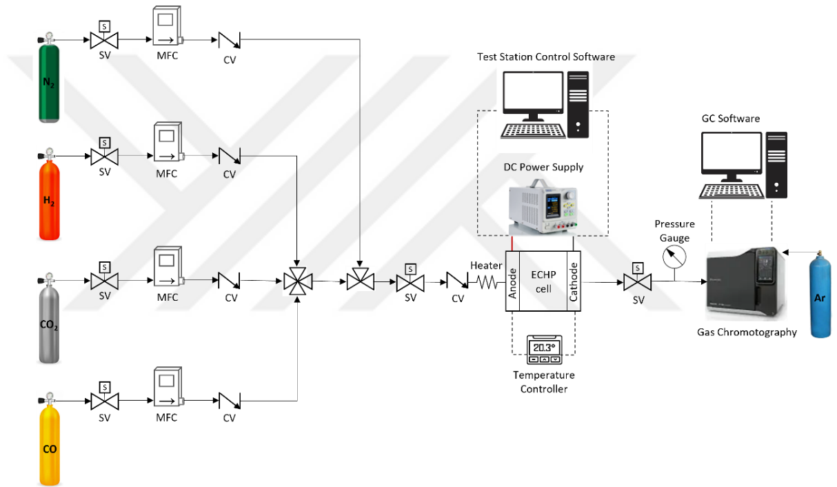
Figure 4.5 HT-ECHP test station diagram
