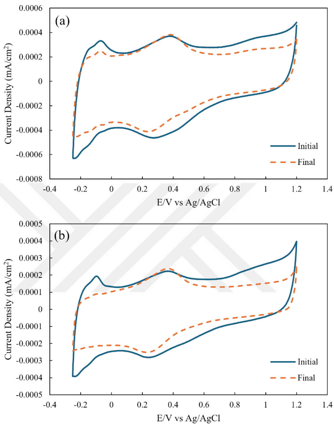
Figure 5.5 CV curves of a) Pt/GNP and b) PtRu/GNP with 100 mV/s between -0.25-1.2 V in 0.1 M HClO 4 solution at 25 C for the 100 th and 1000 th cycles
