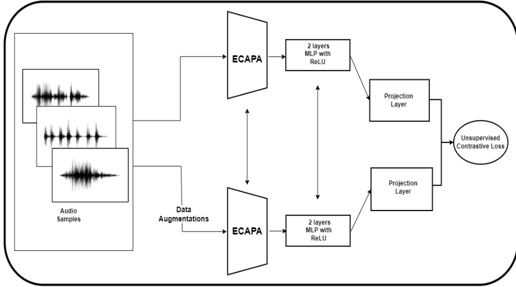
Figure 4.4 First phase of the 2-stage loss optimization
