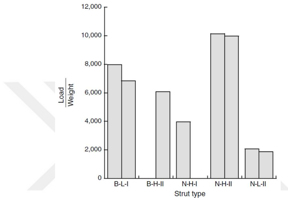
Figure 2.13 Structural efficiency of struts
