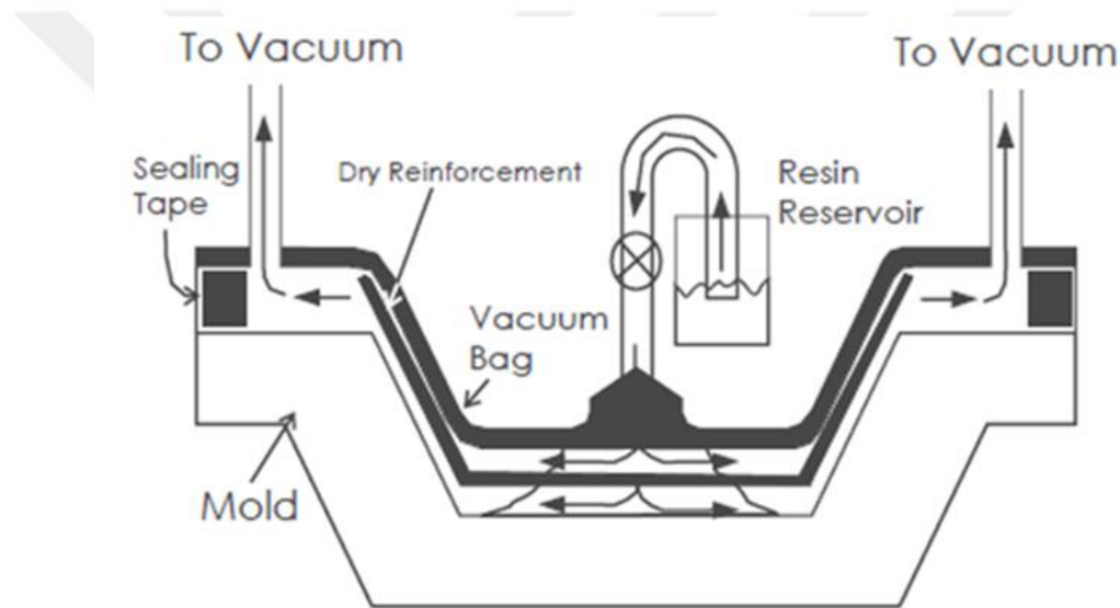
Figure 2.8 VARTM process
