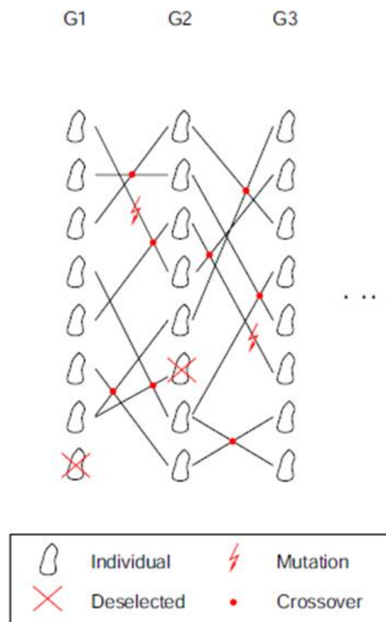
Figure 6.3 An illustration of the genetic algorithm flow.(Source: Dynardo, 2020)
