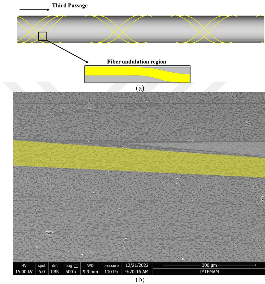
Figure 7.19 Fiber undulation representation (a) schematic drawing, and (b) SEM images of fiber undulation at the start
