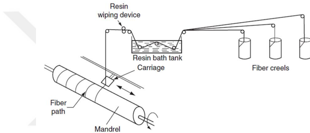
Figure 2.9 Filament winding setup. (Source: Mallick, 2007)
