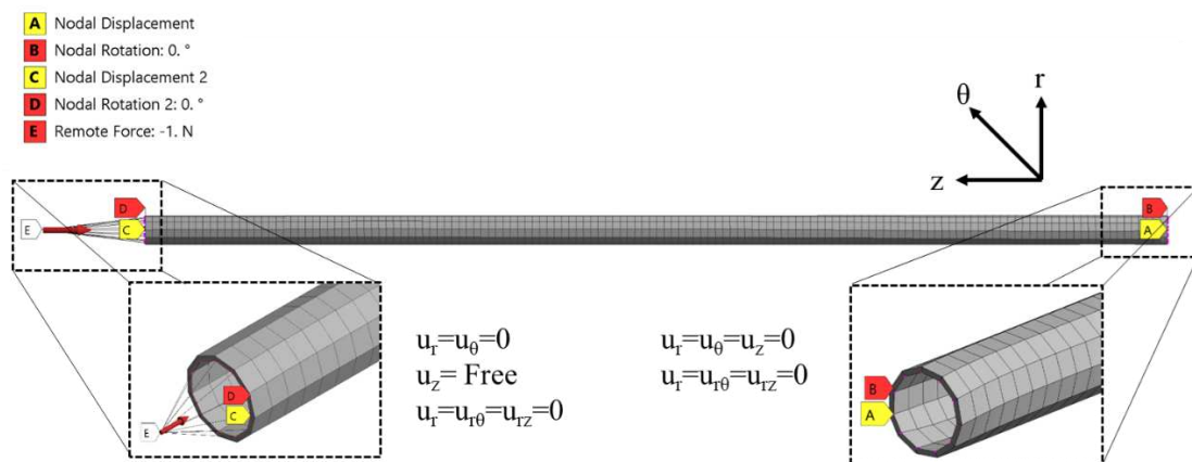
Figure 5.4 Boundary conditions of linear buckling model
