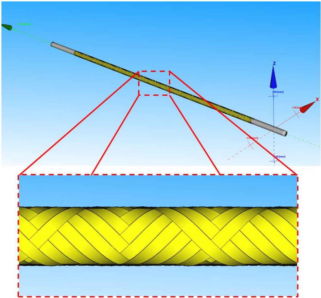
Figure 3.9 Filament winding simulation of [\pm 45]_6 reference rod by means of CADWIND
