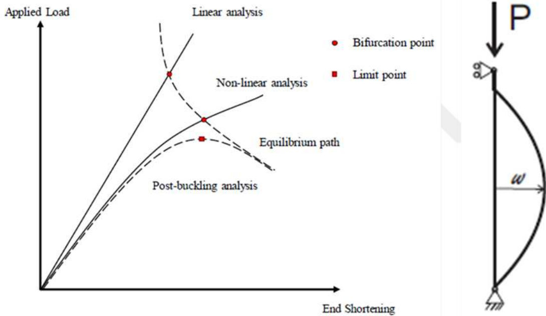
Figure 4.3 Equilibrium paths for the perfect column.
