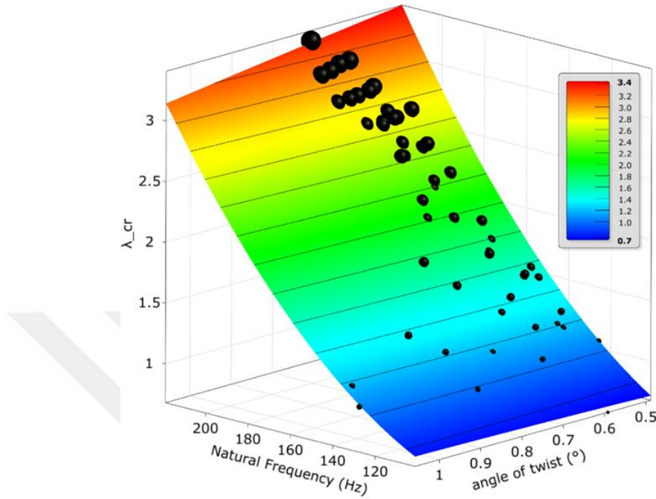
Figure 7.11 Optimization results with respect to design constraints
