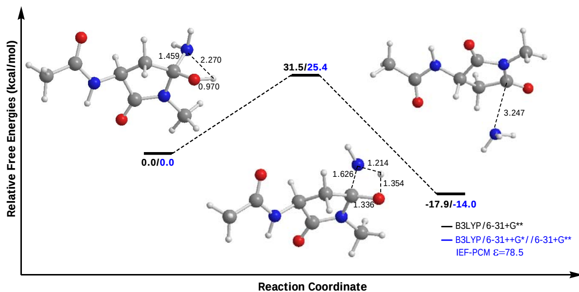
Figure 4.19. Potential free energy profile for the deamination without explicit \text{H}_2\text{O} molecules.
