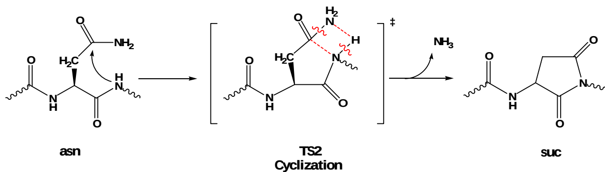
Figure 5.5. Succinimide formation – single-step mechanism ( asn \rightarrow suc ).
