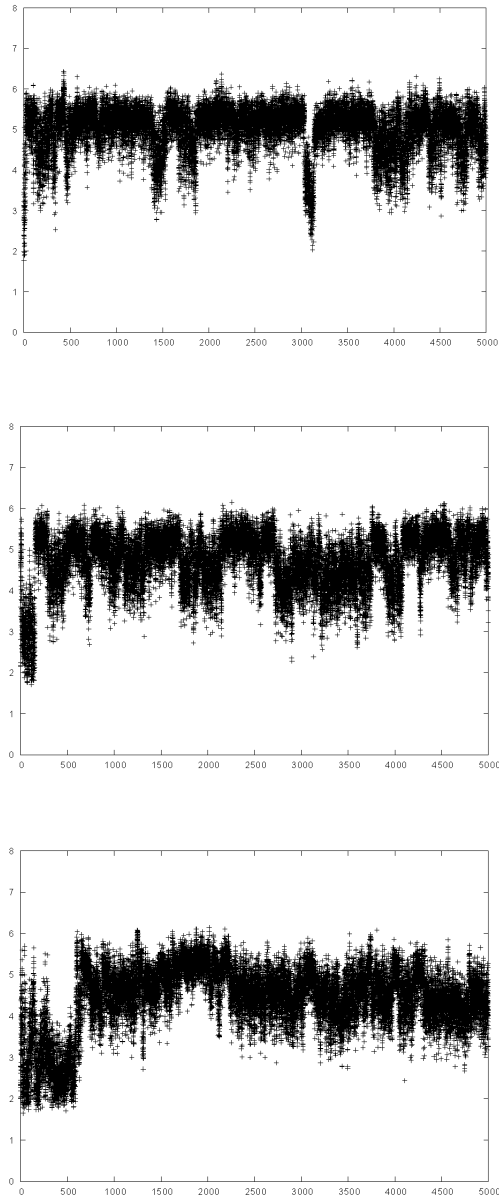
Figure 7.9. Critical distances \text{O}^{25}\text{-H}^{32} .
