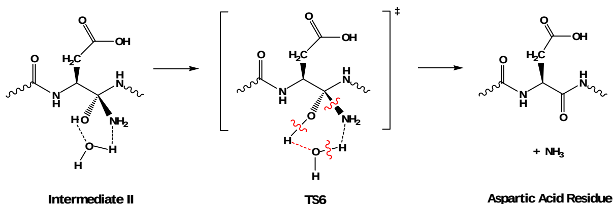
Figure 6.14. Deamination ( \text{NH}_3 expulsion) at Intermediate II.
