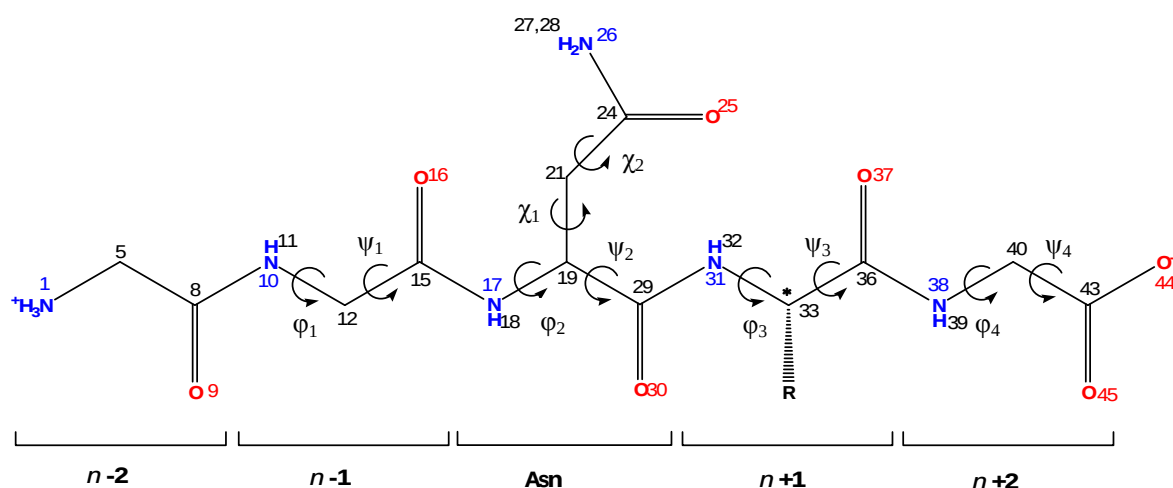
Figure 7.6. Pentapeptide Gly-Gly-Asn-Yyy-Gly.
