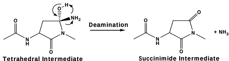
Figure 4.18. Deamination (loss of \text{NH}_3 ) in the tetrahedral intermediate to yield the succinimide intermediate.
