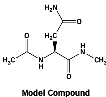
Figure 4.4. Model peptide with L-asparaginyl residue.
