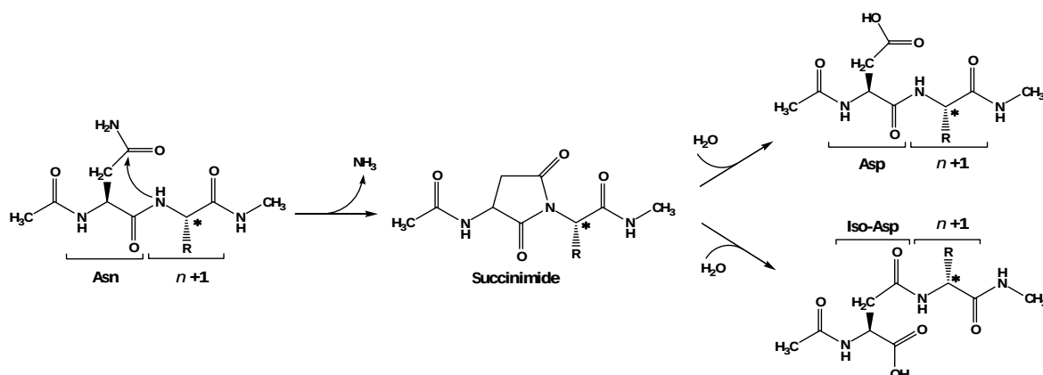
Figure 7.1. Deamidation via a succinimide intermediate.
