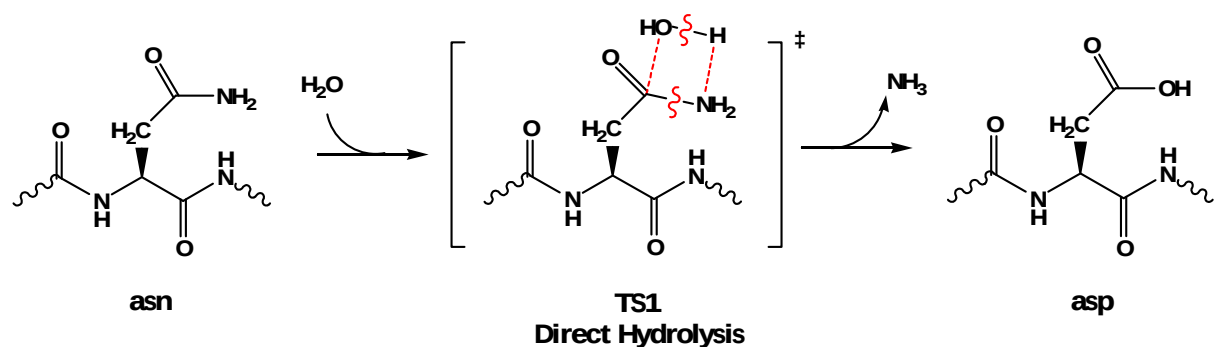
Figure 5.3 Direct hydrolysis of Asn to Asp.
