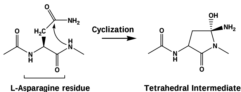
Figure 4.3. Rate determining step for deamidation in neutral media.
