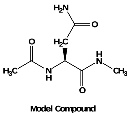
Figure 6.2. Model peptide with Asn residue.
