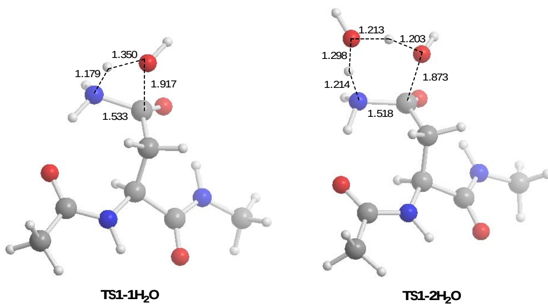
Figure 5.4. Optimized geometries and free energies of activation for the transition state of direct hydrolysis of Asn to Asp ( asn \rightarrow asp ) with one (TS1-1H 2 O) and two (TS1-2H 2 O) water molecules, respectively.
