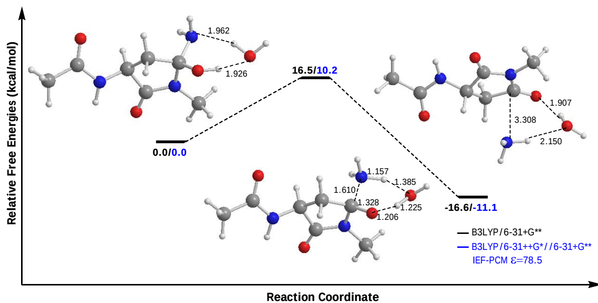
Figure 4.20. Potential free energy profile for the deamination with 1 \text{H}_2\text{O} molecule.
