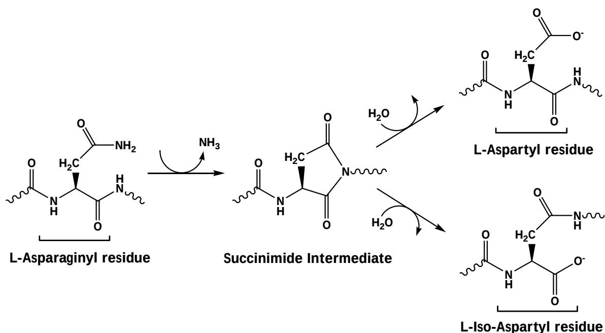
Figure 4.2. Deamidation mechanism.
