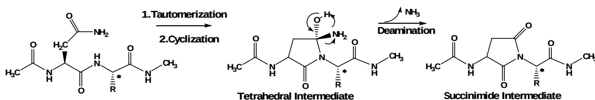
Figure 7.4. Tautomerization route for succinimide formation.
