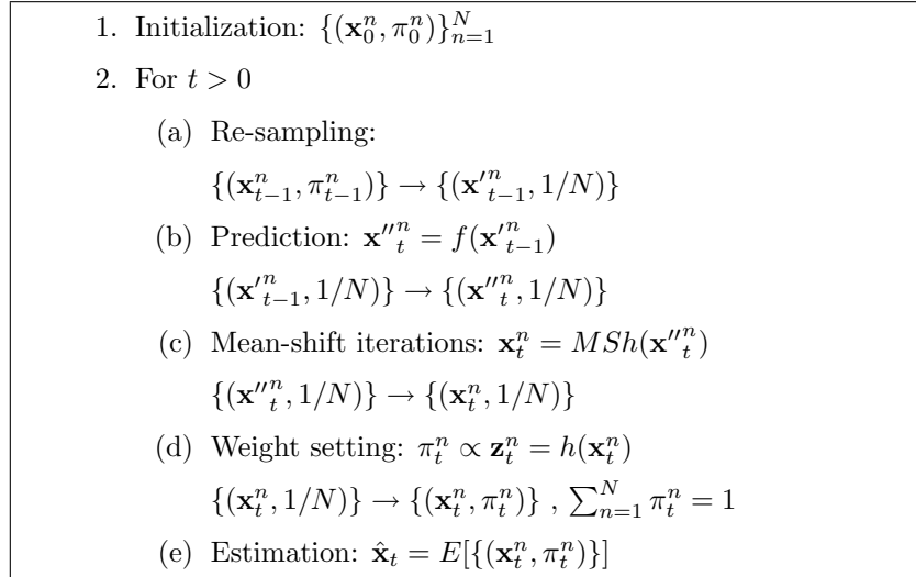
Figure 4.5. Joint PF algorithm
