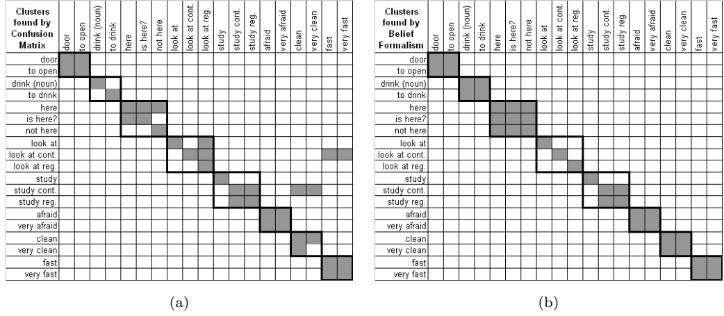
Figure 5.5. Sign clusters (a) identified by the joint confusion matrix of 7-fold CV, (b) identified by the uncertainties between the classes in 7-fold CV. Clusters are shown row-wise, where for each sign row, the shaded blocks show the signs in its cluster. Bold lines show the clusters indicated by prior semantic knowledge, which we do not use
