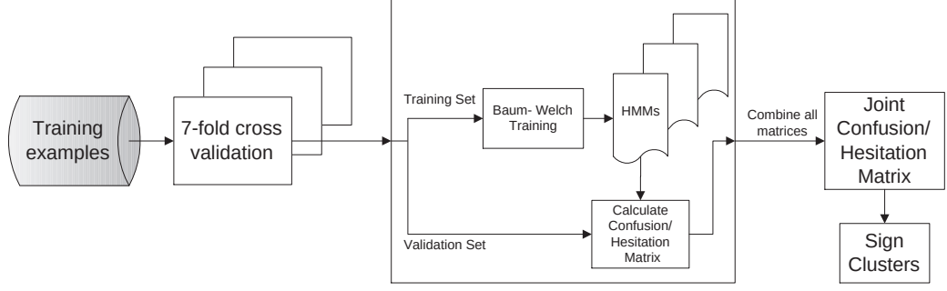
Figure 5.4. Identifying sign clusters by cross validation via confusion or hesitation matrices
