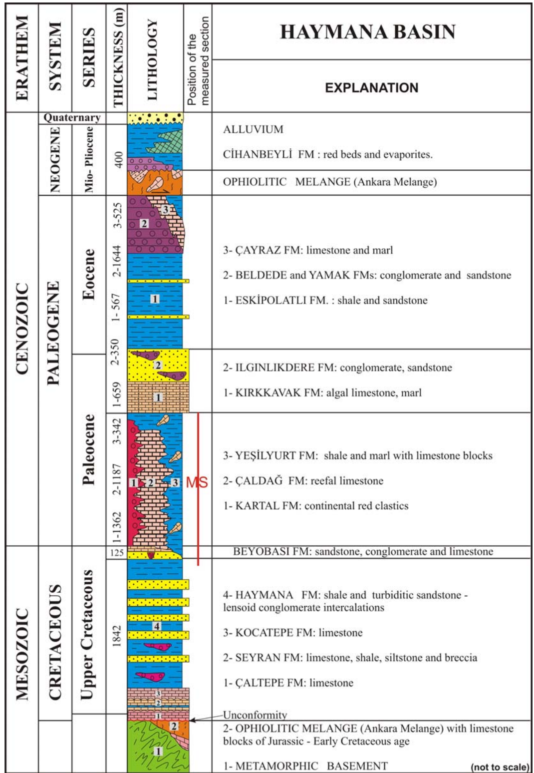
Figure 7. Generalized columnar section of the study area (Haymana basin). The measured section (MS) is shown by the red line (modified from Ünalın et al. , 1976).
