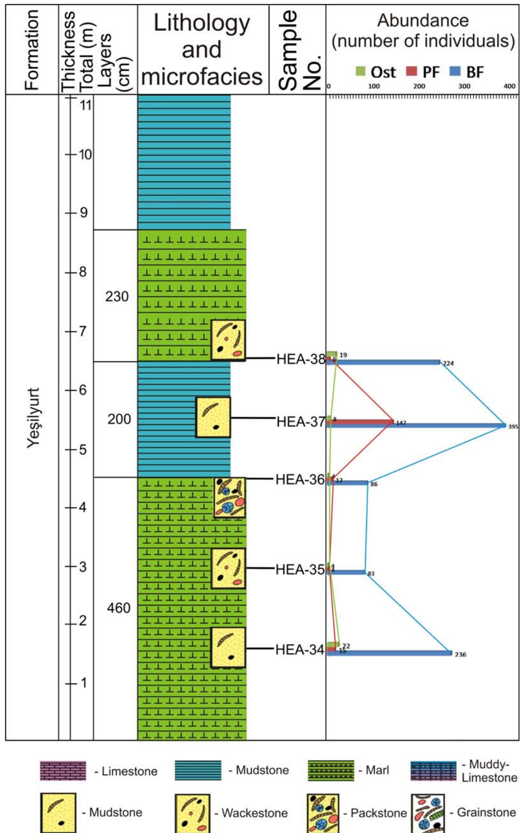
Figure A14. Detailed measured section (continued).
