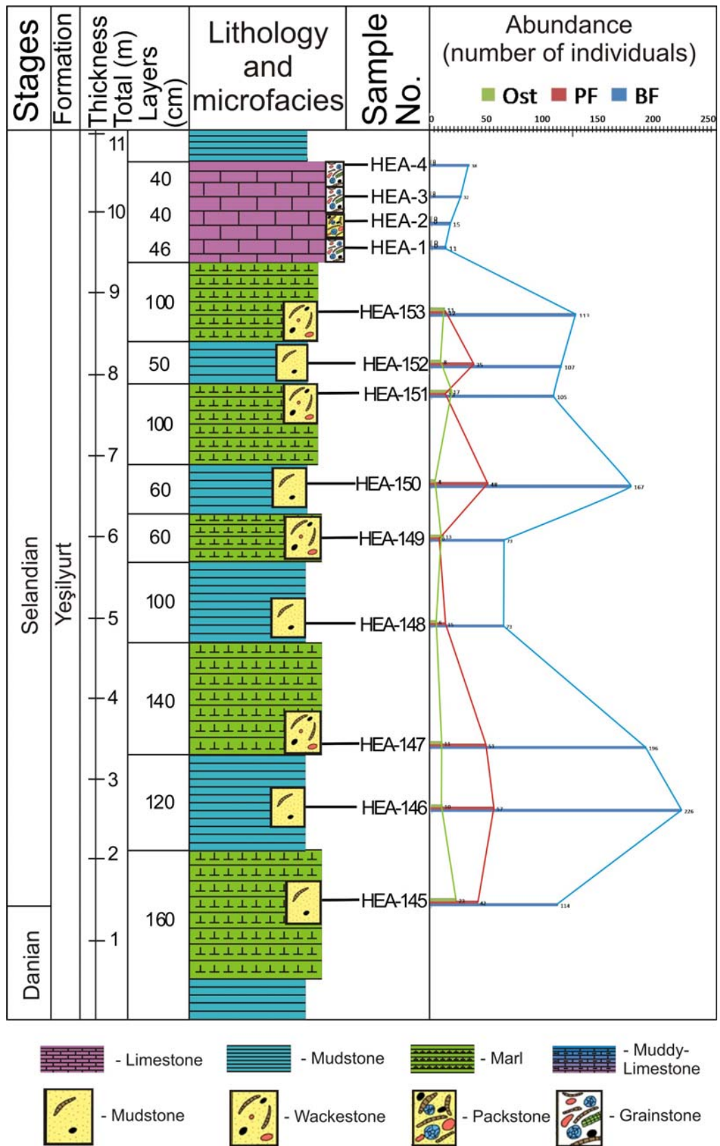
Figure A7. Detailed measured section (continued).
