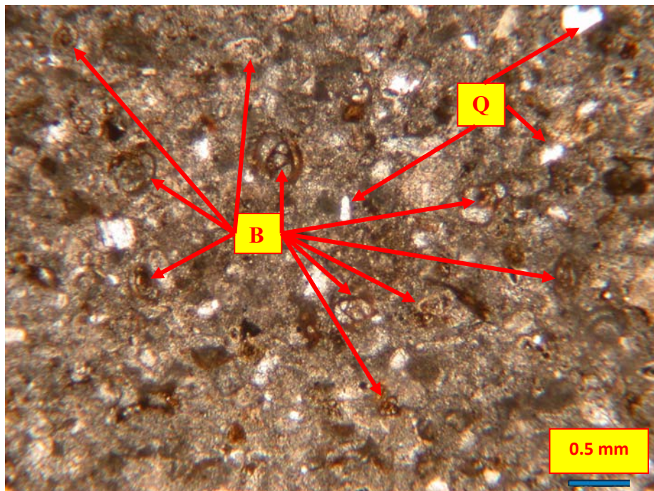
Figure 26. Photomicrograph of the limestone (wackestone), (B-benthonic foraminifera), Q-quartz), (HEA-46).
