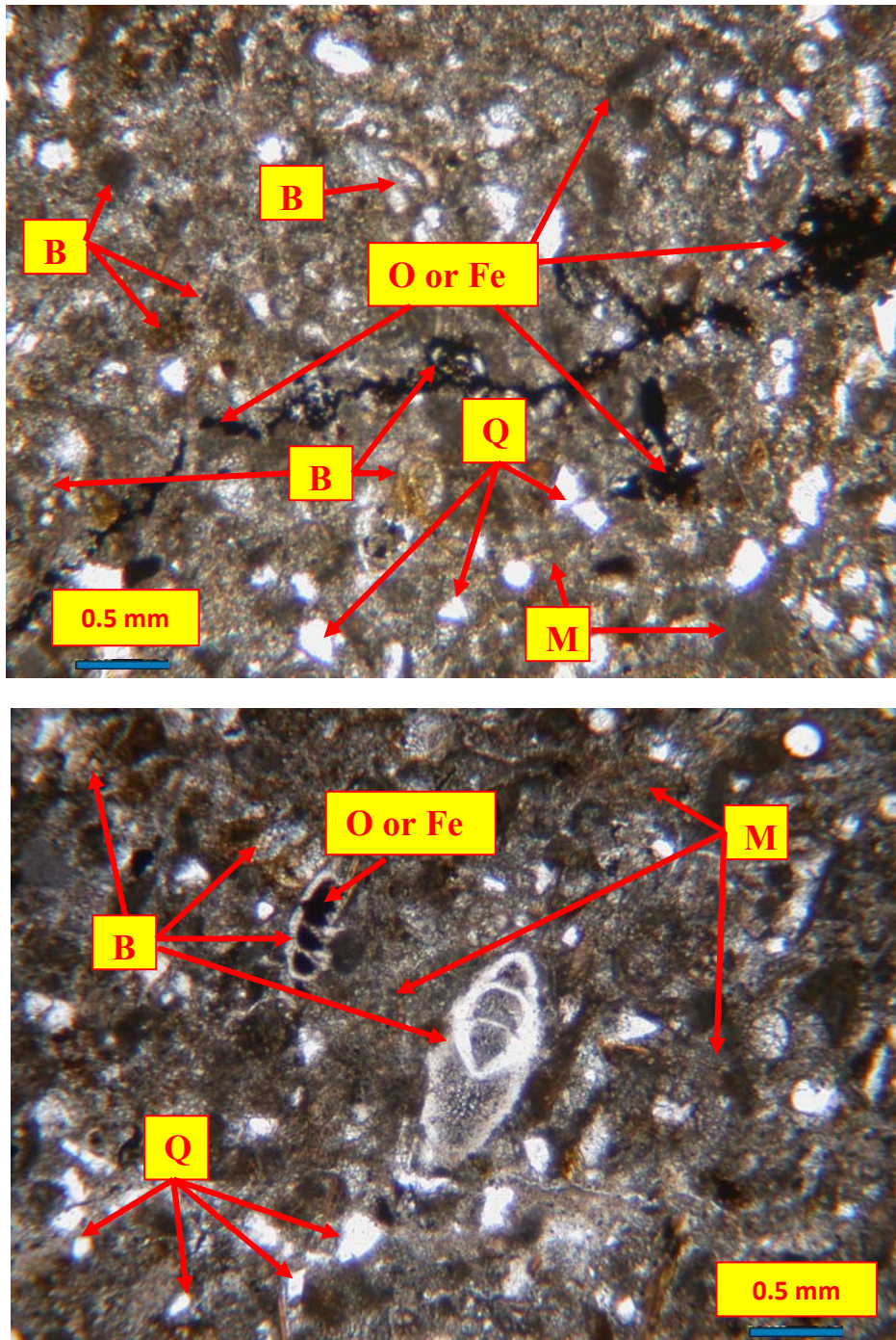
Figure 30. Photomicrographs of the mudstone, (M-matrix, O or Fe-oil impregnation or Fe, Q-quartz, B-benthonic foraminifers), (HEA-33).
