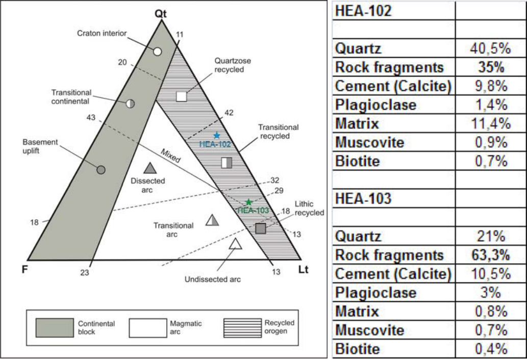
Figure 36. Triangular diagram showing average compositions of sand derived from different provenance terranes (after Dickinson, 1985).
