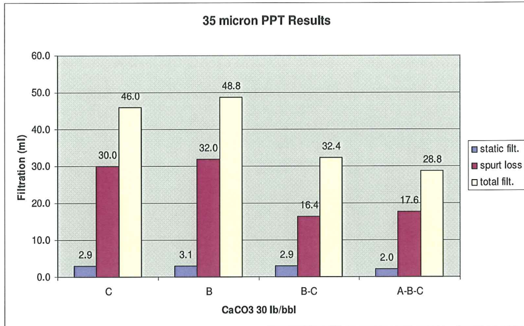
Figure 5-10: Effect of particle size for 35 μ ceramic disks
