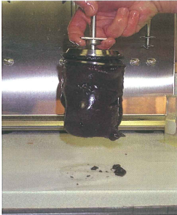
Figure 2-3: Second generation CACP-firm, rubbery and ductile plug (Bruton, Ivan and Heinz, 2001)
