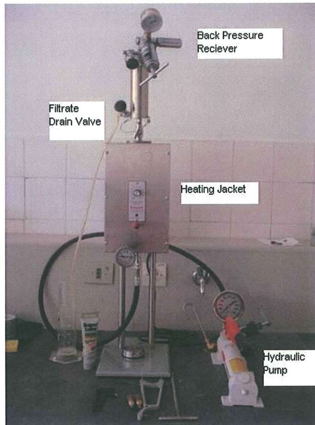
Figure 4-1: Permeability Plugging Apparatus (PPA)
