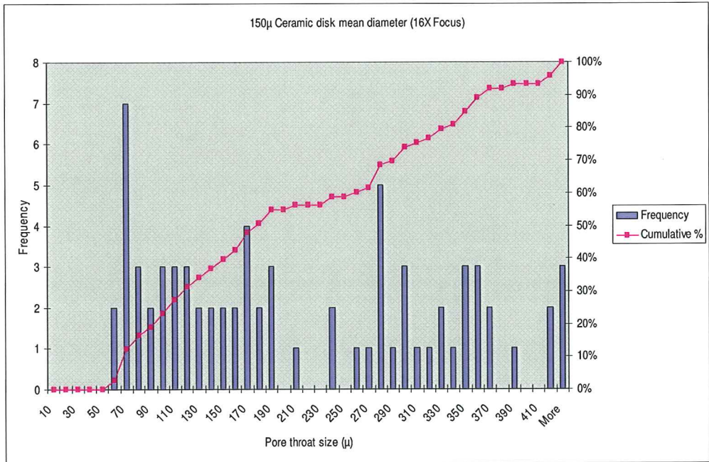
Figure A-19: 150µ Ceramic Disk Mean Diameter (16X Focus)
