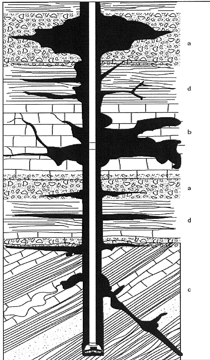
Figure: 2-1: Lost Circulation Sections (MI Drilling Fluids Engineering Manual, Copyright 1998)
