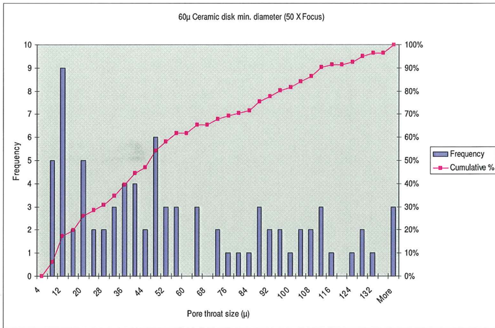
Figure A-14: 60 \mu Ceramic Disk Minimum Diameter (50X Focus)
