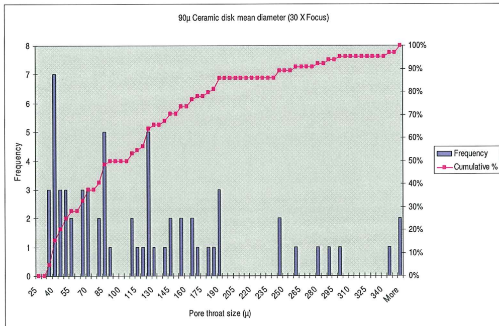
Figure A-17: 90µ Ceramic Disk Mean Diameter (30X Focus)
