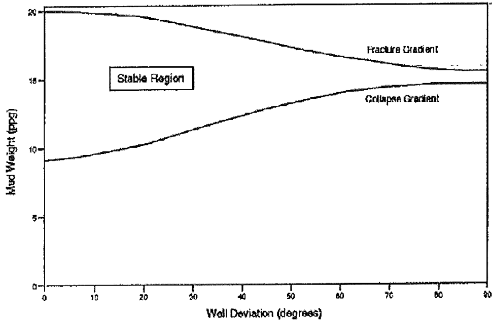
Figure 2-2: The influence of well deviance on wellbore stability (McLean and Addis, 1990)
