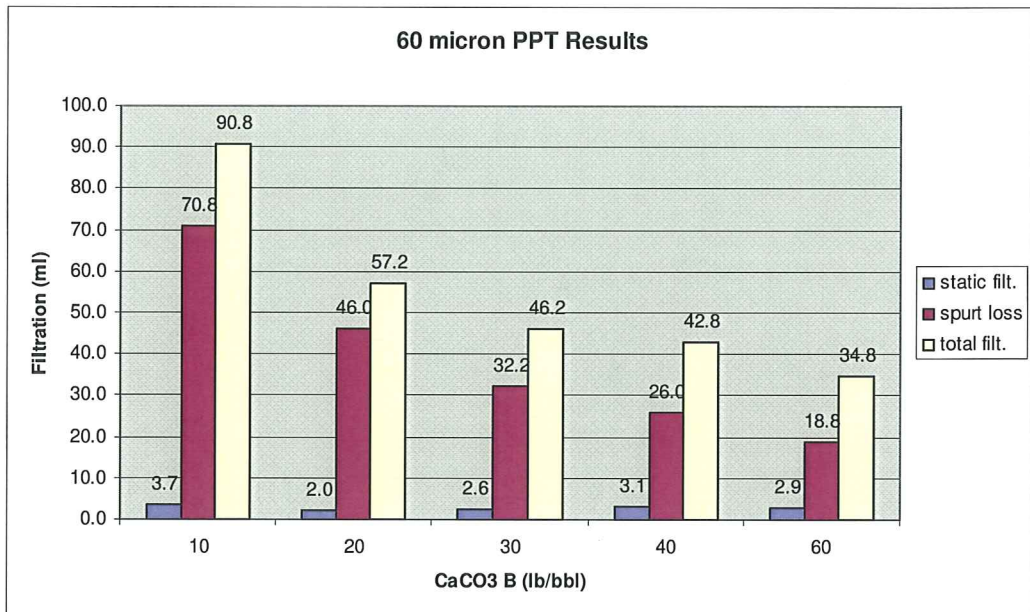
Figure C-4: Effect of Concentration of CaCO 3 B (60 μ Ceramic Disks)
