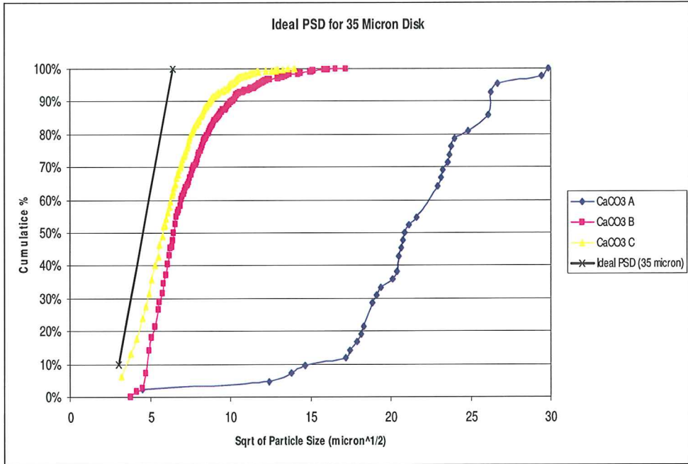
Figure 5-13: Ideal PSD for 35 μ Ceramic Disks & CaCO 3 Grades
