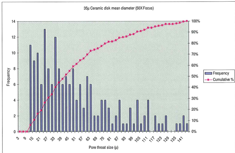
Figure A-7: 35 \mu Ceramic Disk Mean Diameter (50X Focus)
