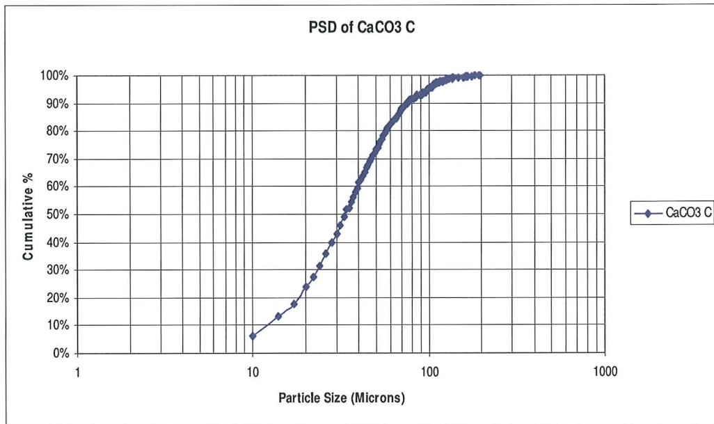
Figure 5-4: PSD of CaCO 3 C
