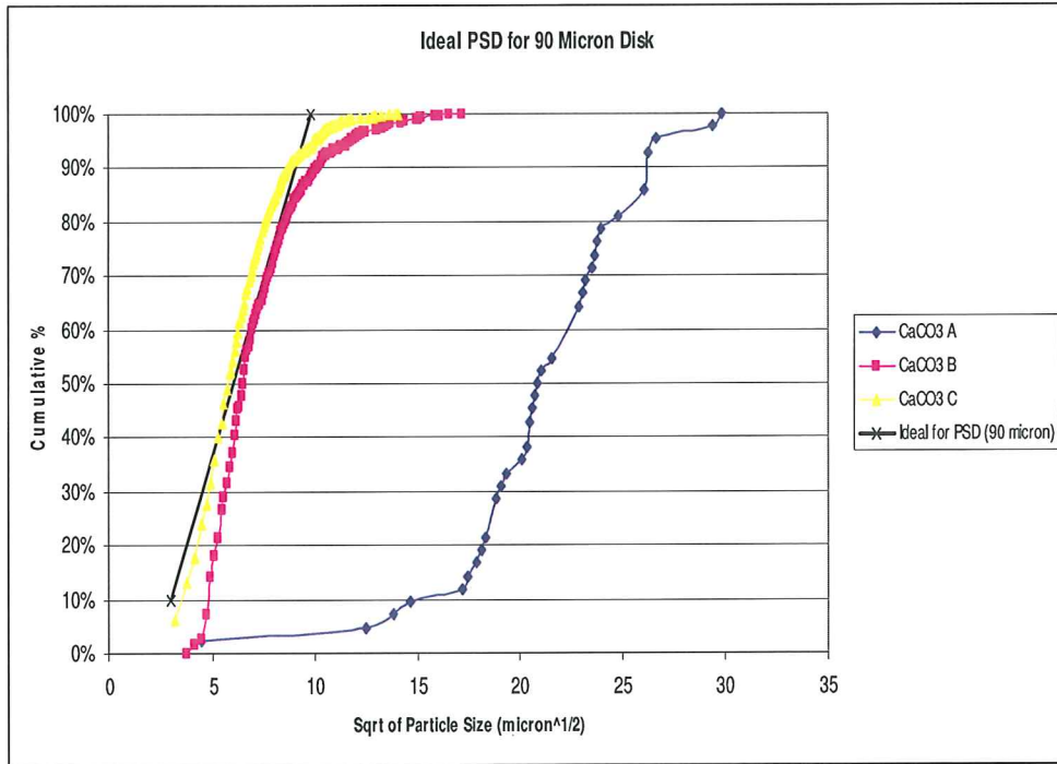
Figure 5-15: Ideal PSD for 90 μ Ceramic Disks & CaCO 3 Grades
