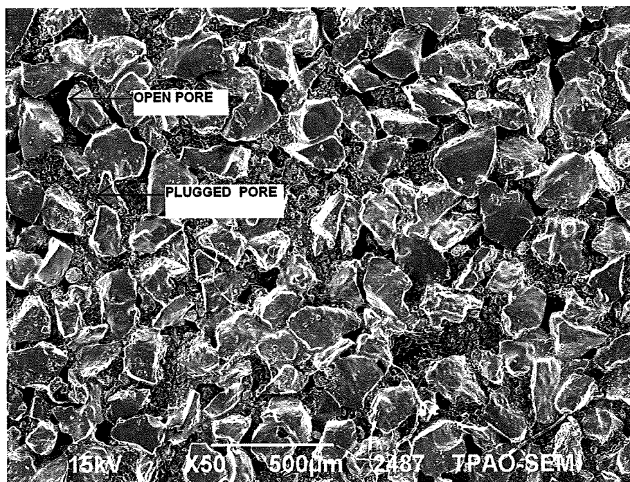
Figure 5-6: 60 μ Ceramic Disk after PPT (30 lb/bbl of CaCO 3 C)
