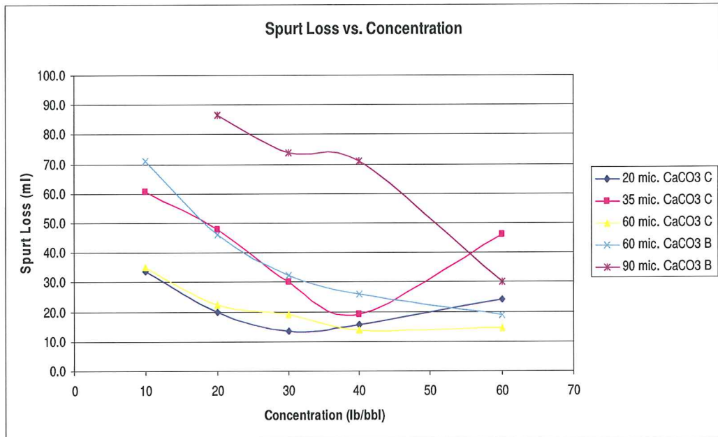
Figure 5-7: Spurt Loss vs. Concentration
