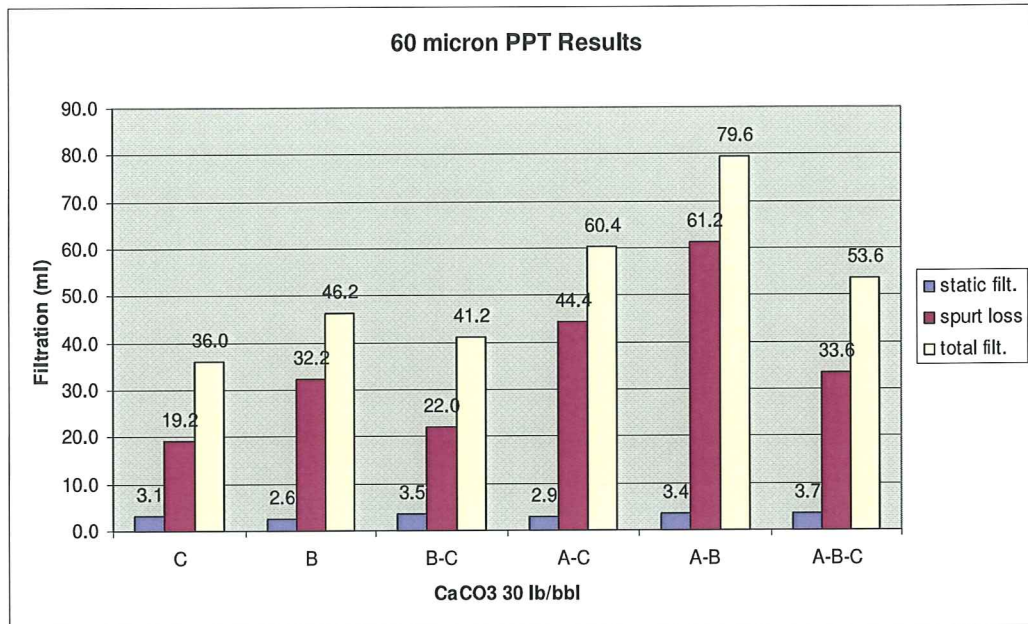
Figure 5-11: Effect of particle size for 60 μ ceramic disks
