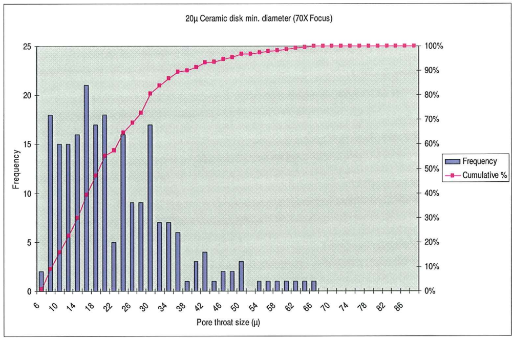
Figure A-4: 20 \mu Ceramic Disk Minimum Diameter (70X Focus)
