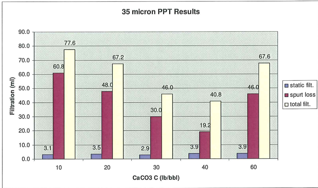
Figure C-2: Effect of Concentration of CaCO 3 C (35 μ Ceramic Disks)
