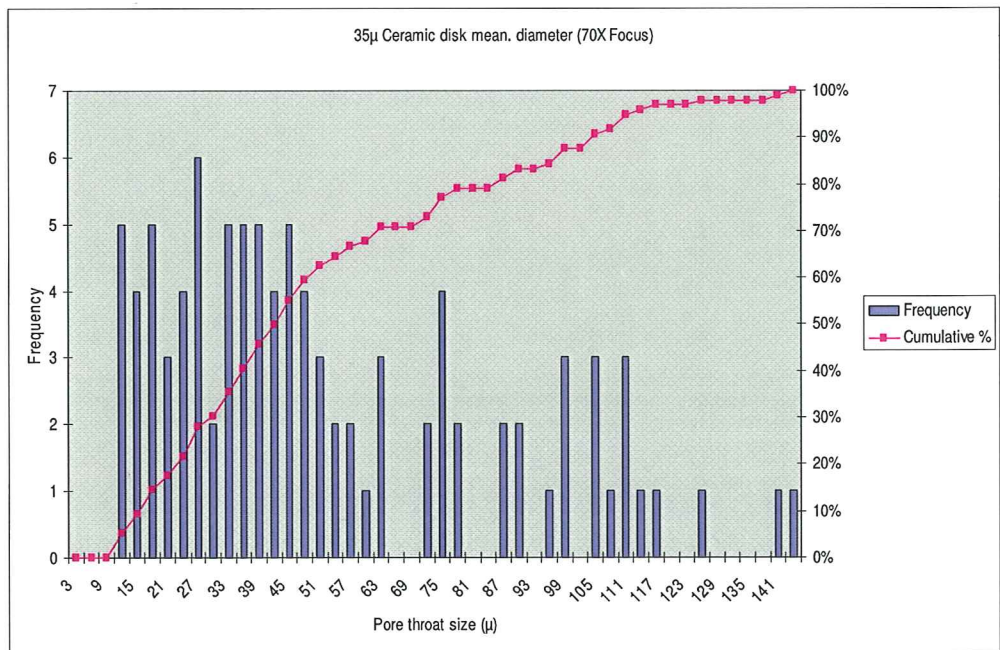
Figure A-9: 35μ Ceramic Disk Mean Diameter (70X Focus)
