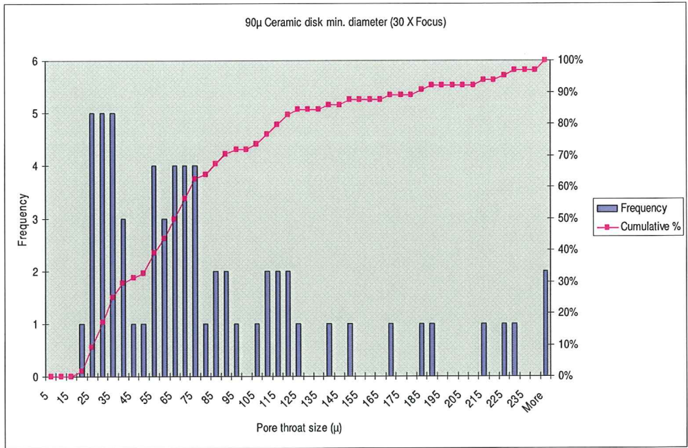
Figure A-18: 90µ Ceramic Disk Minimum Diameter (30X Focus)
