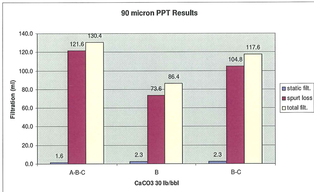
Figure 5-12: Effect of particle size for 90 \mu ceramic disks
