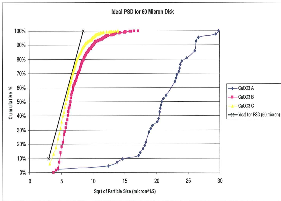
Figure 5-14: Ideal PSD for 60 μ Ceramic Disks & CaCO 3 Grades
