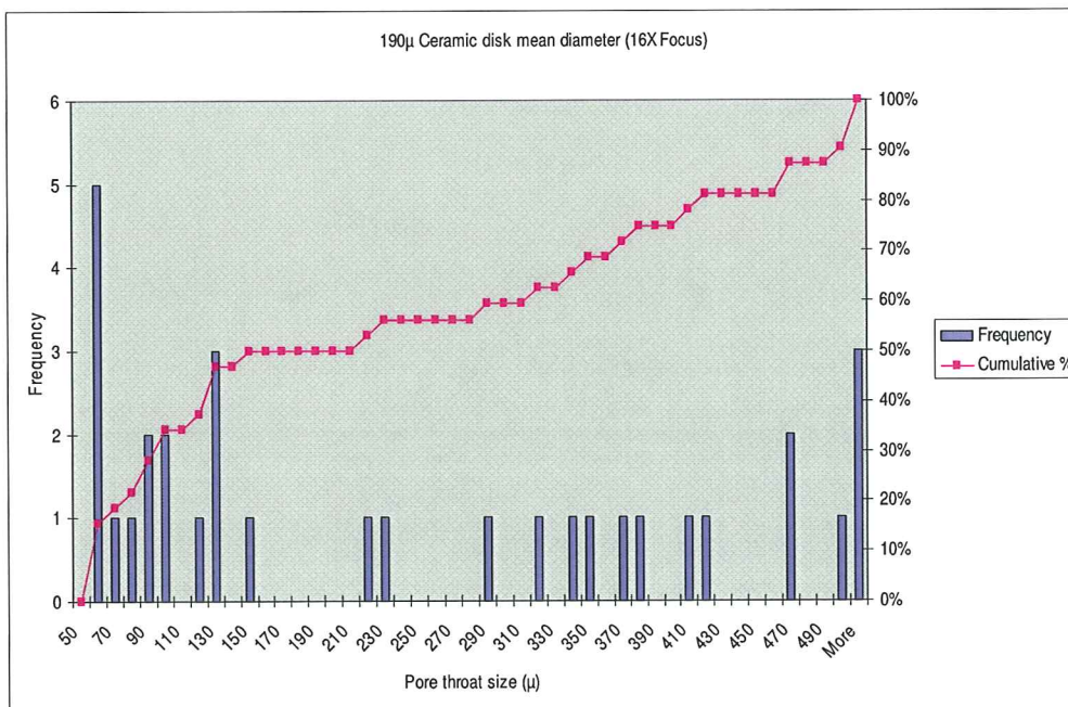
Figure A-21: 190 \mu Ceramic Disk Mean Diameter (16X Focus)
