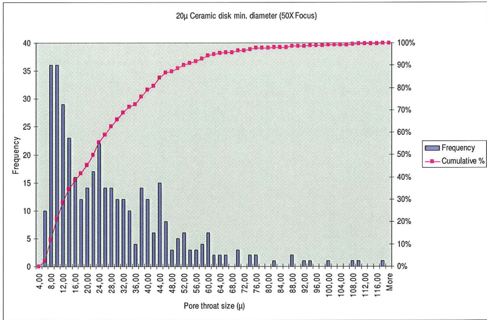
Figure A-2: 20 \mu Ceramic Disk Minimum Diameter (50X Focus)
