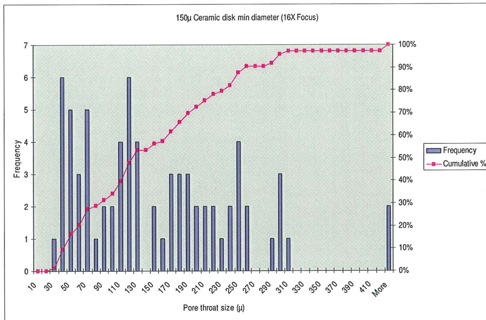
Figure A-20: 150 \mu Ceramic Disk Minimum Diameter (16X Focus)
