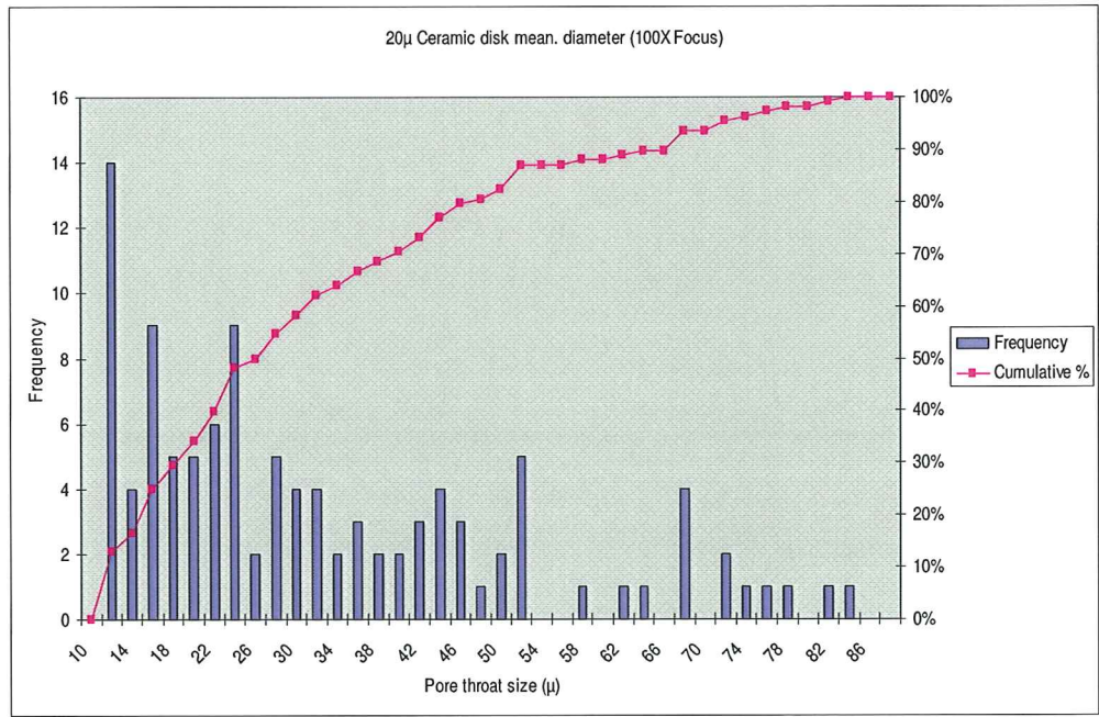
Figure A-5: 20 \mu Ceramic Disk Mean Diameter (100X Focus)
