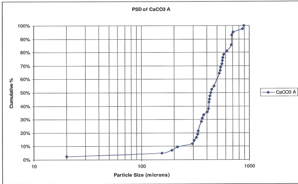
Figure 5-2: PSD of CaCO 3 A
