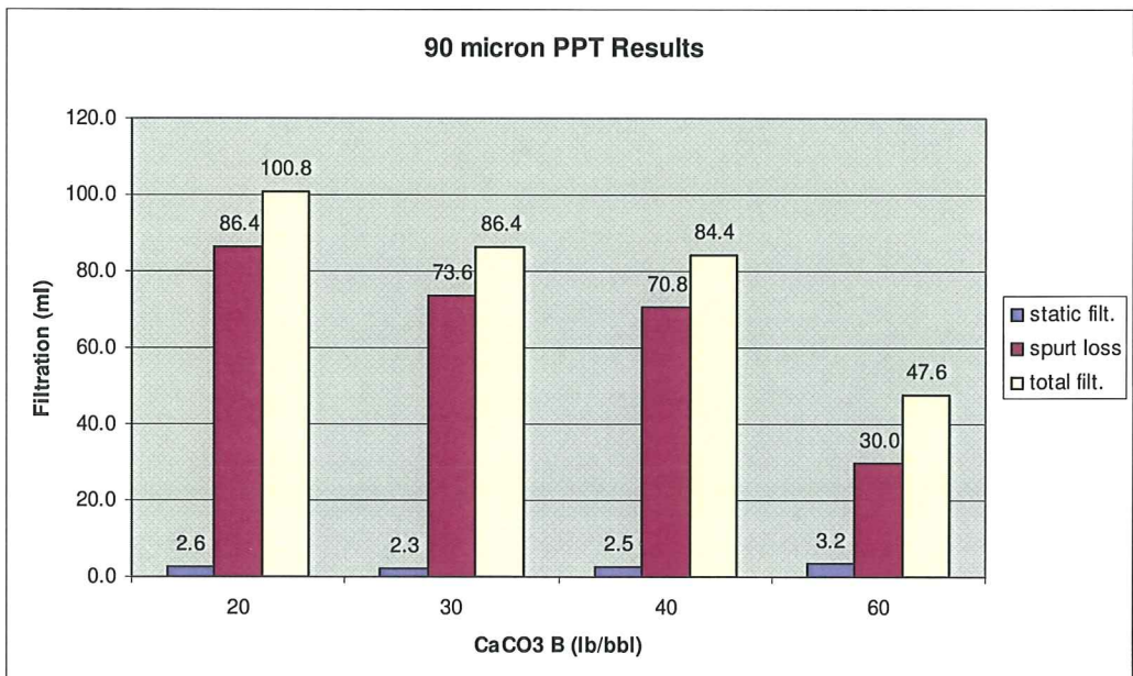
Figure C-5: Effect of Concentration of CaCO 3 B (90 μ Ceramic Disks)
