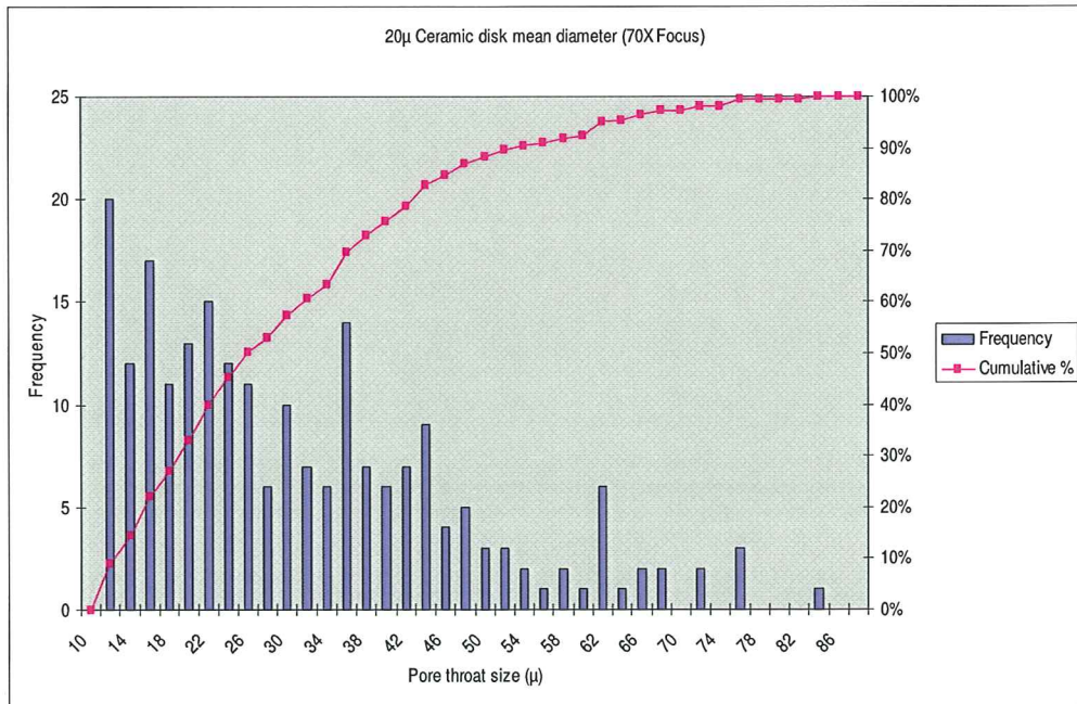
Figure A-3: 20 \mu Ceramic Disk Mean Diameter (70X Focus)
