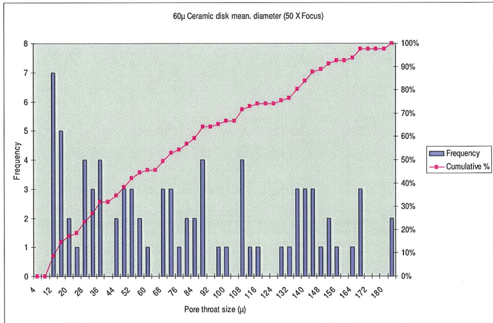
Figure A-13: 60µ Ceramic Disk Mean Diameter (50X Focus)
