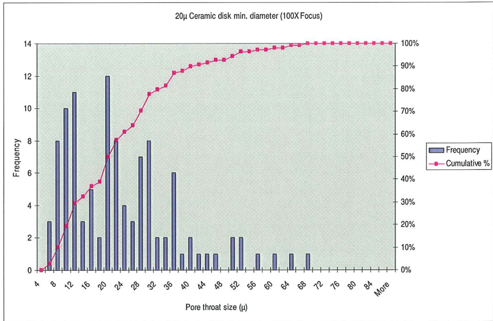
Figure A-6: 20 \mu Ceramic Disk Minimum Diameter (100X Focus)
