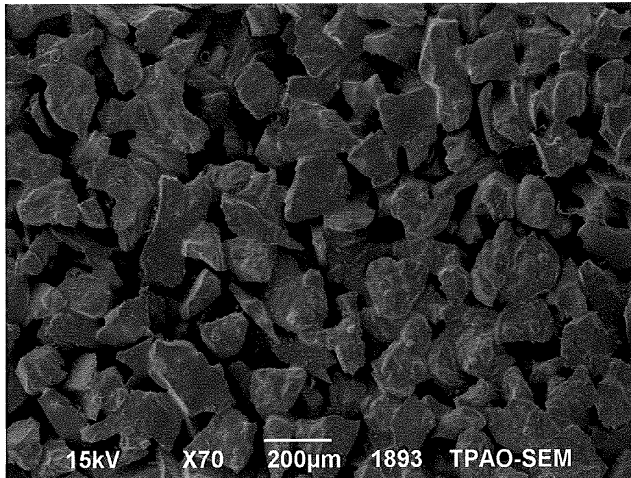
Figure 4-4: SEM photograph of 35 μ Ceramic Disk 70 X Focus
