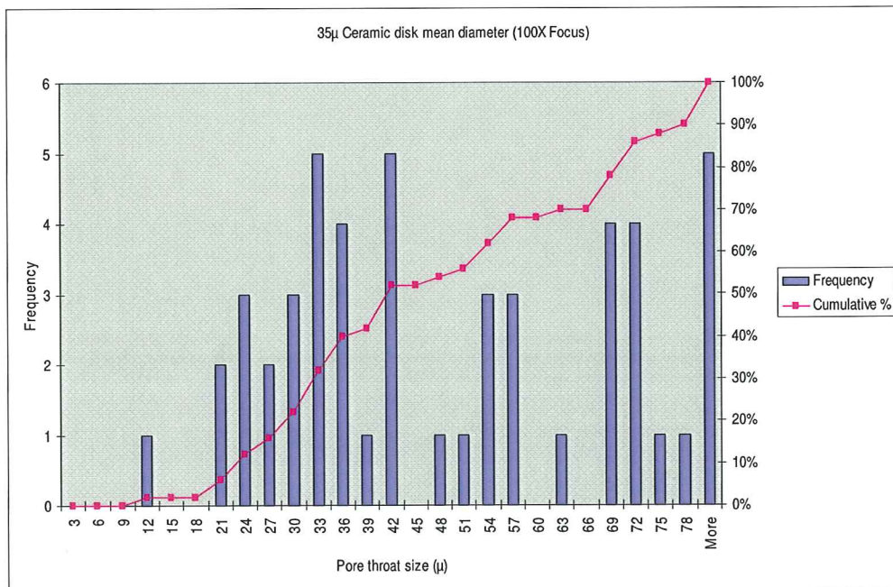
Figure A-11: 35µ Ceramic Disk Mean Diameter (100X Focus)
