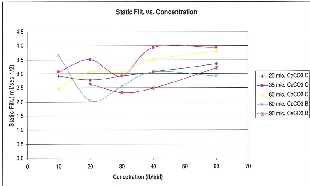
Figure 5-9: Static Filtration vs. Concentration
