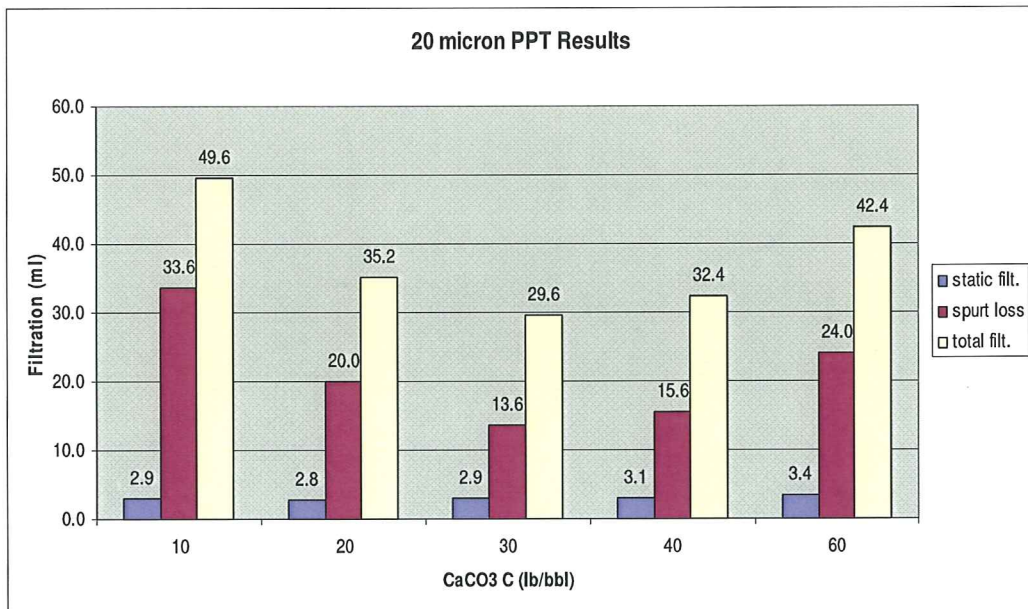
Figure C-1: Effect of Concentration of CaCO 3 C (20 \mu Ceramic Disks)
