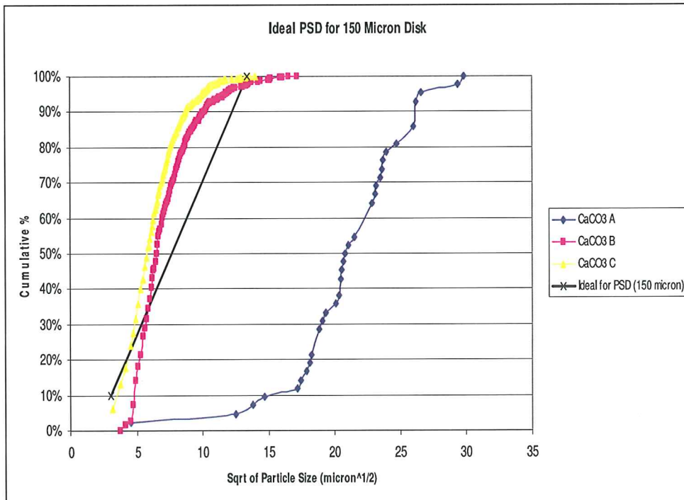
Figure 5-16: Ideal PSD for 90 μ Ceramic Disks & CaCO 3 Grades
