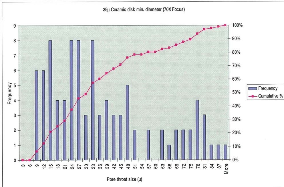
Figure A-10: 35µ Ceramic Disk Minimum Diameter (70X Focus)
