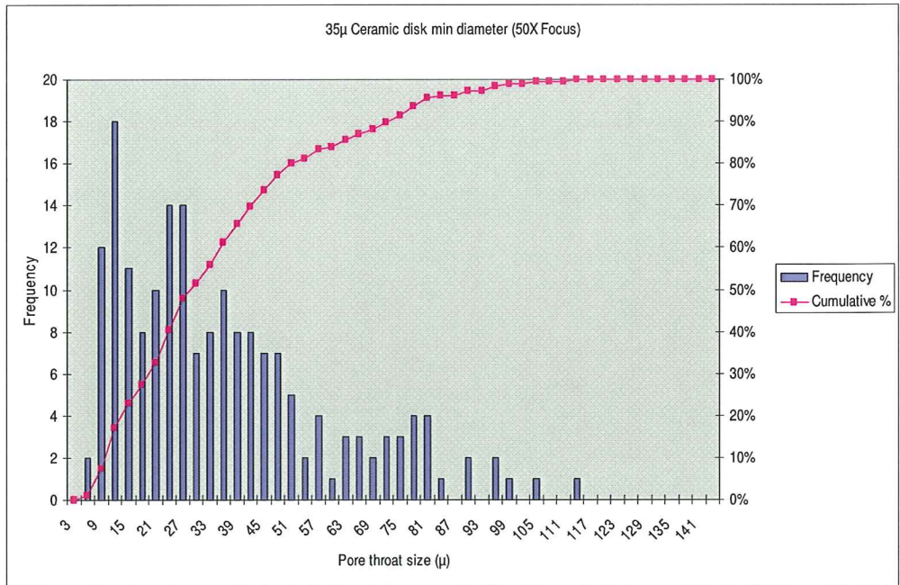
Figure A-8: 35μ Ceramic Disk Minimum Diameter (50X Focus)
