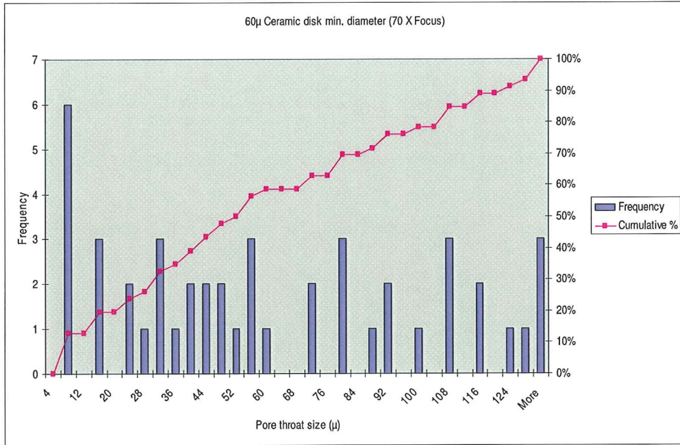
Figure A-16: 60µ Ceramic Disk Minimum Diameter (70X Focus)
