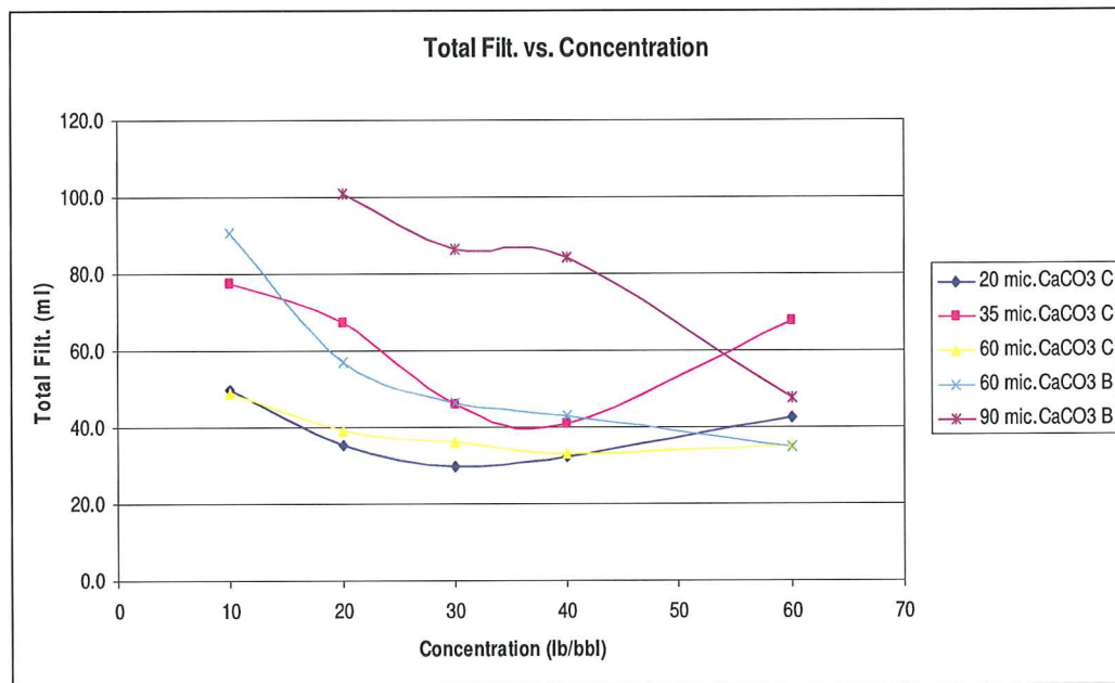
Figure 5-8: Total Loss vs. Concentration
