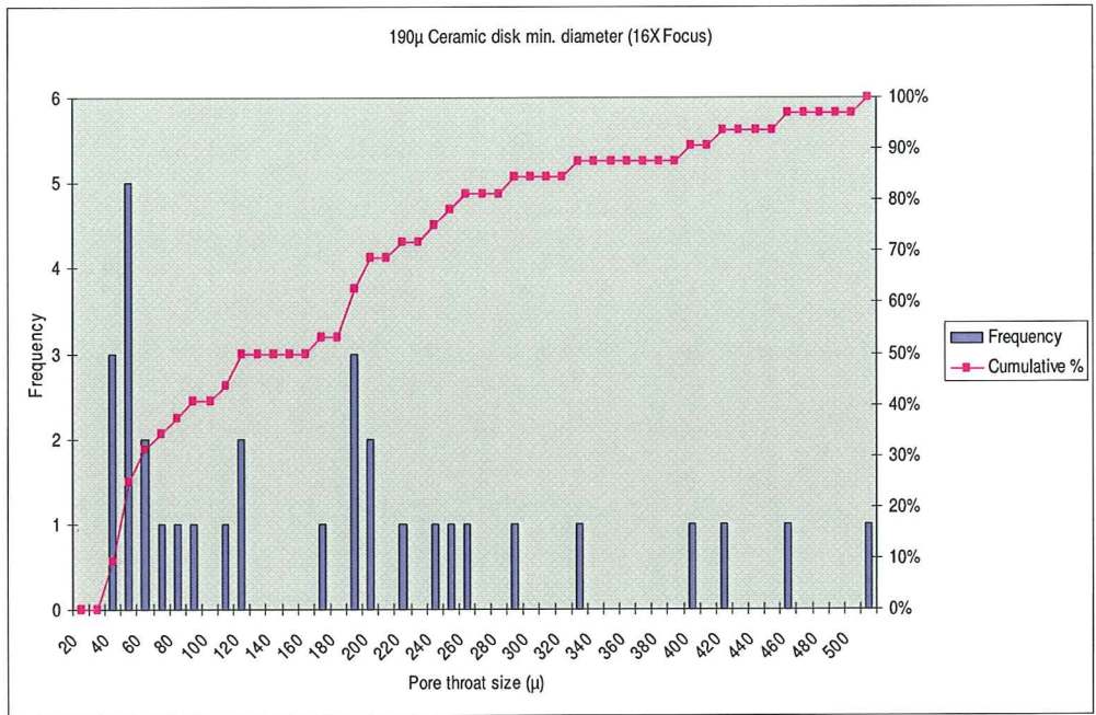
Figure A-22: 190µ Ceramic Disk Minimum Diameter (160X Focus)
