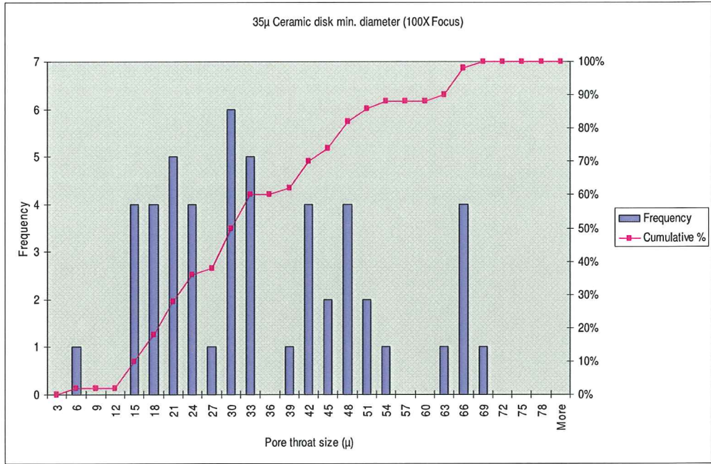
Figure A-12: 35µ Ceramic Disk Minimum Diameter (50X Focus)
