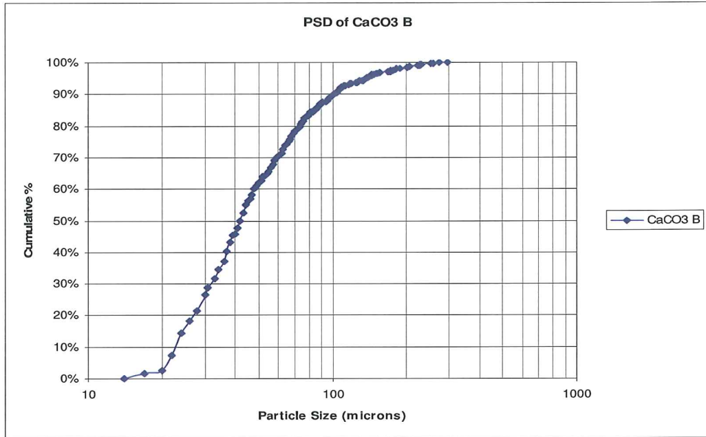
Figure 5-3: PSD of CaCO 3 B
