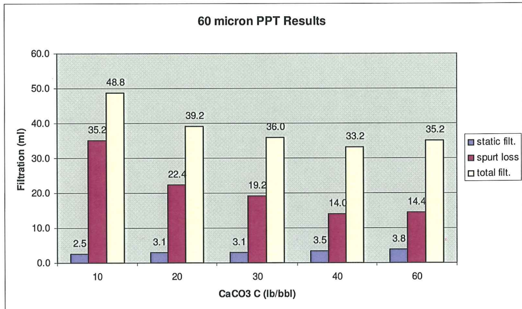
Figure C-3: Effect of Concentration of CaCO 3 C (60 μ Ceramic Disks)
