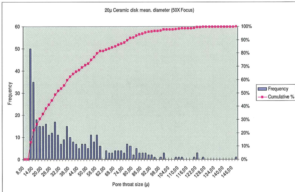
Figure A-1: 20µ Ceramic Disk Mean Diameter (50X Focus)
