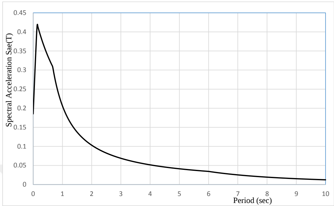
Figure 3.6. Reduced Design Response Spectrum Curve with TBDY.
