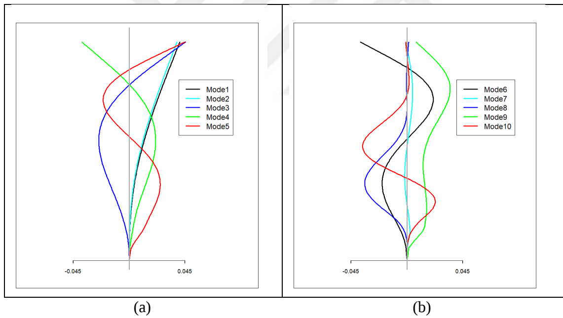
Figure 2.6. Mode shapes (1-5) of Industrial chimney. (b) Mode shapes (6-10) of Industrial chimney.
