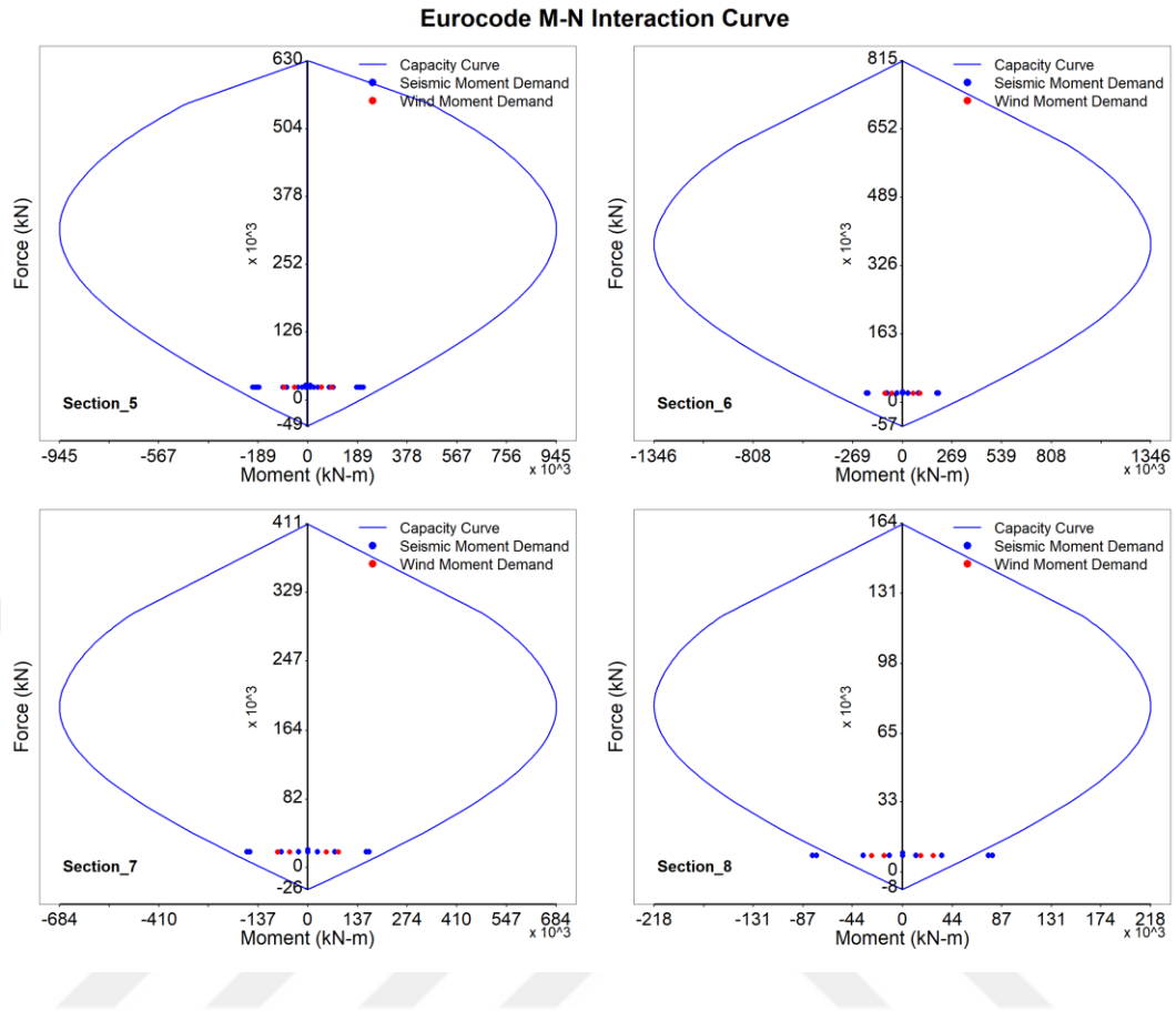
Figure 5.31. Section 5 to Section 8 moment demand and capacity curve in accordance with Eurocode. Section-5, section-6 and section-7 are considered as safe for the load combination 1.0[DL]+1.0[EQ-Y] + 0.3[EQ-X] in accordance with Eurocode specifications.
