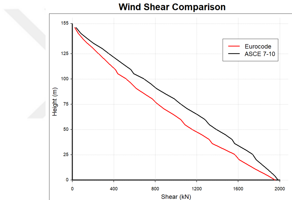
Figure 5.7. Shear demand due to wind load comparison in accordance with Eurocode and ASCE specifications along the height of chimney.
