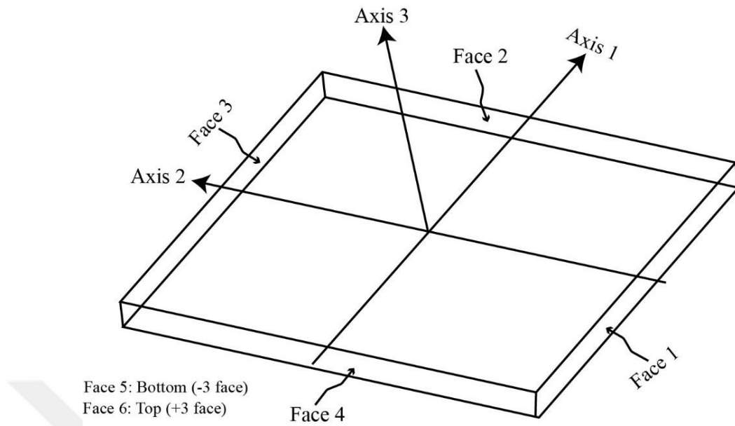
Figure 2.2. Geometry of thin shell element used in the analysis.
