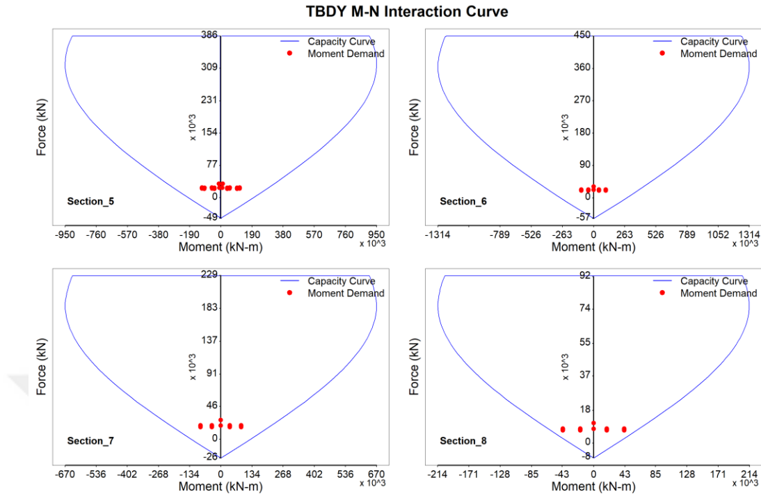
Figure 5.28. Section 5 to Section 8 moment demand and capacity curve in accordance with TBDY.
