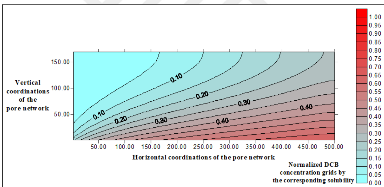
Figure 5.36. Contour plot of the normalized DCB distribution computed with the pore network model for Q = 0.156 mL/min, EtOH = 0 % (sand).
