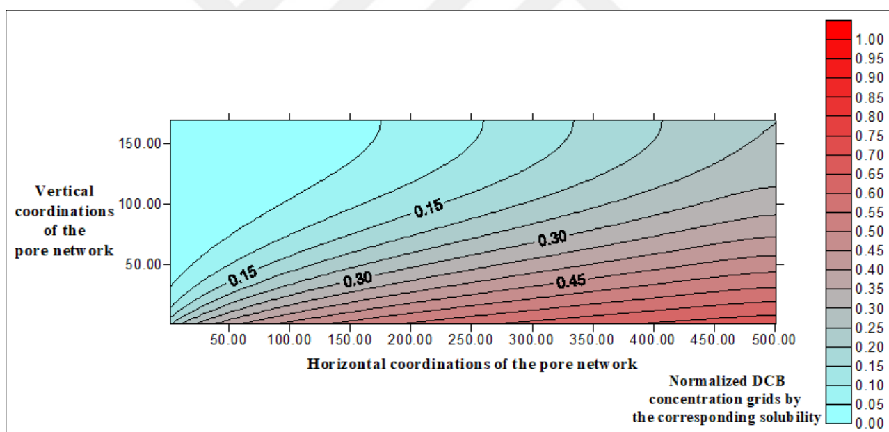
Figure 5.48. Contour plot of the normalized DCB distribution computed with the pore network model for Q = 2 mL/min, EtOH = 10 % (sand).
