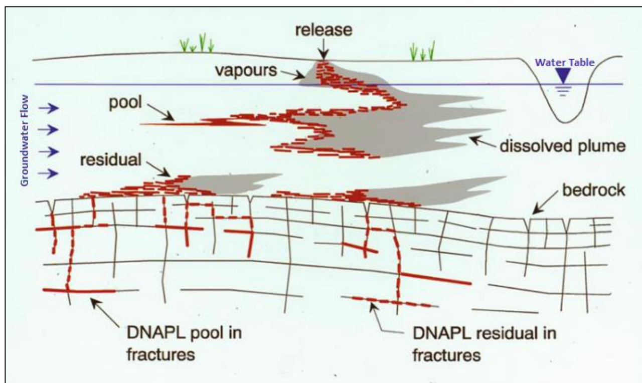
Figure 2.2. Contamination pathways of DNAPLs. Adapted from Figure 1.1(d) of (Kueper et al., 2014b).
