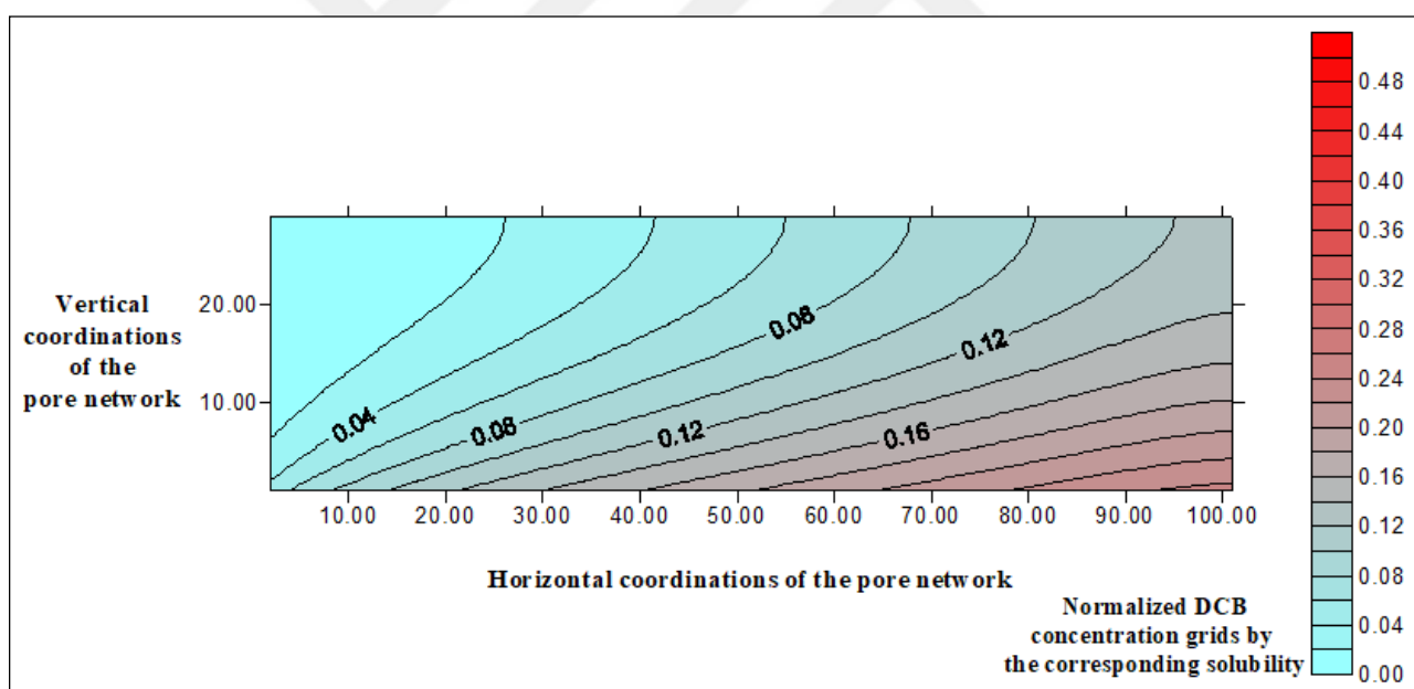
Figure 5.18. Contour plot of the normalized DCB distribution computed with the pore network model for Q = 0.232 mL/min, EtOH = 20 % (glass beads).
