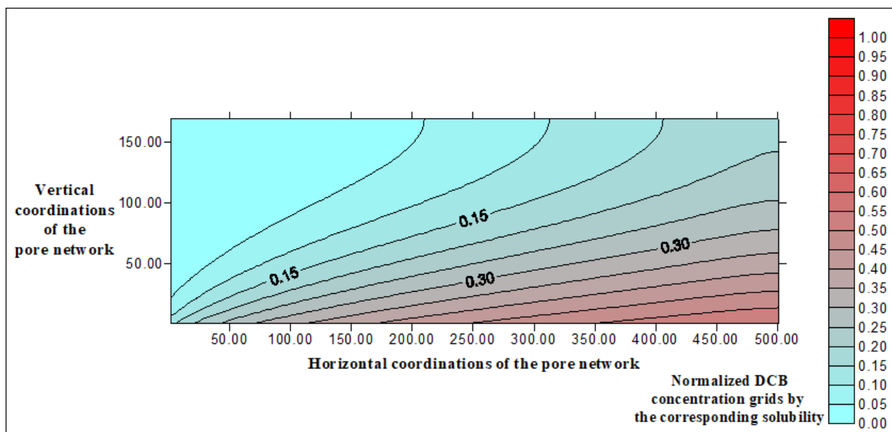
Figure 5.47. Contour plot of the normalized DCB distribution computed with the pore network model for Q = 2 mL/min, EtOH = 0 % (sand).
