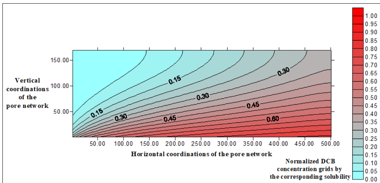
Figure 5.43. Contour plot of the normalized DCB distribution computed with the pore network model for Q = 1 mL/min, EtOH = 10 % (sand).
