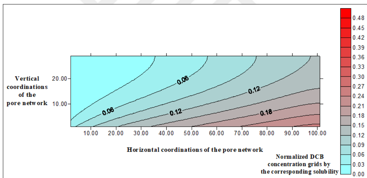
Figure 5.28. Contour plot of the normalized DCB distribution computed with the pore network model for Q = 5 mL/min, EtOH = 0 % (glass beads).
