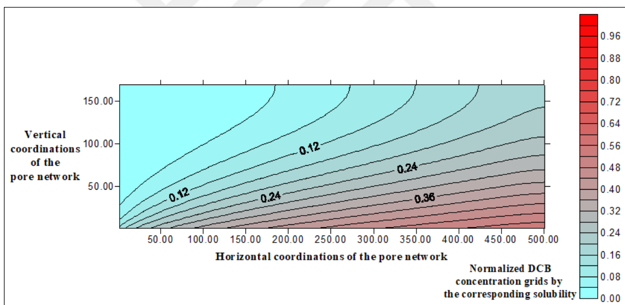
Figure 5.46. Contour plot of the normalized DCB distribution computed with the pore network model for Q = 1 mL/min, EtOH = 40 % (sand).
