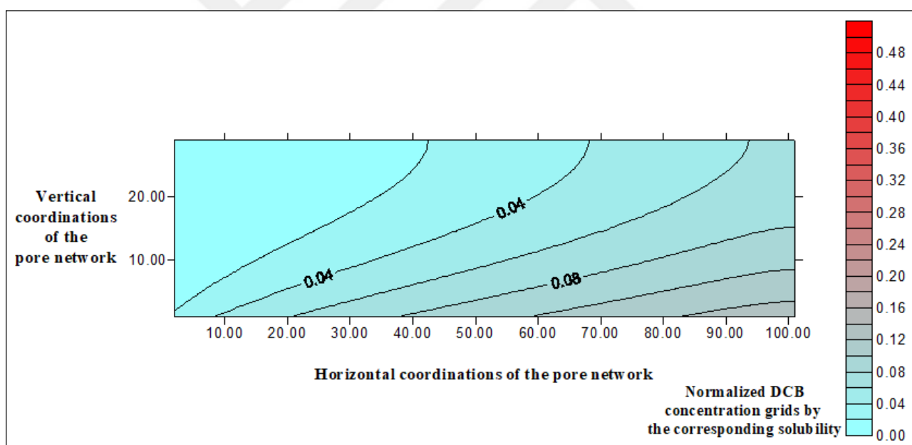
Figure 5.22. Contour plot of the normalized DCB distribution computed with the pore network model for Q = 1 mL/min, EtOH = 20 % (glass beads).
