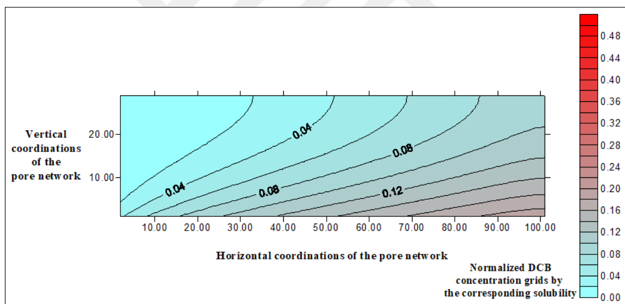
Figure 5.30. Contour plot of the normalized DCB distribution computed with the pore network model for Q = 5 mL/min, EtOH = 20 % (glass beads).
