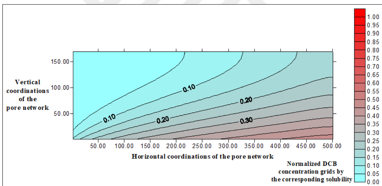
Figure 5.38. Contour plot of the normalized DCB distribution computed with the pore network model for Q = 0.187 mL/min, EtOH = 0 % (sand).
