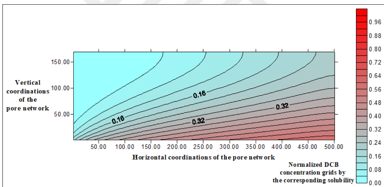
Figure 5.44. Contour plot of the normalized DCB distribution computed with the pore network model for Q = 1 mL/min, EtOH = 20 % (sand).
