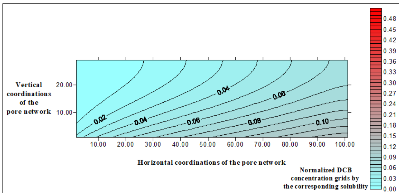
Figure 5.19. Contour plot of the normalized DCB distribution computed with the pore network model for Q = 0.232 mL/min, EtOH = 30 % (glass beads).
