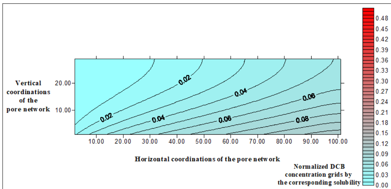
Figure 5.31. Contour plot of the normalized DCB distribution computed with the pore network model for Q = 5 mL/min, EtOH = 30 % (glass beads).
