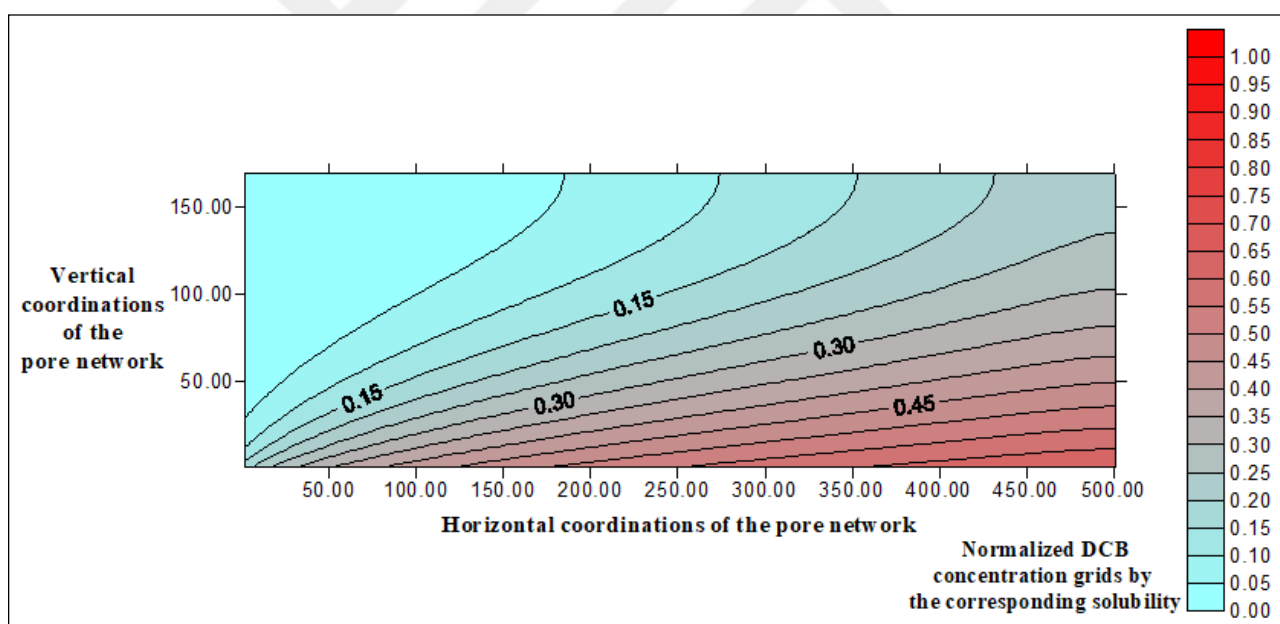
Figure 5.52. Contour plot of the normalized DCB distribution computed with the pore network model for Q = 5 mL/min, EtOH = 0 % (sand).
