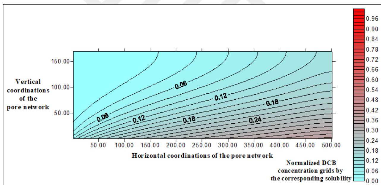
Figure 5.56. Contour plot of the normalized DCB distribution computed with the pore network model for Q = 5 mL/min, EtOH = 40 % (sand).
