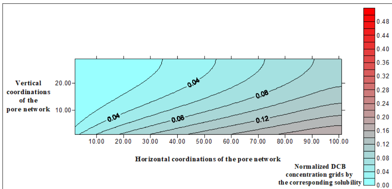
Figure 5.33. Contour plot of the normalized DCB distribution computed with the pore network model for Q = 25 mL/min, EtOH = 10 % (glass beads).
