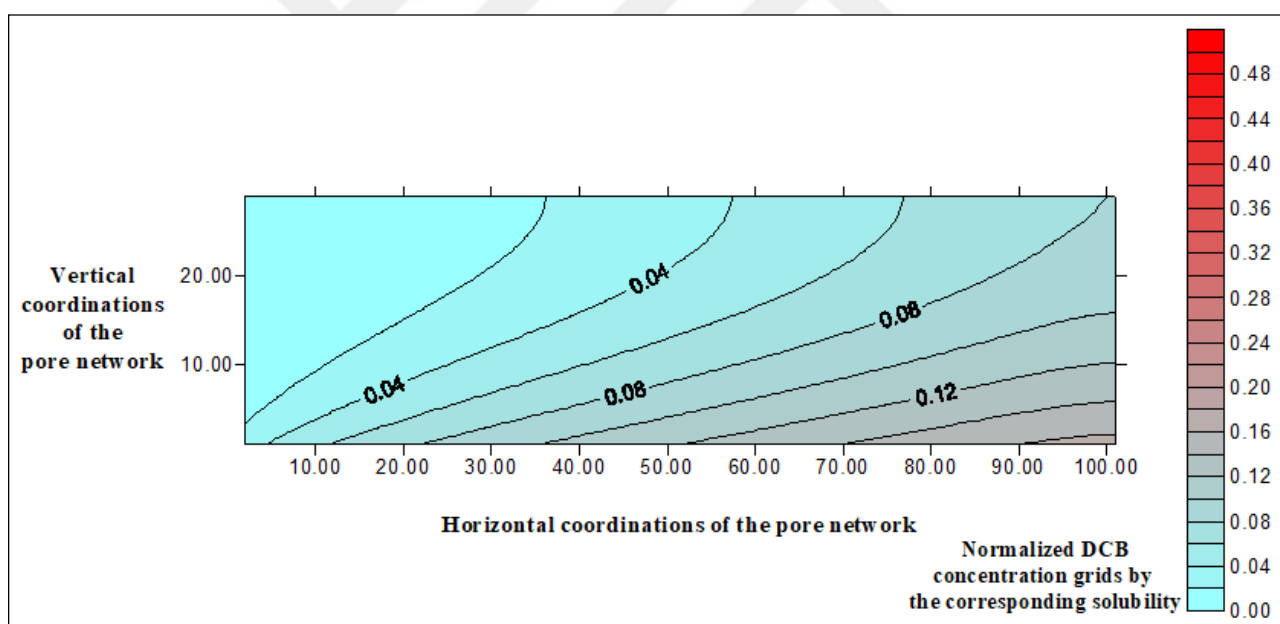
Figure 5.26. Contour plot of the normalized DCB distribution computed with the pore network model for Q = 2 mL/min, EtOH = 20 % (glass beads).
