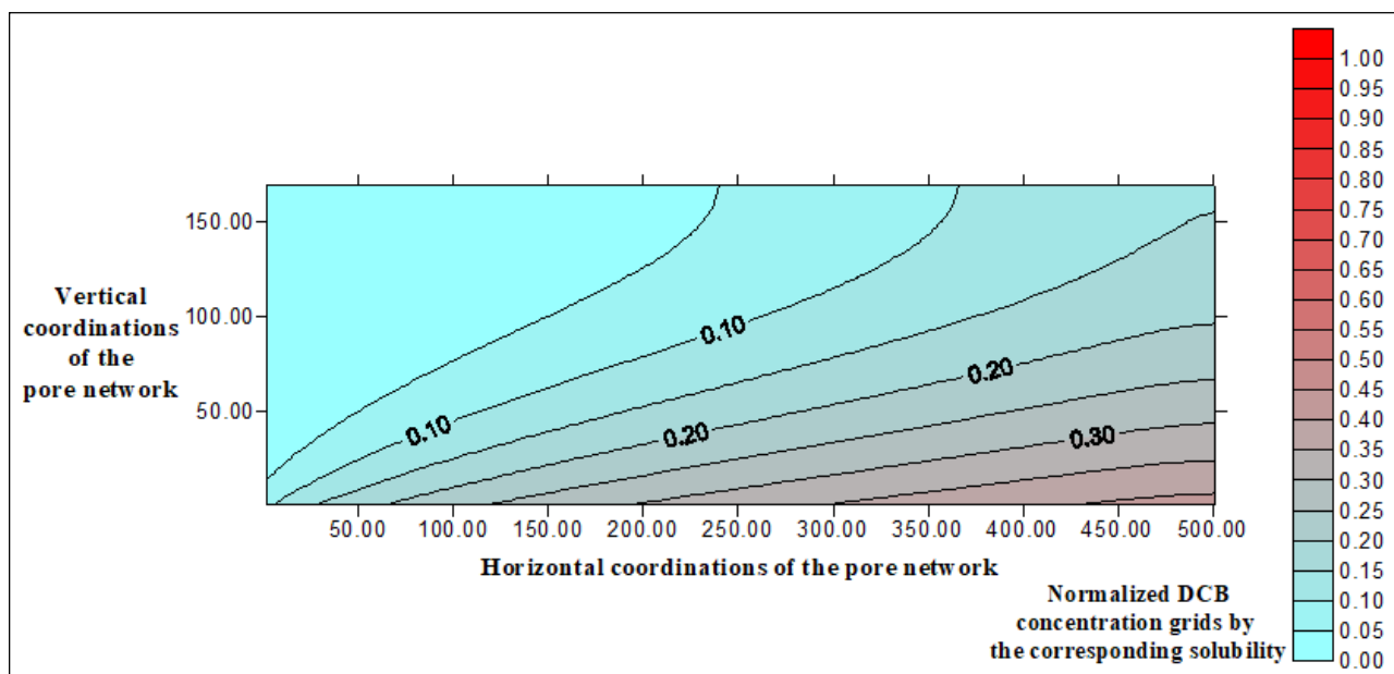
Figure 5.39. Contour plot of the normalized DCB distribution computed with the pore network model for Q = 0.187 mL/min, EtOH = 10 % (sand).
