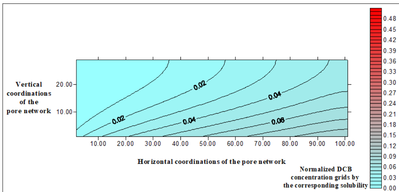
Figure 5.35. Contour plot of the normalized DCB distribution computed with the pore network model for Q = 25 mL/min, EtOH = 30 % (glass beads).
