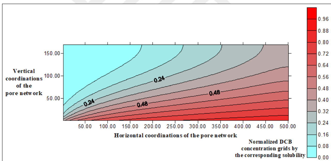
Figure 5.42. Contour plot of the normalized DCB distribution computed with the pore network model for Q = 1 mL/min, EtOH = 0 % (sand).
