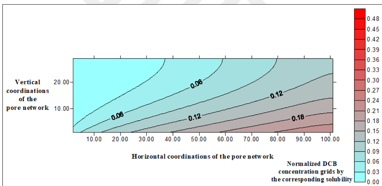
Figure 5.24. Contour plot of the normalized DCB distribution computed with the pore network model for Q = 2 mL/min, EtOH = 0 % (glass beads).
