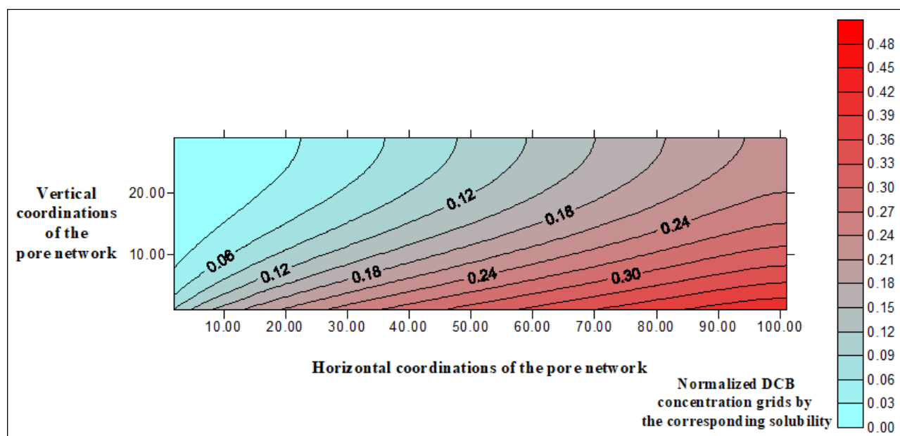
Figure 5.16. Contour plot of the normalized DCB distribution computed with the pore network model for Q = 0.232 mL/min, EtOH = 0 % (glass beads).
