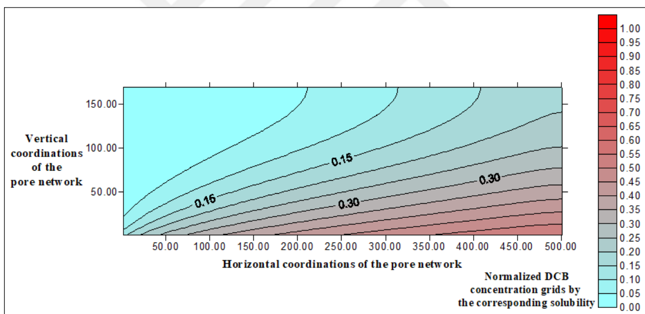
Figure 5.54. Contour plot of the normalized DCB distribution computed with the pore network model for Q = 5 mL/min, EtOH = 20 % (sand).
