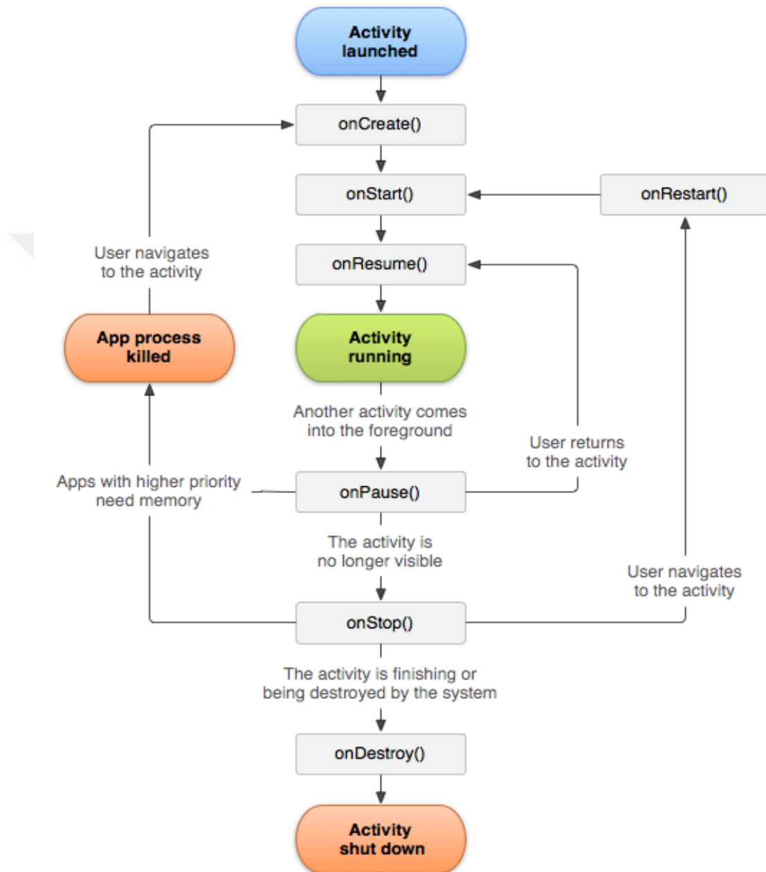
Figure 4.8. Application life cycle: starting, idling, stopping or closing (user / student)
