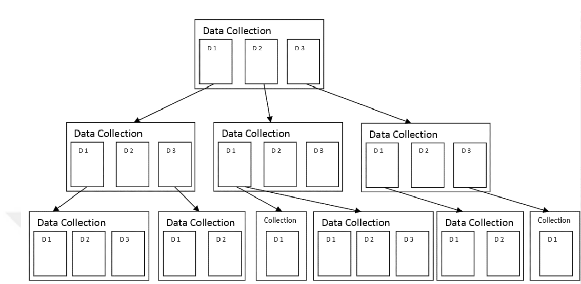
Figure 4.6. Data structure, fetching documents without having to fetch its sub-collections
