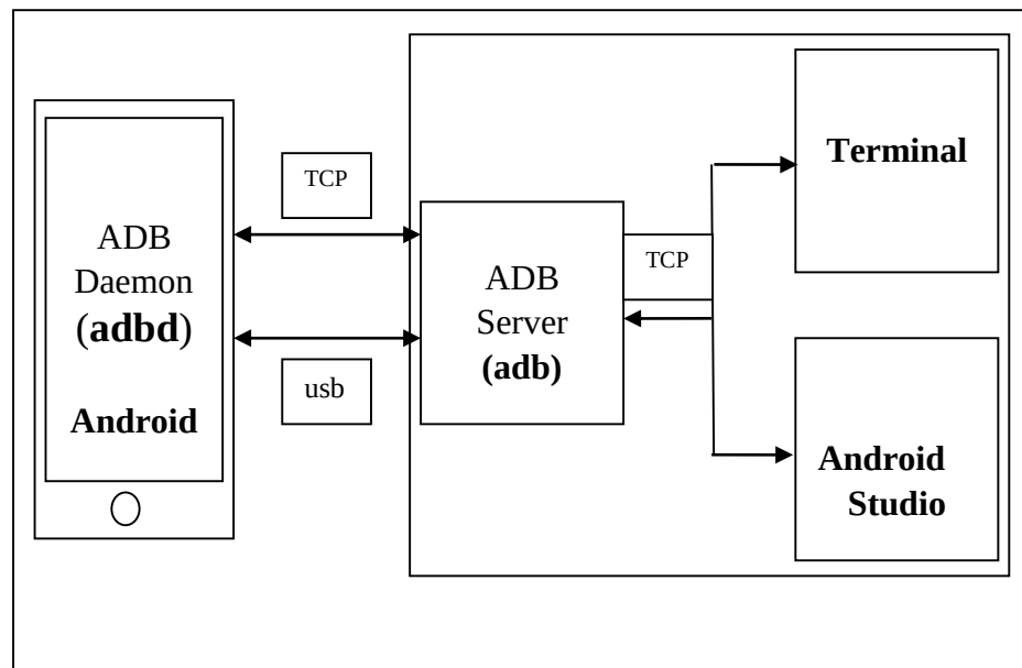
Figure 4.12. Android debug bridge, remotely install an APK on any user device (admin)
