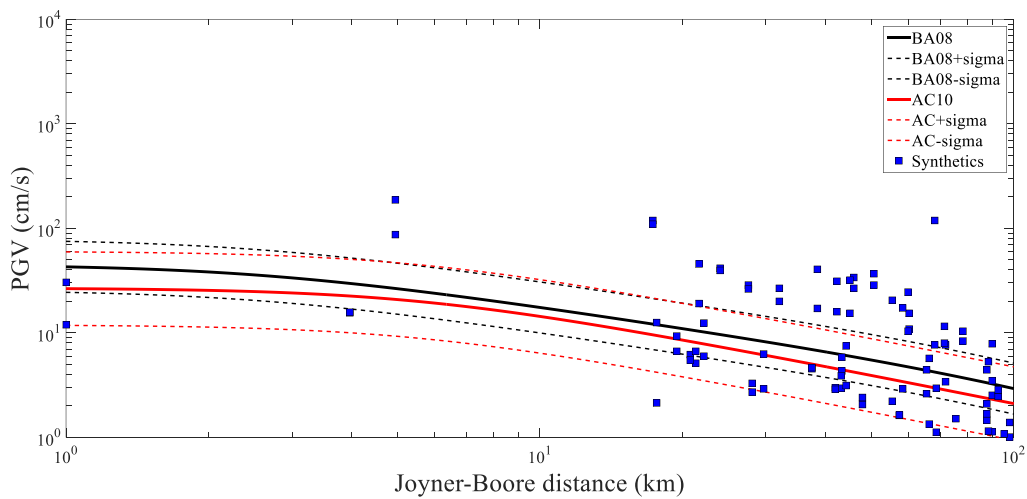
Figure 3.23. Comparison of PGV values of broadband results with PGV values from GMPE's with respect to Joyner – Boore distance for scenario earthquake Mw=6.5
