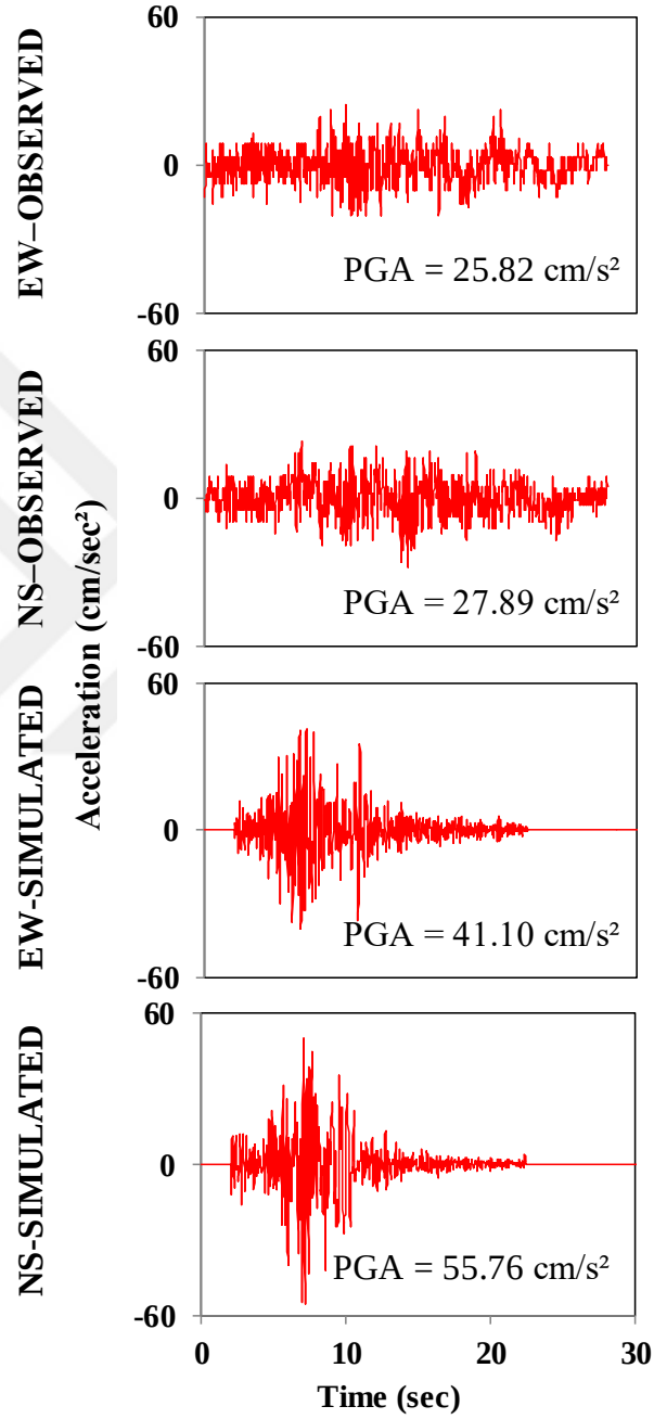
Figure 3.9. Comparison of acceleration-time histories of broadband results with real data for the 12 November 1999 Duzce earthquake in E-W and N-S direction – station GYN
