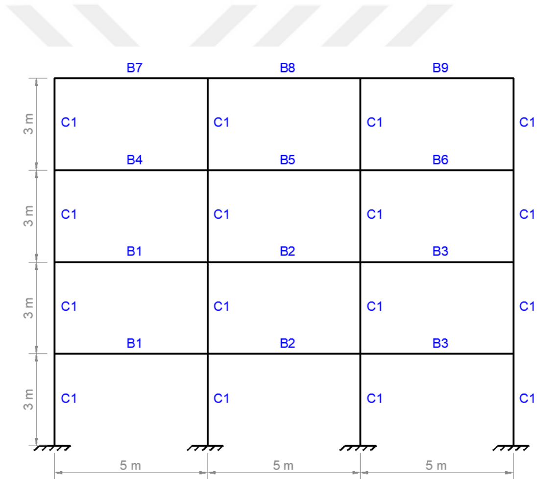
Figure 4.2. Cross-Sectional View of Frame F4S3B
