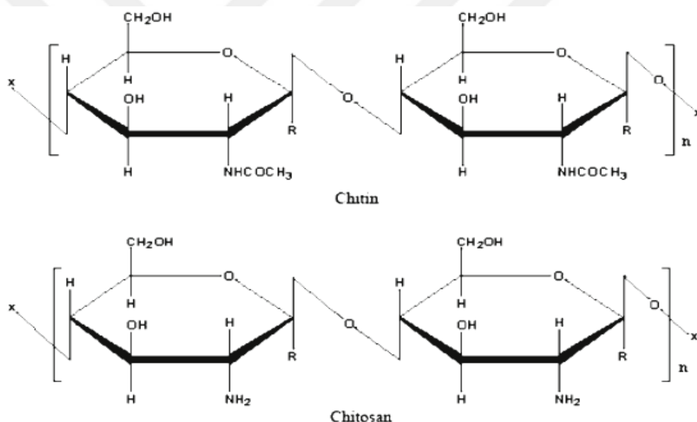
Figure 2.3. Chemical structures of chitin and deacetylated chitosan
