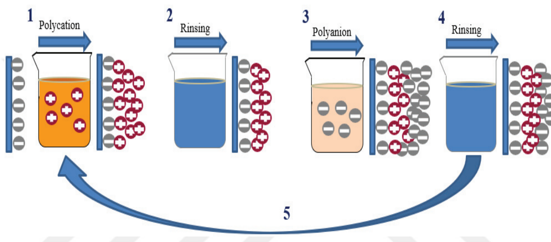
Figure 2.1. Diagram of LbL assembly. (1) deposition of positively charged substrate, (2) rinsing with solvent and dry, (3) deposition of negatively charged substrate, (4) rinsing with solvent and dry, (5) return to step (1)
