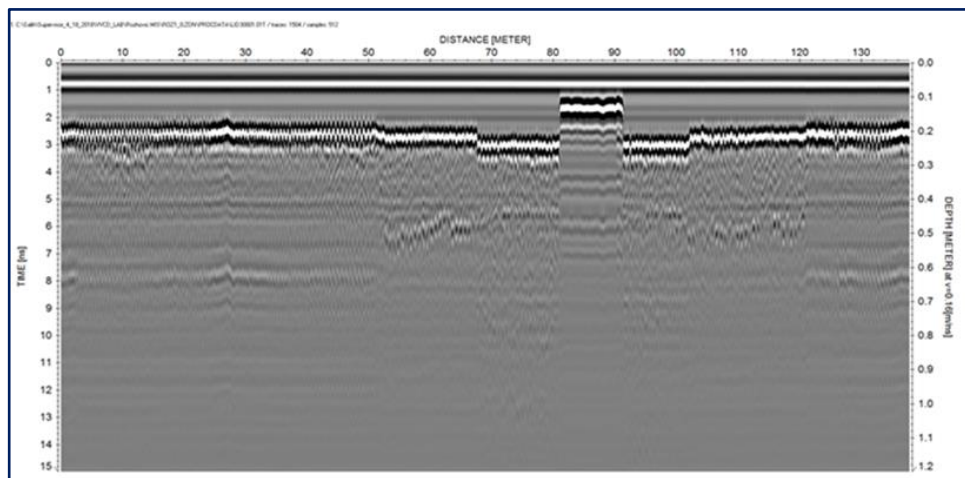
Figure 7.13. Stacking traces applied
