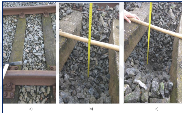
Figure 6.27. Trench 4: a) crib to be opened, b) moderately clean ballast layer thickness measurement, c) fouled ballast layer thickness measurement
