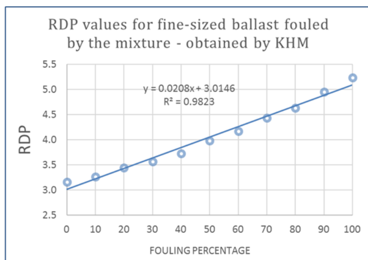
Figure 7.2. a) RDP values for fine-sized ballast fouled by sand, b) by fine-sized gravel, c) by the mixture of sand and fine-sized gravel – All values calculated by KHM
