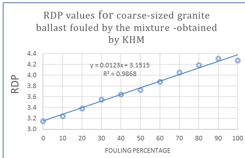
Figure 7.4. a) RDP values for coarse-sized ballast fouled by sand, b) by fine-sized gravel, c) by the mixture of sand and fine-sized gravel – All values calculated by KHM
