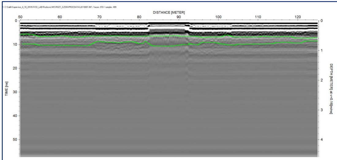
Figure 7.23. Processed data for 900MHz IDS antenna.
