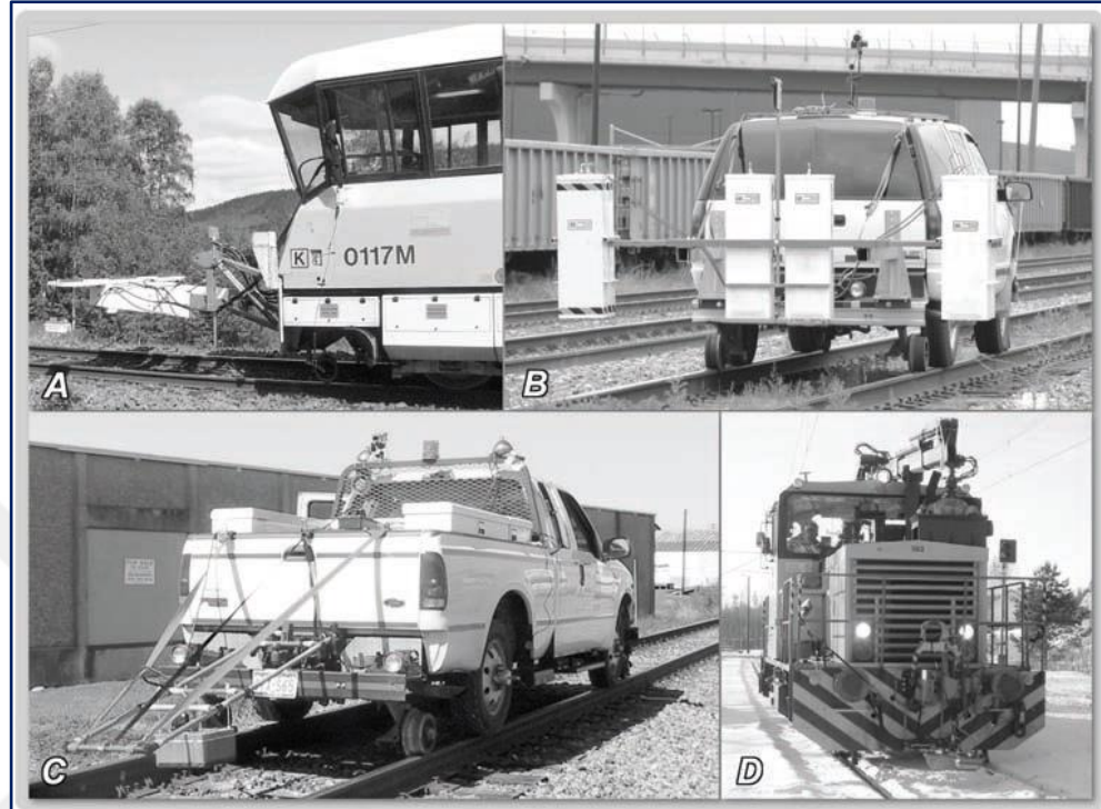
Figure 4.2. Different GPR sets used in Railways [56]: a) Swedish Mala ground-coupled antenna (photo by Mala Geoscience), b) multichannel GSSI air-coupled system (from Olhoeft et al. [81]), c) GSSI 400MHz ground-coupled antenna and d) Radar Team Sweden 350MHz 1.2GHz Sub-Echo HBD antennas (photo Mika Silvast)
