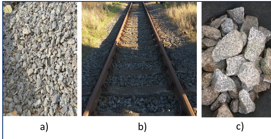
Figure 6.7. a) Coarse-size granite ballast used in the laboratory experiments, b) the same kind of granite ballast laid in the railway segment in Rozhovice, in the Czech Republic, c) sample taken from the railway segment in Rozhovice
