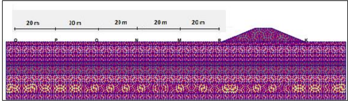
Figure 7.19 Location of points near the ground surface for finding extreme velocity
