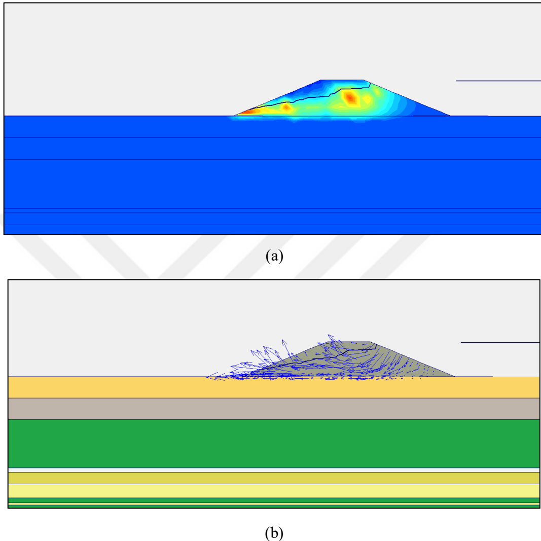
Figure B.58. Flow field at 2+005.66 km on left shore of Filyos River during h_{\max} a.) Shadings view b.) Arrows view
