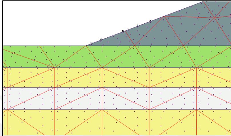
Figure B.141 Location of points above the levee for finding extreme velocity
