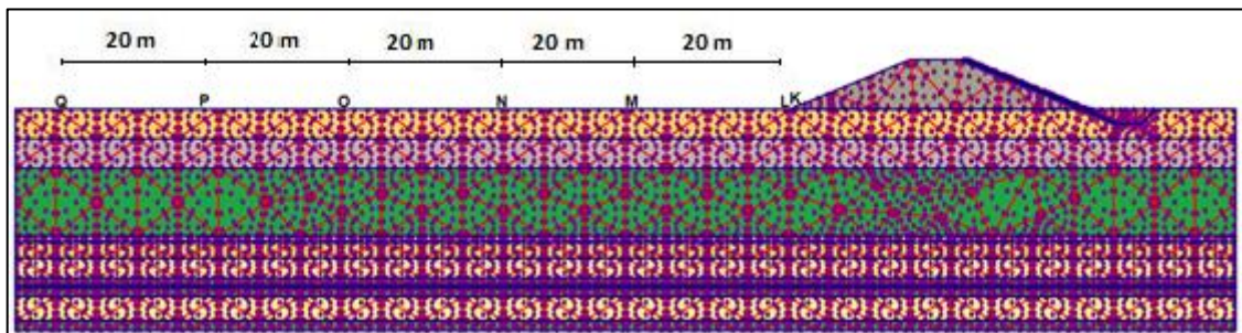
Fig. B.67. Location of points near the ground surface for finding extreme velocity
