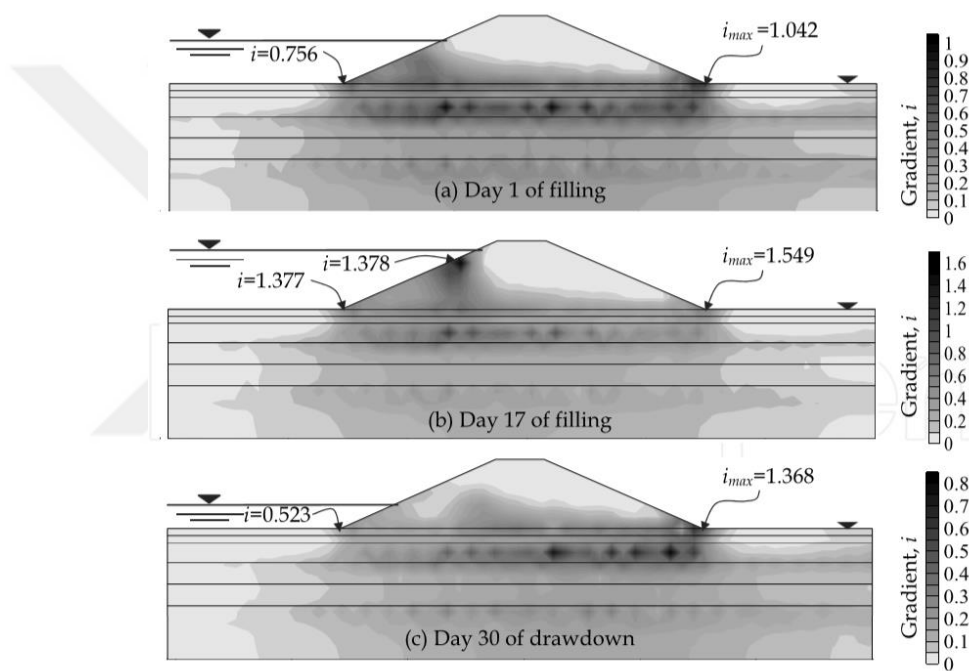
Figure 4.26 Hydraulic gradients (magnitude) for three different times during rapid filling and drawdown (Source: Lopez-Acosta et. al. , 2010)
