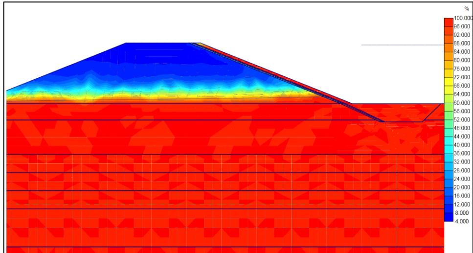
Figure 7.25 Degree of Saturation of Filyos Levee with cover materials at 271.05 m on right shore of Filyos River during h_{\max}
