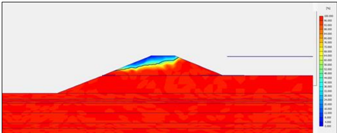
Figure B.36 Degree of Saturation of Filyos Levee at 1+513.22 km on left shore of Filyos River during h_{\max}
