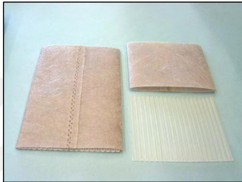
Figure 4.12 Example of a 4-inch-wide wick drain composed of a polymeric corrugated core and outer geotextile
