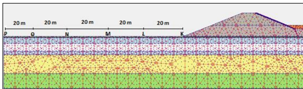
Figure B.28 Location of points near the ground surface for finding extreme velocity
