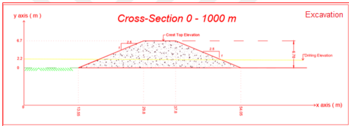
Figure 5.4 Uncovered materials Filyos Levee sections (excavation)
