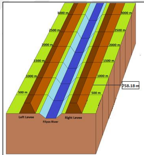
Figure B.83 Filyos Levee at 758.18 m on right shore of Filyos River
