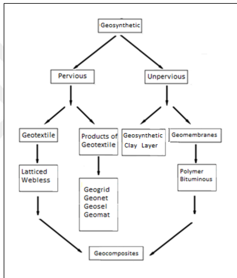
Figure 4.7 Geocomposite
