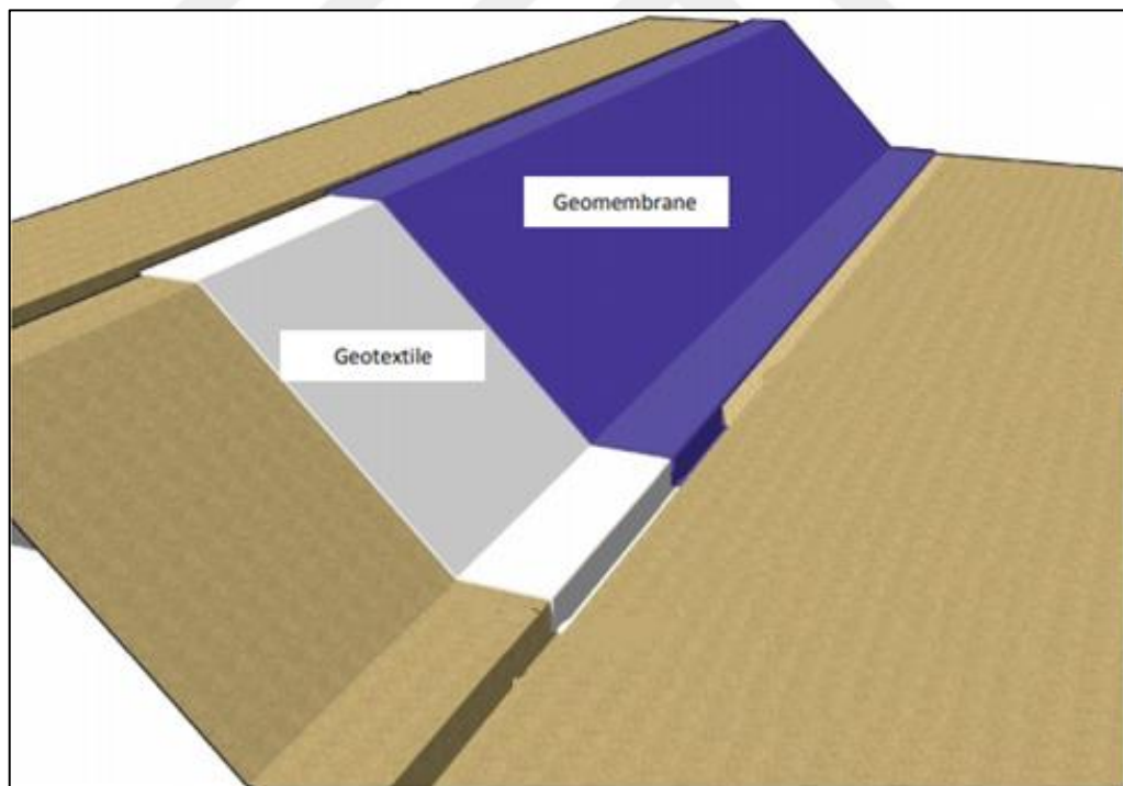
Figure 4.22 Geocomposite Covering
