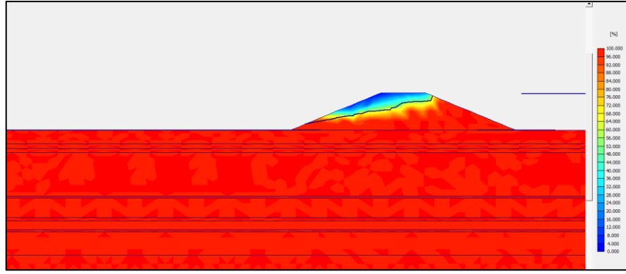
Figure B.71 Degree of Saturation of Filyos Levee at 2+501.94 km on left shore of Filyos River during h_{max}
