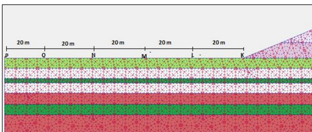
Figure B.129 Location of points near the ground surface for finding extreme velocity
