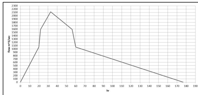
Figure 6.1 Unit Hydrograph
