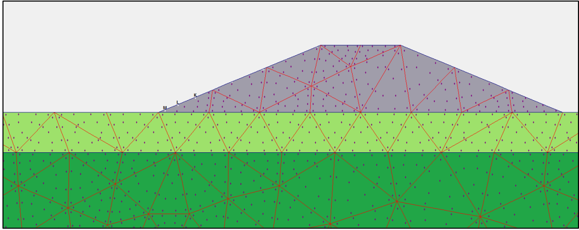
Figure 7.7 Location of points above the levee for finding extreme velocity
