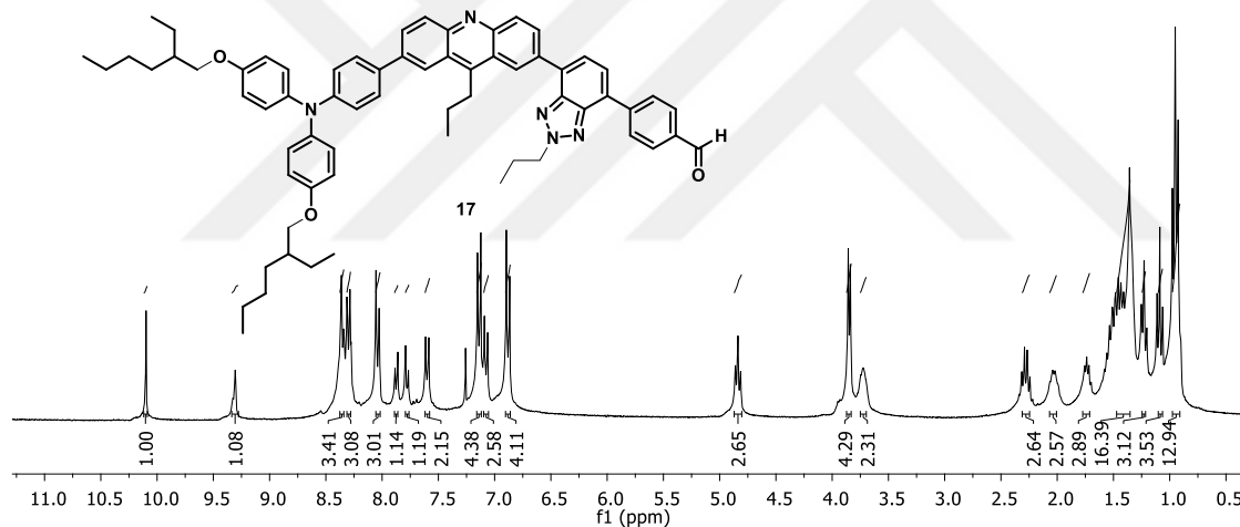
EK 36: 17 bileşiminin ^1\text{H} NMR spektrumu (300 MHz, \text{CDCl}_3 )
