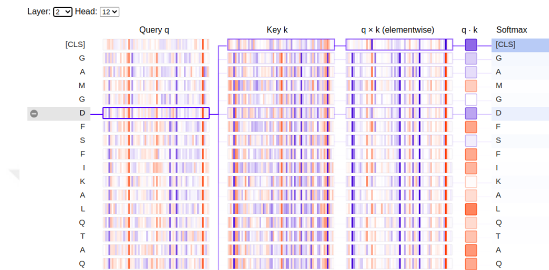
Figure 4.29: ProtBERT Neuron View
