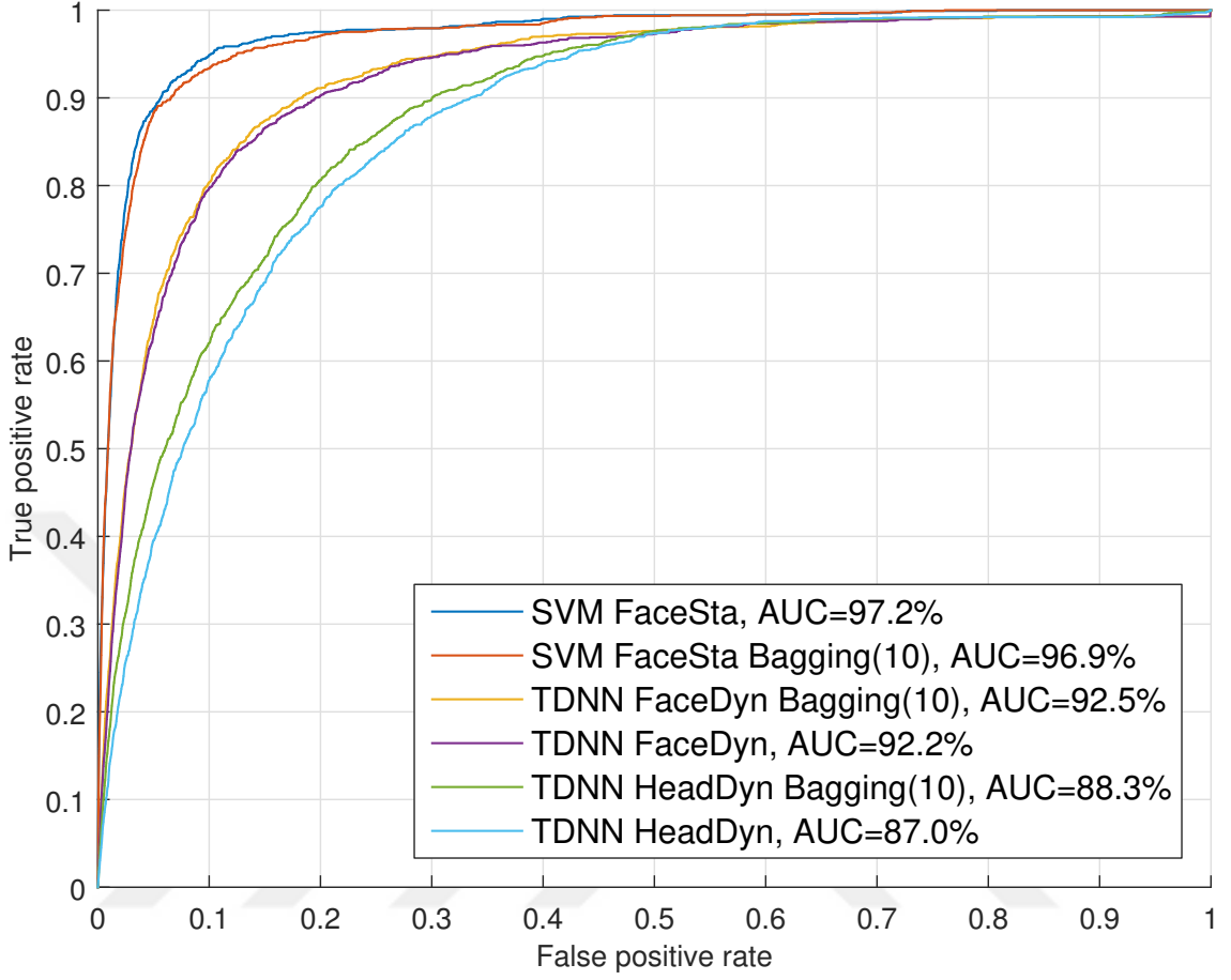
Figure 2.6: ROC curves and AUC performances of laughter detection from head and facial features using different classifier-feature combinations with and without bagging.
