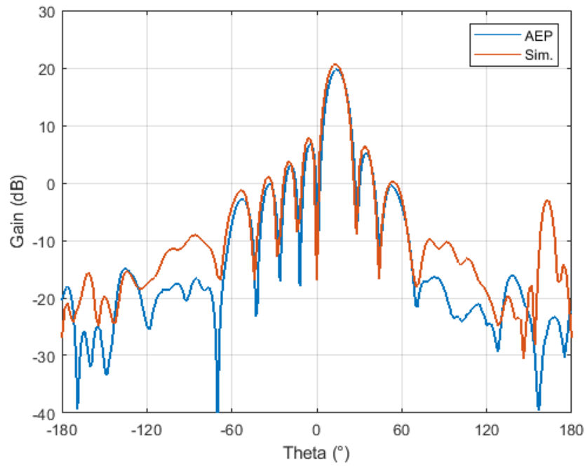
Figure 5.7. Co-Pol radiation pattern at \phi=0^\circ plane beam steered to \theta=13^\circ with 45° progressive phase shift between elements (3.5 GHz)
