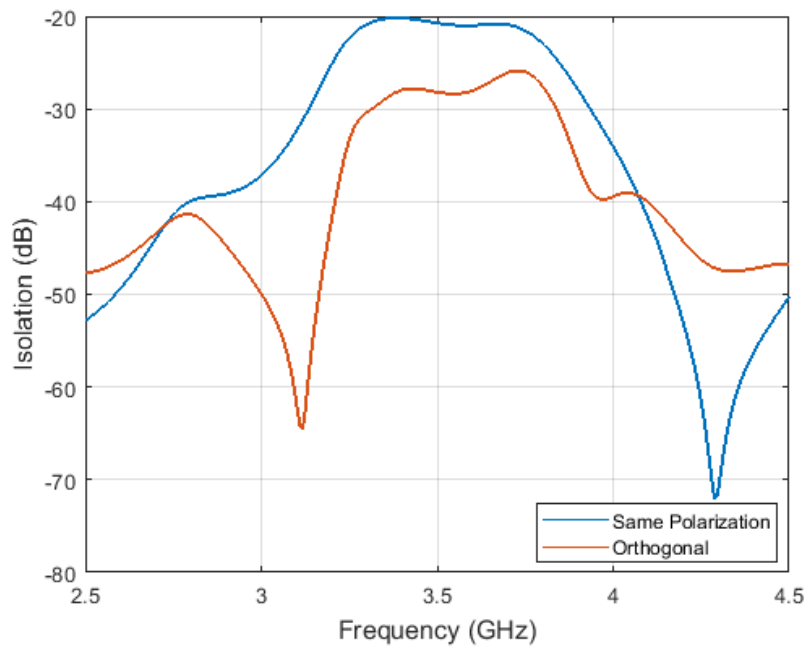
Figure 4.19. Isolation between adjacent sub-arrays for same and orthogonal polarized ports
