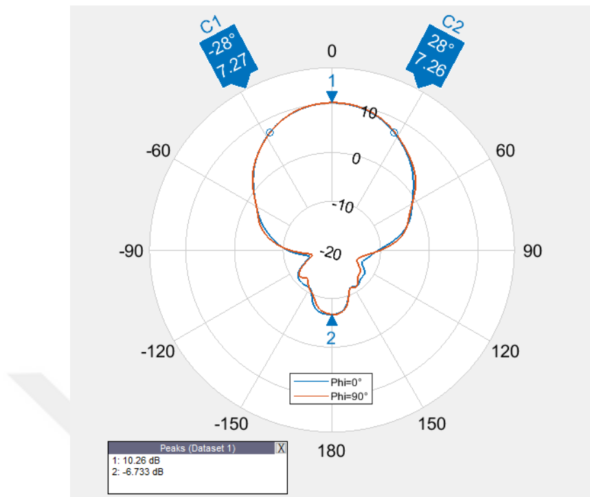
Figure 3.17. Radiation pattern of the unit element for \phi=0^\circ and \phi=90^\circ at 3.8 GHz
