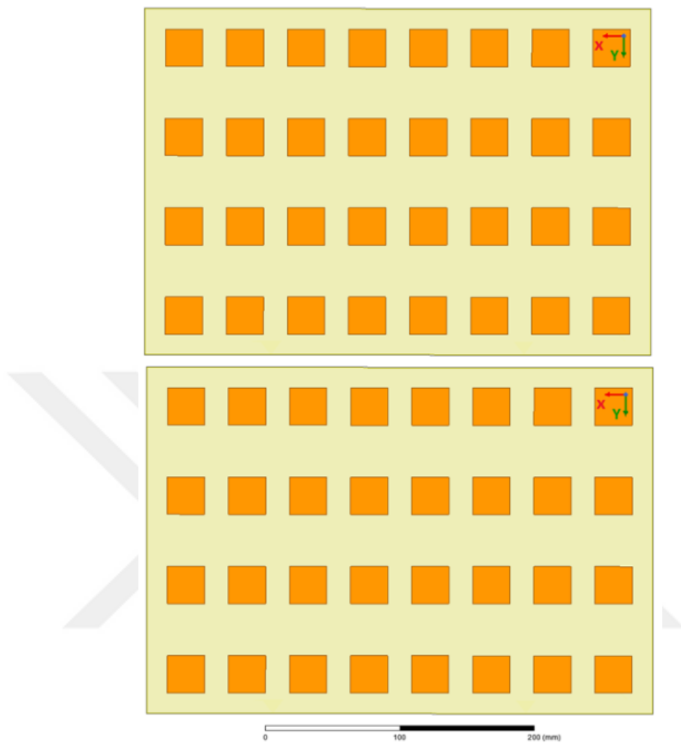
Figure 6.1. Two identical 8×4 arrays located side by side
