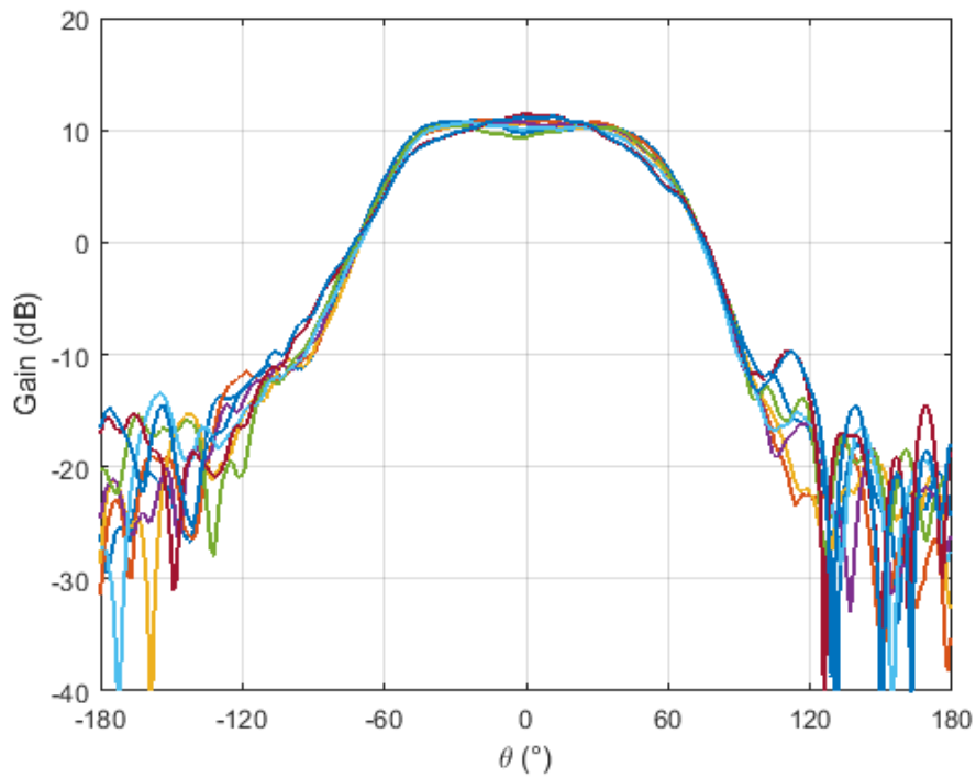
Figure 4.47. Co-Pol radiation pattern for port 9 through port 16 at \phi=0^\circ (3.5 GHz)
