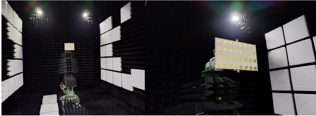
Figure 4.33. Radiation pattern measurements in the anechoic chamber
