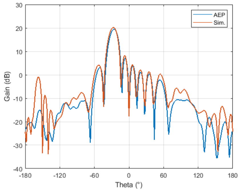
Figure 5.8. Co-Pol radiation pattern at \phi=0^\circ plane beam steered to \theta=-27^\circ with 90° progressive phase shift between elements (3.5 GHz)
