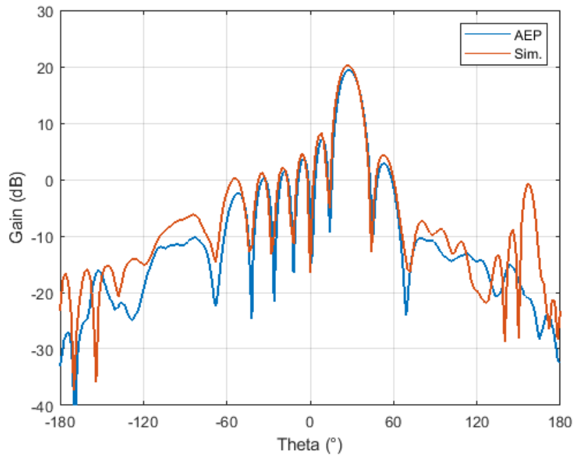
Figure 5.9. Co-Pol radiation pattern at \phi=0^\circ plane beam steered to \theta=27^\circ with 90° progressive phase shift between elements (3.5 GHz)
