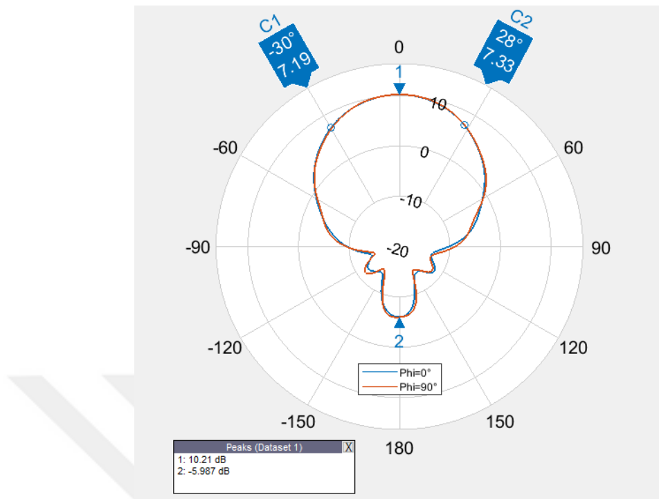
Figure 3.15. Radiation pattern of the unit element for \phi=0^\circ and \phi=90^\circ at 3.6 GHz
