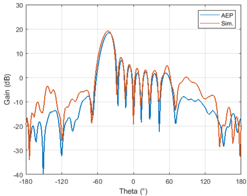
Figure 5.10. Co-Pol radiation pattern at \phi=0^\circ plane beam steered to \theta=-42^\circ with 135° progressive phase shift between elements (3.5 GHz)
