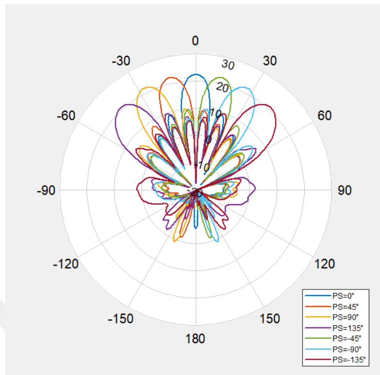
Figure 4.7. Steered beams in xz plane at 3.5 GHz
