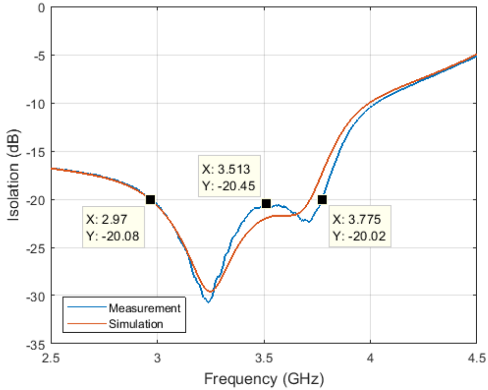
Figure 3.21. Simulation and measurement results comparison of port isolation of the prototype
