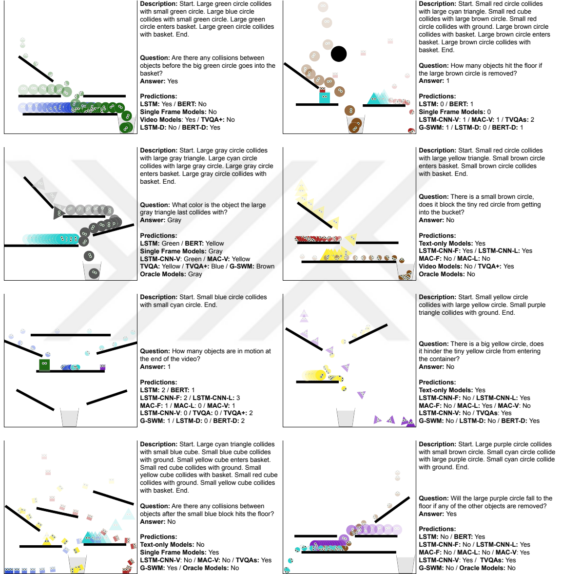
Figure 3.3: Selected baseline model predictions. The examples on the left belong to the descriptive category and the right column contains examples from the other categories.
