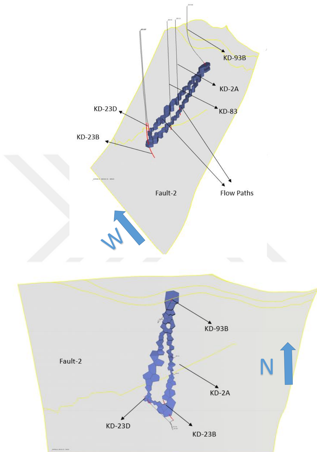
Figure 5-21 Flow paths between KD-93B and Observation Wells.
