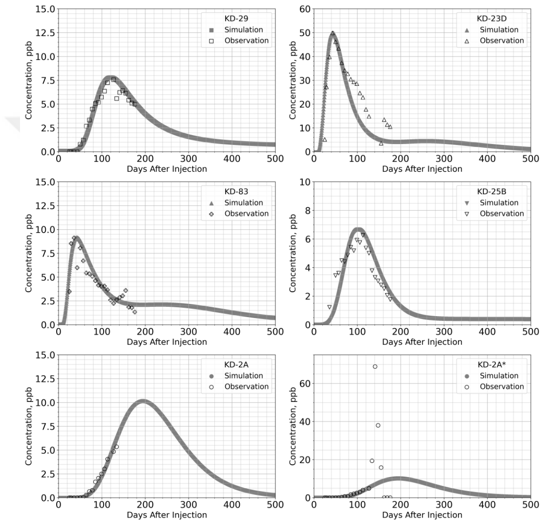
Figure 5-27 Numerical model results - Tracer breakthrough curves for the slug tracer test (2-6-NS) from KD-50A. The observation values are represented by the white markers and the simulated results by the dark markers.
