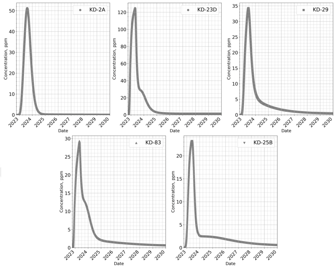
D. 5 CO 2 breakthrough curves for 6 months of 2500 tons/year CO 2 -brine injection.
