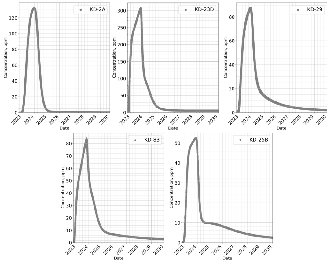
D. 10 CO 2 breakthrough curves for 12 months of 5000 tons/year CO 2 -brine injection.
