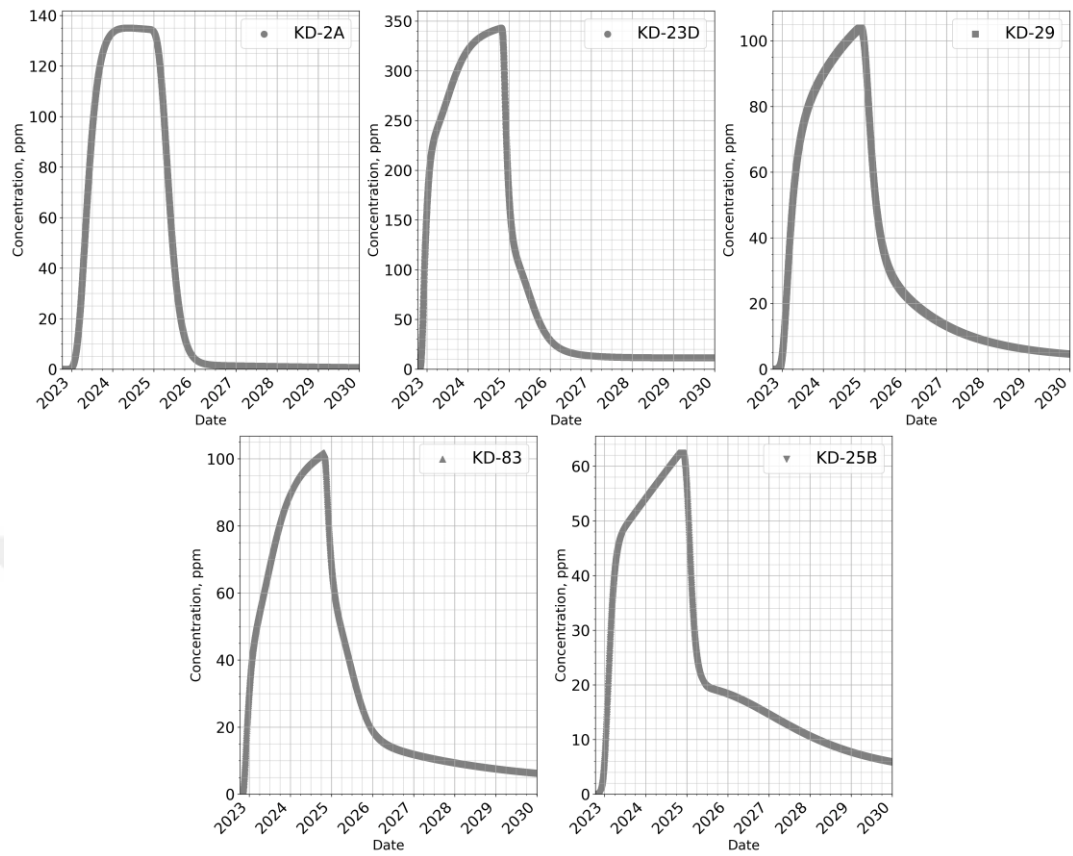
D. 11 CO 2 breakthrough curves for 24 months of 5000 tons/year CO 2 -brine injection.
