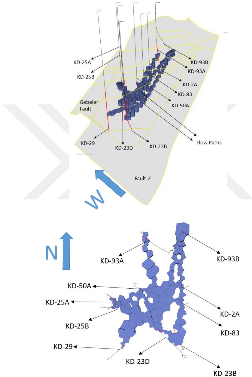
Figure 5-26 Flow paths between KD-93B, KD-50A, and neighbor wells.
