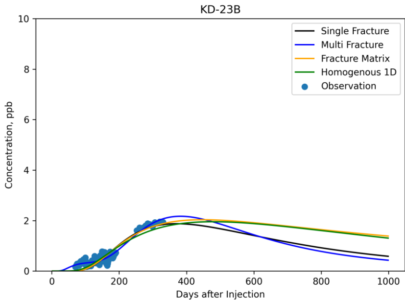
B. 1 Tracer Breakthrough Curves of the Analytical Models for KD-23B
