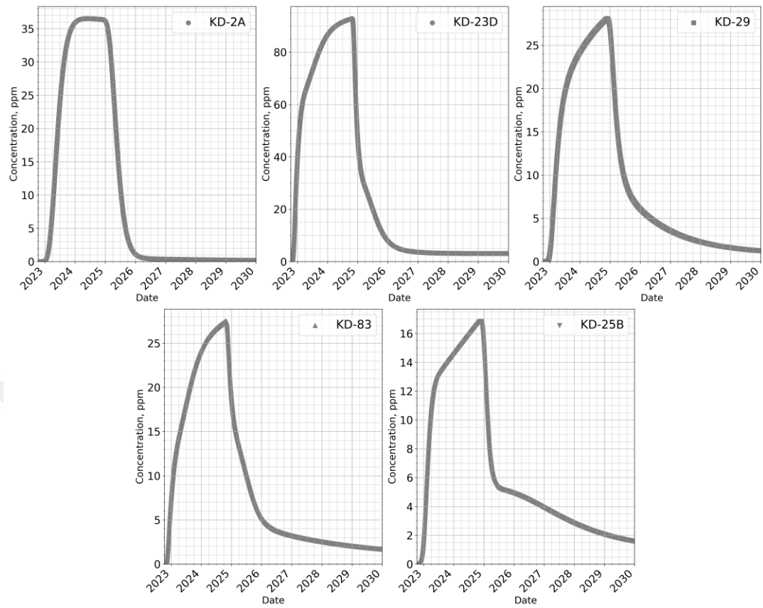
D. 3 CO 2 Breakthrough curves for 24 months of 1250 tons/year CO 2 -brine injection
