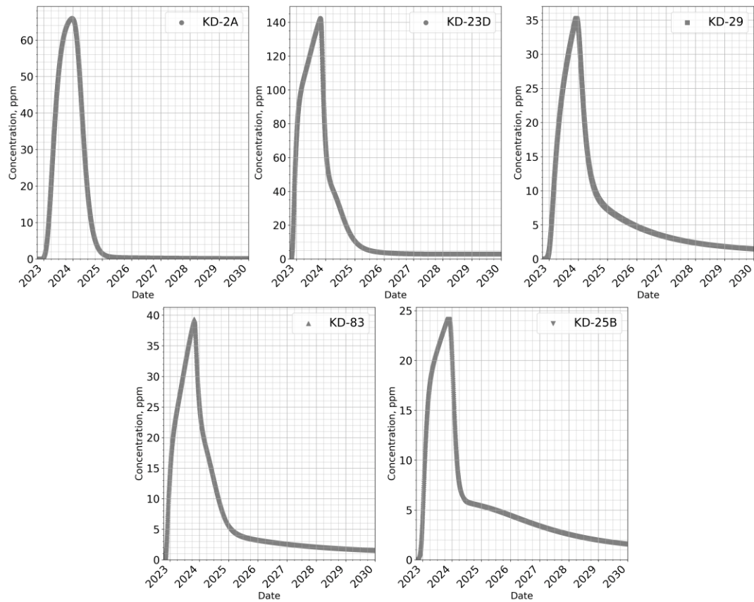
E. 4 CO 2 breakthrough curves for 12 months of 2500 tons/year CO 2 -brine injection (-6 bar constant bottom-hole pressure).
