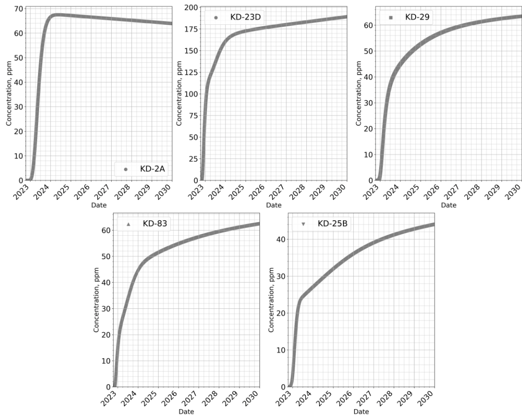
D. 8 CO 2 breakthrough curves for 8 years of 2500 tons/year CO 2 -brine injection.
