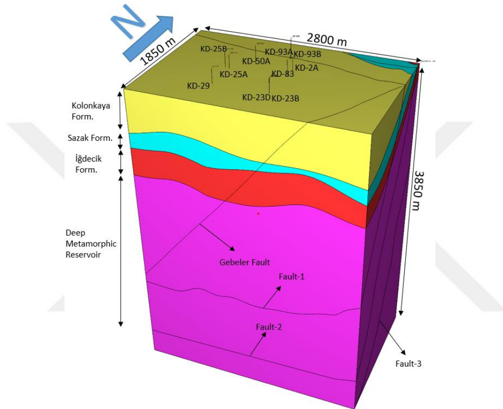
Figure 5-5 Finalized 3D Geological Model of the sector model region with formation boundaries, fault zones, and wells via Petrasim
