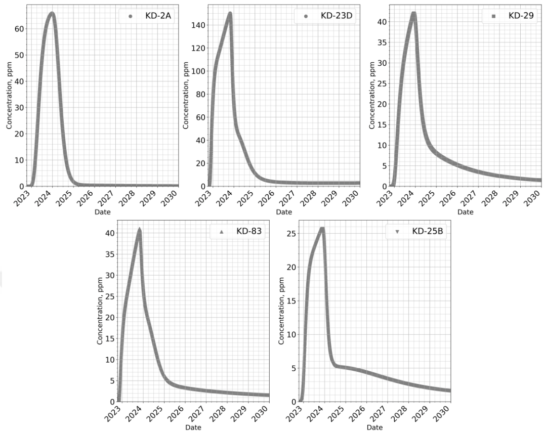
E. 3 CO 2 Breakthrough curves for 12 months of 2500 tons/year CO 2 -brine injection (-3 bar constant bottom-hole pressure).
