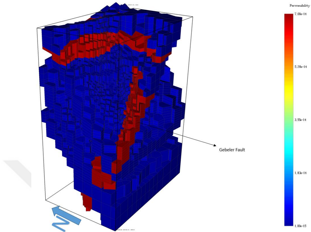
Figure 5-8 Initial permeability distribution along the faults.
