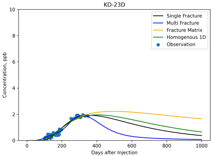
B. 2 Tracer Breakthrough Curves of the Analytical Models for KD-23D
