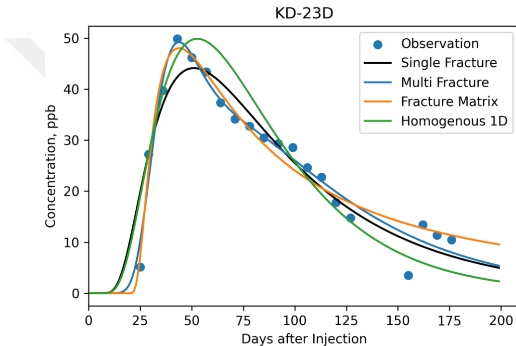
Figure 5-25 Tracer Breakthrough Curves of the Analytical Models for KD-23D.
