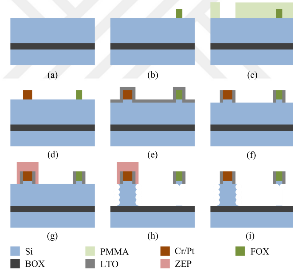
Figure 26: Single piezoresistive silicon nanowire fabrication flow on 10μm device layer SOI: a) n^{++} doping, b) e-beam lithography on FOX16, c) coating and e-beam patterning of double PMMA layers, d) Cr/Pt deposition and lift-off, e) RIE etching of Si and LTO coating, f) directional etching of LTO, g) Dicing, coating and patterning of ZEP520A 100%, h) BOSCH Process on Si, and i) Removal of ZEP520A 100% and other residuals with O_2 plasma.
