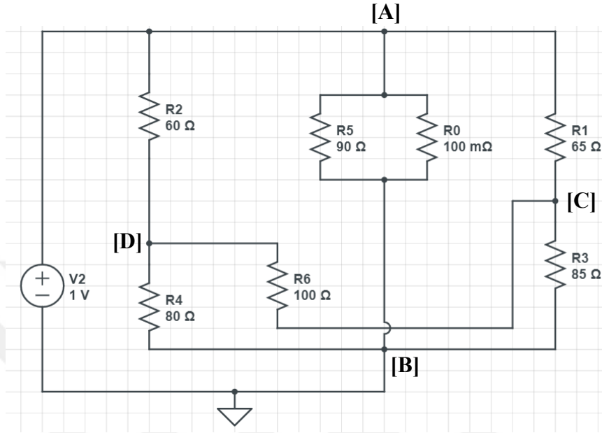
Figure 51: Path A-B circuitry simulation from www.circuitlab.com .
