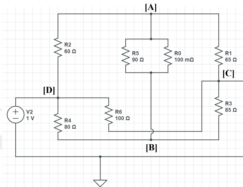
Figure 52: Path D-C circuitry simulation from www.circuitlab.com .
