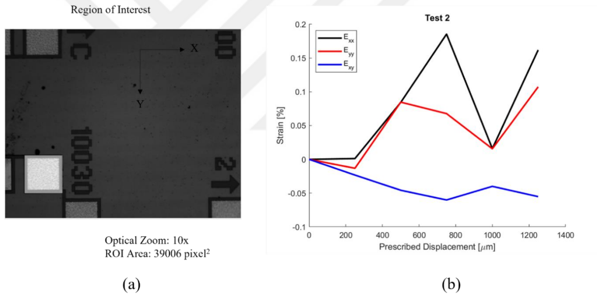
Figure 75: (a) Image taken from PixelINK camera with 10x lens and selected ROI, (b) engineering strain obtained with DIC analysis for test 2.
