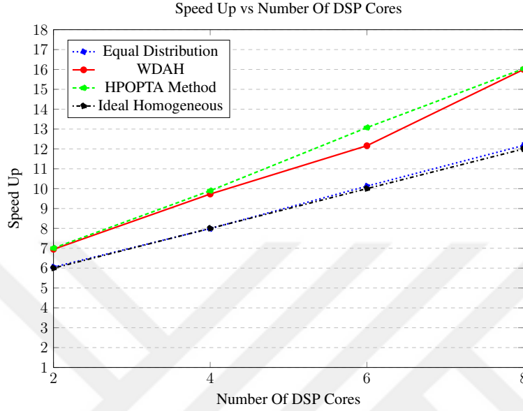
Figure 5.6: Matrix Multiplication Speed Up ( 4ARM_{Cores} + xDSP_{Cores} )
