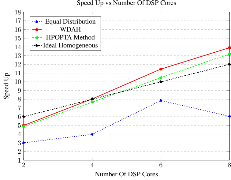
Figure 5.8: FIR Speed Up ( 4ARM_{Cores} + xDSP_{Cores} )
