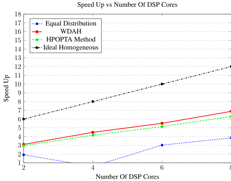
Figure 5.7: FFT Speed Up ( 4ARM_{Cores} + xDSP_{Cores} )
