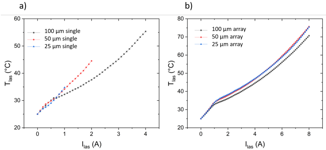
Figure 5.16: Laser temperature of all LDs (a) single lasers, and (b) array lasers
