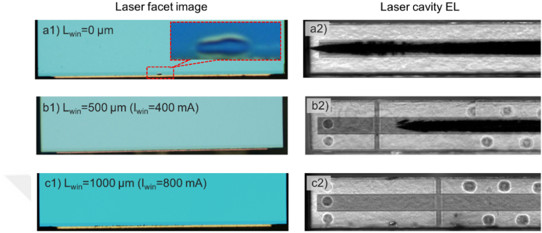
Figure 4.20: Optical microscope image of the laser facet and top EL image of the laser cavity after 20 A, CW, 20 °C overdrive tests: (a1-2) L_{win} = 0 \mu\text{m} , (b1-2) L_{win} = 500 \mu\text{m} , (c1-2) L_{win} = 1000 \mu\text{m} .
