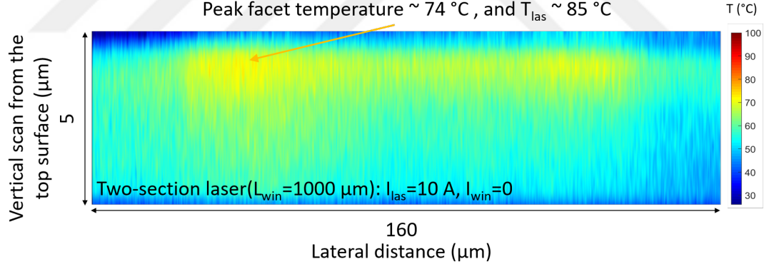
Figure 4.15: An enlarged view of the facet temperature map of the two section LD with L_{win}=1000\text{ }\mu\text{m} at I_{las} = 10\text{ A} .
