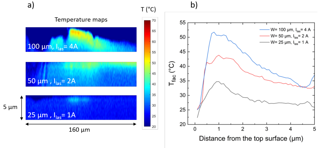
Figure 5.17: Comparison of facet temperature for all single waveguide two-section LDs at I_{las}=4 , 2, and 1 A with I_{win}=0 at T=24^{\circ}\text{C} . (a) Facet temperature maps. (b) Vertical temperature scan of the temperature maps.
