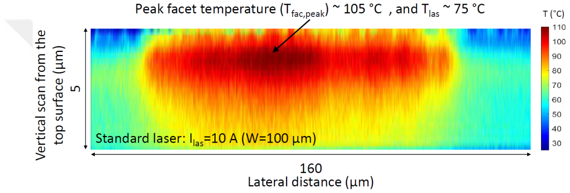
Figure 3.7: An enlarged view of the facet temperature map at I_{las}=10 A.
