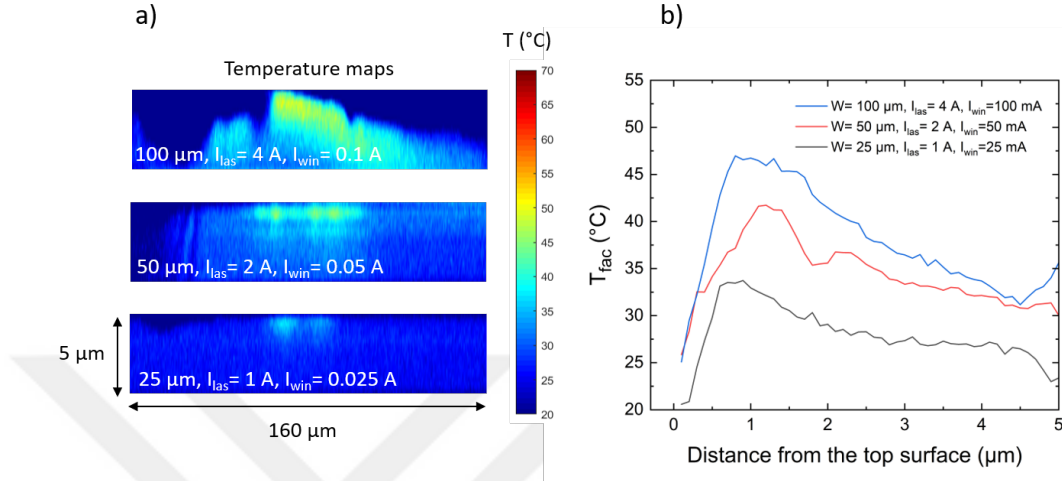
Figure 5.18: Temperature characterization results of the two-section single waveguide LDs with I_{win} (a) Temperature maps. (b) Vertical temperature scan of the temperature maps.
