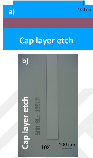
Figure 5.5: (a) Schematic of out put facet after cap layer etch. (b) Top view of the device after cap layer etch taken by optical microscopy with 10x lens.
