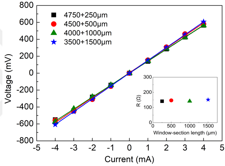
Figure 4.4: Resistance comparison of 4750+250 \mu\text{m} , 4500+500 \mu\text{m} , 4000+1000 \mu\text{m} , 3500+1500 \mu\text{m} LDs.
