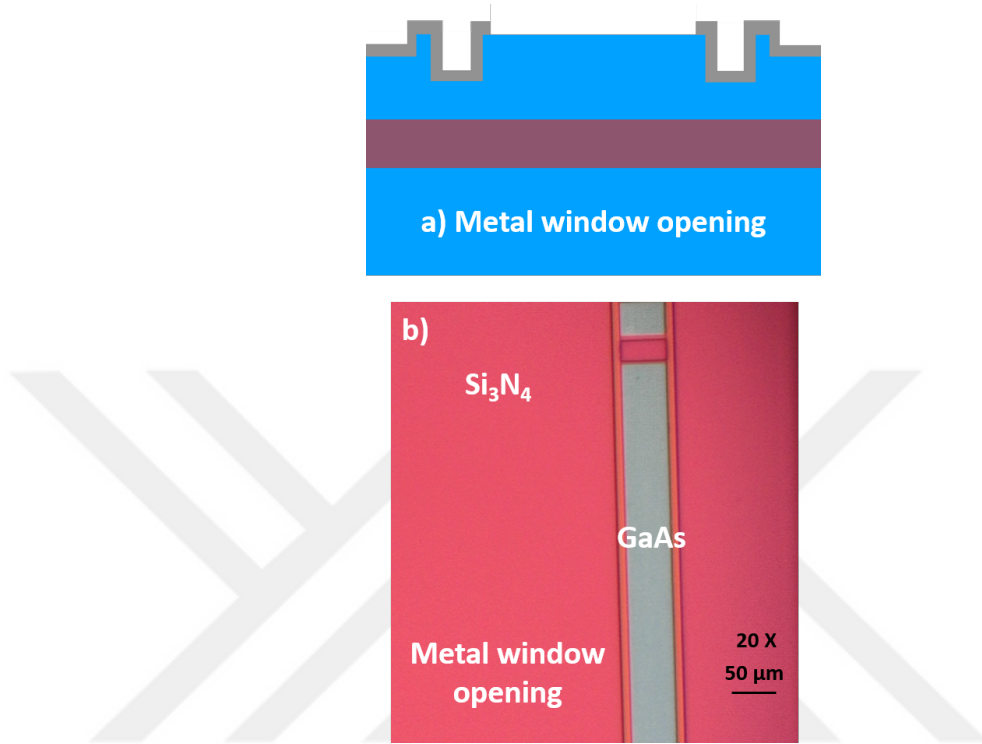
Figure 5.7: (a) Facet view of the structure after window opening. (b) Optical microscopy image from the top after window opening, red area is silicon nitride, and white area is the window opening.
