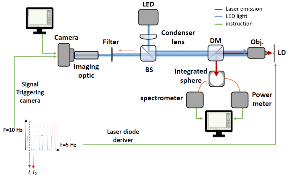
Figure 2.2: Schematic of the thermoreflectance setup.
