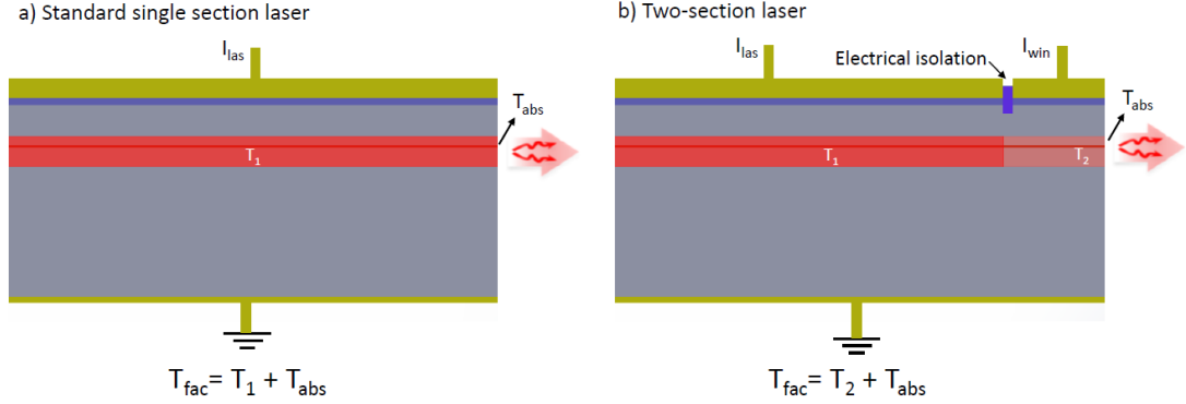
Figure 4.1: Schematic description of internal heat in (a) standard LD, and (b) two-section LD.
