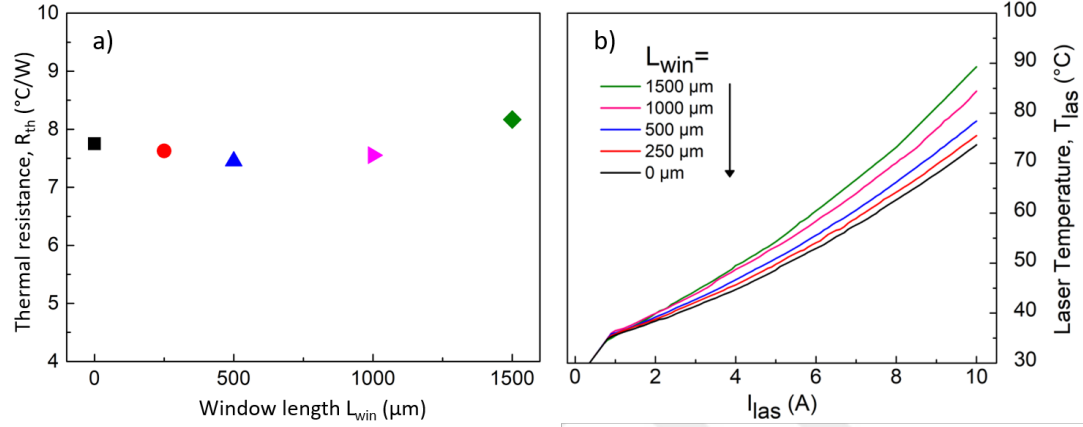
Figure 4.13: (a) Thermal resistance value of LDs studied in this work (b) Laser temperature of all LDs.
