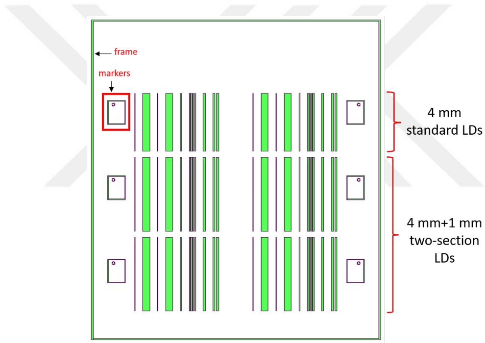
Figure 5.3: General view of the mask design.
