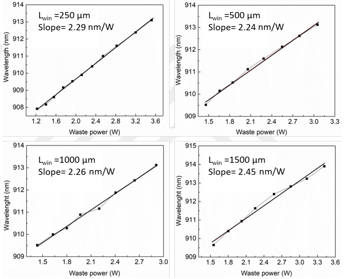
Figure 4.12: Graphs of wavelength variation with waste power at T = 25^\circ C for each LD with L_{win} .
