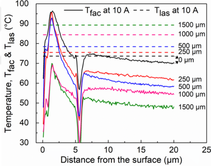
Figure 4.16: Vertical temperature scan of the figure 2-D temperature maps showing T_{fac} vs. distance from the top surface and T_{las} for I_{las}=10 A.
