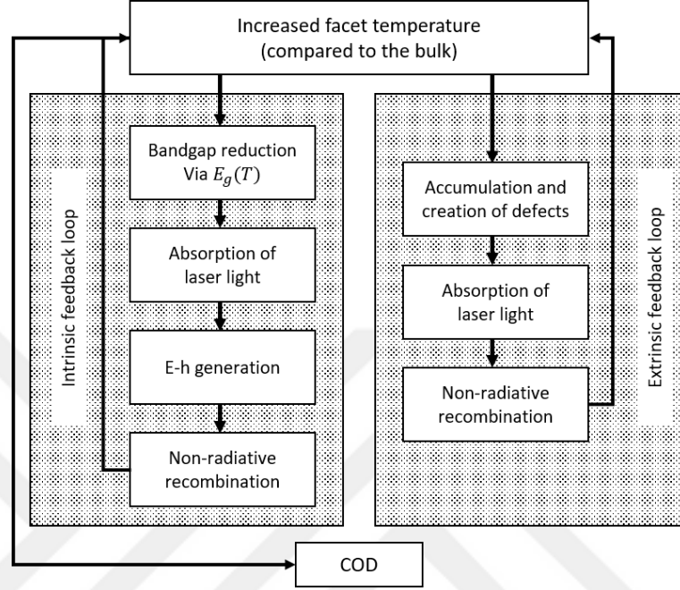
Figure 1.2: Thermal runaway feedback mechanism for COD [14].
