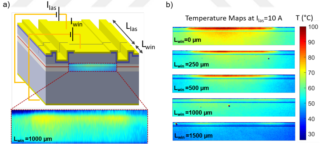
Figure 4.14: Comparison of temperature characteristics for all multi-section LDs at I_{las}=10\text{ A} and I_{win}=0 . (a) LD structure and the enlarged image corresponding to the heated region of the facet for L_{win}=1000\text{ }\mu\text{m} . (b) temperature distribution maps.
