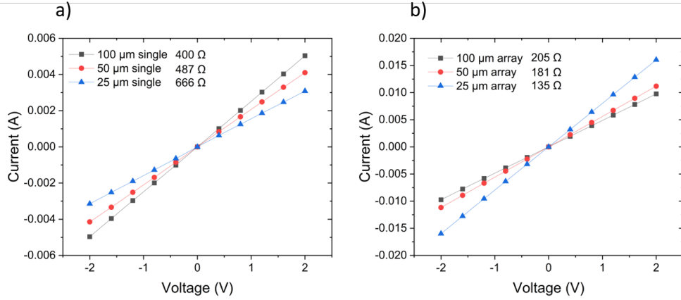
Figure 5.10: Resistance value between gain section and transparent window for (a) single lasers (b) array lasers.
