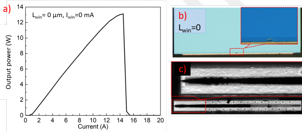
Figure 3.9: LD failure test. (a) output power versus current for LD with L_{win}=0 , under CW, 20 °C operation. (b) optical microscope image of the LD output facet. (c) EL image of the laser cavity.
