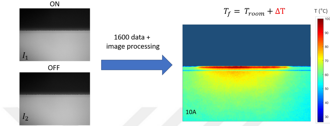
Figure 2.7: Obtaining LD facet temperature from raw data by doing image processing.
