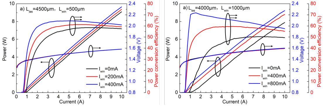
Figure 4.10: I_{win} effect on performance of two-section LDs. (a) L_{win}=500\text{ }\mu\text{m} and (b) L_{win}=1000\text{ }\mu\text{m} .
