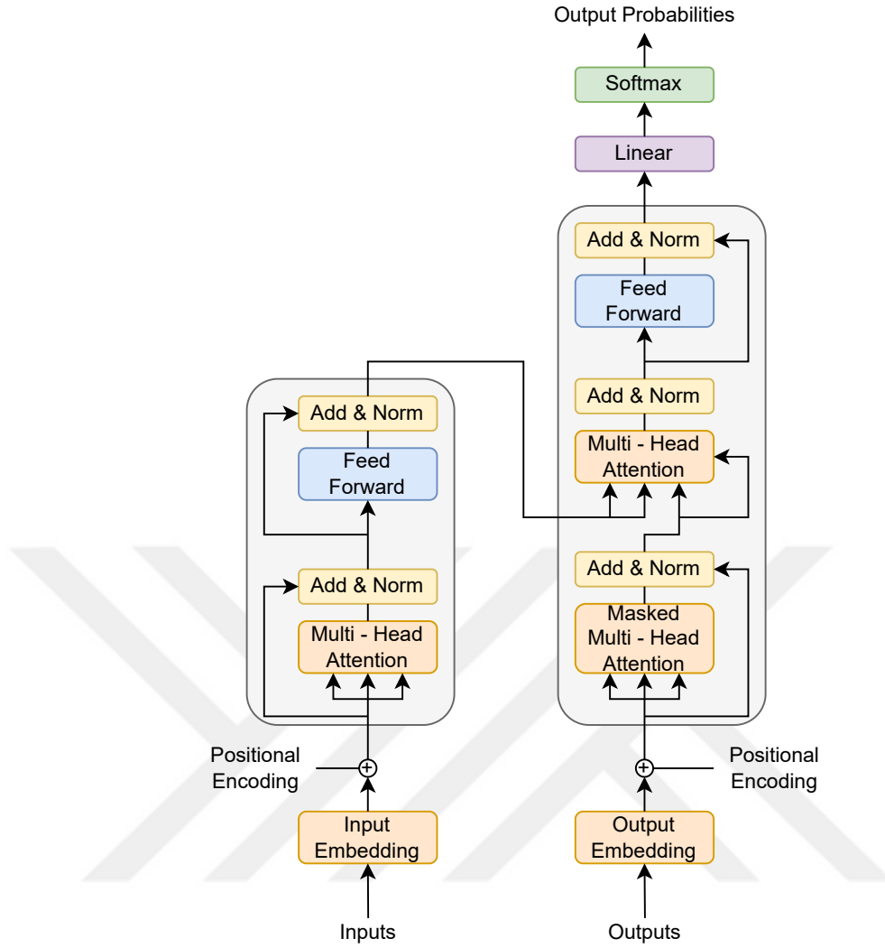
Figure 3.8 Transformer (Vaswani et al., 2017). The encoder layer is placed on the left, and the decoder layer is placed on the right. In the figure, both encoder and decoder layers contain a single block. Different implementations can use multiple blocks in both encoder and decoder layers.
