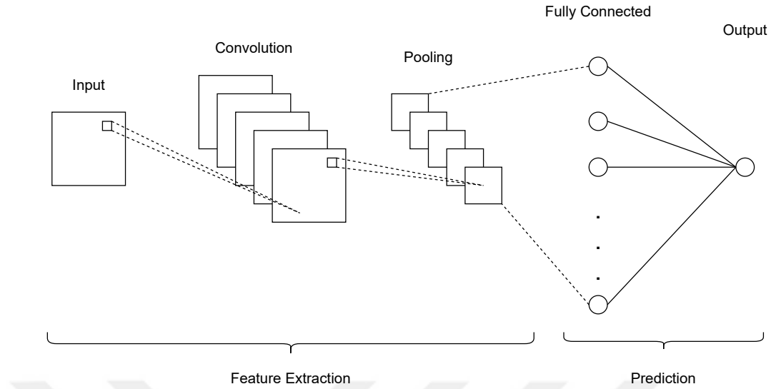
Figure 3.3 Architecture of a basic convolutional neural network. Contains a single convolution layer with 5 filters and single pooling layer for each filter. Output of the pooling layer is flattened and fed to the fully connected layer to perform prediction.
