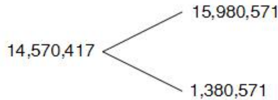
Figure 2.14 The NPV lattice ($) - investment between centers 1 and 2, Option 2
