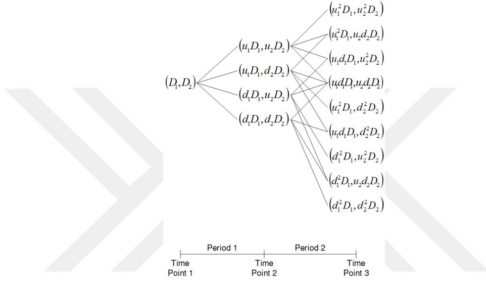
Figure 2.3 The multiple-branch lattice
