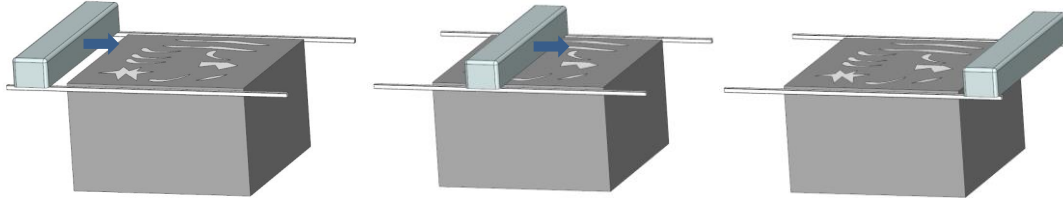
Figure 6.4 Inspection array probe surface inspection (probe moving rightwards)
