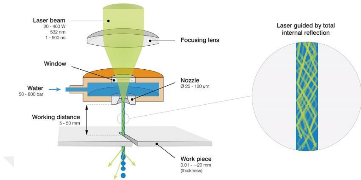
Figure 4.12 Water jet guided laser system (Synova) [31]
