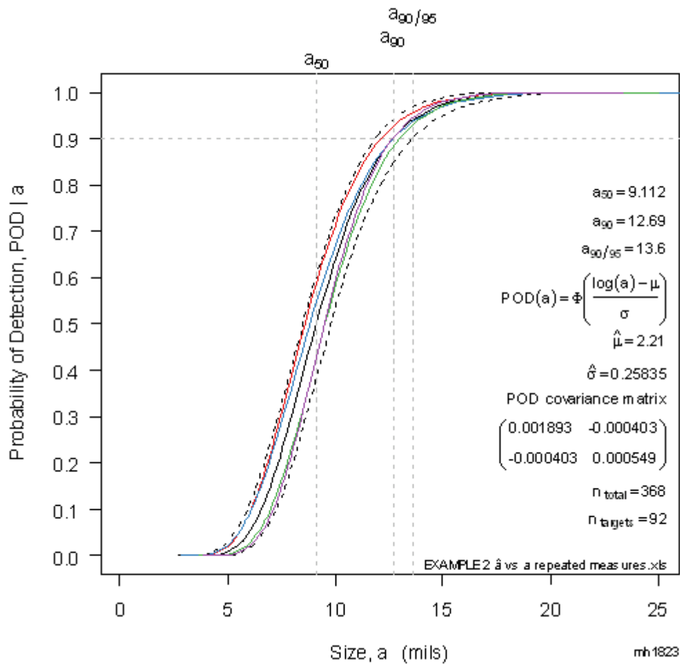
Figure 5.24 POD(a) for the data sample data set (4 test repeat) [32]
