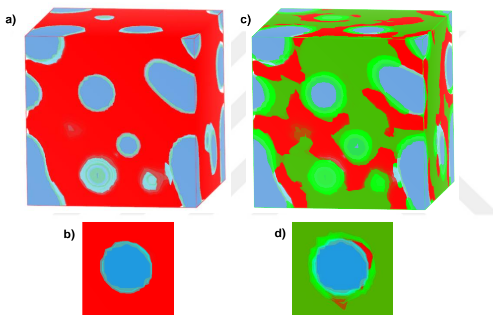
Figure 5.67. The field density distribution of nanoparticles in oil without (a, b) and with (c, d) the depiction of polar amine center in dispersant and sulfonate head group.
