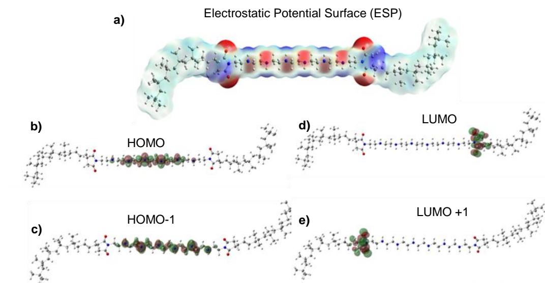
Figure 5.3. a) Electrostatic Surface Potential, b) HOMO, c) HOMO-1, d) LUMO, and e) LUMO+1 structures of dispersant molecule.
