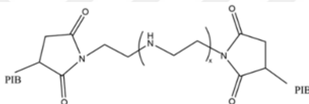
Figure 5.2. PIB-bis-succinimide dispersant molecular structure.
