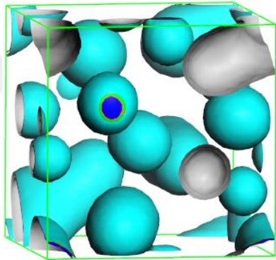
Figure 5.63. Insoluble nanoparticle isosurface structures with a) 10% disp - 85% oil - 5% np, b) 10% disp- 80% oil - 10% np, c) 10% disp- 75% oil - 15% np, d) 10% disp- 60% oil - 30% np ratios.
