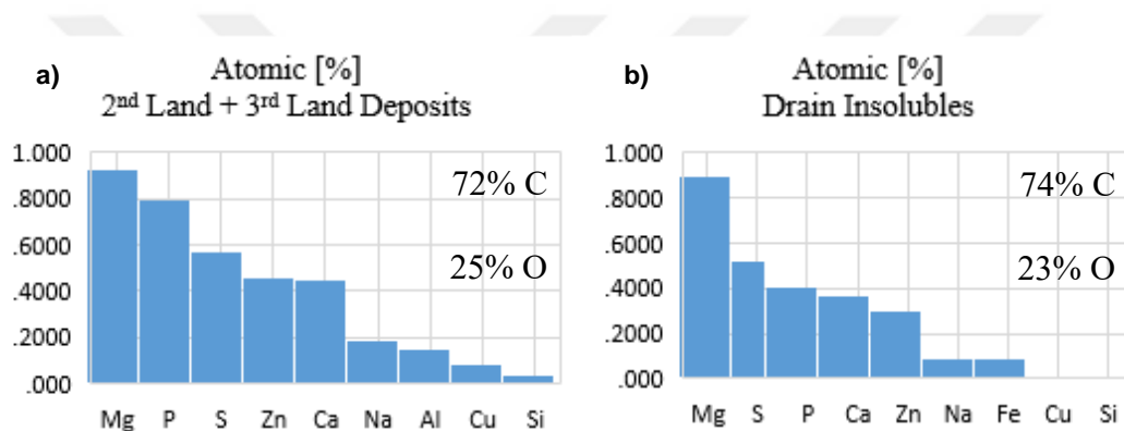
Figure 2.6. Elemental analysis of a) land deposits b) drain insolubles.
