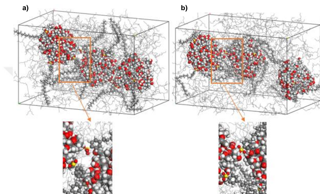
Figure 5.47. a) The first frame and b) the last frame of MD simulations of three nanoparticles with twelve sulfonate detergent molecules. Inset figures show detailed captures.
