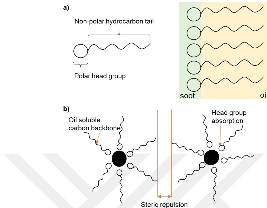
Figure 1.2. a) Schematic representation of groups of dispersant molecule and mechanism, b) steric repulsion of engine oil contaminants surrounded with dispersant molecules.
