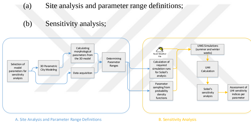
Figure 26 Framework for urban heat island sensitivity analysis
