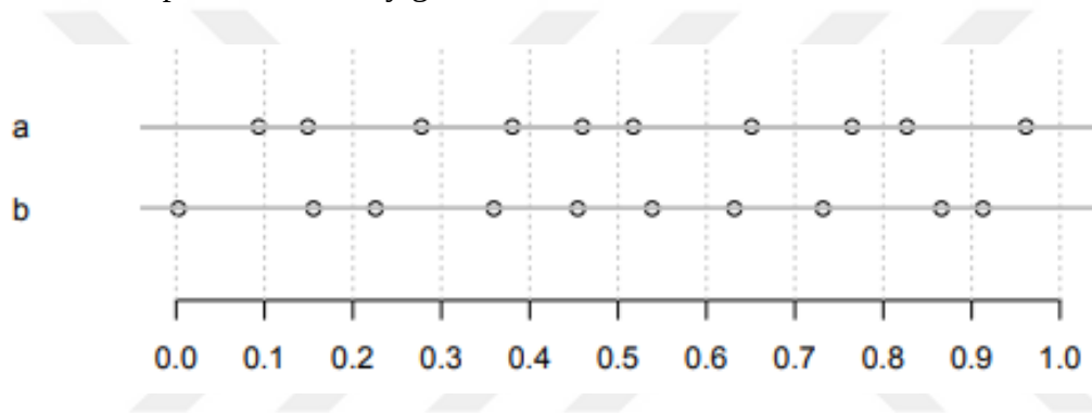
Figure 22 - Example of an plot generated with one dimensional stratified sampling 168 .
