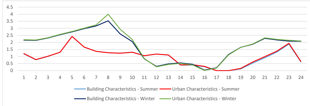
Figure 31 Mean UHI intensity for all parameter groups by hour
