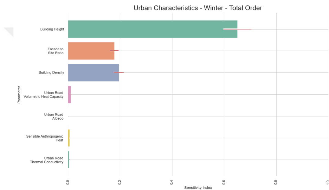
Figure 34 Winter season total order urban characteristics sensitivity analysis result
