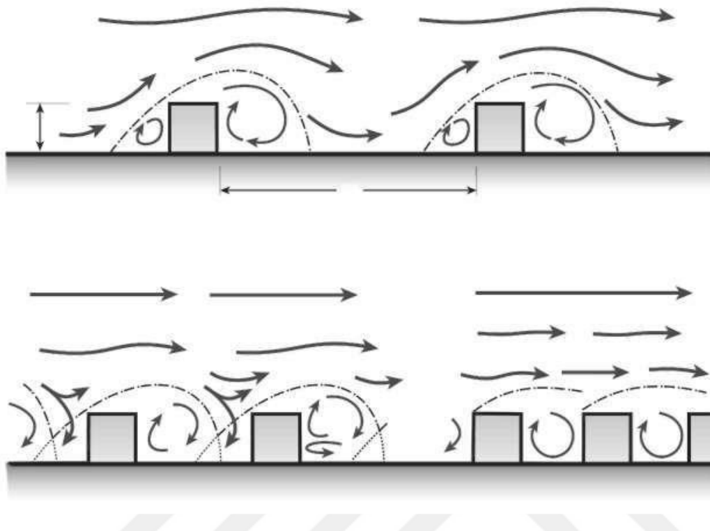
Figure 13 – Air flow patterns associated with various urban geometries, drawn by Oke 66 with regards to the wind tunnel experiments carried out by Hussain and Lee 67 and redrawn by Erell et. al. 68
