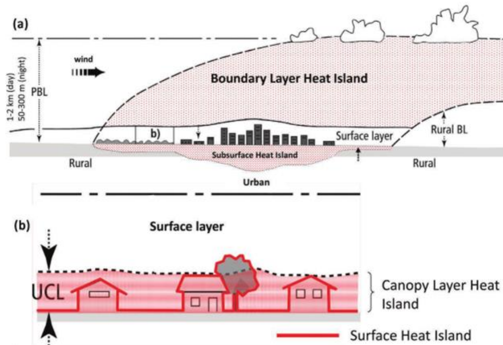
Figure 5 (a): Under certain weather conditions, inside the planetary boundary layer (PBL) which exists 1-2km above the planet's surface, a characteristic plume shape extending in the downwind direction defines the boundary layer heat island (b): Zoomed in diagram of a canopy layer and surface heat island 34
