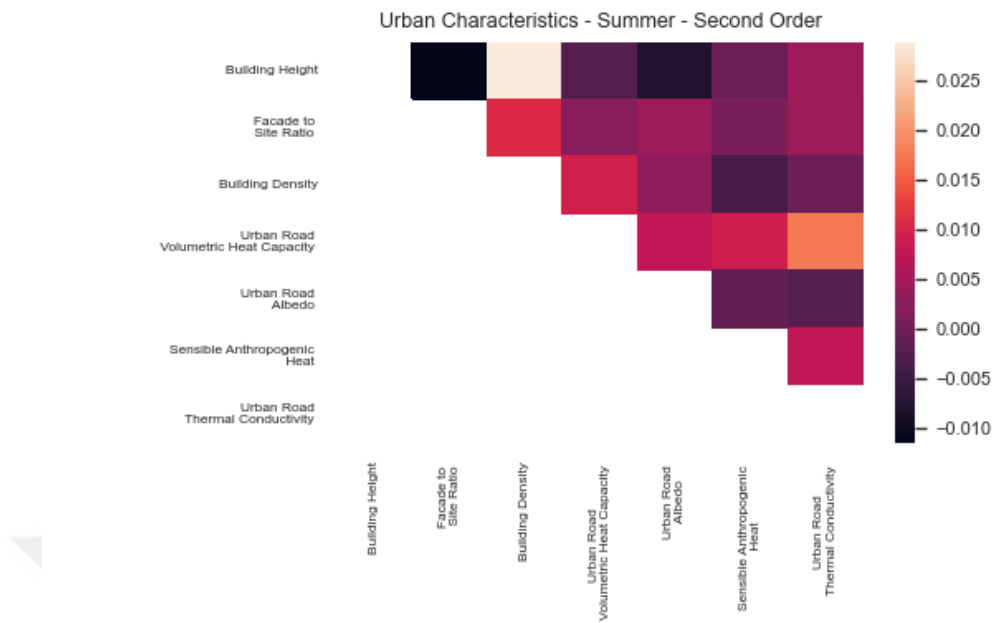
Figure 37 Summer season second order urban characteristics sensitivity analysis result
