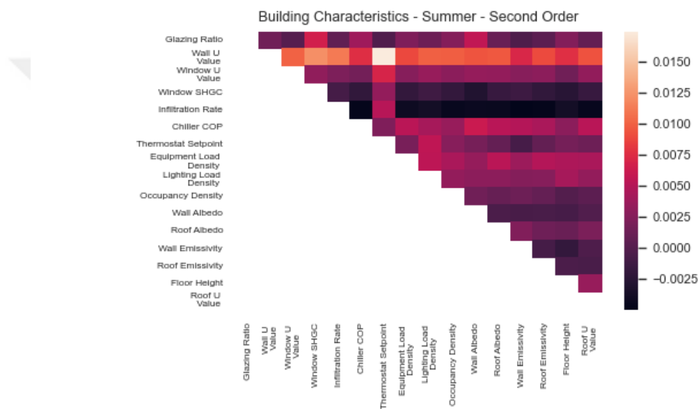
Figure 39 Summer season second order building characteristics sensitivity analysis result
