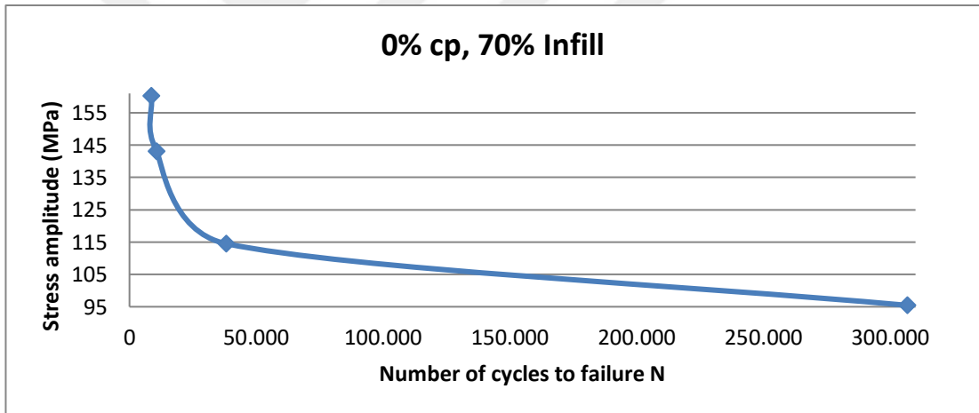
Figure 4.18. S-N Curve for (Sample 2).
