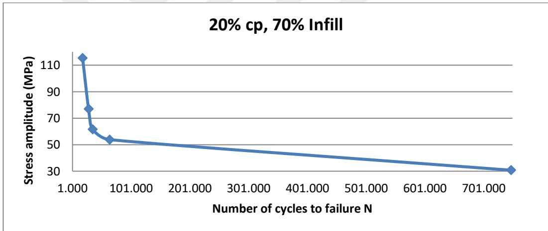
Figure 4.22. S-N Curve for (Sample 6).
