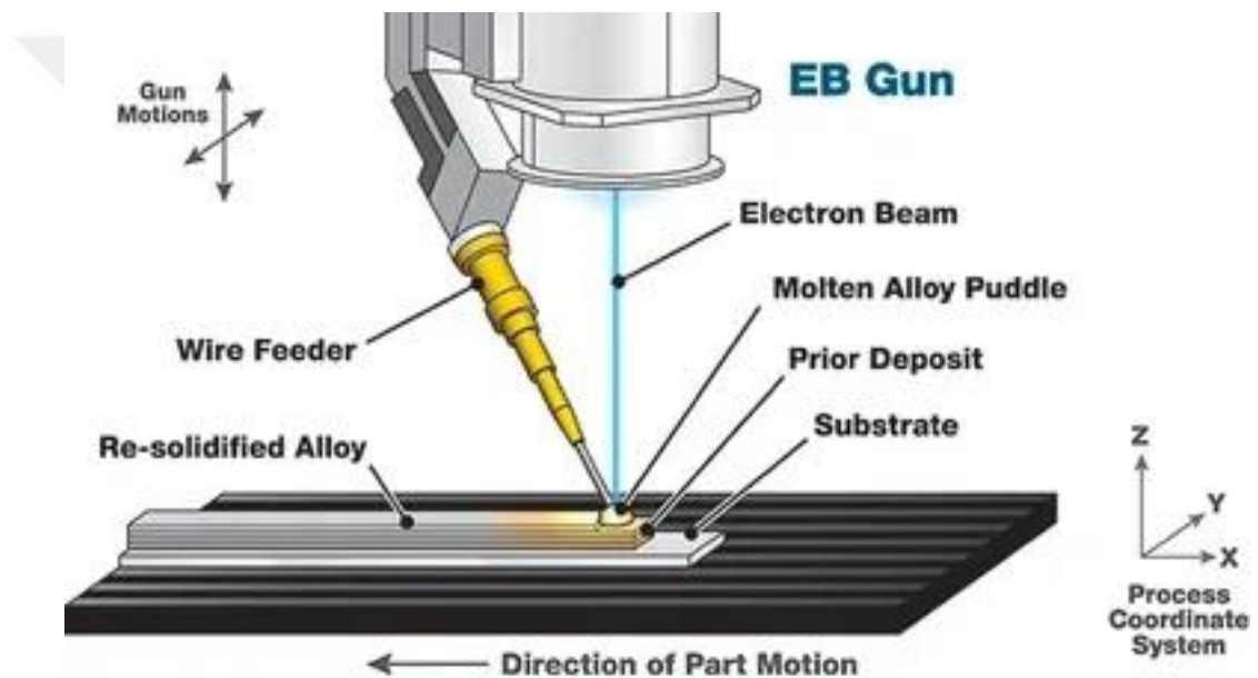
Figure 2.12. EBAM Technology Working Principle [38].
