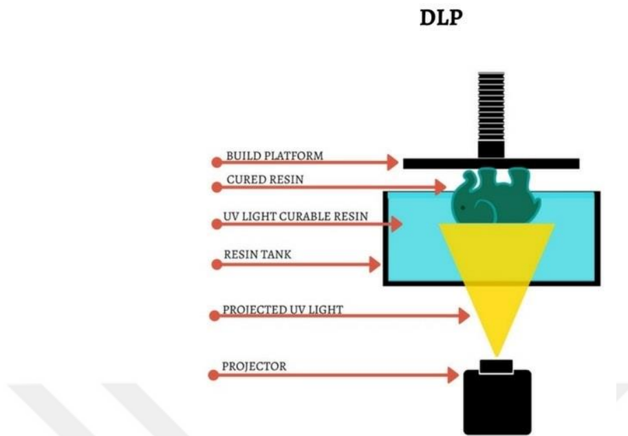
Figure 2.14. Principle of DLP Technology [40].
