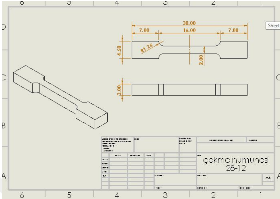
Figure 4.2. Tensile test design.
