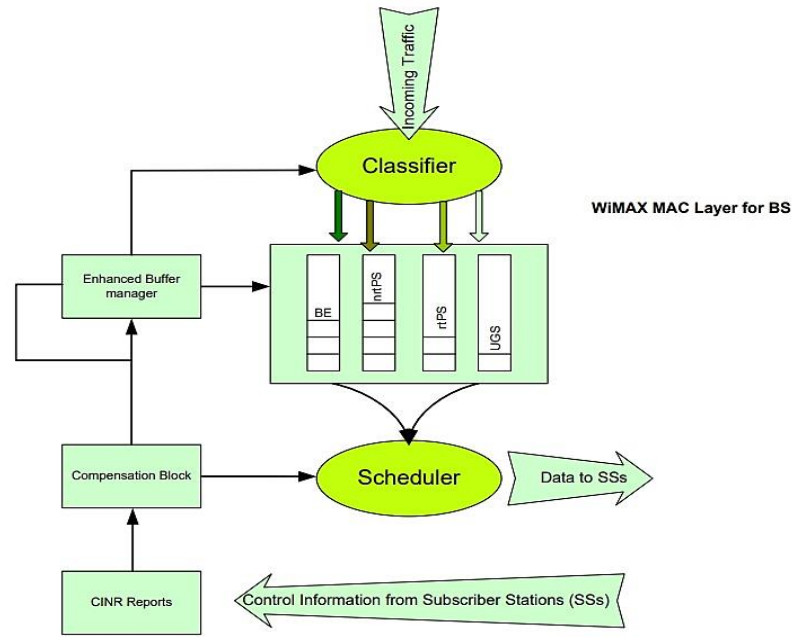
Figure 3.6. WiMAX BS Architecture
