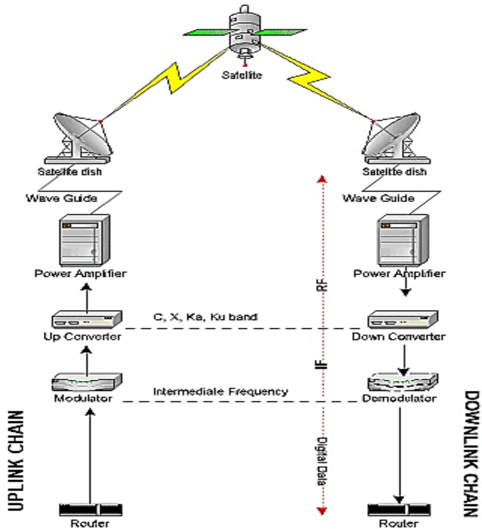
Figure 3.19.Uplink and downlink in wireless networks.
