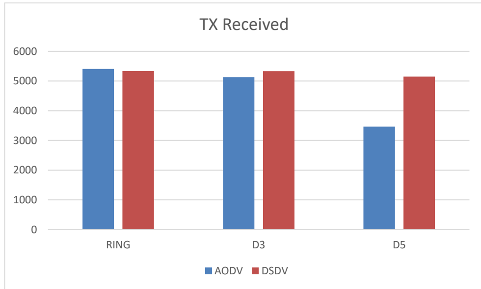
Figure 4.8.Total received packets in both proposed routing protocols.
