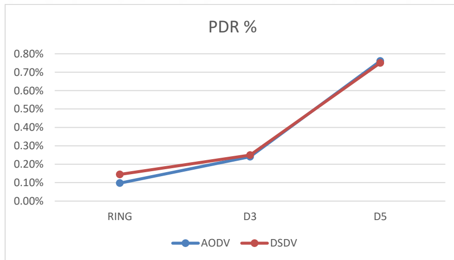
Figure 4.9.Packet delivery rate in both proposed routing protocols.
