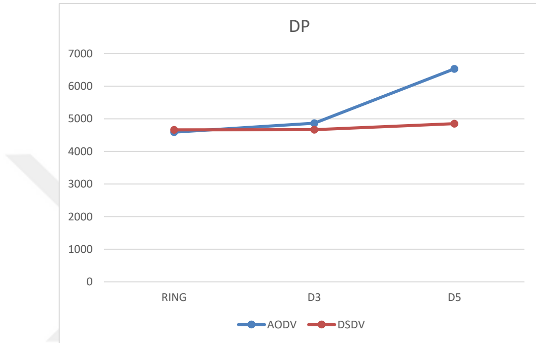
Figure 4.10.Total dropped packets in both proposed routing protocols.
