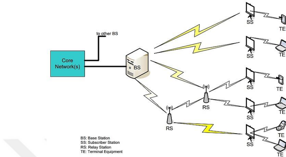
Figure 3.8.IEEE 802.16 network architecture (WiMAX)
