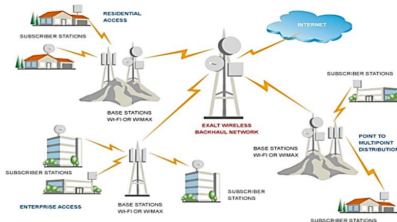
Figure 2.13.IEEE 802.16 WiMAX Network
