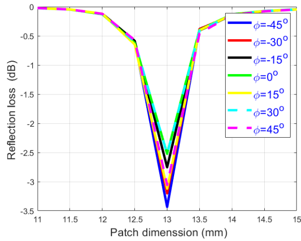
Figure 5.10. S11 parameter of single layer unit cell ( \theta=30^\circ ).
