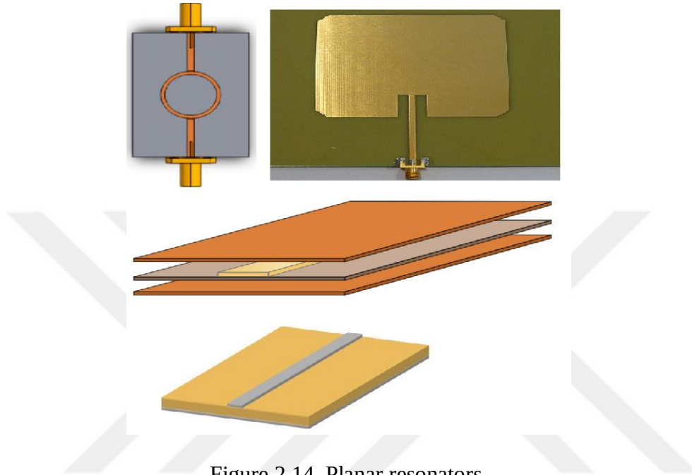
Figure 2.14. Planar resonators.
