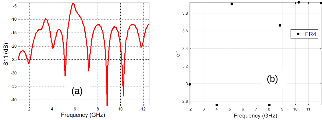
Figure 3.47. (a) S11-Parameter of the microstrip line on the FR4 substrate. (b) Dielectric constant of FR4 using the transmission line method.
