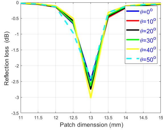
Figure 5.8. Reflection loss single layer unit cell ( \varphi=90^\circ ).
