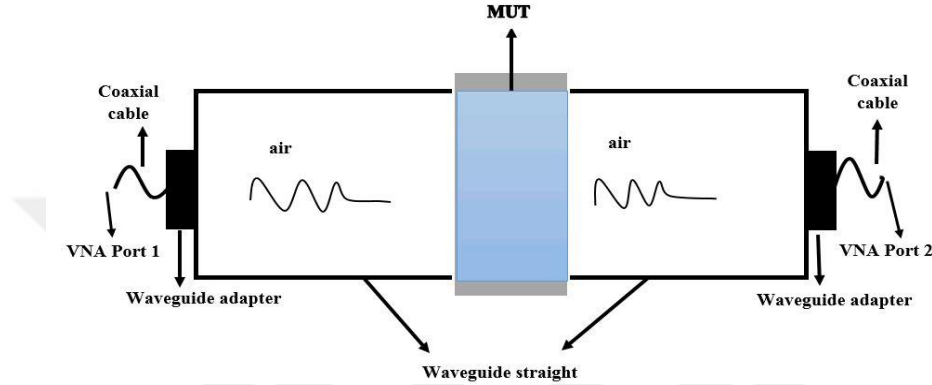
Figure 3.1. Waveguide setup.
