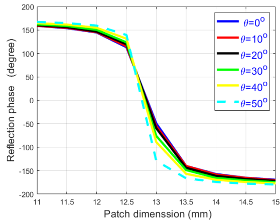
Figure 5.3. Phase variation of single layer unit cell ( \phi=0^\circ ).
