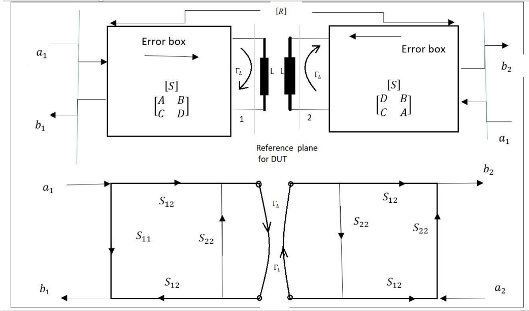
Figure 3.8. Block diagram and signal flow graph of reflection connection [25].
