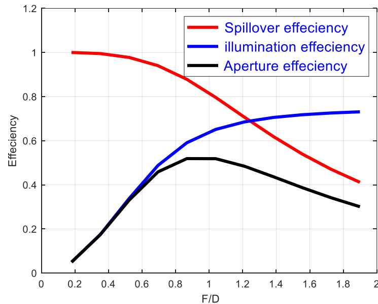
Figure 5.47. Efficiencies for F/D ratio.
