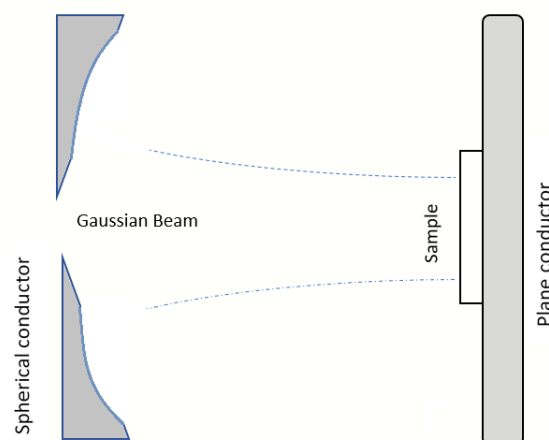
Figure 2.13. Open resonator.
