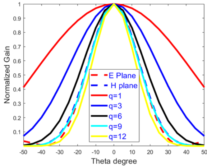
Figure 5.38. Feed antenna radiation pattern corresponding to different values of q .
