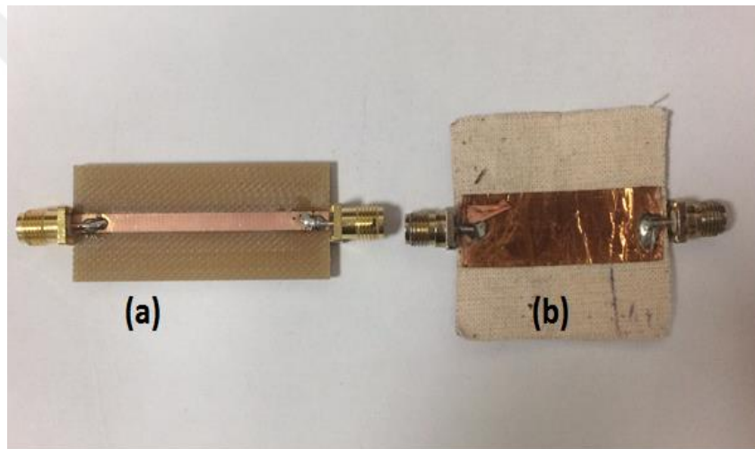
Figure 3.12. (a) Transmission line fabricated on FR4. (b) Transmission line fabricated on cotton textile.
