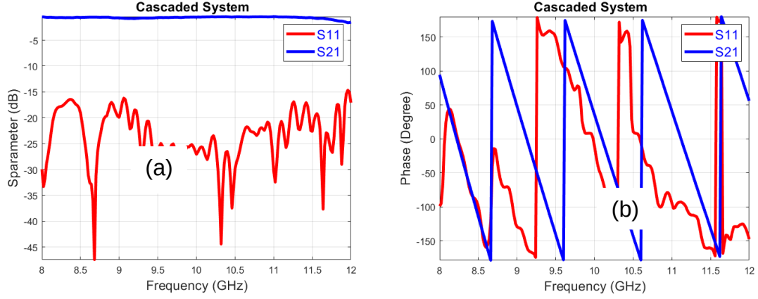
Figure 3.18. S-Parameters of cascaded system. (a) S-Parameters magnitude in dB. (b) Phase in degree.
