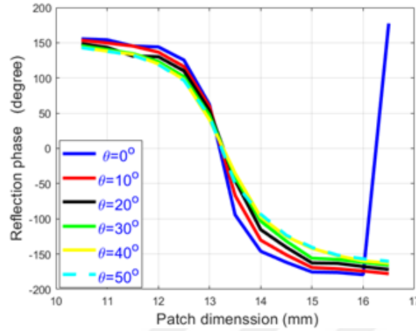
Figure 5.18. The return phase of two-layer unit cell ( \varphi=0^\circ ).
