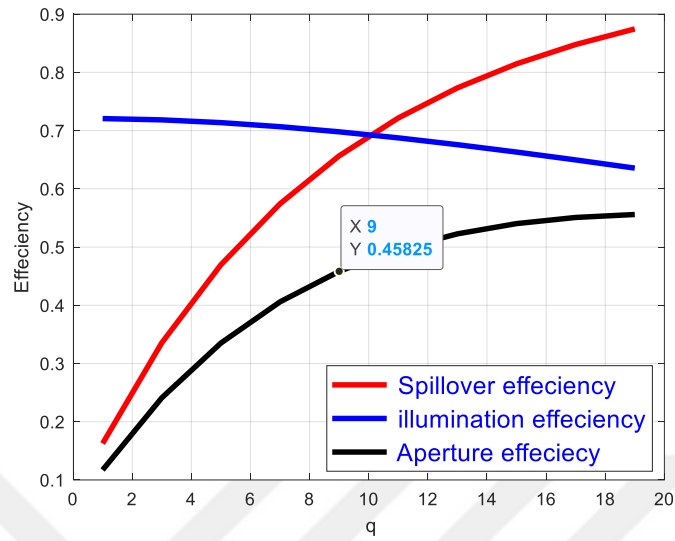
Figure 5.46. Calculated efficiencies of offset feed configuration concerning q . It is observed from the figure that for offset configuration for q=9 , the illumination efficiency is around 70%, Spillover efficiency is 65%, whereas the aperture efficiency is about 45%. The effect of the F/D ratio on efficiency is shown in Figure 5.47.
