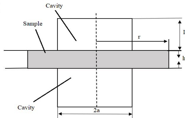
Figure 2.12. Split resonator method.
