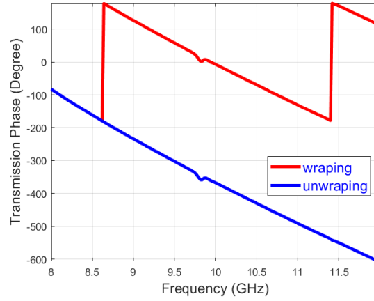
Figure 3.27. Transmission phase wrapping and unwrapping.
