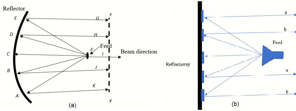
Figure 5.26. (a) Parabolic reflector. (b) Reflectarray.
