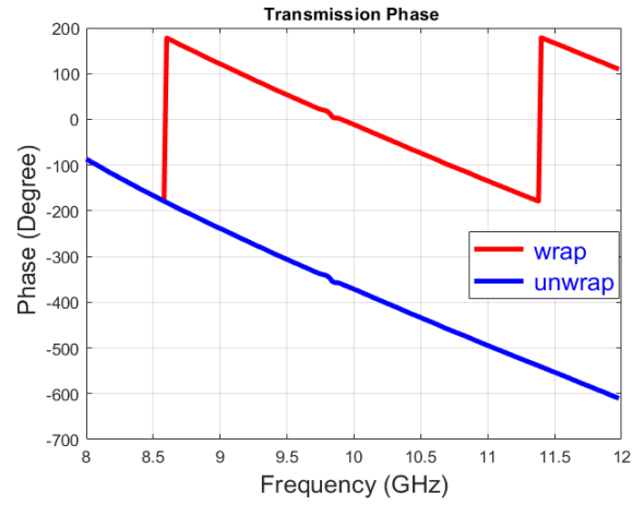
Figure 3.33. Transmission phase wrapping and unwrapping.
