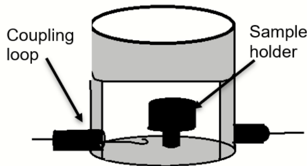
Figure 2.11. 3D view of the cavity resonator.
