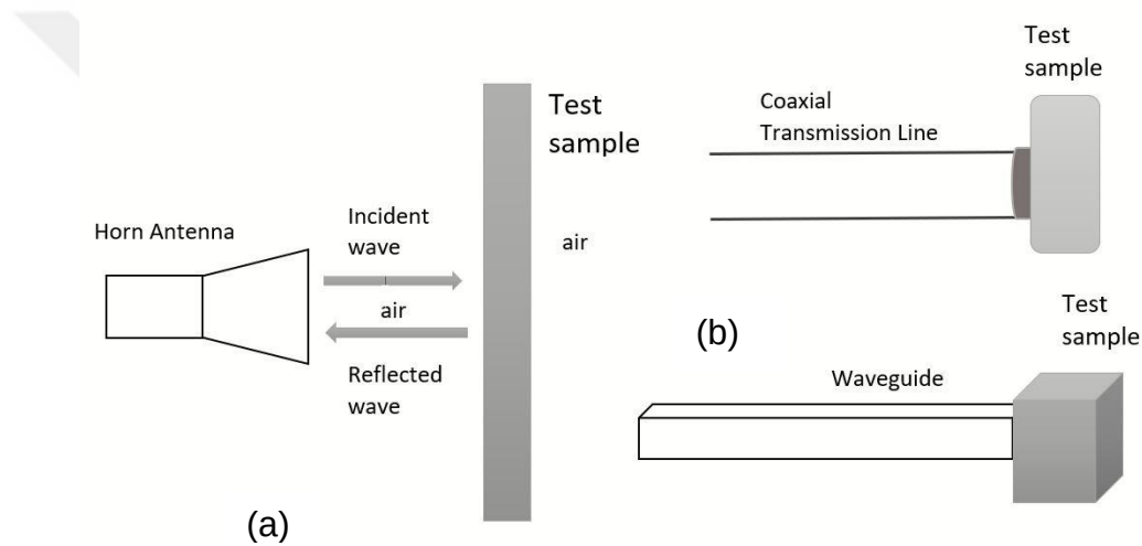
Figure 2.6. (a) Free Space open circuit reflection-only method. (b) Transmission line open circuit reflection-only method.
