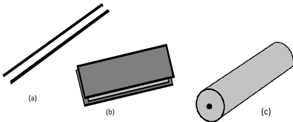
Figure 2.5. A transmission line with more than one conductor. (a) Parallel line, (b) parallel plate (c) coaxial transmission line.
