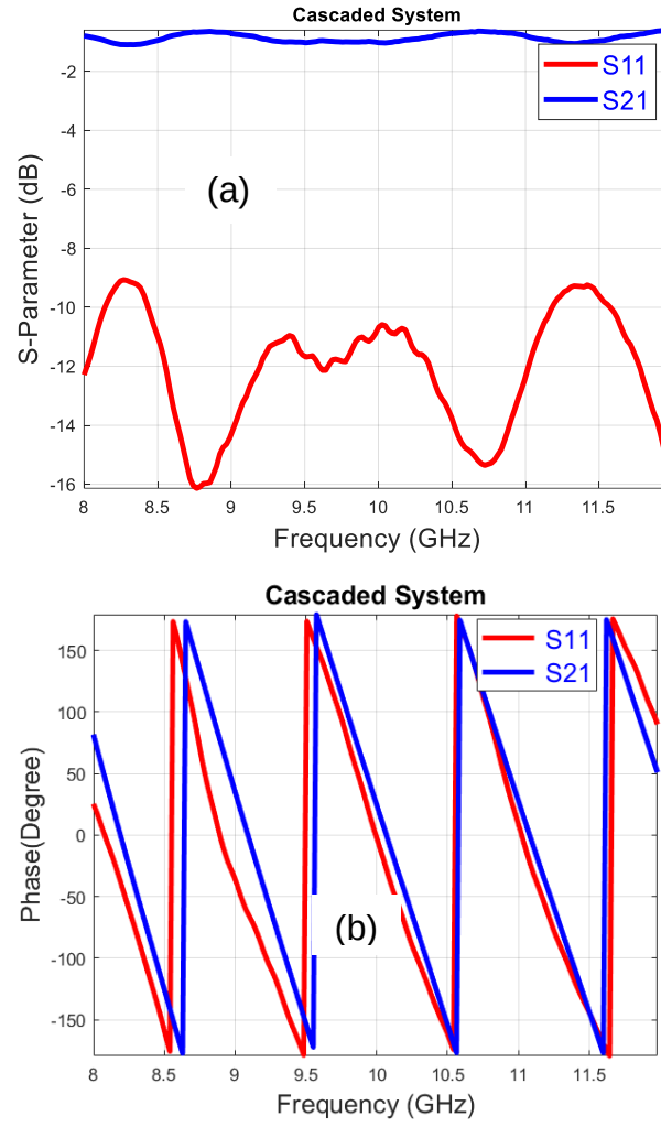
Figure 3.31. S-Parameters of cascaded system. (a) S-Parameters magnitude in dB. (b) Phase in degree.
