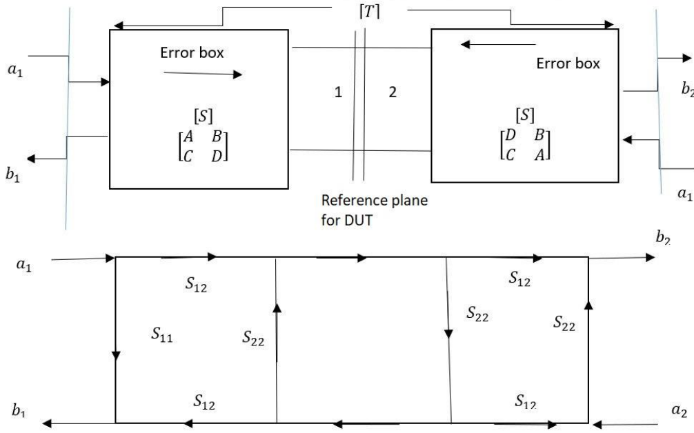
Figure 3.7. Block diagram and signal flow graph of Thru connection [25].
