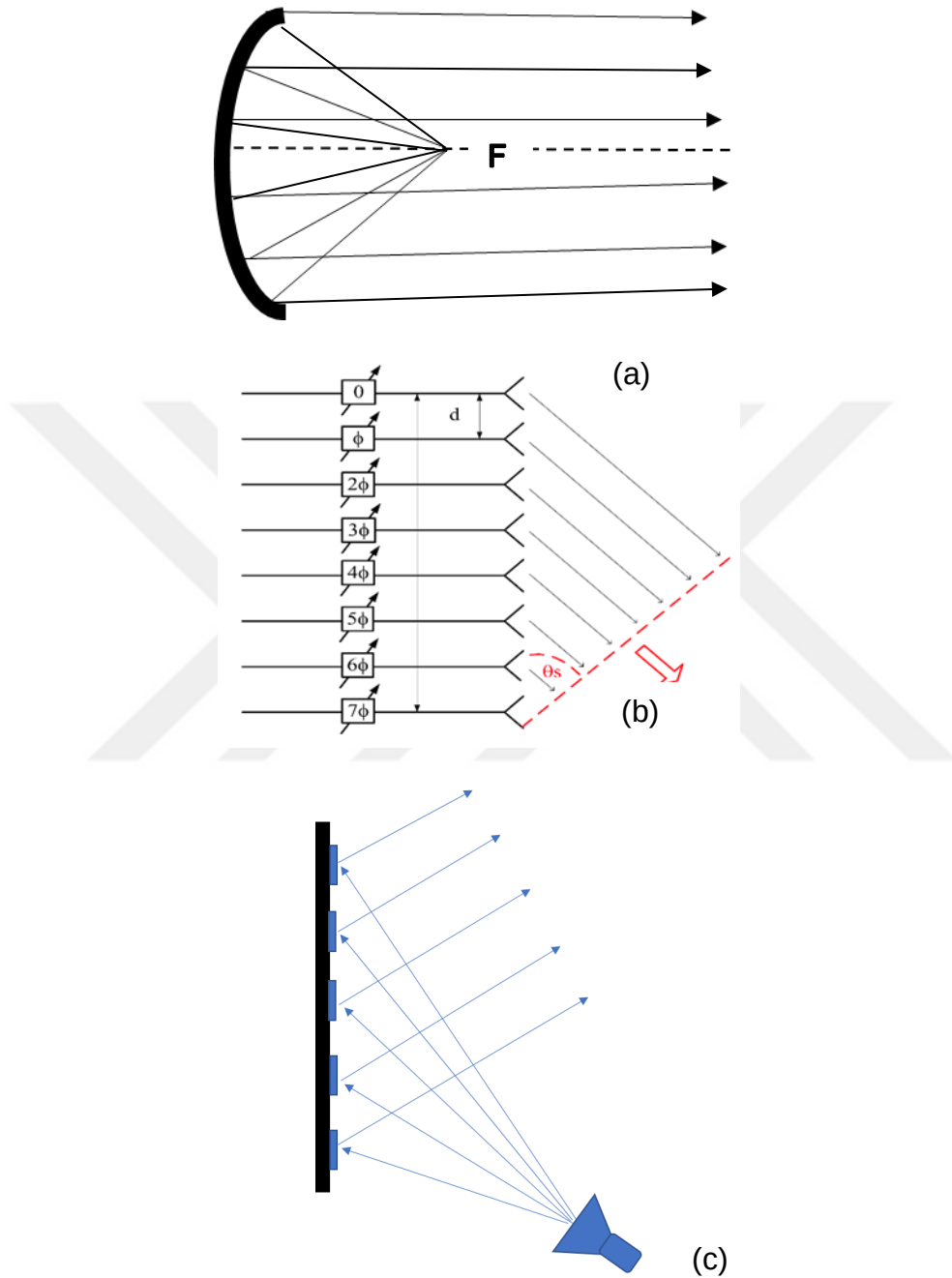
Figure 4.1. (a) Parabolic reflector. (b) Phased array antenna. (c) Reflectarray
