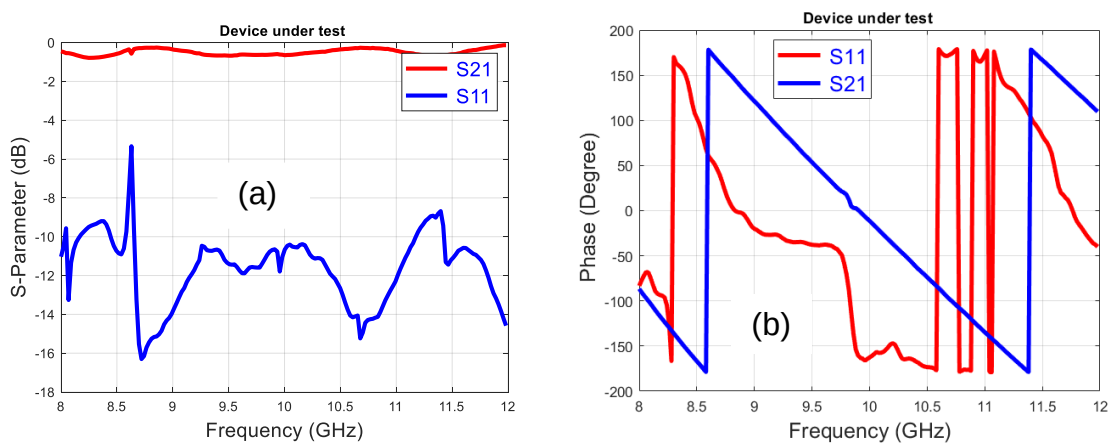
Figure 3.31. S-Parameters of cascaded system. (a) S-Parameters magnitude in dB. (b) Phase in degree.
