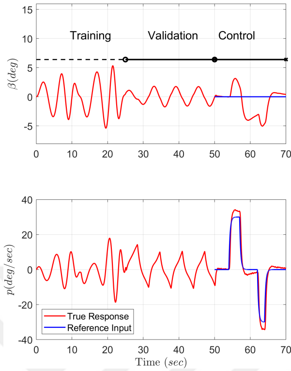
Figure 5.25: Output response for all stages for high noise
