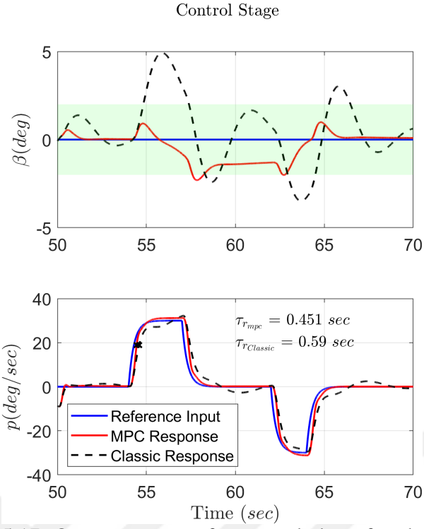
Figure 5.17: Output response for control phase for clean data
