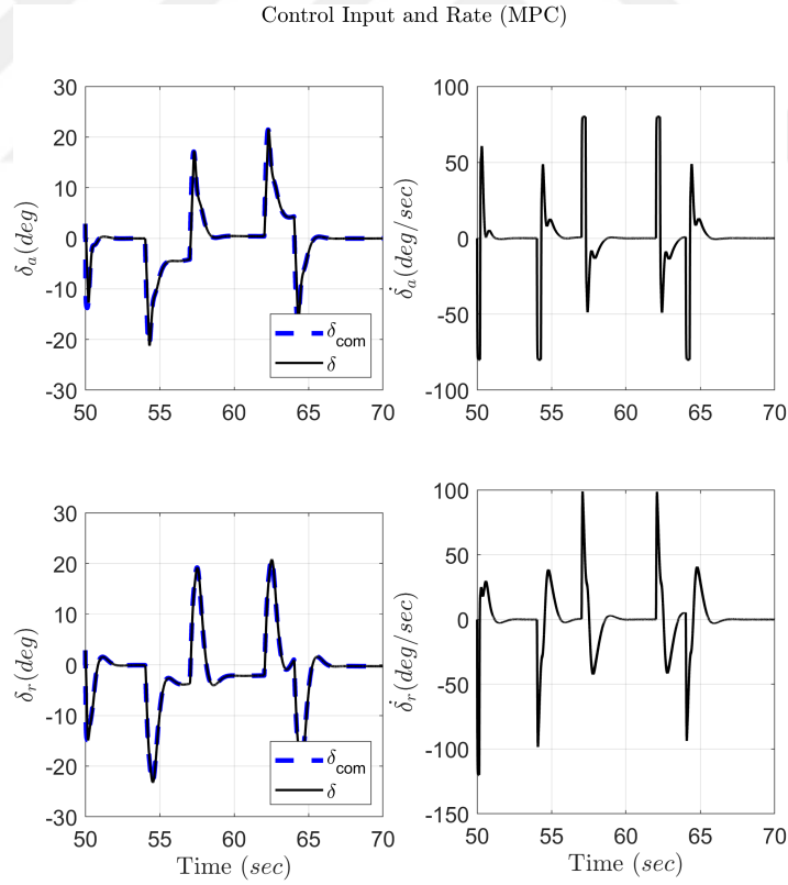
Figure 5.18: Actuator activity at control stage for MPC for clean data
