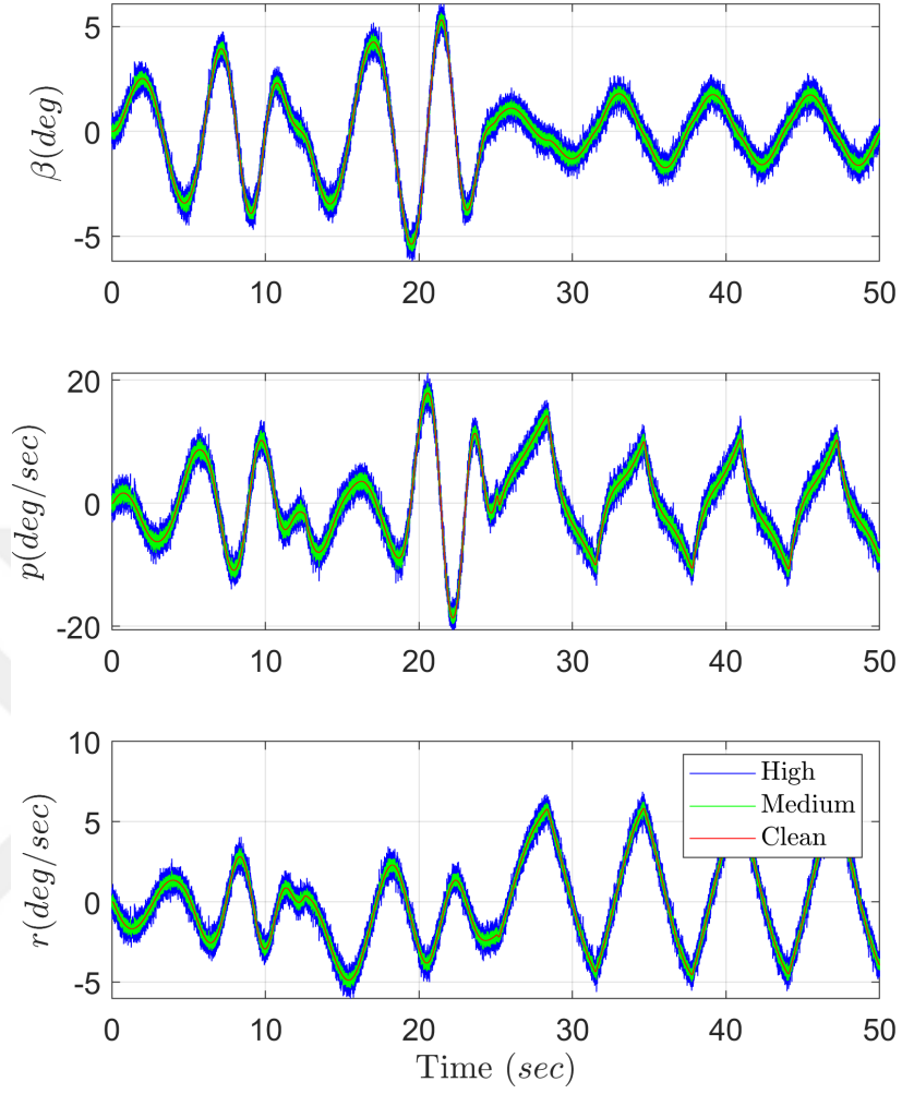
Figure 5.7: Noise Levels
