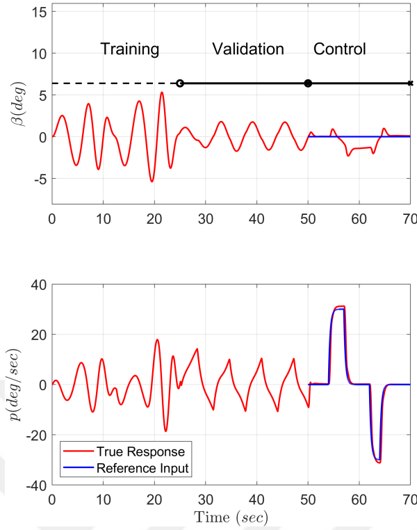
Figure 5.16: Output response for all phases for clean data
