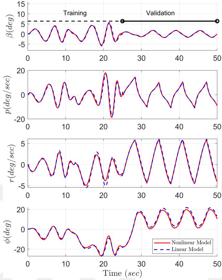
Figure 5.3: Linear vs Nonlinear Model
