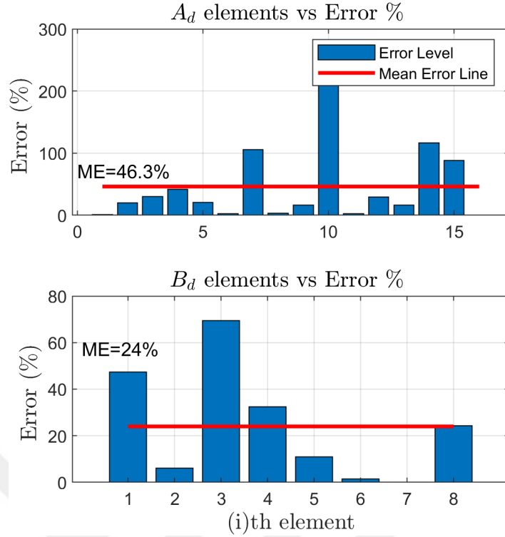
Figure 5.9: Error percentage for each matrix element for medium noise case
