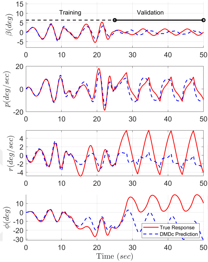
Figure 5.11: Training and validation results for high noise
