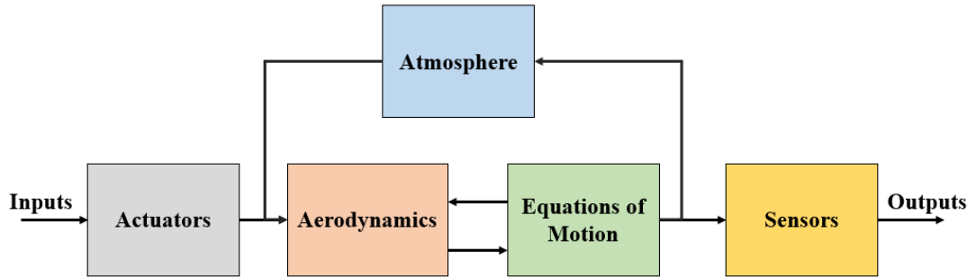
Figure 4.1: Fighter Aircraft Simulation Model
