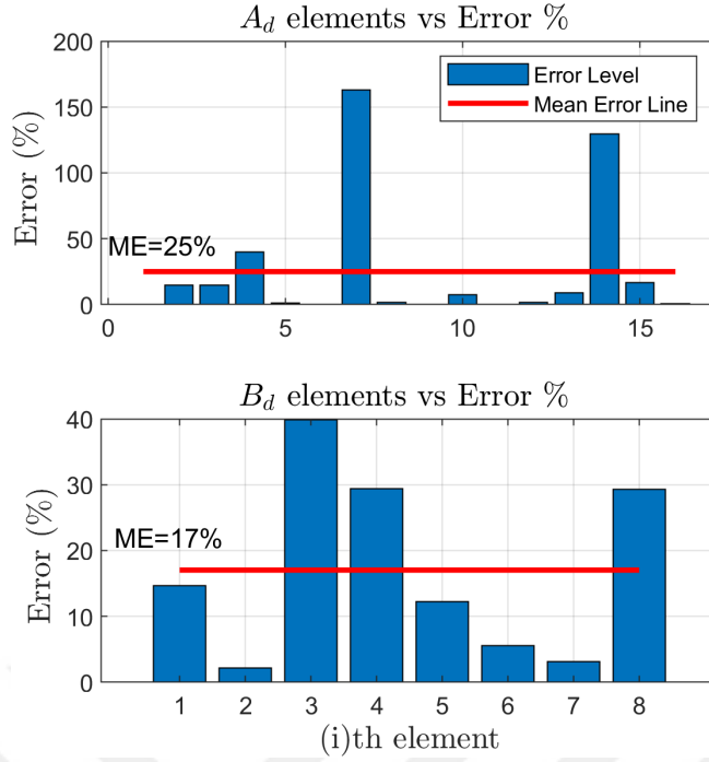
Figure 5.5: Error percentage for each matrix element in the clean data case
