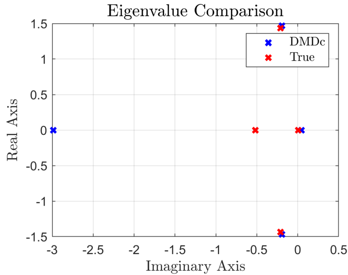
Figure 5.13: Eigenvalue comparison for high noise case
