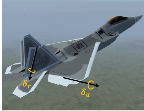
Figure 4.2: Control Surface Deflections
