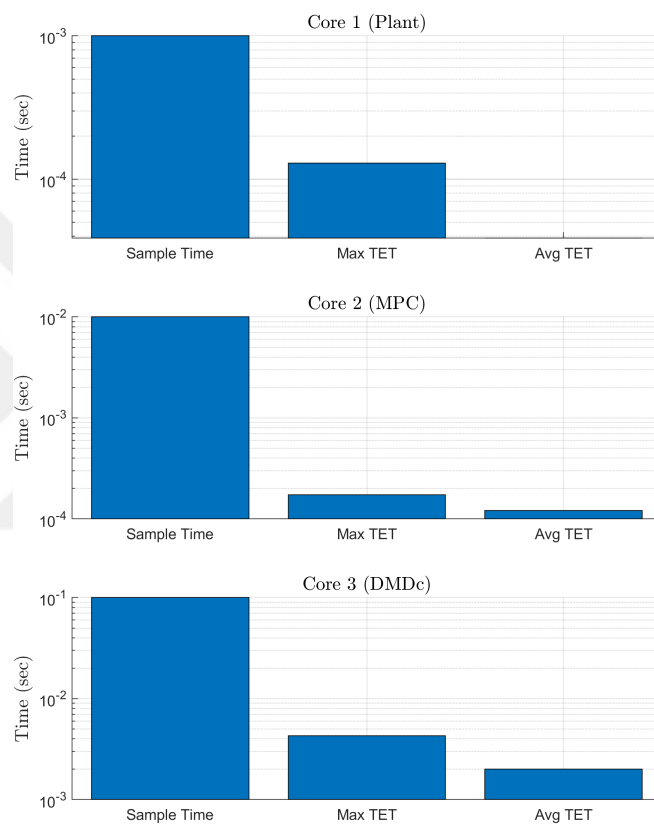
Figure 5.33: Summarized TET results
