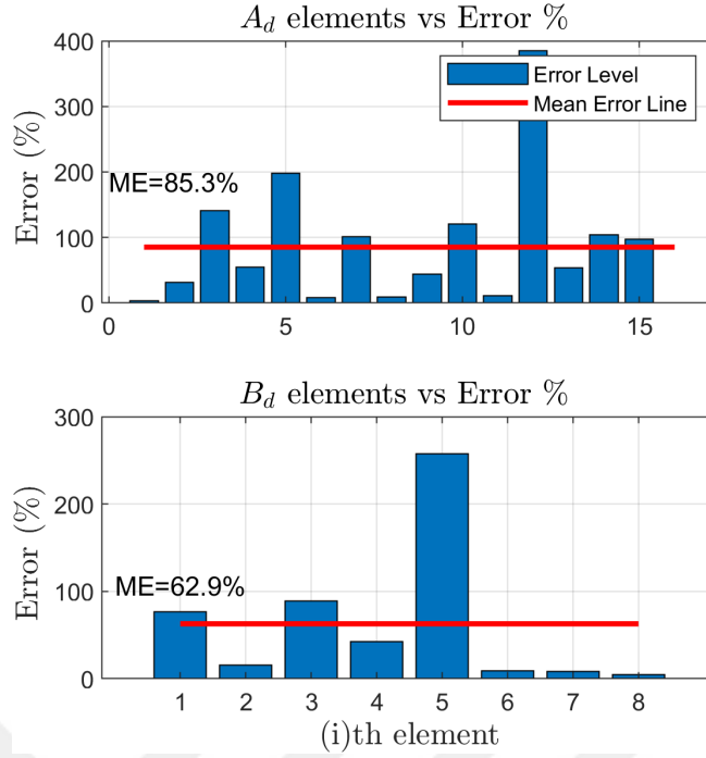
Figure 5.12: Error percentage for each matrix element for high noise case
