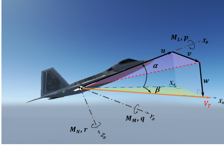
Figure 4.5: Aircraft reference frames
