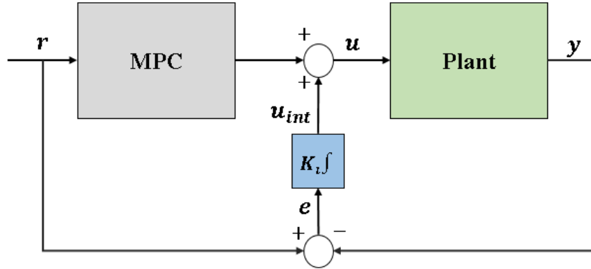
Figure 3.3: MPC with Integral Action
