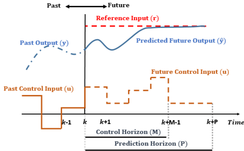
Figure 3.1: MPC Strategy
