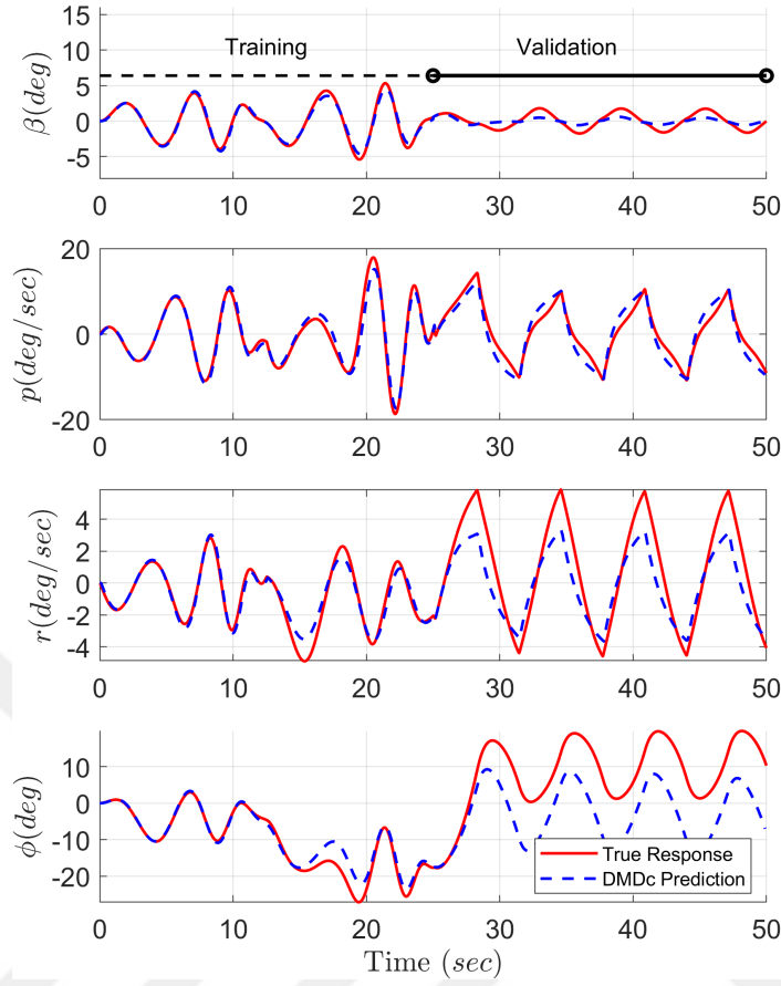
Figure 5.8: Training and validation results for medium noise
