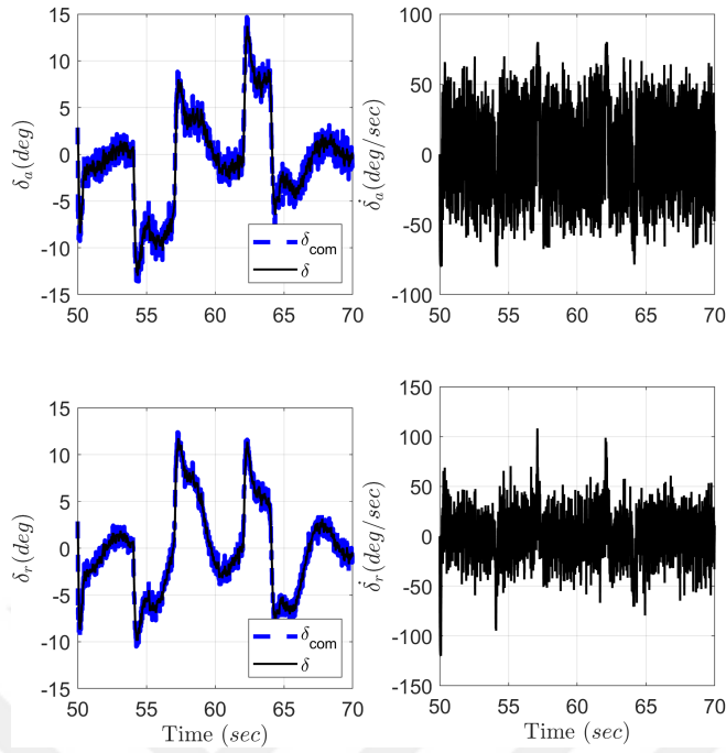
Figure 5.28: Actuator activity at control stage for classical controller for high noise
