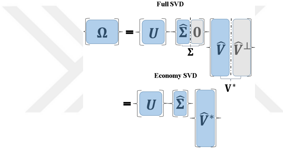
Figure 2.2: Schematic of matrices in the full and economy SVD
