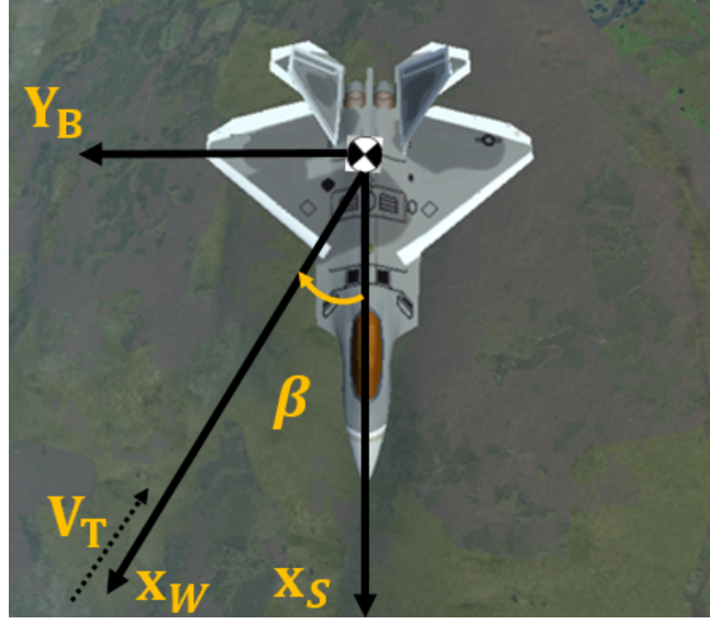
Figure 4.4: Stability frame and related angles
