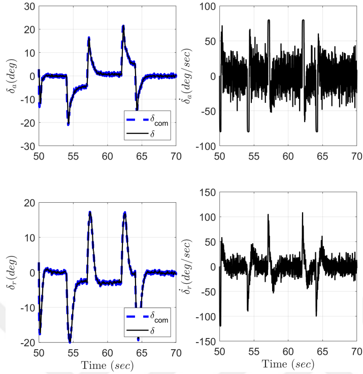
Figure 5.23: Actuator activity at control stage for MPC for medium noise
