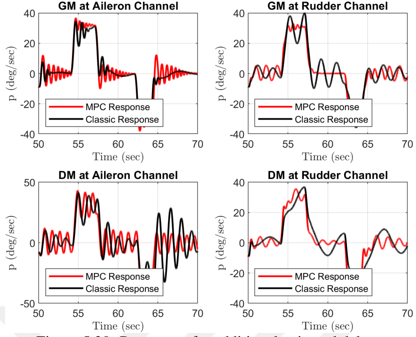
Figure 5.20: Responses for additional gain and delays
