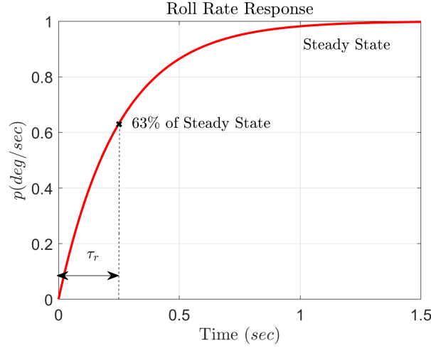
Figure 5.15: Roll mode time constant calculation
