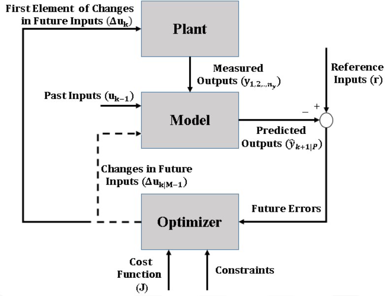
Figure 3.2: Basic Structure of MPC
