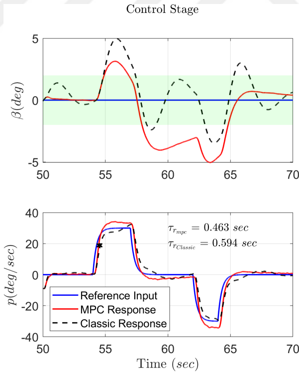
Figure 5.26: Output response for control stage high noise
