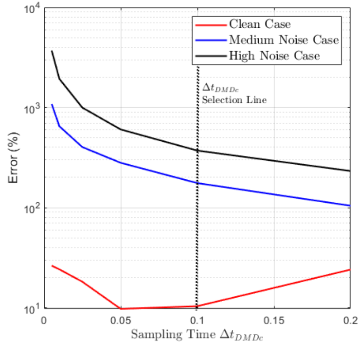
Figure A.1: MEE vs Sample rate \Delta_{DMDc}
