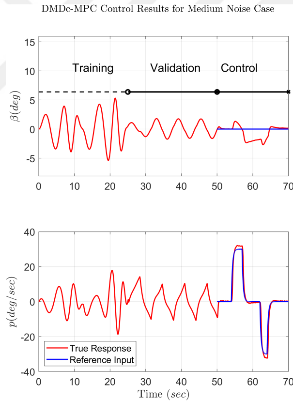
Figure 5.21: Output response for all Stages for medium noise
