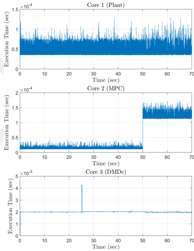
Figure 5.32: Target execution times for each cores during simulation
