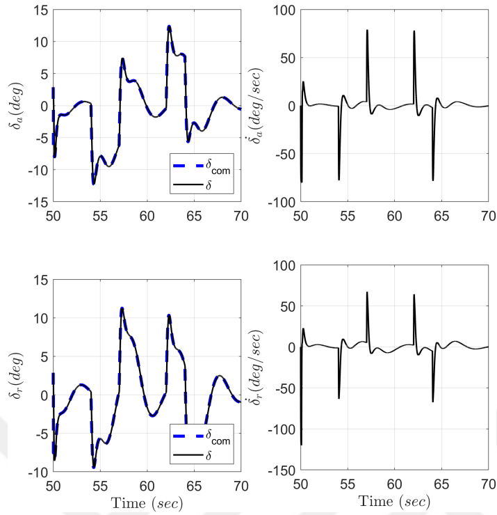
Figure 5.19: Actuator activity at control stage for Classic Controller for clean data
