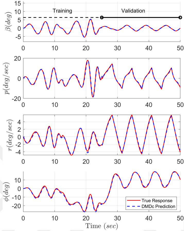
Figure 5.4: Training and validation results from clean data
