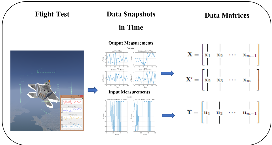
Figure 2.1: Data Collection process of DMDc
