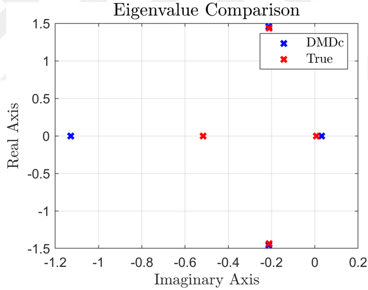
Figure 5.10: Eigenvalue comparison for medium noise case
