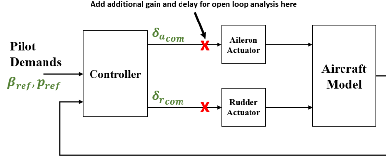
Figure 5.14: Closed loop system showing point for analysis
