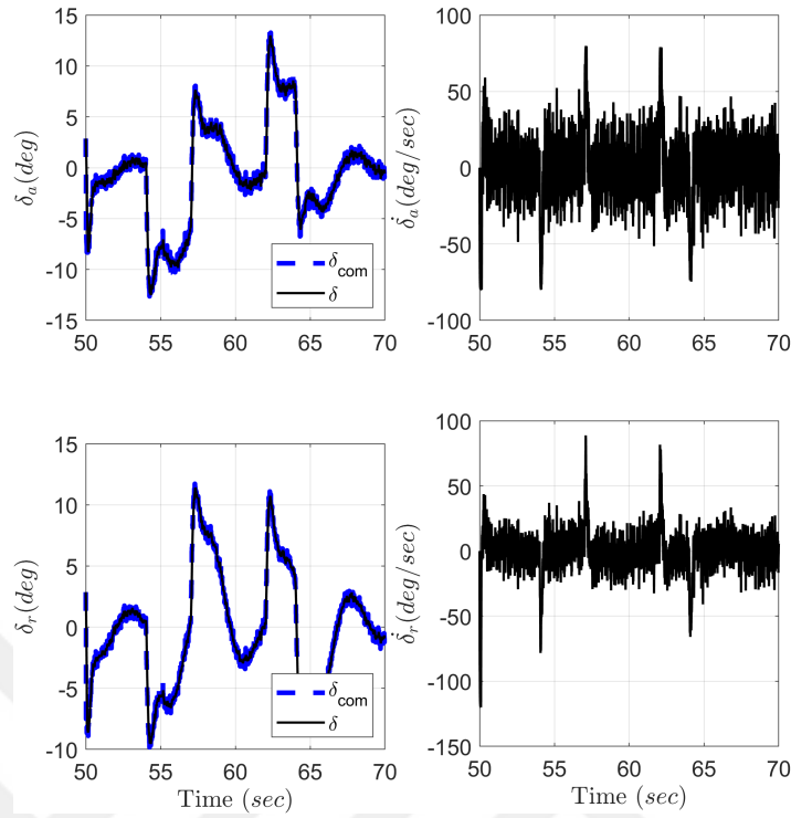
Figure 5.24: Actuator activity at control stage for classical controller for medium noise
