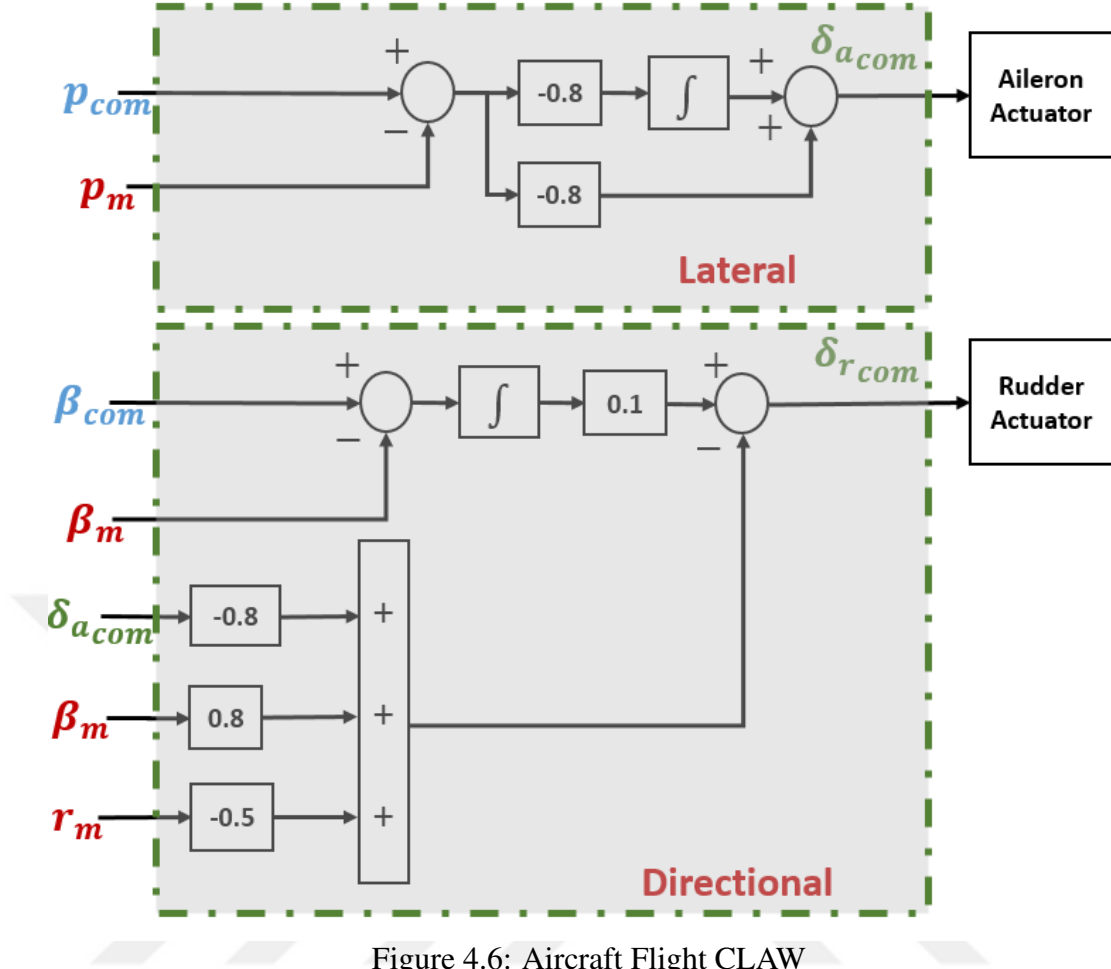
Figure 4.6: Aircraft Flight CLAW
