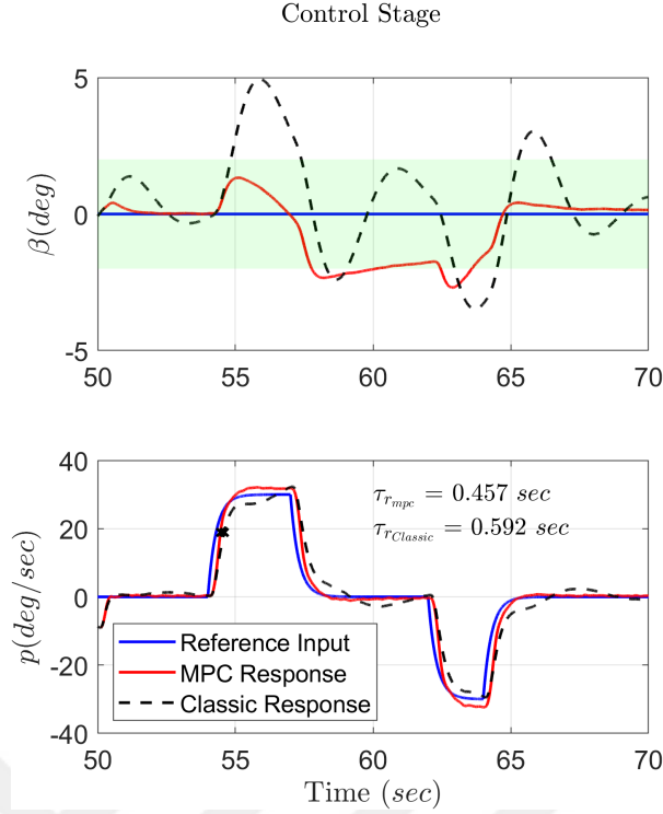
Figure 5.22: Output response for control stage for medium noise
