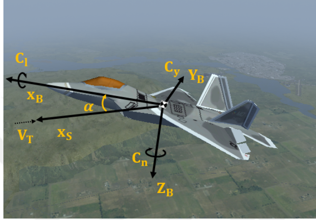
Figure 4.3: Body frame and aerodynamic coefficients
