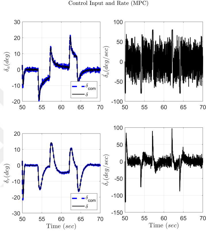
Figure 5.27: Actuator activity at control stage for MPC for high noise
