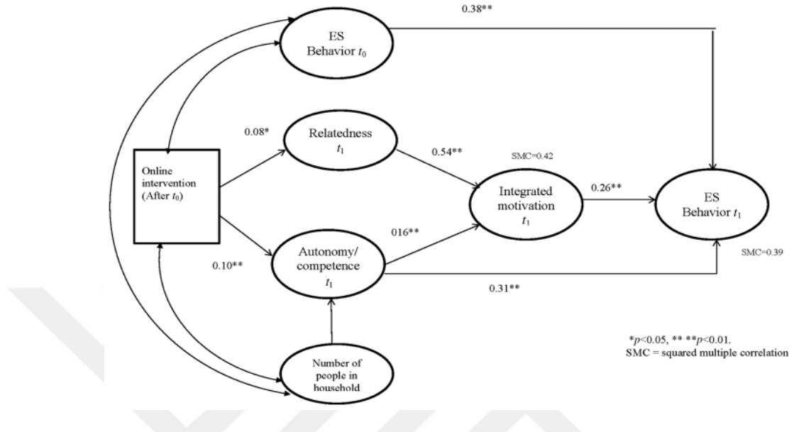
Figure 2.5 The path model proposed in Sweeney et al. (2014) and results obtained from that study
