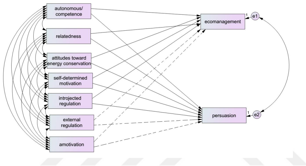
Figure 4.1 Improved path model to be tested
