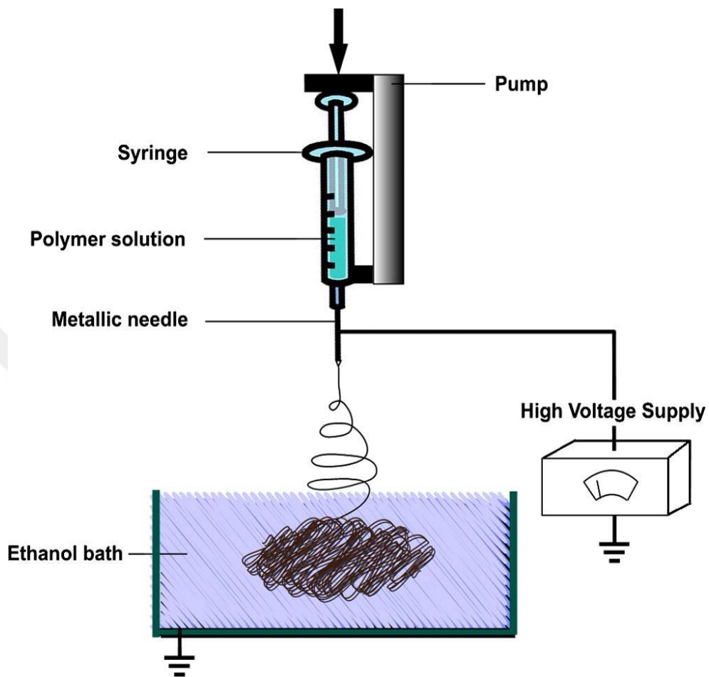
Fig. 1- 7 Scheme for wet electrospinning representing how the scaffold is in bulk formation (3-D) instead of a mate or a 2D membrane form obtained in conventional Electrospinning) (Yang et al., 2013)
