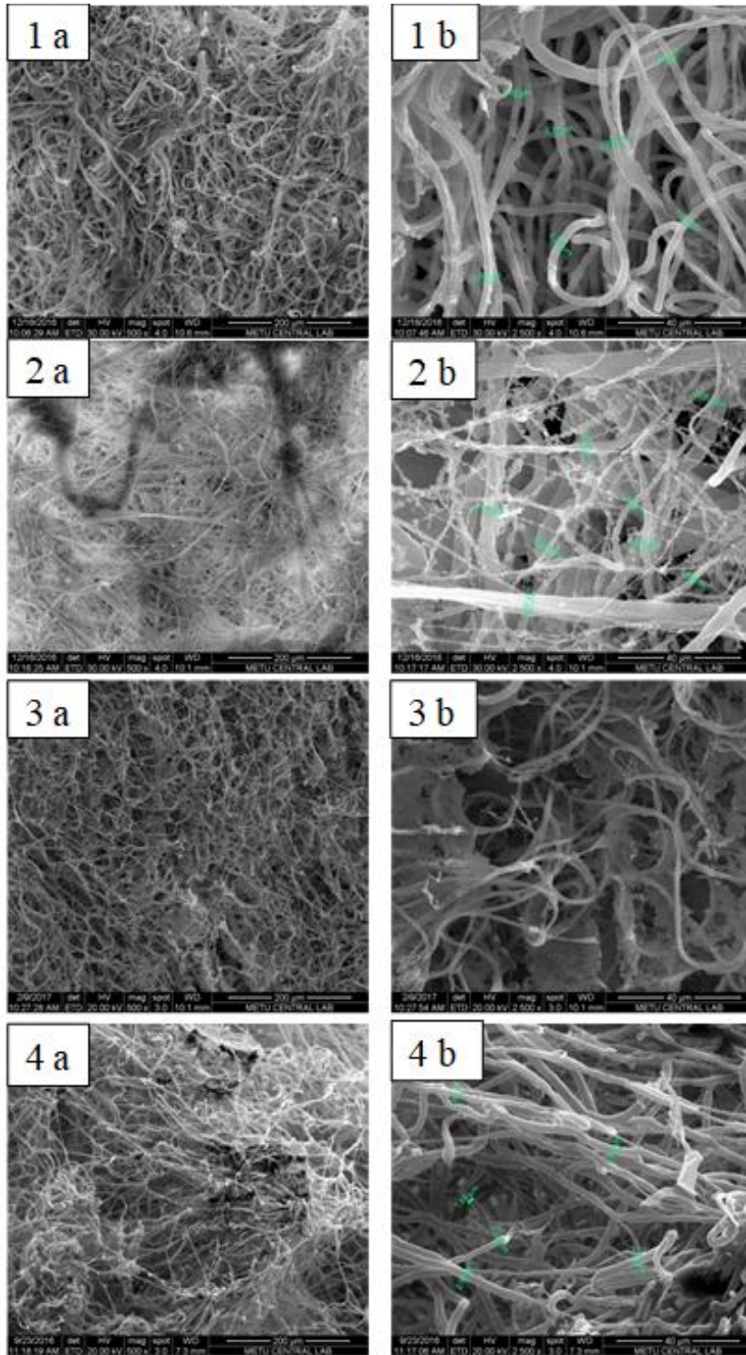
Fig. 3- 5 SEM images of electrospun scaffolds. Number codes on figures are corresponding to those given in Table3-2, a) 500x, b) 2500x magnification 1) Core: 5%PCL+: 5% P-188, Shell: 5%Gelatin +: 5% P-188, ethanol – 2) Core: 10% PCL, Shell: 10% Gelatin, ethanol; 3)Core: 10% PCL, Shell: 9%Gelatin +1% P-188, ethanol 4) Core: 10% Gelatin, Shell: 10% PCL, ethanol
