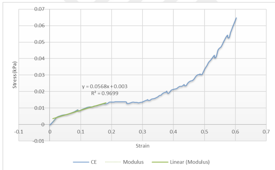
Fig. 3- 18 Stress-Strain Curve of representative for CE scaffold
