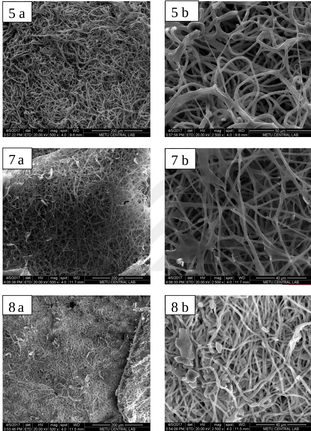
Fig. 3- 6 SEM images of electrospun scaffolds, Number codes on figures are corresponding to those given in Table3-2, a) 500x, b) 2500x magnification 5) Core: 10% PCL, Shell: 10% Gelatin, ethanol 7) Core: 5%Gelatin+: 5% P-188, Shell: 5%PCL +: 5% P-188, water8) Core: 10% PCL, Shell: 5% Gelatin + 5% P-188, water.
