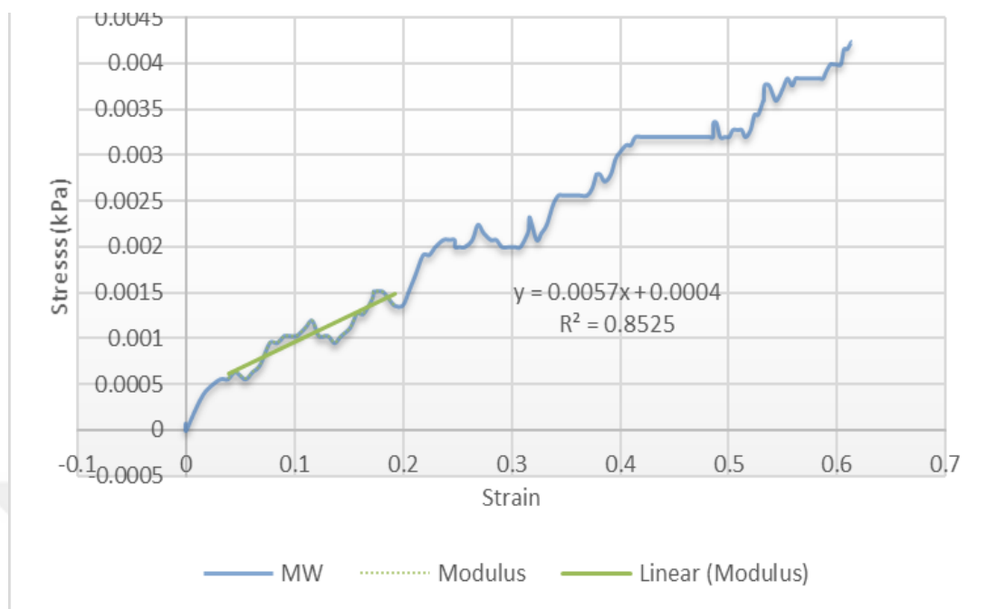
Fig. 3- 15 Stress-Strain Curve of representative for MW scaffold
