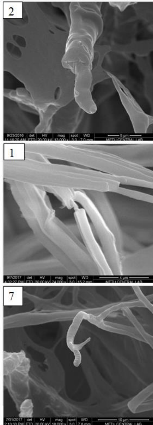
Fig. 3- 7 Structure of coaxial electrospun nanofibers taken by SEM of samples exposed by freeze fracturing with liquid nitrogen showing both the core and shell of electrospun fiber. Number codes on figures are corresponding to those given in Table 3-2.
