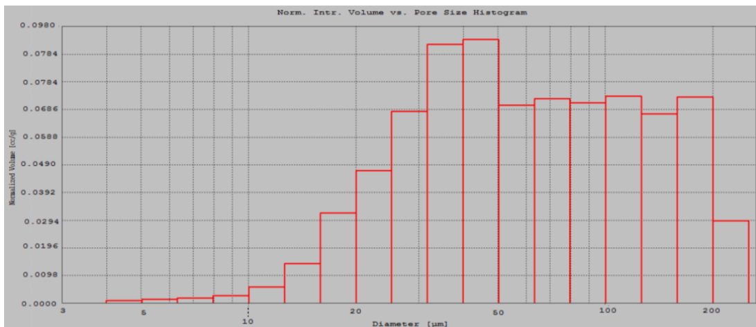
Fig. 3- 10 Pore size distribution of MW scaffolds
