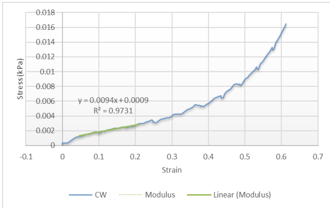
Fig. 3- 17 Stress-Strain Curve of representative for CW scaffold
