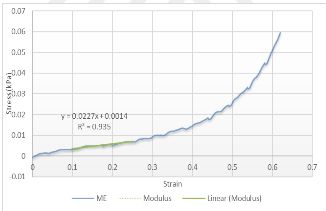
Fig. 3- 16 Stress-Strain Curve of representative for ME scaffold
