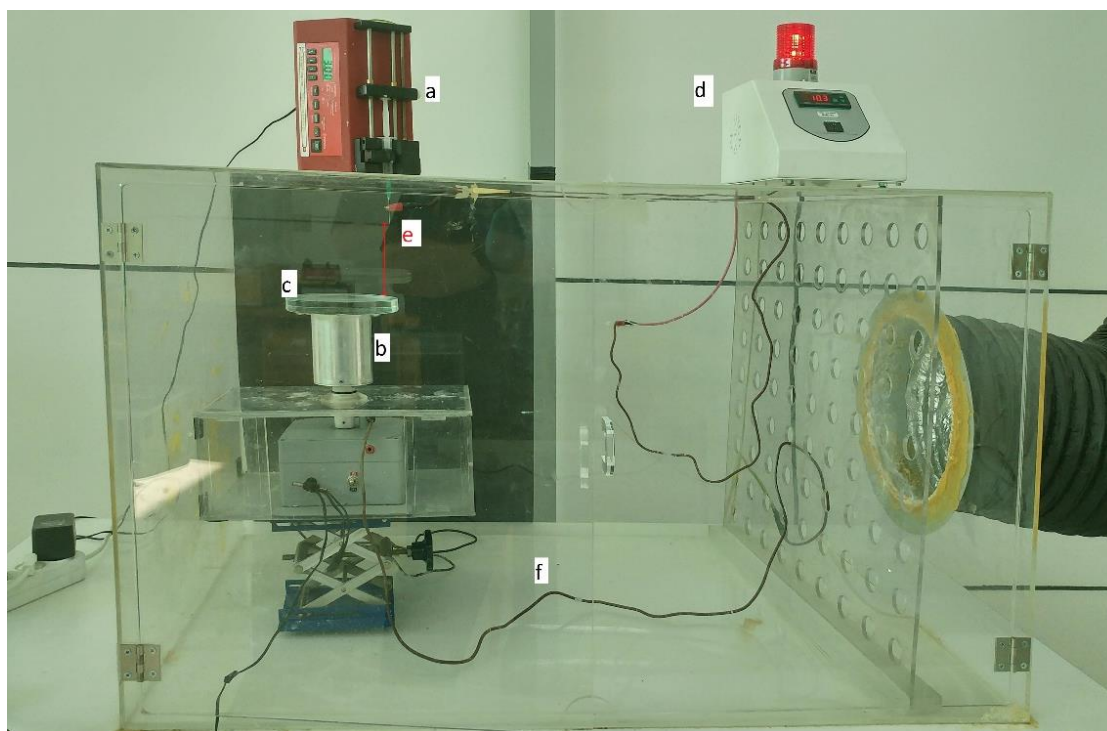
Fig. 2- 1 The setup for electrospinning a) NE-1000 syringe pump b) Rotational collector stand c) Glass dish contain the collector solvent d) High voltage source e) Distance between needle tip and collector f) cable connecting the stand to the ground
