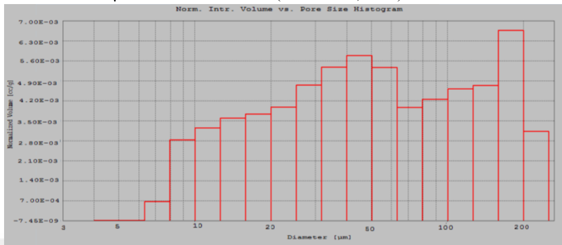
Fig. 3- 11 Pore size distribution of CW scaffolds
