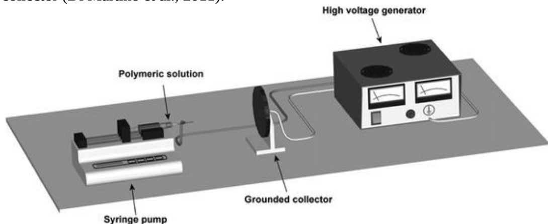
Fig. 1- 6 Schematic representation of an electrospinning setup (Di Martino et al., 2011)
