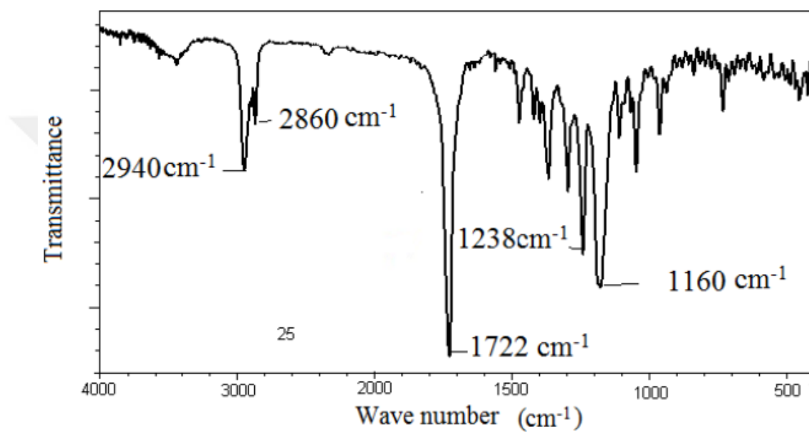
Fig. C – 1 FTIR Spectra of PCL compound (Abderrahim et al., 2015)
