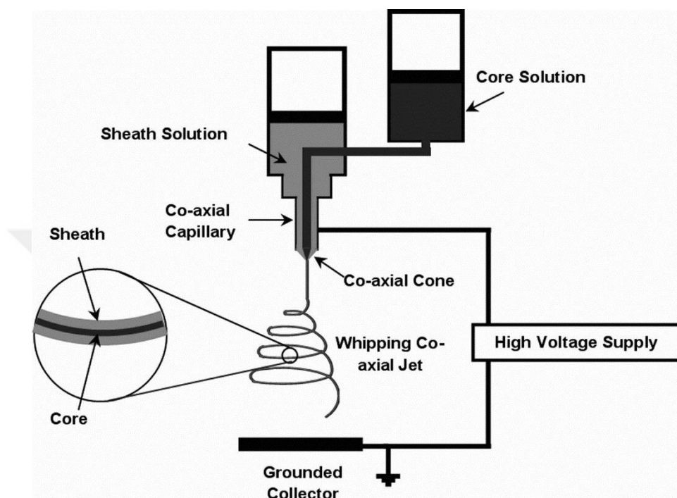
Fig. 1- 8 Schematic showing the coaxial electrospinning setup (Moghe & Gupta, 2008)
