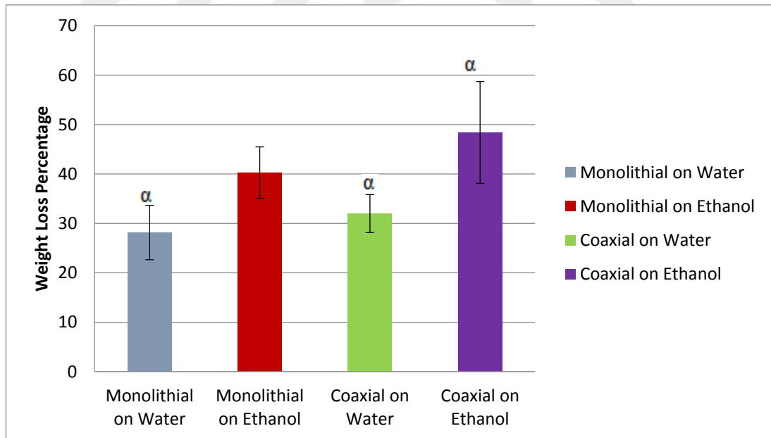
Fig. 3- 8- Degradation percentage of scaffolds after being submitted in PBS (0.1 M, pH 7.4) inside a water bath at 37°C for 10 days (n=3). \alpha : statistically significant difference between degradation of CE and degradation of MW or CW
