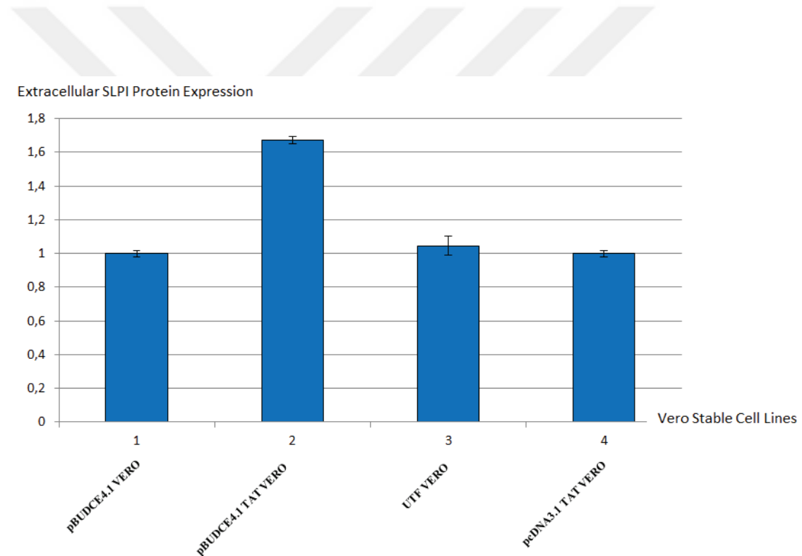
Figure 3.26. Extracellular SLPI Expression Analysis with Sandwich ELISA.
