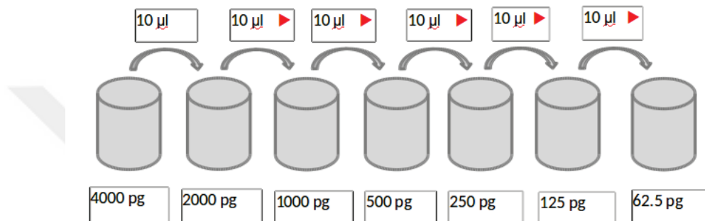
Figure 2.7. Serial Dilutions for Elisa standard
