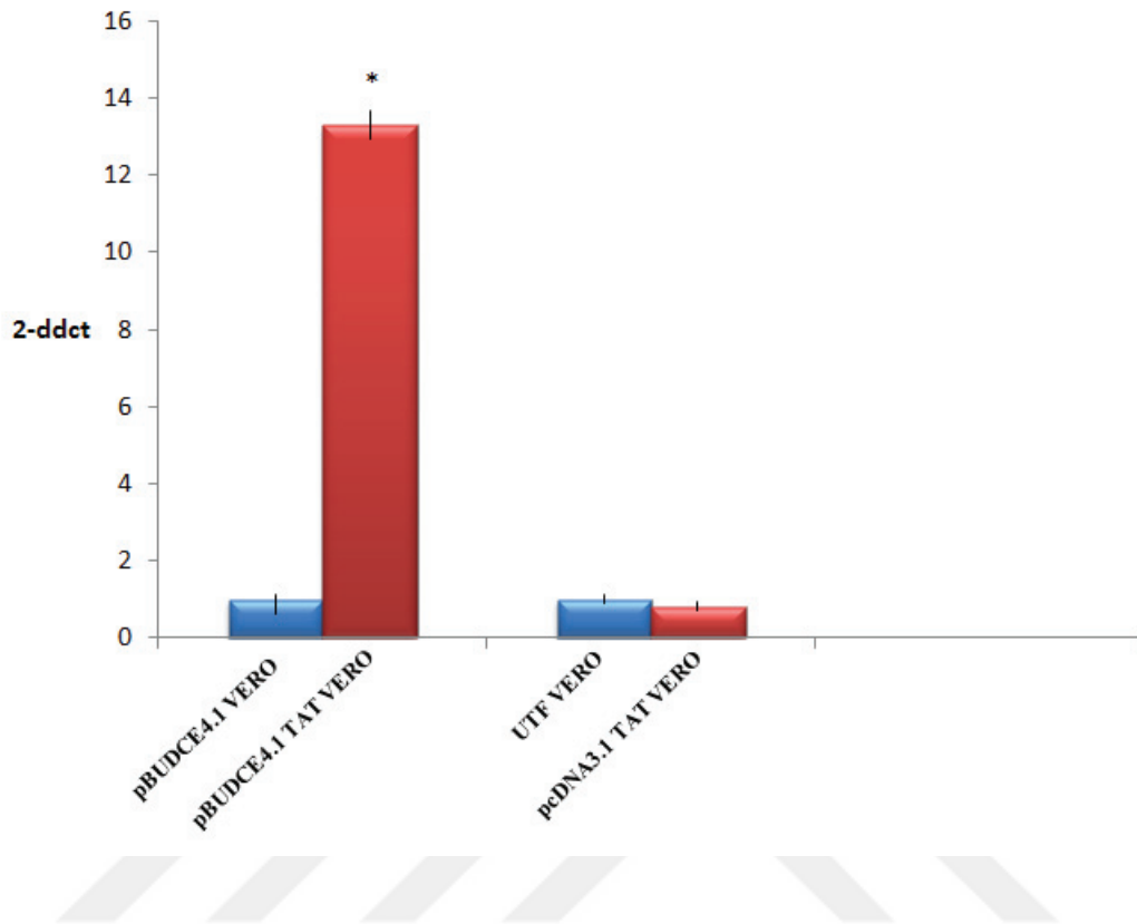
Figure 3.18. SLPI expression of generated stable Vero Cell Lines.
