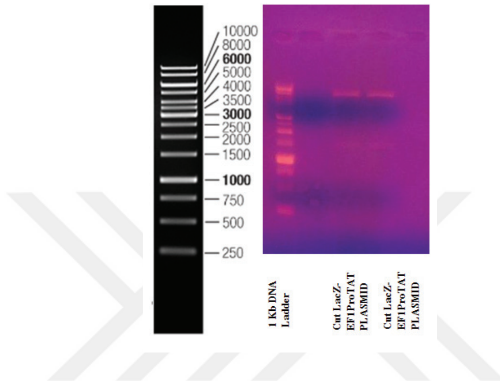
Figure 3.10. Agarose Gel Analysis of LacZ-Ef1ProTAT
