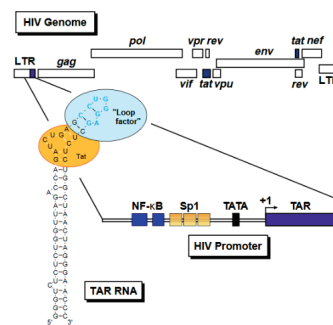
Figure 1.1. Genome Structure of HIV (Source: Karn, 2000)
