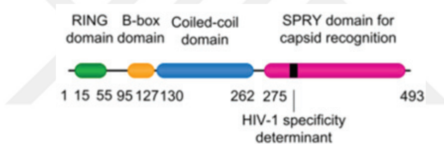
Figure 1.7. Structure of TRIM5 \alpha (Source: Blanco-Melo et al., 2012)
