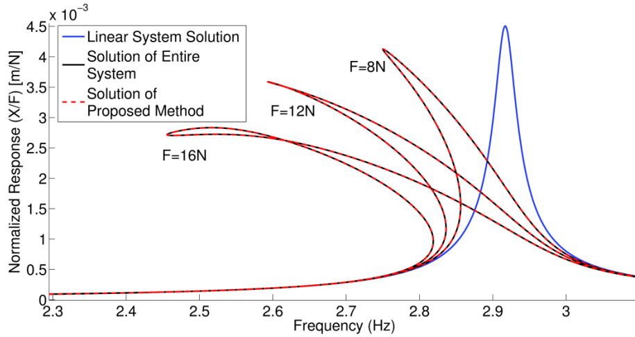
Figure 4.4 Normalized response of the 8 th DOF in case study 1
