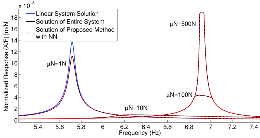
Figure 4.15 (a) Normalized response of the 2 nd DOF in case study 4
