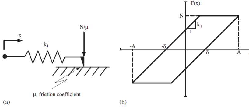
Figure 2.3 (a) Schematic drawing, (b) corresponding hysteresis curve for dry friction nonlinearity [28]
