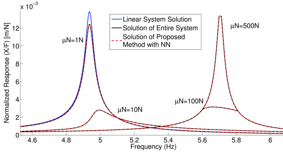
Figure 4.32 (a) Normalized response of the 1 st DOF in case study 9
