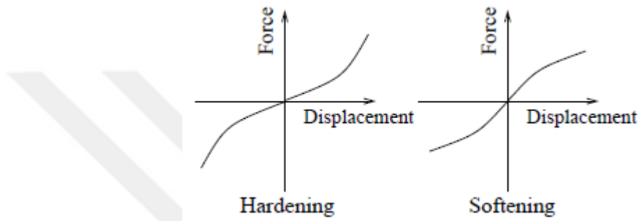
Figure 2.2 Characteristic of hardening and softening cubic stiffness elements [27]
