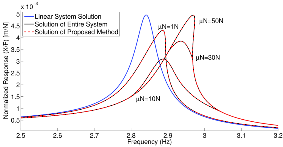
Figure 4.11 Normalized response of the 1 st DOF in case study 3
