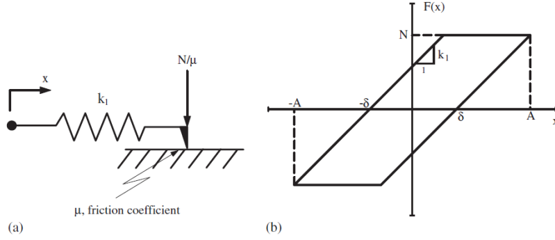
Fig. 3 (a) Schematic drawing, (b) corresponding hysteresis curve for dry friction nonlinearity [22] Describing function of the hysteresis curve given in Fig. 3(a) can be written as [22, 24]
