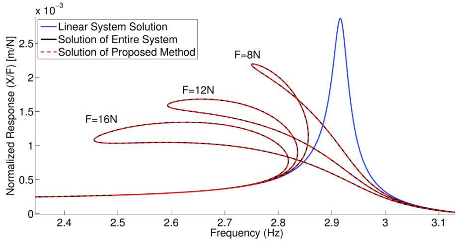
Figure 4.2 Normalized response of the 1 st DOF in case study 1
