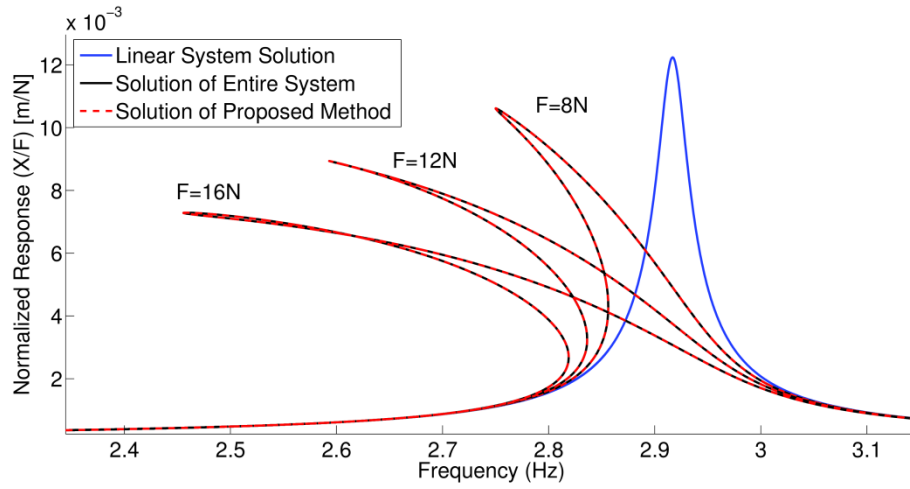
Figure 4.3 Normalized response of the 3 rd DOF in case study 1
