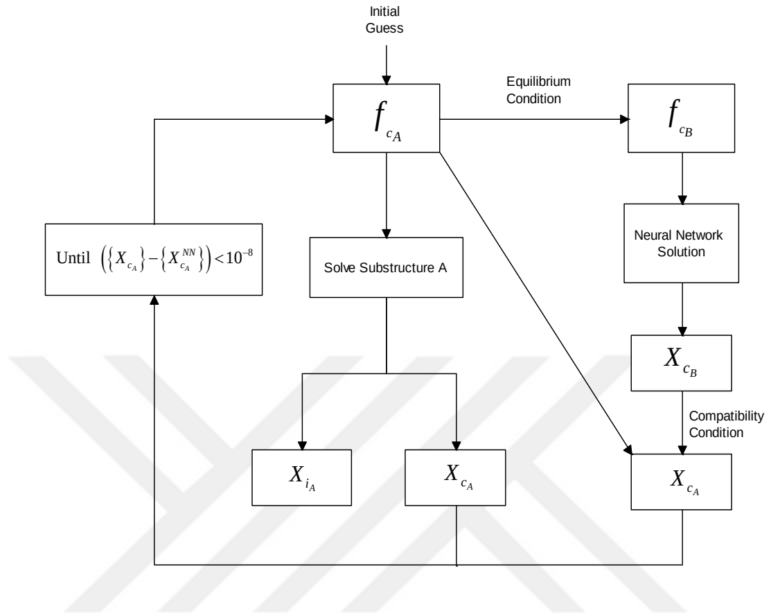
Figure 3.6 Nonlinear Structural Coupling Algorithm using Artificial Neural Networks
