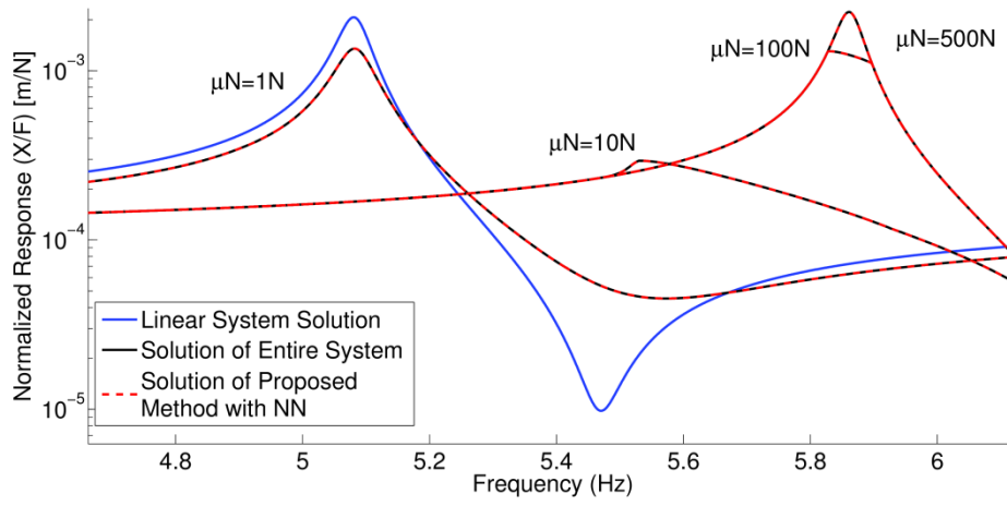
Figure 4.19 (b) Normalized response of the 1 st DOF in case study 5
