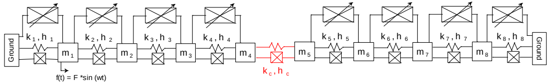
Figure 4.1 Schematic view of 8-DOF coupled system
