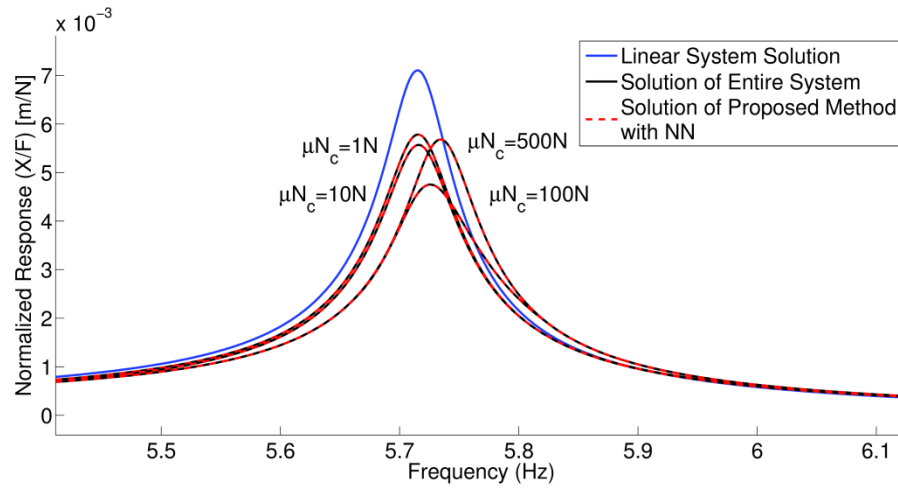
Figure 4.16 Normalized response of the 1 st DOF in case study 4
