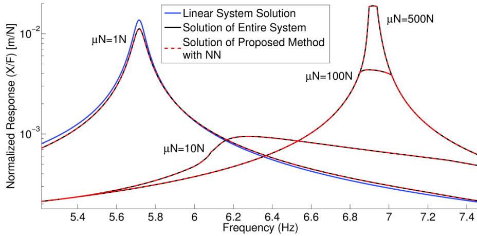
Figure 4.15 (b) Normalized response of the 2 nd DOF in case study 4
