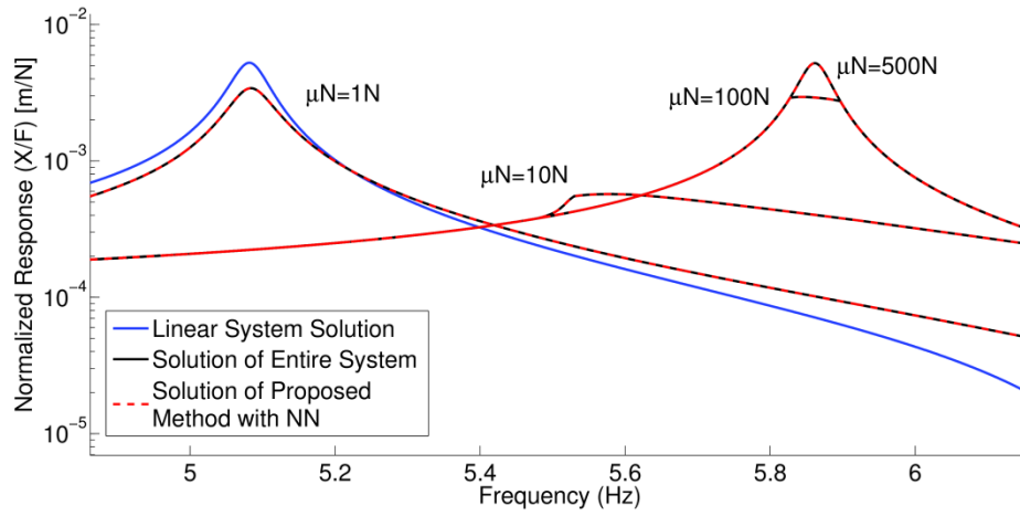
Figure 4.20 (b) Normalized response of the 2 nd DOF in case study 5
