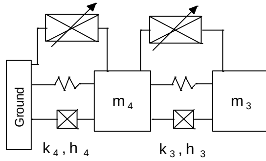
Figure 4.31 Schematic view of neural network trained substructure
