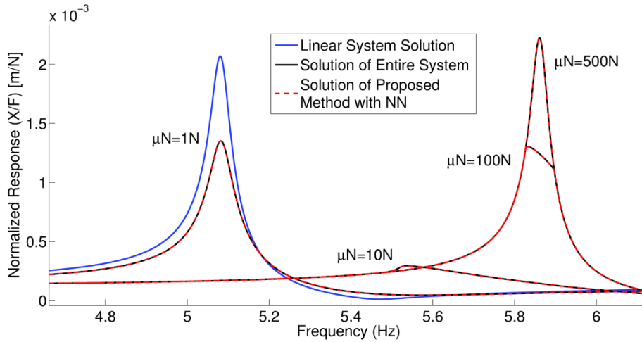
Figure 4.19 (a) Normalized response of the 1 st DOF in case study 5
