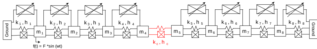
Fig. 4 Schematic view of 8-DOF coupled system
