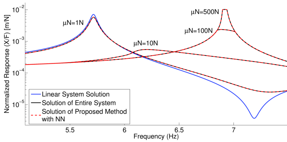
Figure 4.14 (b) Normalized response of the 1 st DOF in case study 4
