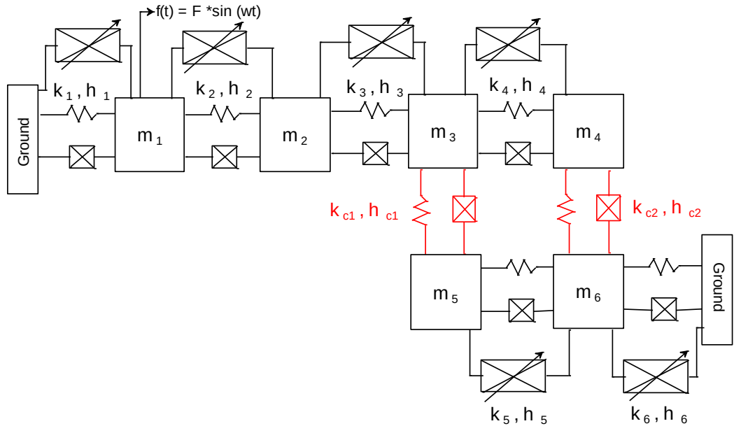
Figure 4.27 Schematic view of 4-DOF coupled system
