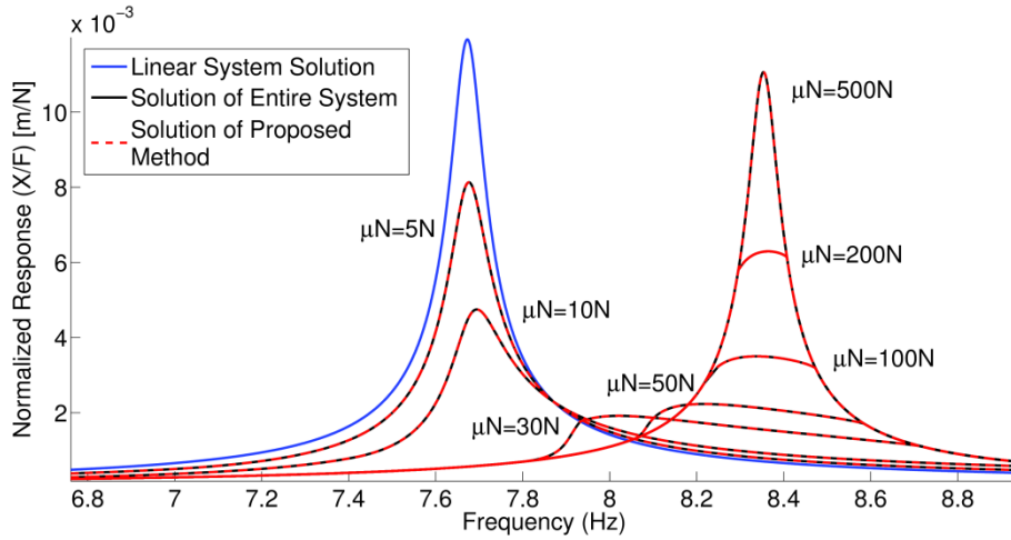
Figure 4.8 Normalized response of the 3 rd DOF in case study 2
