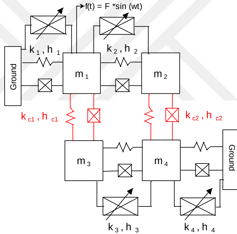
Figure 4.25 Schematic view of 4-DOF coupled system
