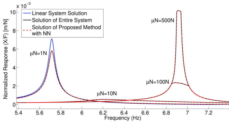
Figure 4.14 (a) Normalized response of the 1 st DOF in case study 4
