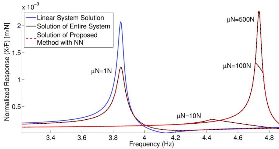
Figure 4.22 (a) Normalized response of the 1 st DOF in case study 6
