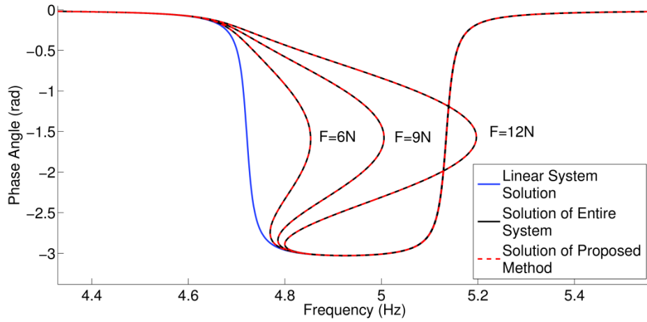
Figure 4.29 Phase angle of the 1 th DOF in case study 8
