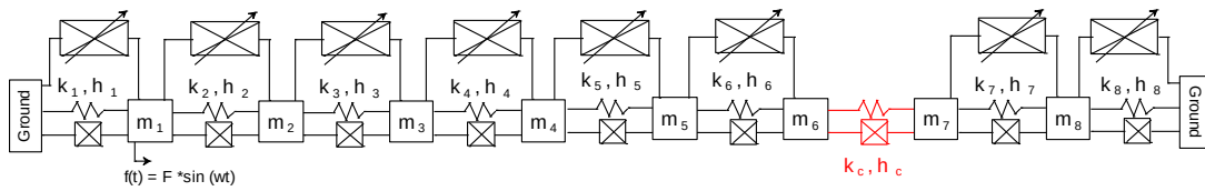
Figure 4.9 Schematic view of 8-DOF coupled sytem
