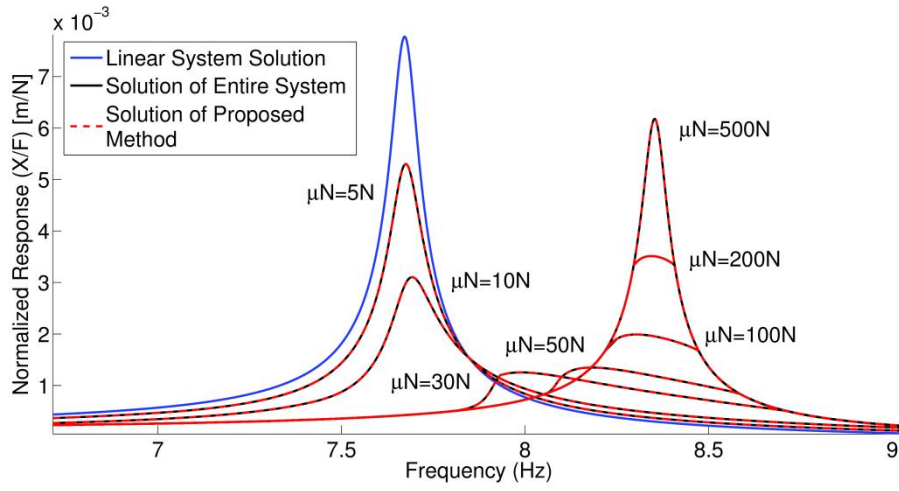
Figure 4.7 Normalized response of the 1 st DOF in case study 2
