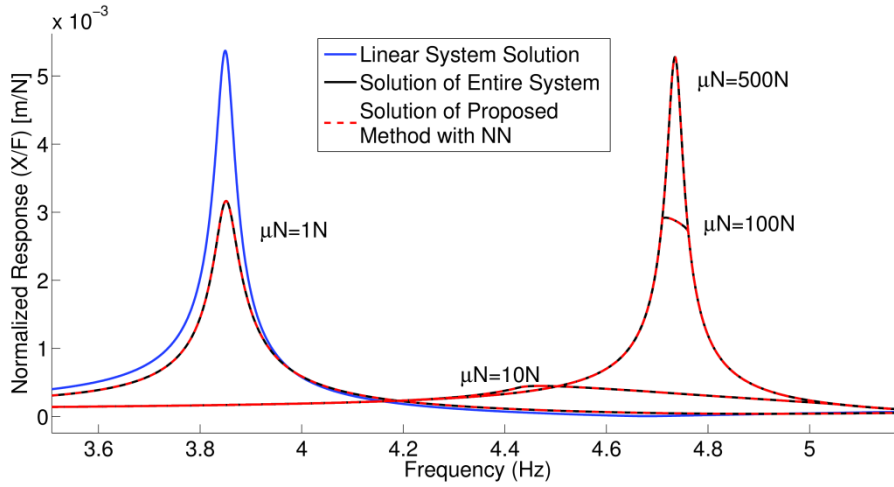
Figure 4.23 (a) Normalized response of the 2 nd DOF in case study 6
