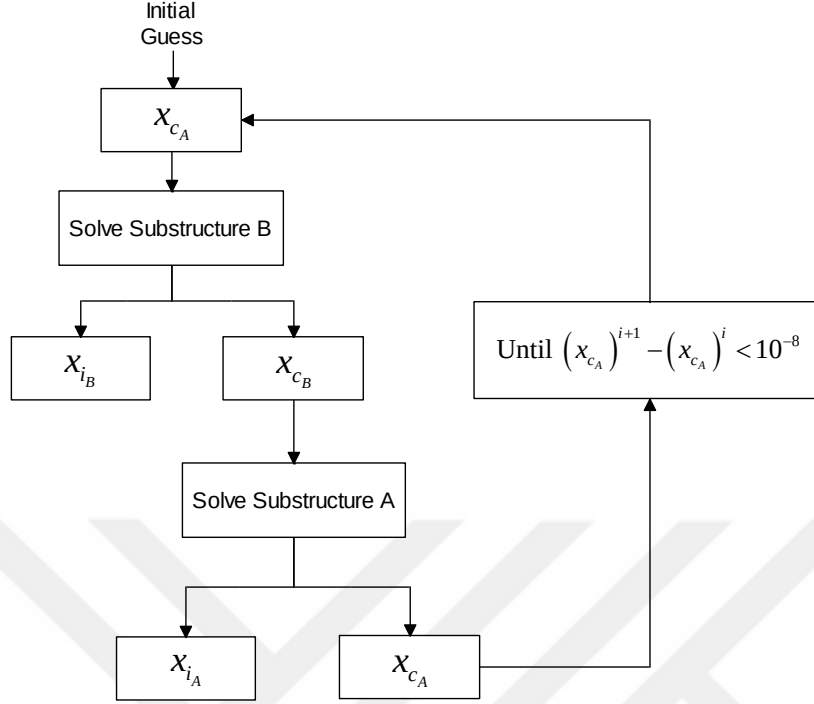
Fig. 2 Algorithm of the proposed method
