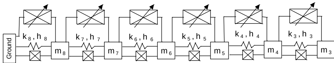
Figure 4.21 Schematic view of neural network trained substructure
