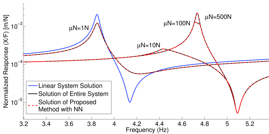
Figure 4.22 (b) Normalized response of the 1 st DOF in case study 6
