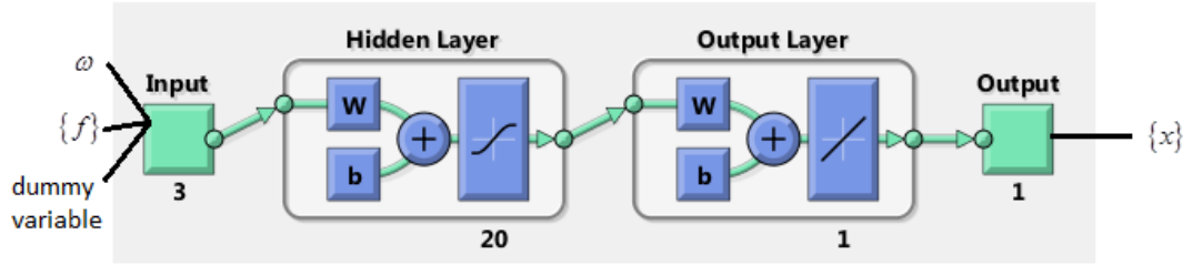
Figure 3.5 Classification of neural network with dummy variable [36]
