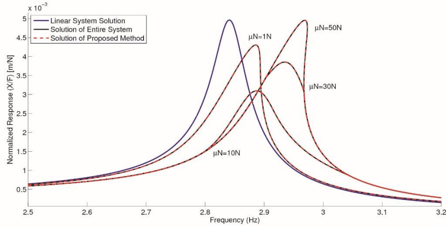
Fig. 9 Normalized response of the 1 th DOF in case study 2
