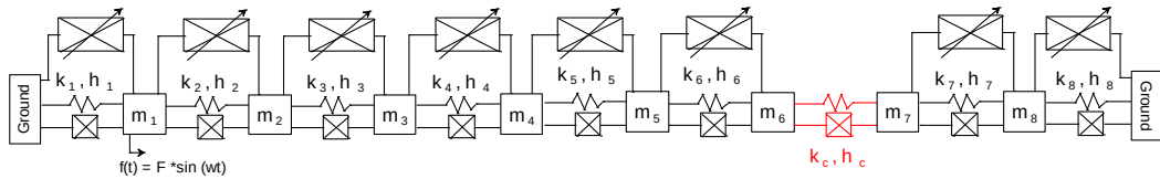
Fig. 7 Schematic view of 8-DOF coupled system
