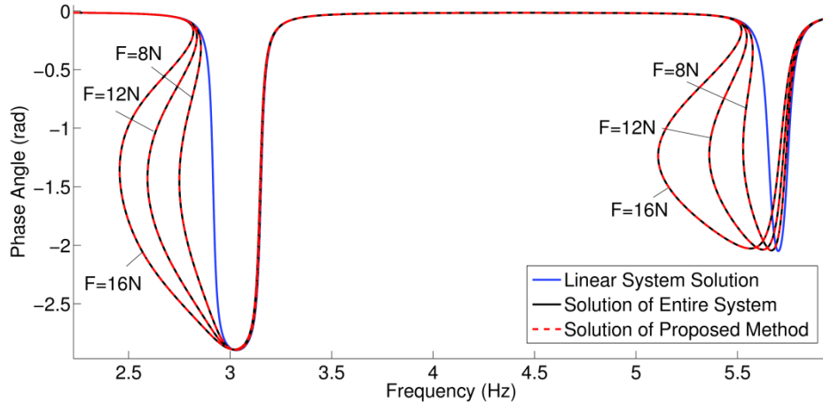
Figure 4.5 Phase angle of the 1 th DOF in case study 1
