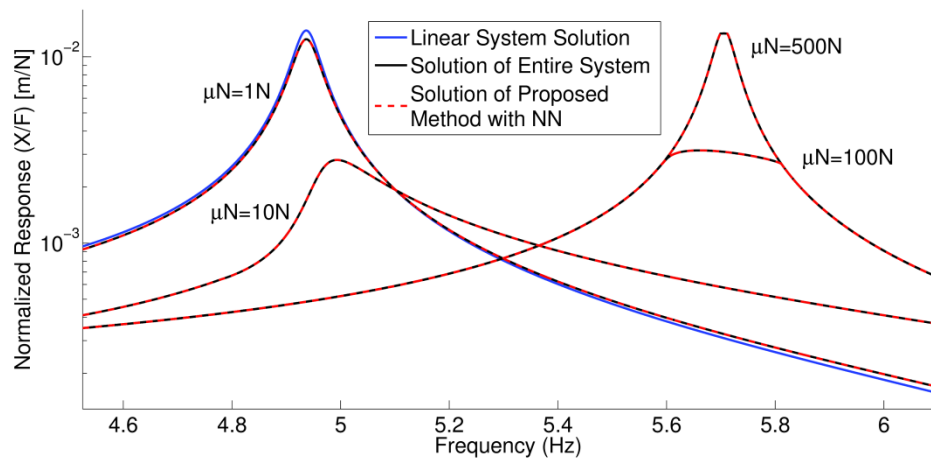
Figure 4.32 (b) Normalized response of the 1 st DOF in case study 9
