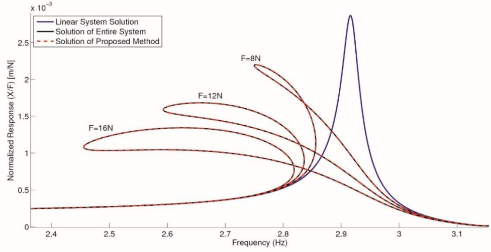
Fig. 5 Normalized response of the 1 st DOF in case study 1
