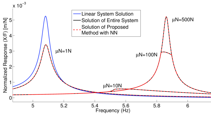
Figure 4.20 (a) Normalized response of the 2 nd DOF in case study 5
