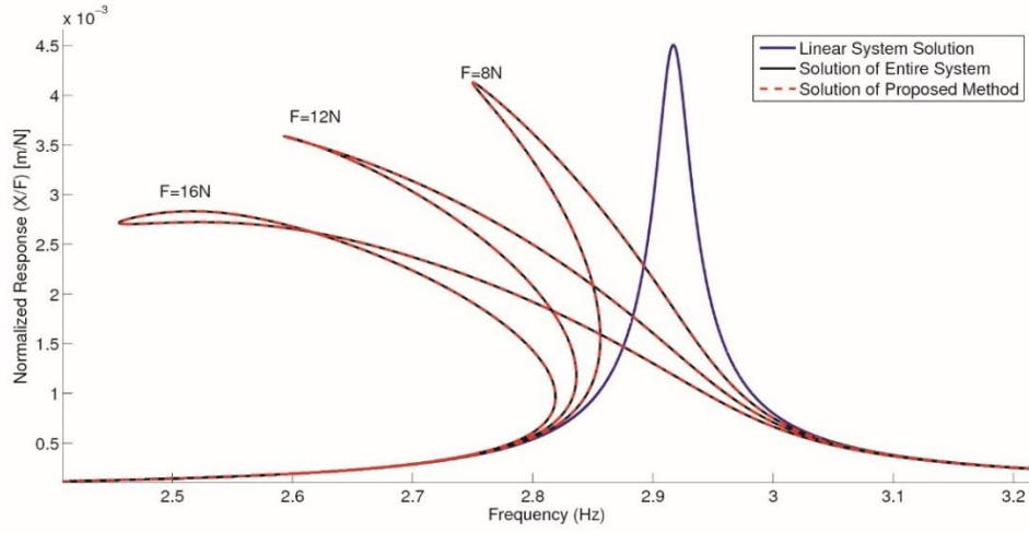
Fig. 6 Normalized response of the 8 th DOF in case study 1
