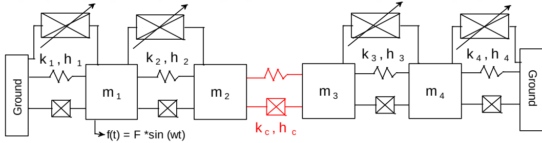
Figure 4.6 Schematic view of 4-DOF coupled system
