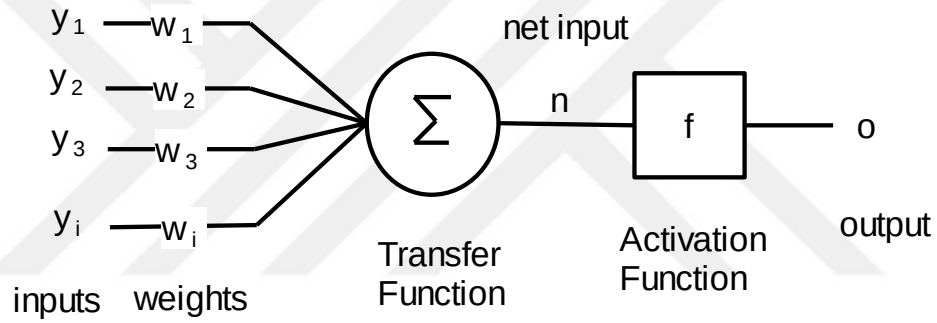
Figure 3.2 Simple neuron model
