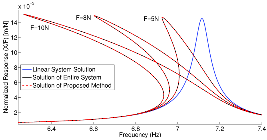
Figure 4.26 Normalized response of the 1 st DOF in case study 7
