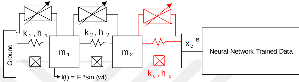
Figure 4.12 Schematic view of 4-DOF coupled system
