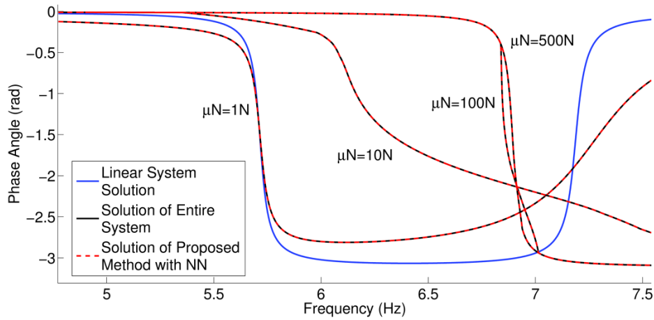
Figure 4.17 Phase angle of the 1 th DOF in case study 4
