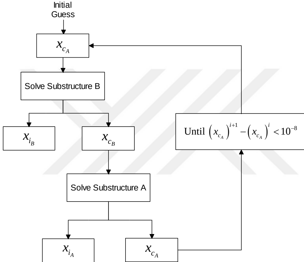
Figure 3.1 Nonlinear Structural Coupling Algorithm
