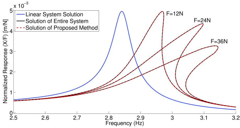
Figure 4.10 Normalized response of the 1 st DOF in case study 3
