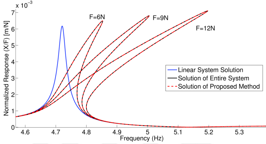
Figure 4.28 Normalized response of the 1 st DOF in case study 8
