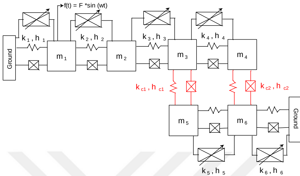
Fig. 10 Schematic view of 6-DOF coupled system
