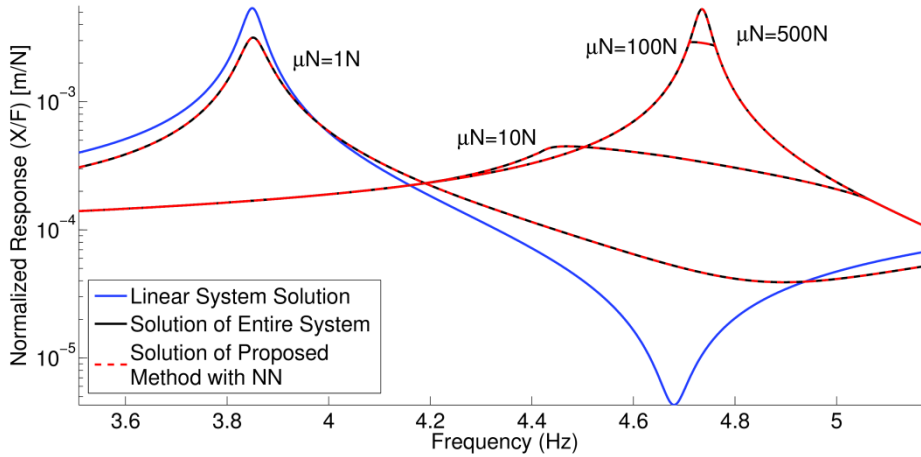
Figure 4.23 (b) Normalized response of the 2 nd DOF in case study 6
