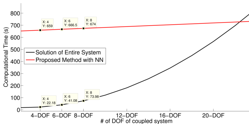
Figure 4.24 Comparison of computational time between proposed method with neural networks and entire system solution
