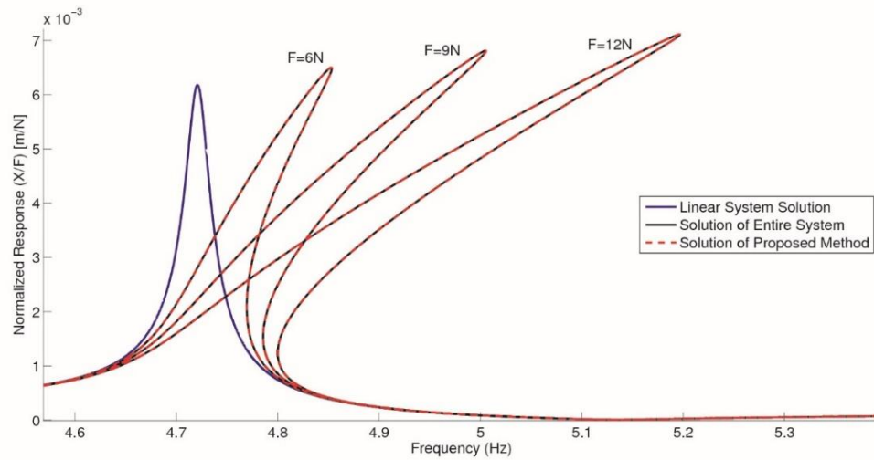
Fig. 11 Normalized response of the 1 th DOF in case study 3
