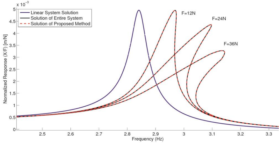
Fig. 8 Normalized response of the 1 th DOF in case study 2
