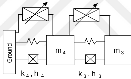
Figure 4.13 Schematic view of neural network trained substructure
