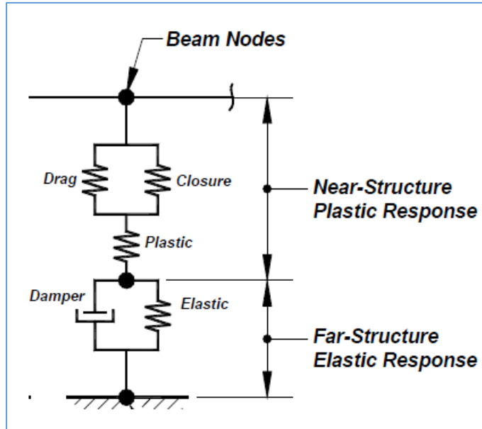
Figure 9. Typical zero length spring (proposed model)
