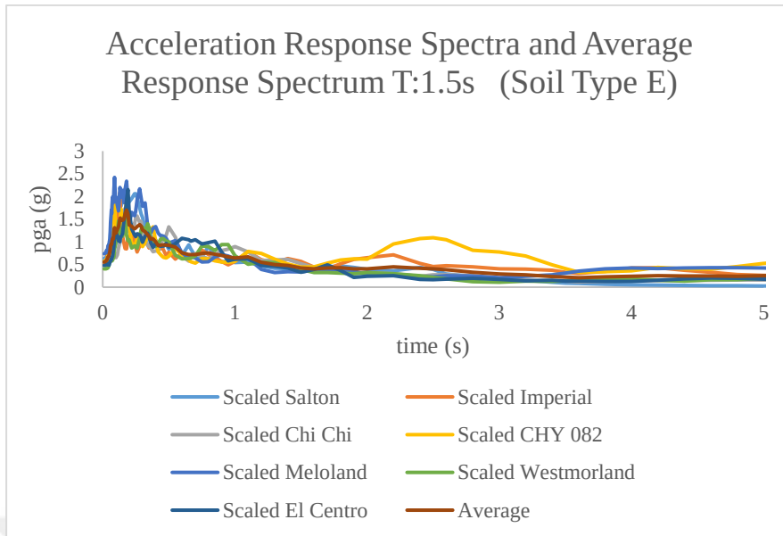
Figure 31. Acceleration Response Spectra and Average Response Spectrum of Soil Type E
