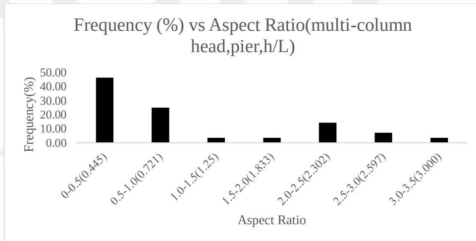
Figure 2. Frequency vs Aspect Ratios of Multi-Column Pier Bent (h/L)
