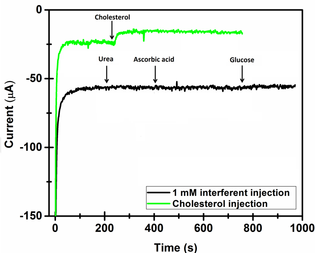
Figure 4.8 Amperometric responses of P(BImTh:Fmoc-Gly-OH)/ChOx biosensor to cholesterol and interference studies with ascorbic acid, urea and glucose solutions in 50 mM phosphate buffer, pH 7.0, 25 °C, -0.7 V.
