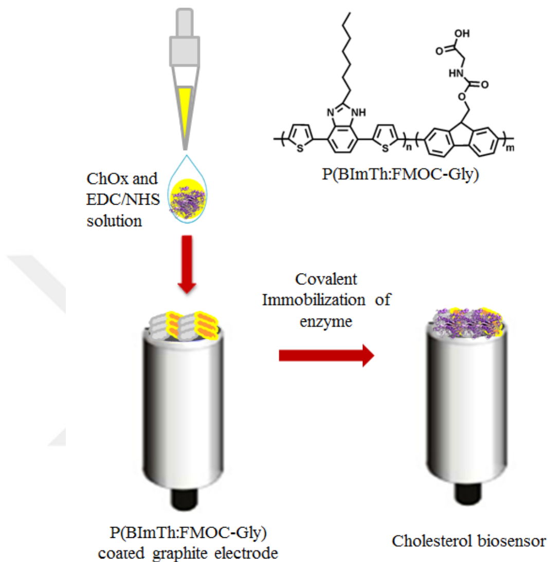
Figure 4.1 Typical preparation of the proposed biosensor.
