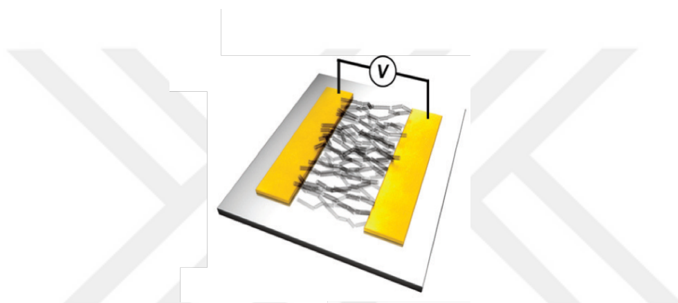
Figure 1.5 A chemiresistor based on a randomly oriented network of SWCNTs spanning two metallic electrodes [145].
