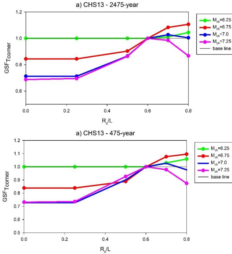
Figure 5.23 Calculation of Geometric Scale Factor for AMP_{T_{corner}} - 475-year CHS13
