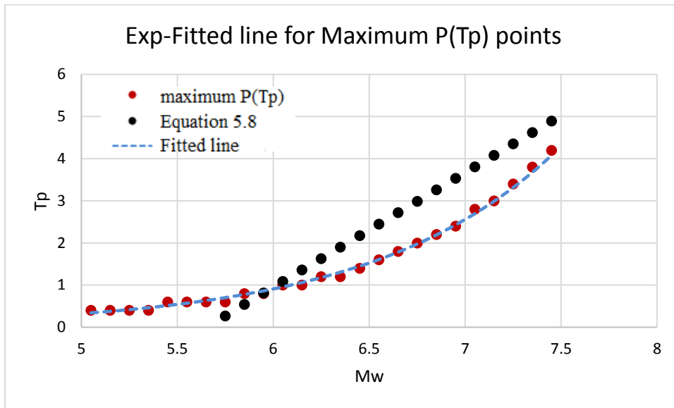
Figure B.3 Relation between magnitude and pulse period with maximum probability
