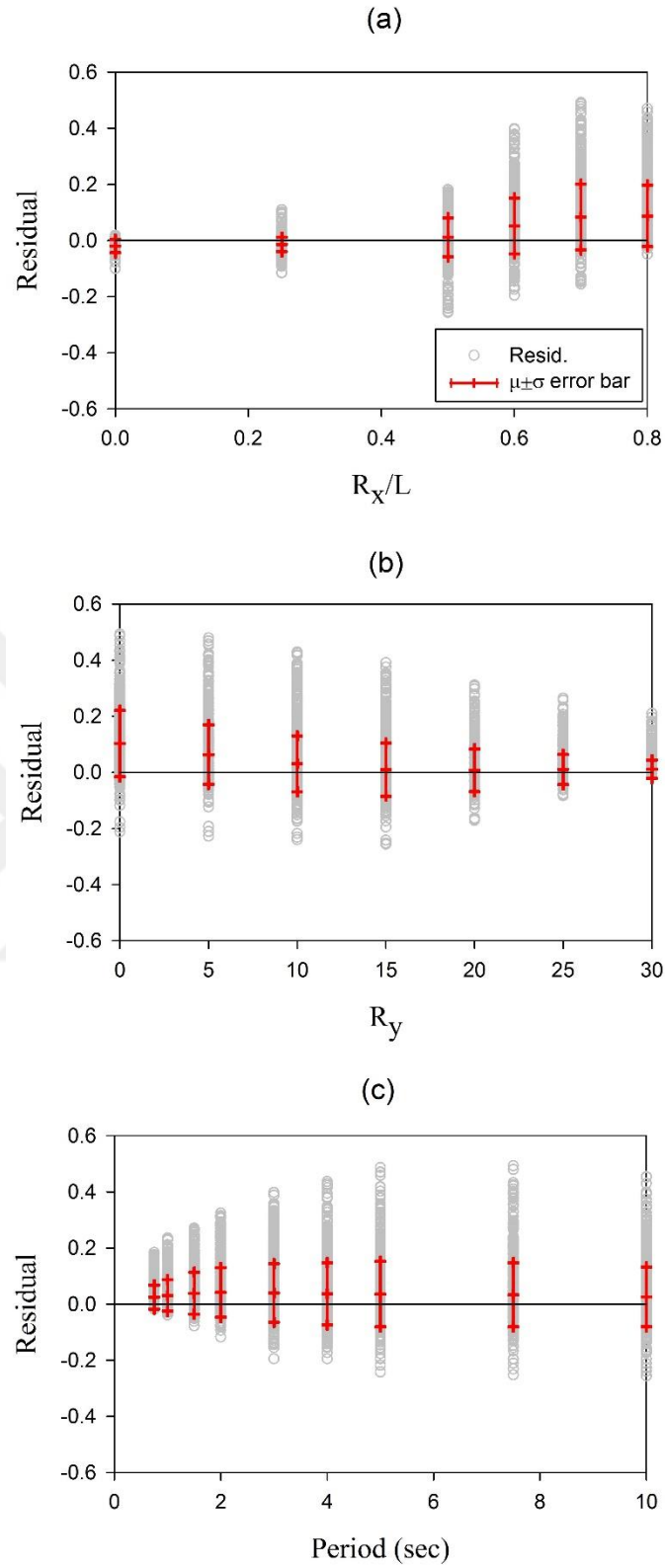
Figure 5.30 Residuals of PSHA and estimated amplification factors for CHS13 model, for the 475-year return period
