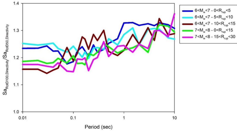
Figure 4.15 RotD100 to RotD50 spectral amplitude ratios for the pulselike bins in Table 4.2
