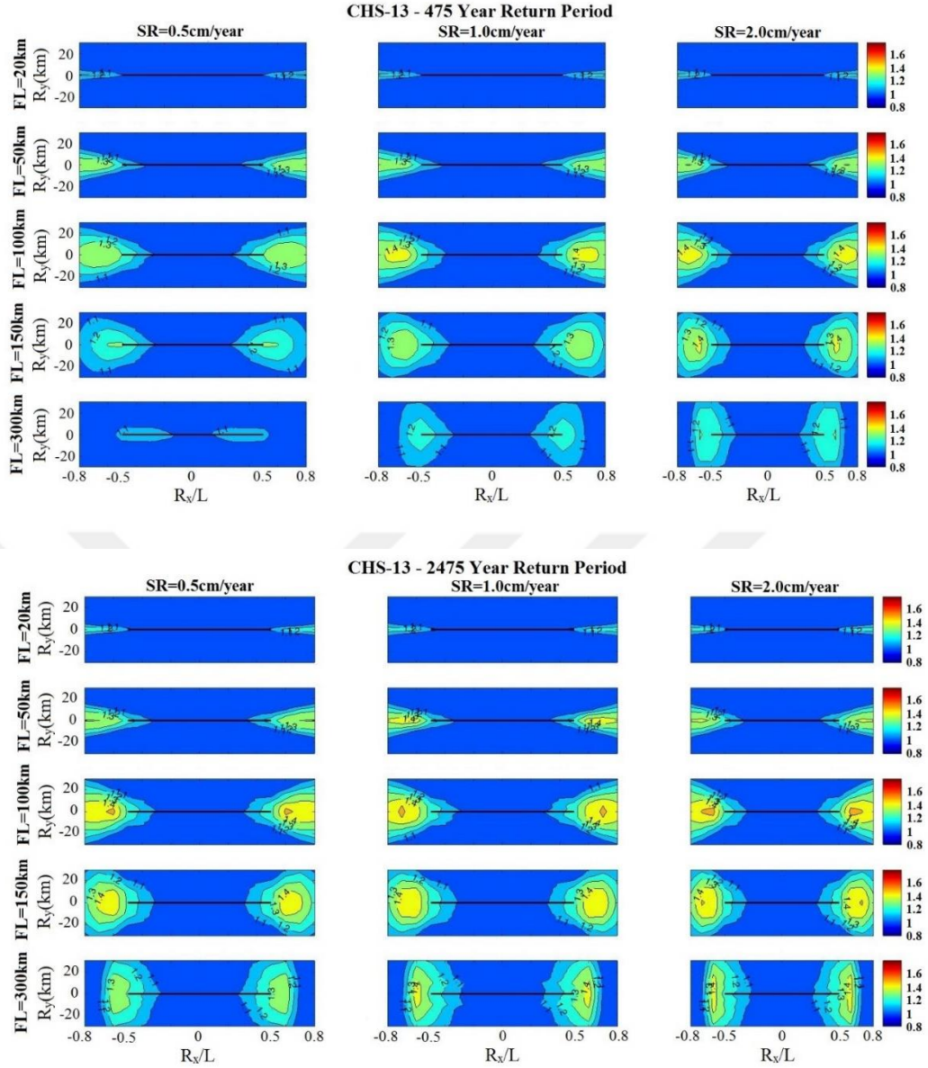
Figure 3.14 The spatial distribution of the forward-directivity spectral amplifications by CHS13 in terms of the return period, slip rate and the fault length (thus the characteristic earthquake magnitude)
