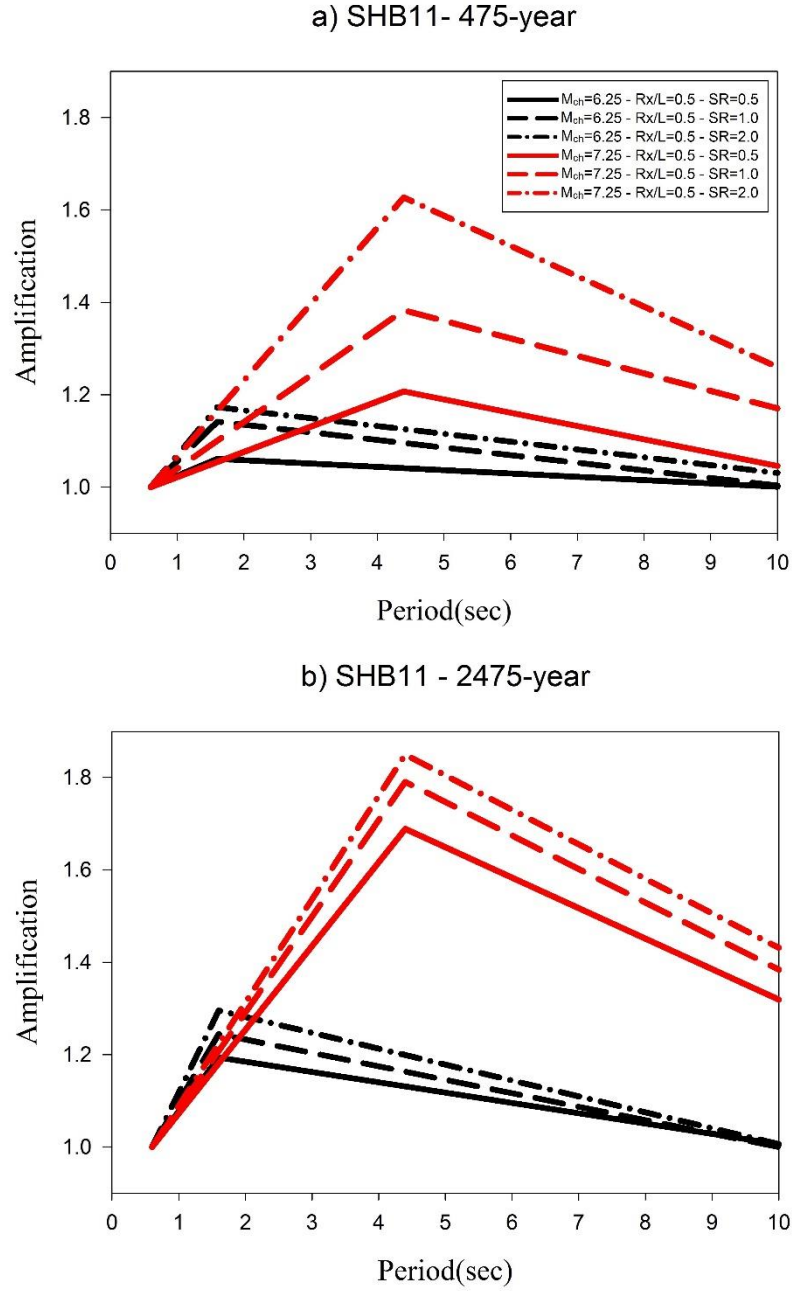
Figure 5.20 Effect of characteristic magnitude and slip rate on the directivity amplifications for SHB11 model computed from proposed simplified expressions a) 475-year return period b) 2475-year return period
