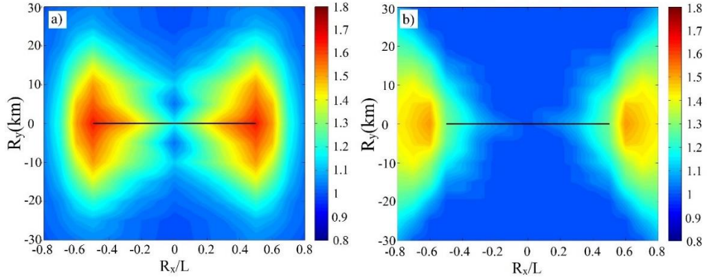
Figure 3.9 475-year probabilistic spectral amplifications for forward-directivity computed by (a) SHB11 and (b) CHS13 (via CY14) for a fault length of L = 100\text{km} and \dot{s} = 2\text{cm/year}
