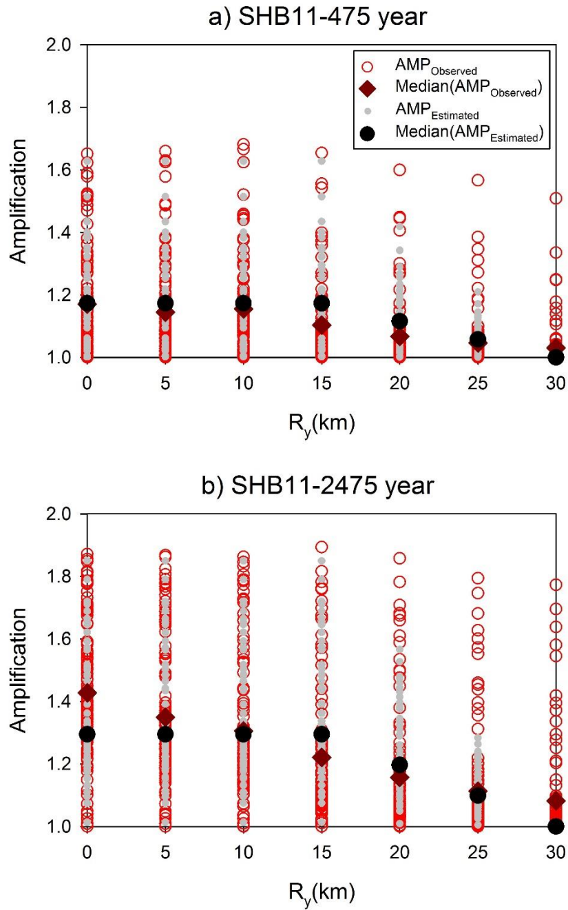
Figure 5.26 Observed and estimated directivity amplifications as a function of R_y for simplified SHB11 model
