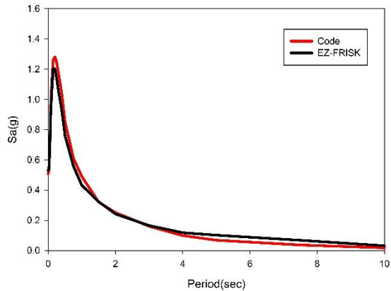
Figure B.6 Response spectrum calculated for FL=20km, \dot{S}=1.0\text{com/year} for site 15 with EZ-FRISK and the Matlab code (2475-year return period)
