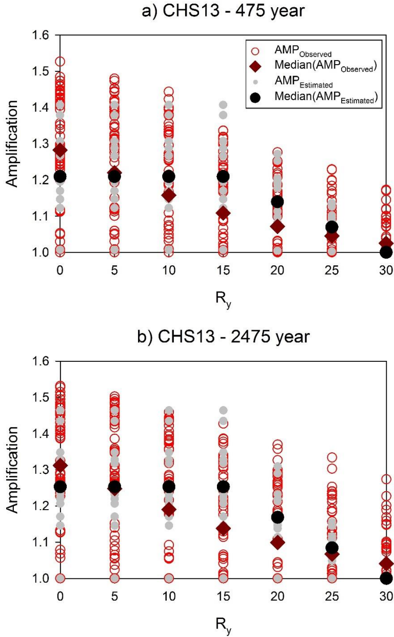
Figure 5.27 Observed ad estimated directivity amplifications as a function of R_y for CHS13 model
