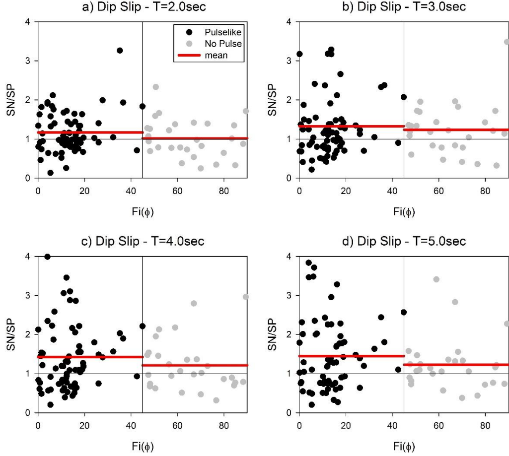
Figure 4.4 Comparisons of SN/SP spectral ratios at T = 2\text{s} , 3\text{s} , 4\text{s} and 5\text{s} by considering the \phi = 45^\circ criterion as the boundary between pulselike and non-pulse dip-slip recordings. The red solid lines show the average of pulselike and non-pulse SN/SP ratios.
