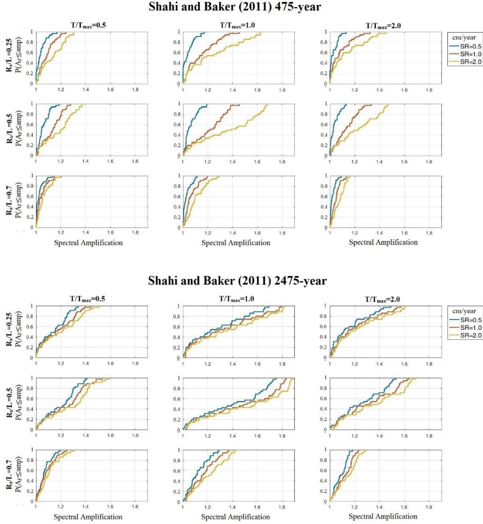
Figure 3.10 Non-exceedance probabilities (cumulative density functions) of directivity spectral amplifications according to Shahi and Baker (2011) directivity model given a range of R_x/L , T/T_{max} and average slip rate. First three rows show the probabilities for the 475-year return period. The last three rows pertain to the 2475-year return period probabilities
