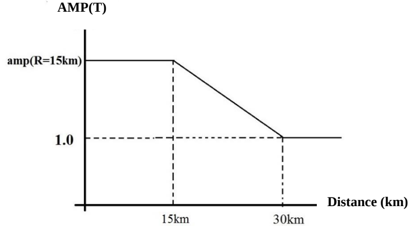
Figure 5.25 Distance Tapering of Directivity Amplification Factor
