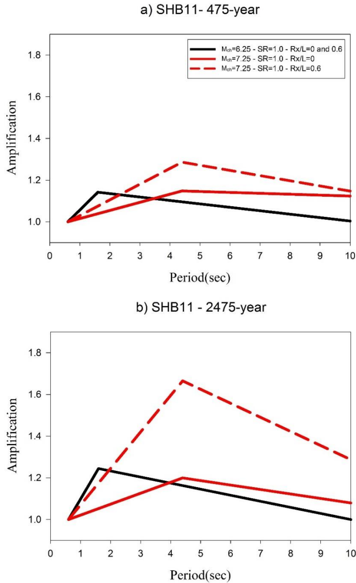
Figure 5.21 Effect of fault-site geometry ( R_x/L ) on the directivity amplifications of SHB11 narrow-band model computed from the proposed simplified formulations a) 475-year return period b) 2475-year return period
