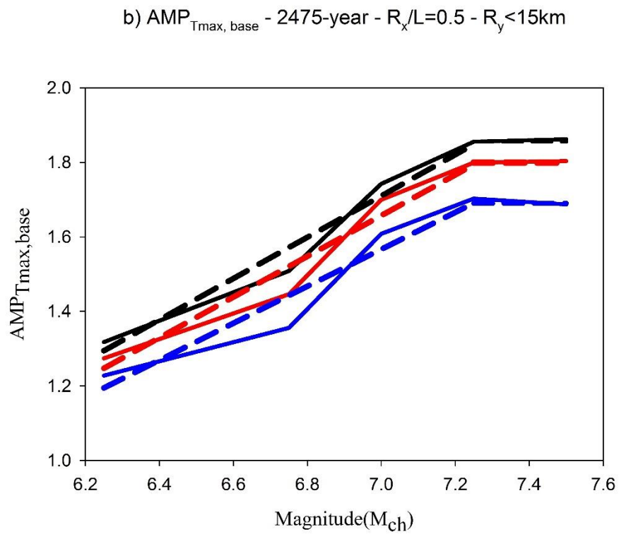
Figure 5.13 SHB11-based directivity amplification vs M_{ch} relationship together with linear fits calculated for the sites 3, 9, 15 and 21 at spectral period T_{max} a) 475-year return period b) 2475-year return period
