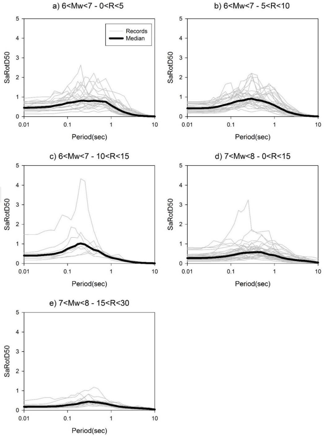
Figure 4.11 Sa_{RotD50directivity} (from pulslike records) spectral amplitudes of individual ground motions of the bins given in Table 4.2. The solid black lines are the log-mean (median) spectral curves of each bin.
