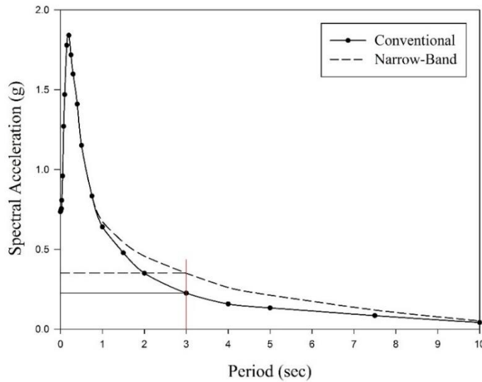
Figure 5.5 Normalization of 2475-year return period narrow-band spectrum to conventional spectrum
