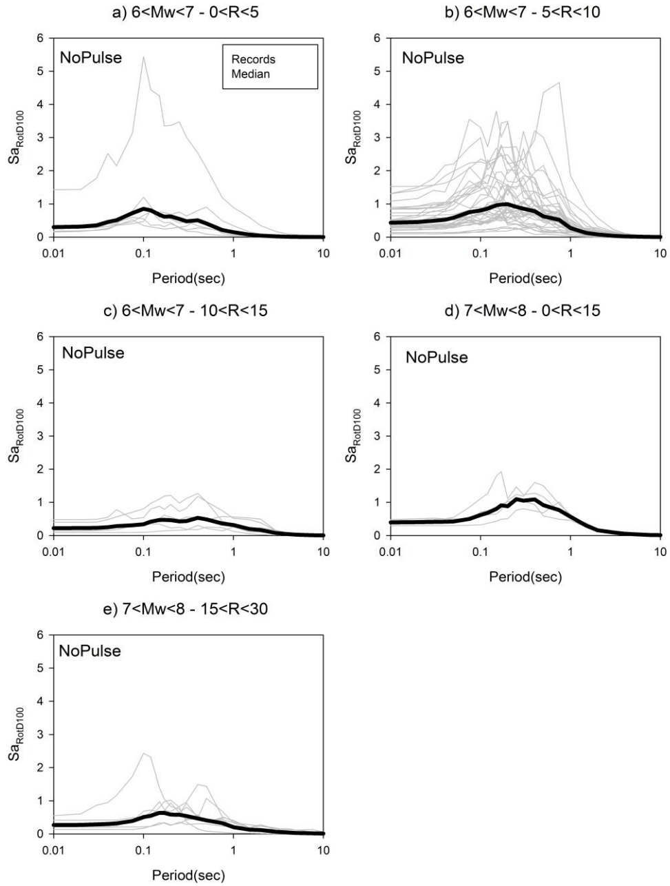
Figure 4.9 Sa_{RotD100nodirectivity} (from non-pulse records) spectral amplitudes of individual ground motions of the bins given in Table 4.2
