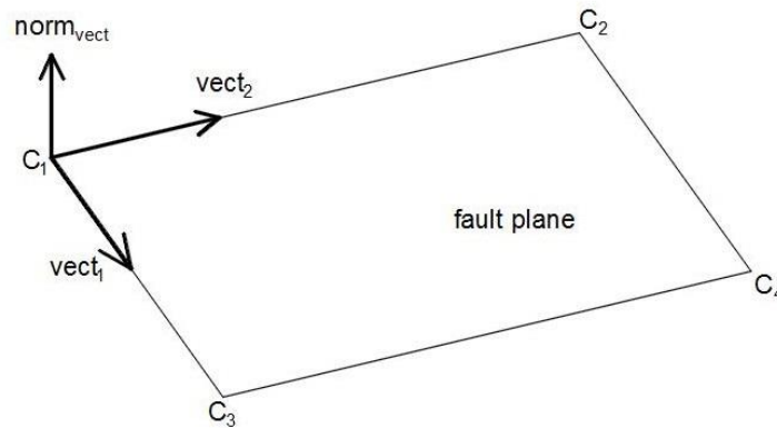
Figure A.1 Fault normal vector
