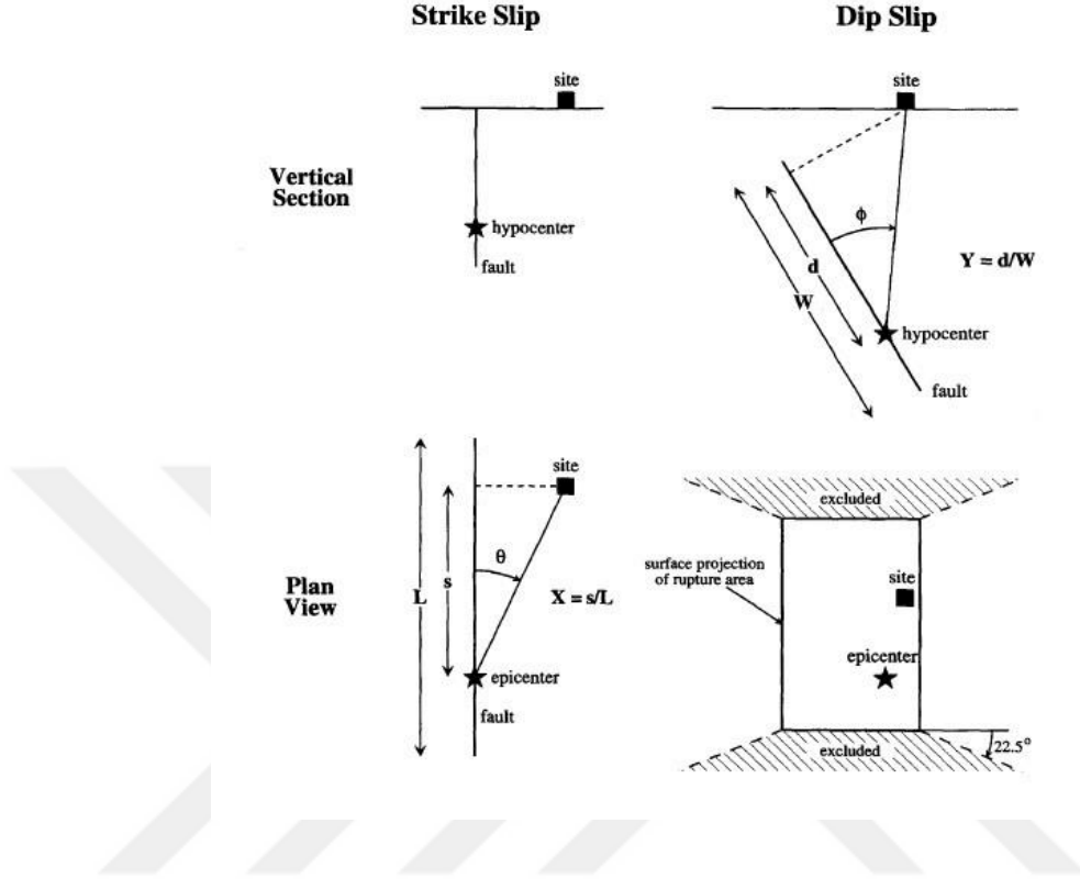
Figure 2.5 Geometric parameters used in Somerville (1997) directivity model.
