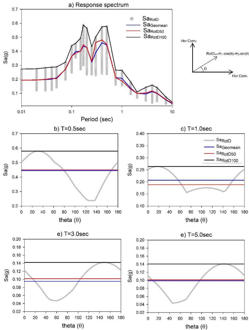
Figure 2.8 Response spectrum of Gebze station-1999 Kocaeli earthquake calculated for different rotated orientations of two horizontal components, together with geometric mean, RotD50 and RotD100 components illustrated for different spectral periods
