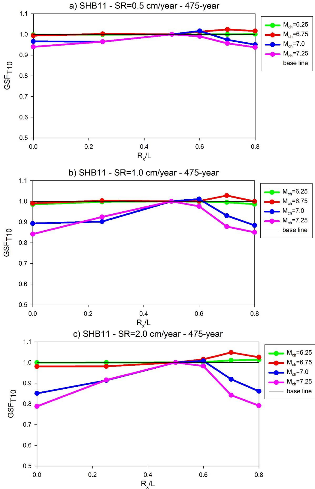
Figure 5.18 Observed geometric scale factors for AMP_{T10} - 475-year return period and \dot{s} = 0.5\text{cm/year} , \dot{s} = 1.0\text{cm/year} and \dot{s} = 2.0\text{cm/year} (SHB11)
