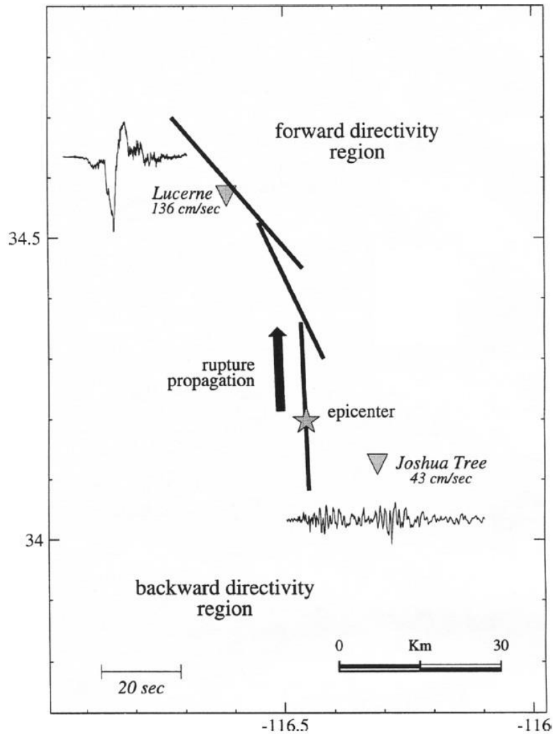
Figure 2.1 Strike normal forward-directivity and backward-directivity ground velocities from the 1992 Landers earthquake (Somerville et al. 1997)
