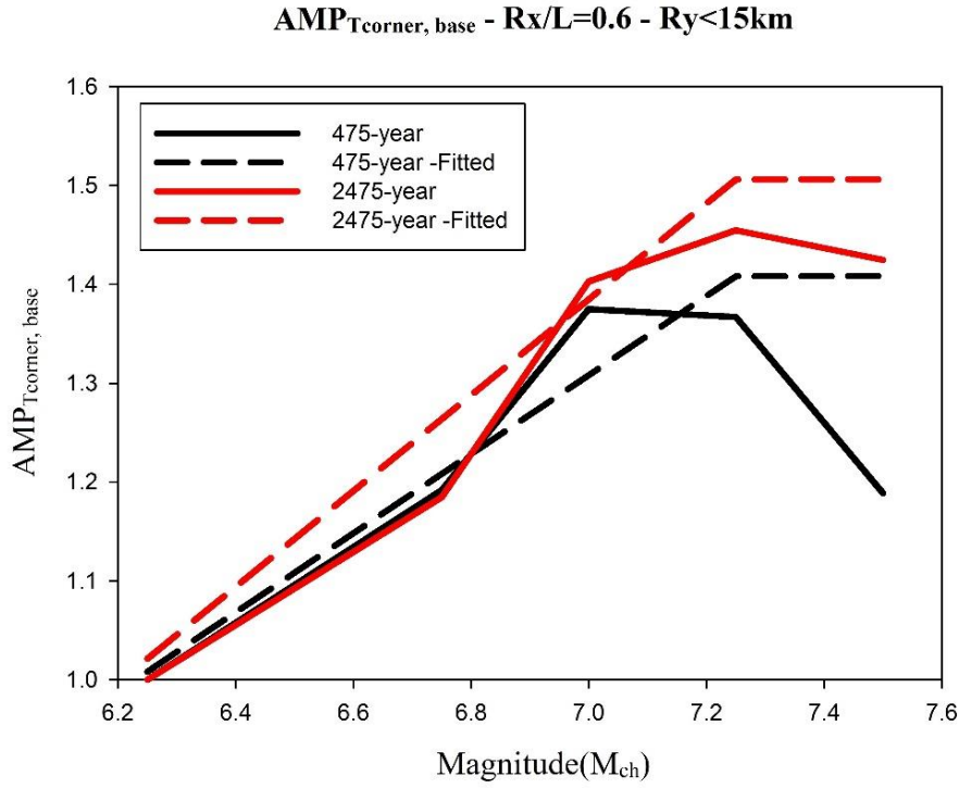
Figure 5.22 Base amplification factors and magnitude relationships together with linear line fits calculated for sites 4, 10, 16 and 22 at spectral period T_{corner} - CHS13 model, 475- and 2475-year return period
