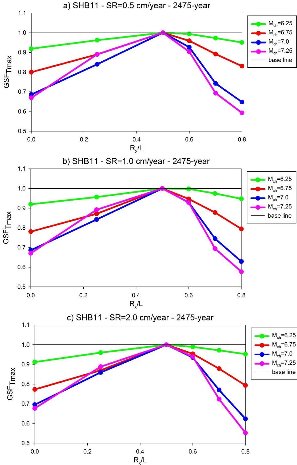
Figure 5.17 Observed geometric scale factors for AMP_{Tmax} - 2475-year return period and \dot{s} = 0.5\text{cm/year} , \dot{s} = 1.0\text{cm/year} and \dot{s} = 2.0\text{cm/year} (SHB11)
