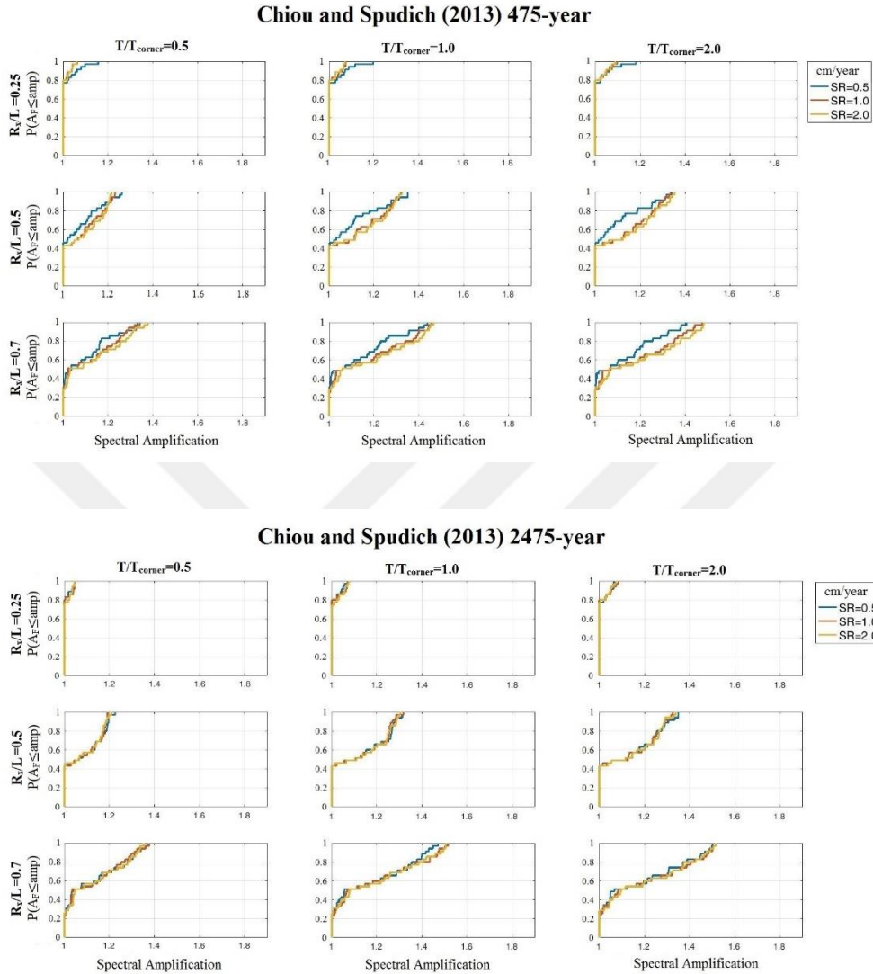
Figure 3.11 Same as Figure 3.10 but the forward-directivity model is Chiou and Spudich (2013; Chapter 6 in Spudich et al., 2013) implemented in Chiou and Youngs (2014) GMPM
