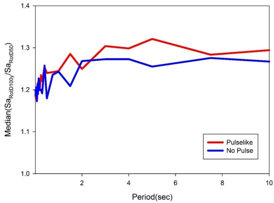
Figure 4.17 Medians of RotD100 to RotD50 spectral ratio curves computed from pulselike (Figure 4.15) and non-pulse (Figure 4.16) bins
