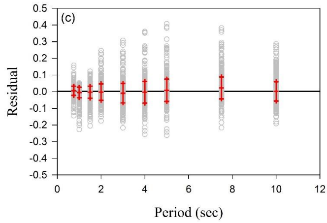
Figure 5.4 Residuals between PSHA (observed) and the estimated directivity amplifications for 475-year return period
