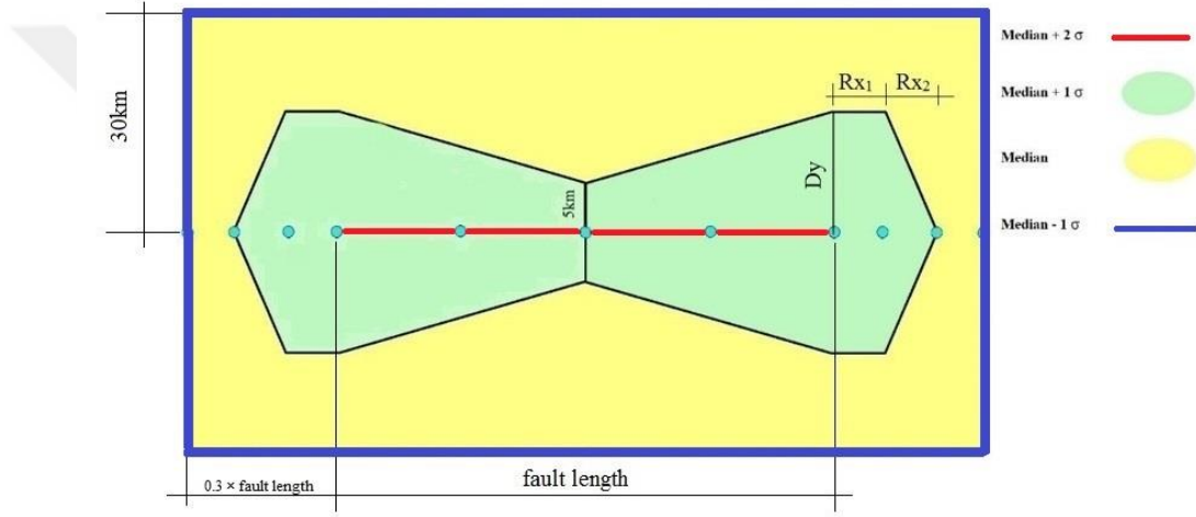
Figure 5.8 Classification of the area around the fault into four regions with respect to NRM_{amp}(T) intensities
