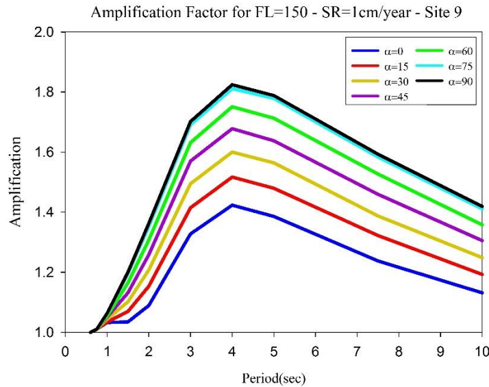
Figure 3.8 Variation of forward-directivity spectral amplifications as a function of \alpha (alpha) at Site 9 for the fictitious PSHA scenario considered in Figure 3.6.
