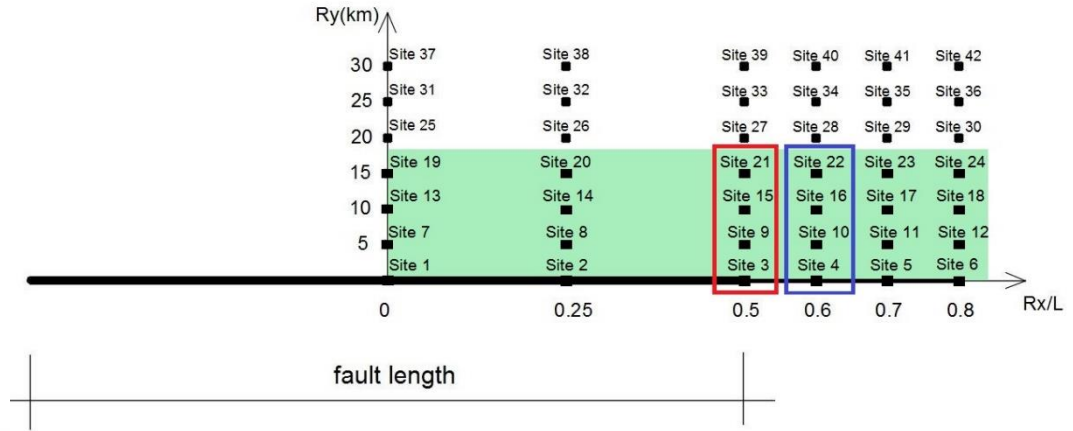
Figure 5.9 Spatial distribution of the sites around the fault and the sites located in the boundary region
