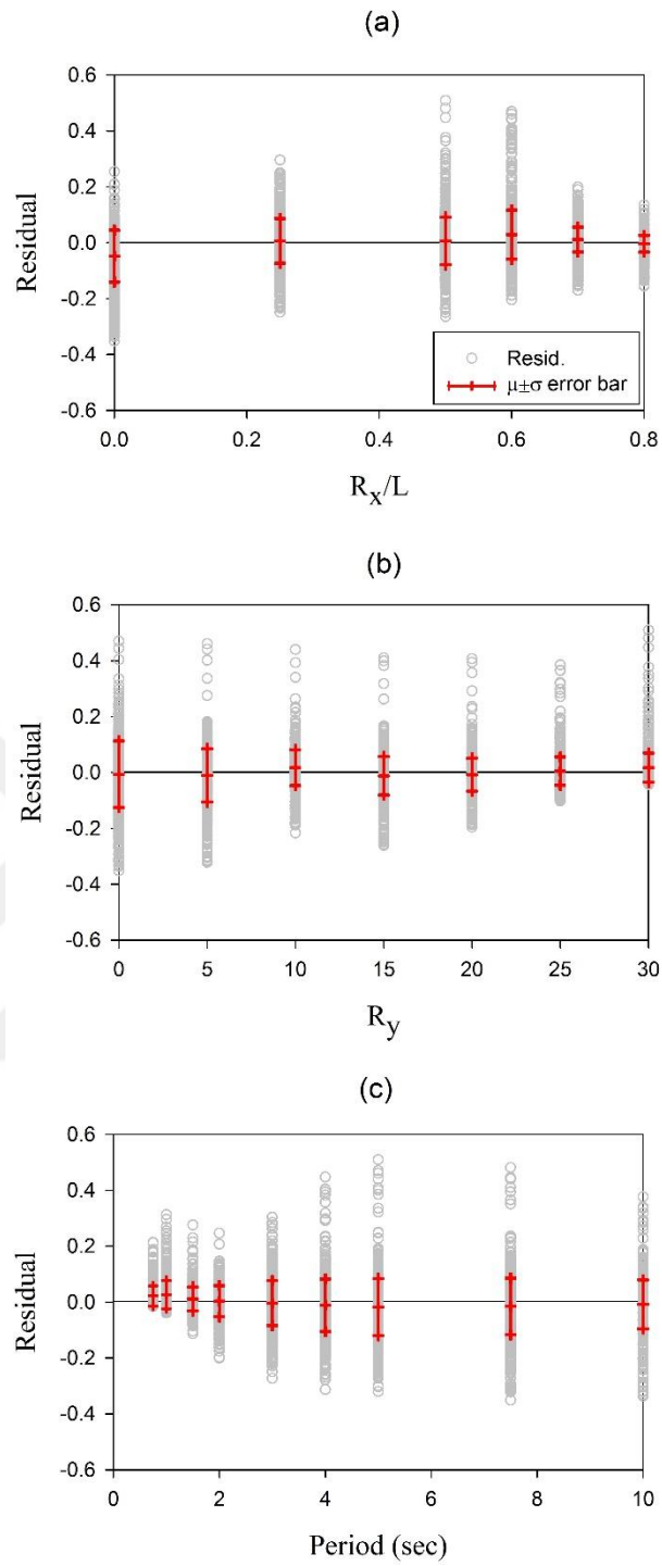
Figure 5.28 Residuals computed from PSHA (observed) and estimated directivity amplifications for SHB11 narrow-band directivity model, for the 475-year return period
