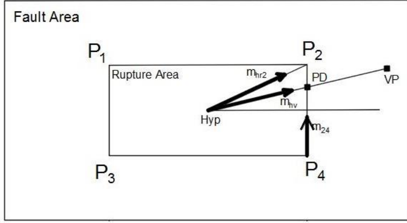
Figure A.4 Calculation of direct point for the case that closest point is located outside the rupture area
