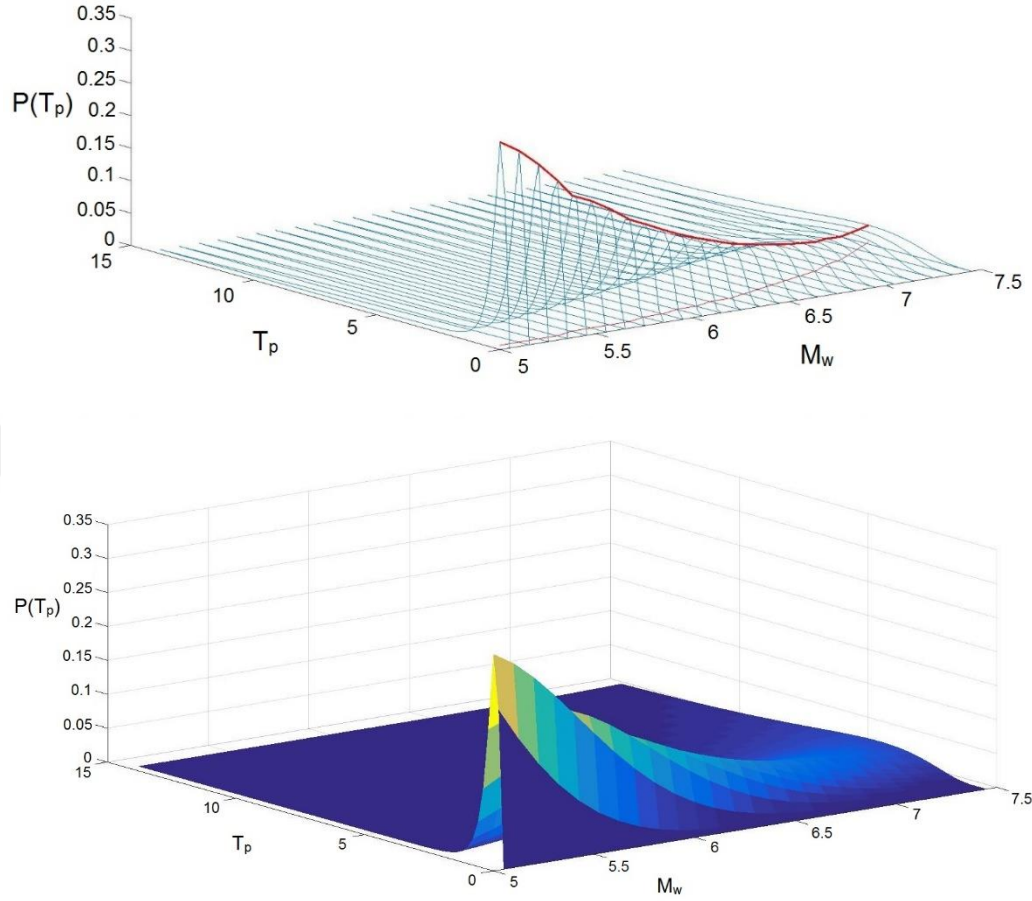
Figure B.2 Illustration of lognormal distribution for magnitude-pulse period and related probability of pulse period
