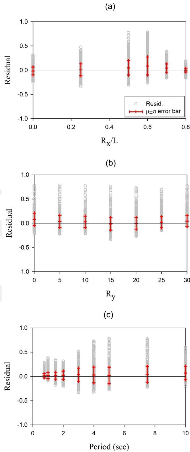
Figure 5.29 Residuals computed from PSHA (observed) and estimated directivity amplifications for SHB11 narrow-band directivity model for the 2475-year return period
