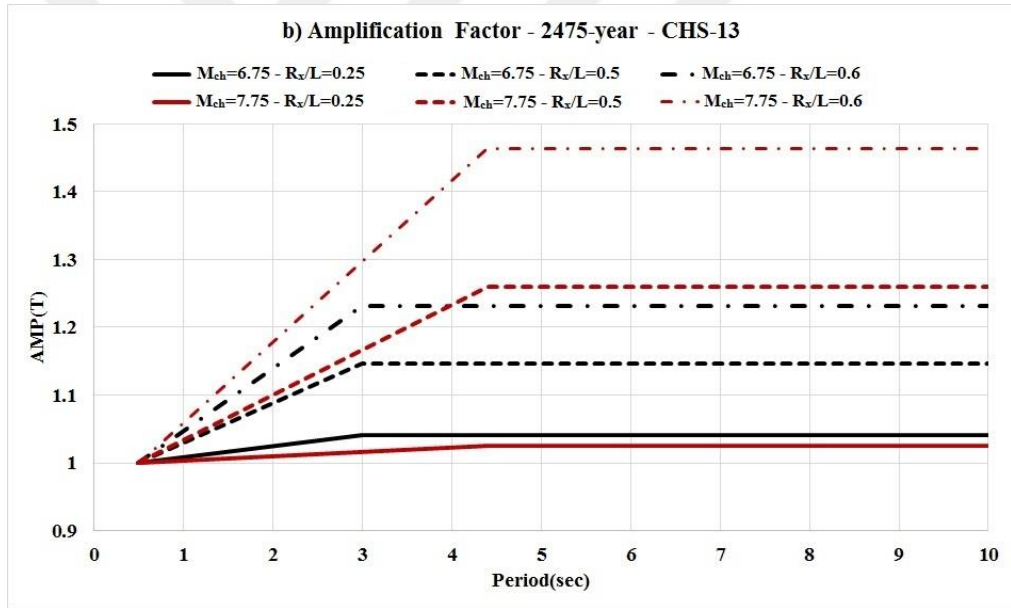
Figure 5.24 Amplification Model for RotD50 Component of CHS13
