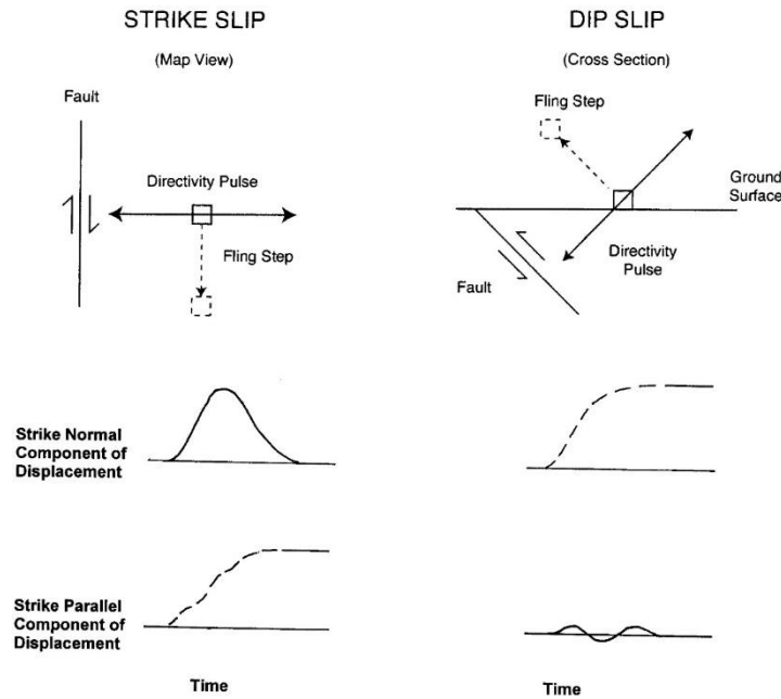
Figure 2.2 Illustration of orientations of motion from fling step and directivity effects in strike slip and dip-slip ruptures (Somerville 2002)
