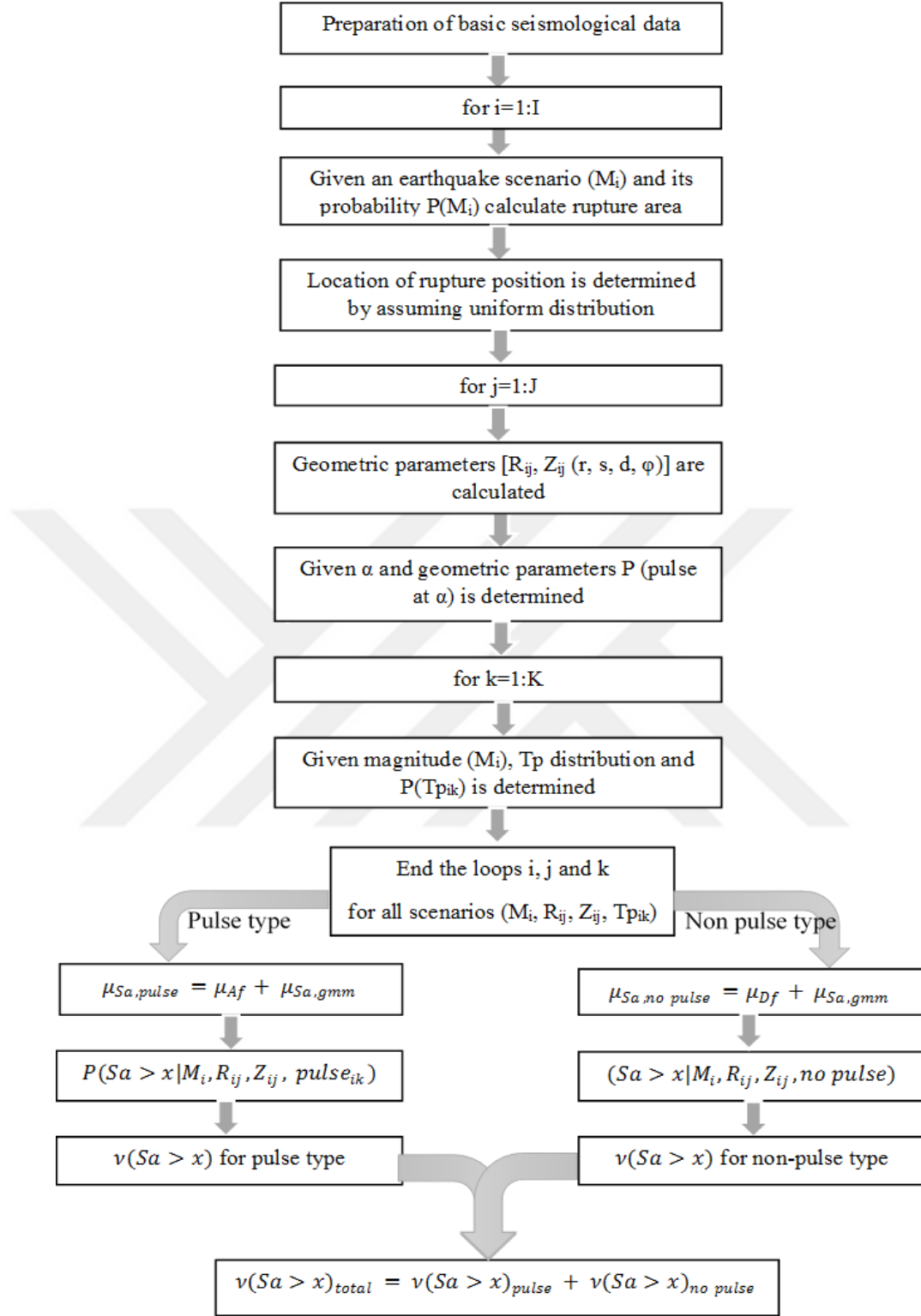
Figure B.1 Algorithm for SHB11 PSHA narrow-band model
