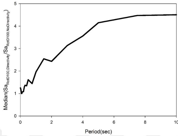
Figure 4.14 Median of Sa_{\text{RotD100directivity}} to Sa_{\text{RotD100nodirectivity}} ratios presented in Figure 4.10
