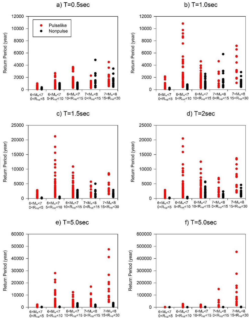
Figure 5.32 Return periods related to the spectral amplitudes of pulse-like and nonpulse recordings
