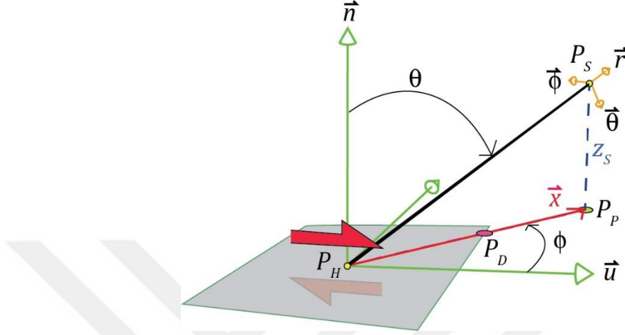
Figure A.5 Geometrical information for the calculation of average scalar radiation pattern ( \overline{\mathbf{FS}} ) parameter (Spudich et al. 2013)
