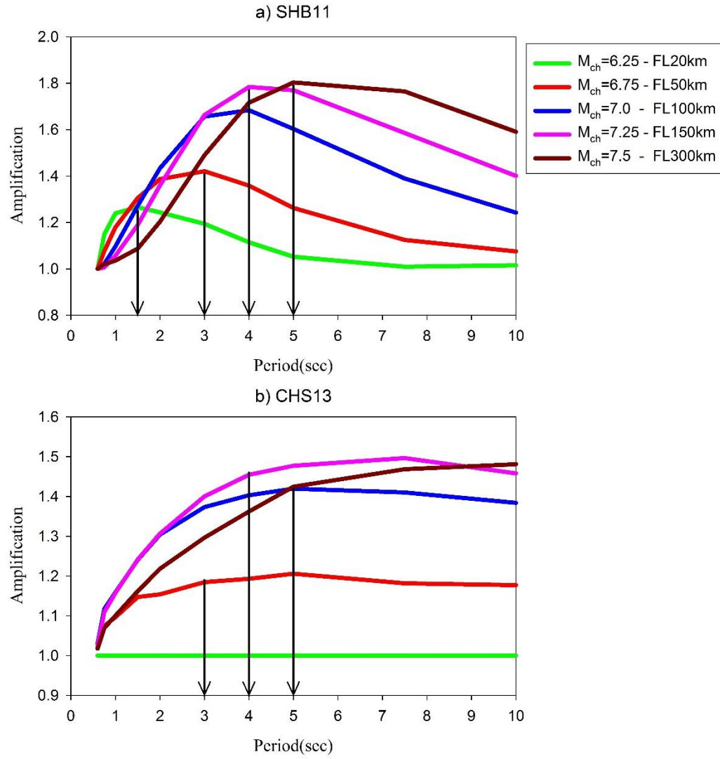
Figure 5.11 Median SHB11 and CHS13 directivity amplifications in terms of M_{ch} and the variation of T_{max} and T_{corner} with the characteristic magnitudes
