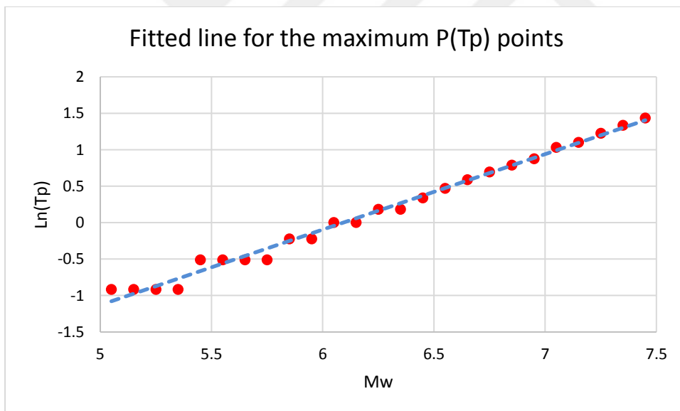
Figure B.4 Relation between magnitude and pulse period with maximum probability
