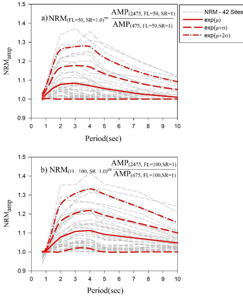
Figure 5.6 Normalized period-dependent 2475-year to 475-year directivity dominant spectral amplification ratios of 42 sites (grey curves) and corresponding logarithmic mean, \pm\sigma as well as 2\sigma over logarithmic mean a) fictitious fault with 50km length and \dot{s} = 1\text{cm/year} b) fictitious fault with 100km length and \dot{s} = 1\text{cm/year}
