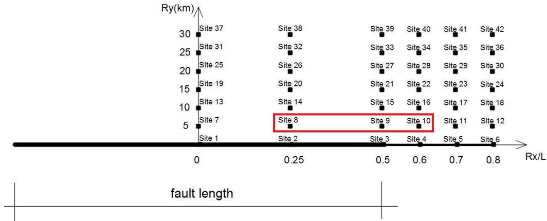
Figure 3.5 Plan view of fault-site configuration used in this study. (The red rectangle encloses the sites 8, 9 and 10 that are used in the deterministic scenario)
