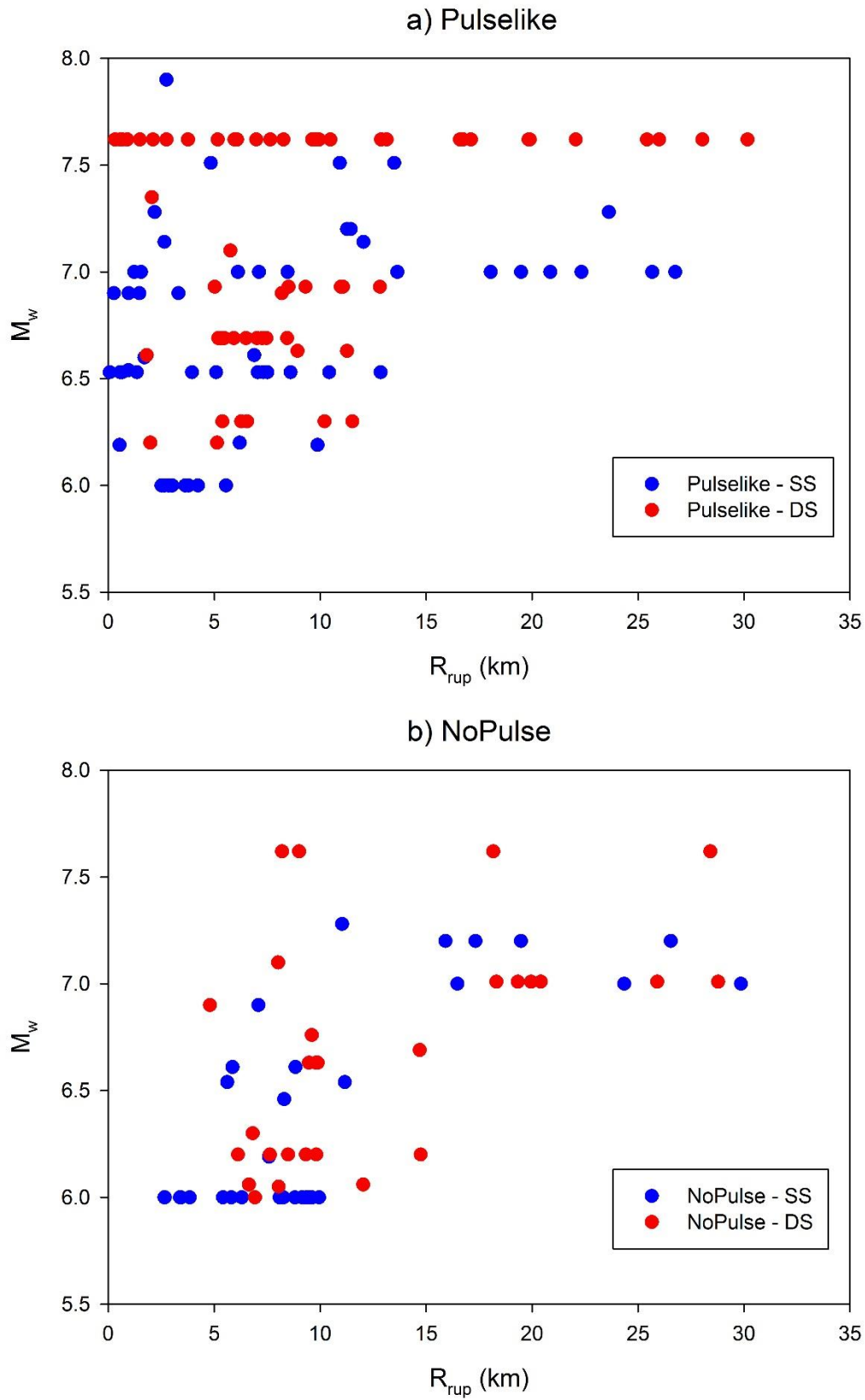
Figure 4.2 Magnitude versus distance distribution of (a) pulslike and (b) non-pulse ground motions for different styles of faults (dip-slip and strike-slip)
