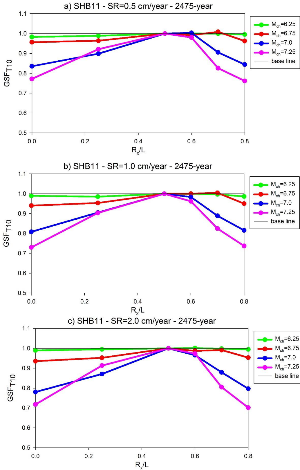
Figure 5.19 Observed geometric scale factors for AMP_{T10} - 2475-year return period and \dot{s} = 0.5\text{cm/year} , \dot{s} = 1.0\text{cm/year} and \dot{s} = 2.0\text{cm/year} (SHB11)
