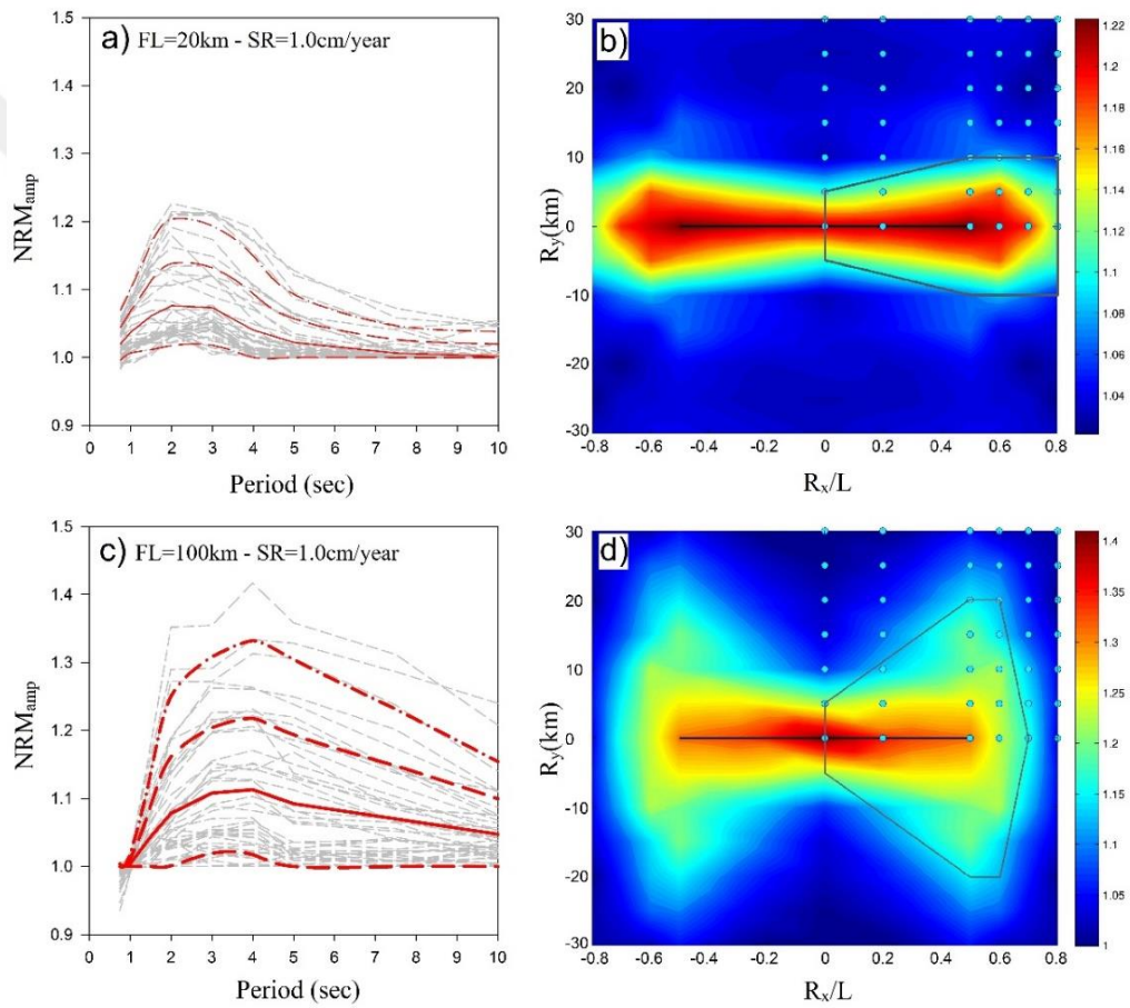
Figure 5.7 Comparison of \text{NRM}_{\text{amp}} and the related contour maps for classification of the sites a) \text{NRM}_{\text{amp}} vs T(\text{sec}) for \text{FL}=20\text{km} , \dot{S}=1\text{cm/year} b) contour map of \text{NRM}_{\text{amp}} for T=2.0\text{sec} \text{FL}=20\text{km} , \dot{S}=1\text{cm/year} c) \text{NRM}_{\text{amp}} vs T(\text{sec}) for \text{FL}=100\text{km} , \dot{S}=1\text{cm/year} d) contour map of \text{NRM}_{\text{amp}} for T=4.0\text{sec} \text{FL}=100\text{km} , \dot{S}=1\text{cm/year}
