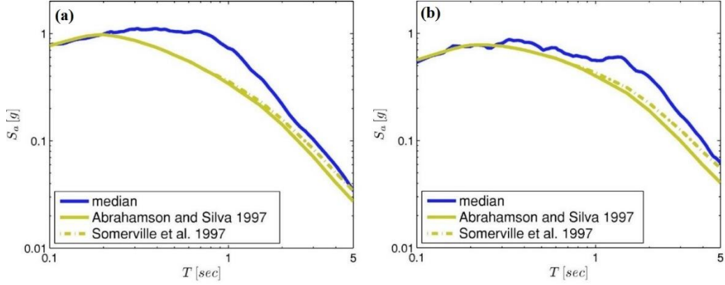
Figure 2.3 Response spectrum of pulse-type records with a) 0.6 \leq T_p < 1.5 (mean T_p = 1.0s ) and b) 1.5 \leq T_p < 2.5 (mean T_p = 1.9s ). The plots also show the response spectrum computed from conventional Abrahamson and Silva (1997) GMPE and the broad-band model by Somerville et al. (1997) (Tothong et al. 2007)
