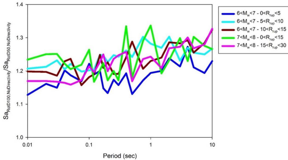
Figure 4.16 RotD100 to RotD50 spectral amplitude ratios for the nonpulse bins in Table 4.2
