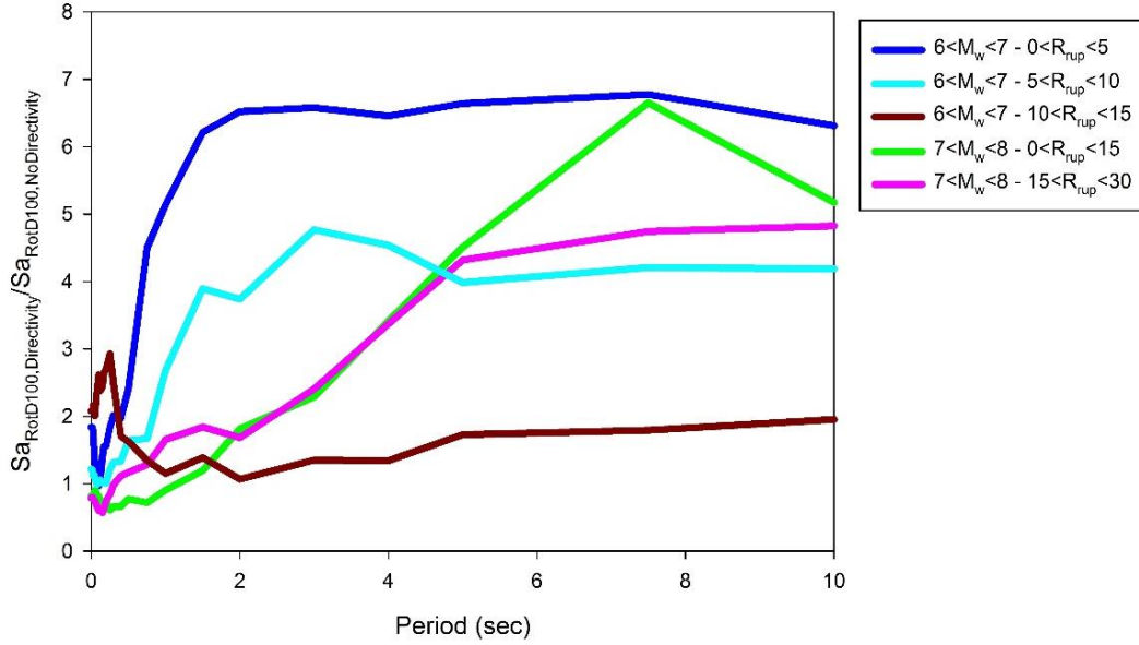
Figure 4.10 AF_{\text{directivity}} curves computed from median Sa_{\text{RotD100directivity}} to Sa_{\text{RotD100nondirectivity}} ratios of the ground-motion bins presented in Table 4.2
