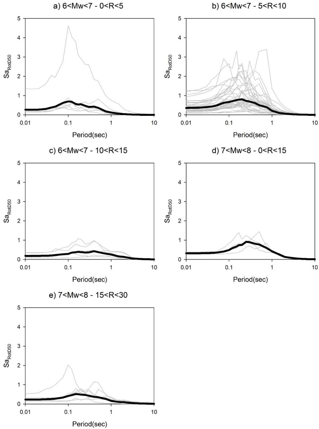
Figure 4.12 Sa_{RotD50_{nondirectivity}} (from non-pulse records) spectral amplitudes of individual ground motions of the bins given in Table 4.2. The solid black lines are the log-mean (median) spectral curves of each bin
