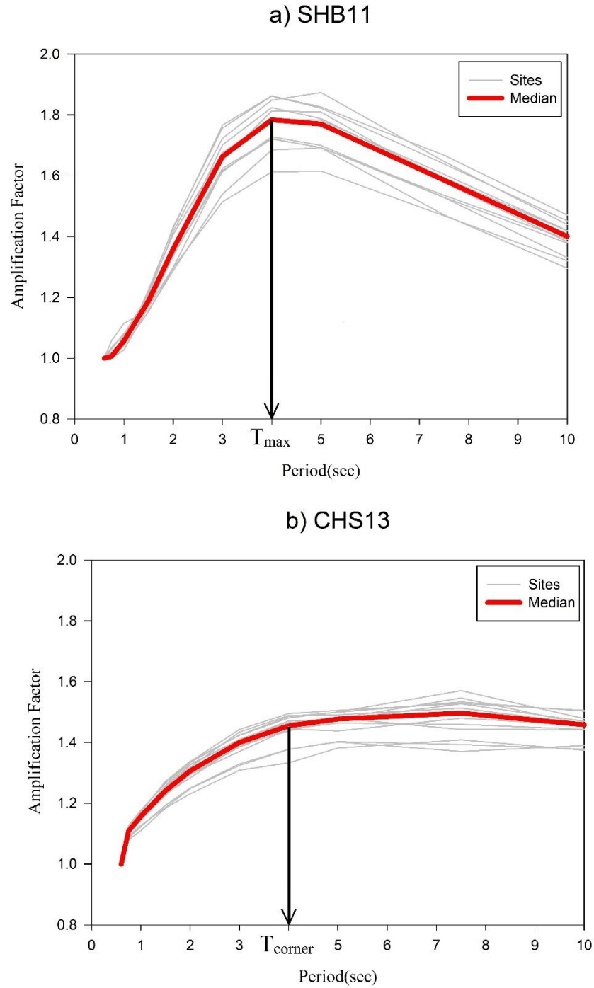
Figure 5.10 T_{\max} and T_{\text{corner}} values for directivity amplifications. The earthquake scenario is FL=150km ( M_{\text{ch}}=7.25 ), \dot{s} = 0.5\text{cm/year} , 1\text{cm/year} , 2\text{ cm/year} a) SHB11 model b) CHS13 model
