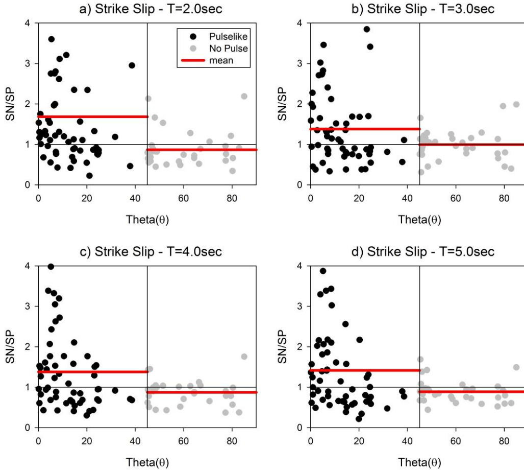
Figure 4.3 Comparisons of SN/SP spectral ratios at T = 2\text{s} , 3\text{s} , 4\text{s} and 5\text{s} by considering the \theta = 45^\circ criterion as the boundary between pulselike and non-pulse strike-slip recordings. The red solid lines show the average of pulselike and non-pulse SN/SP ratios.
