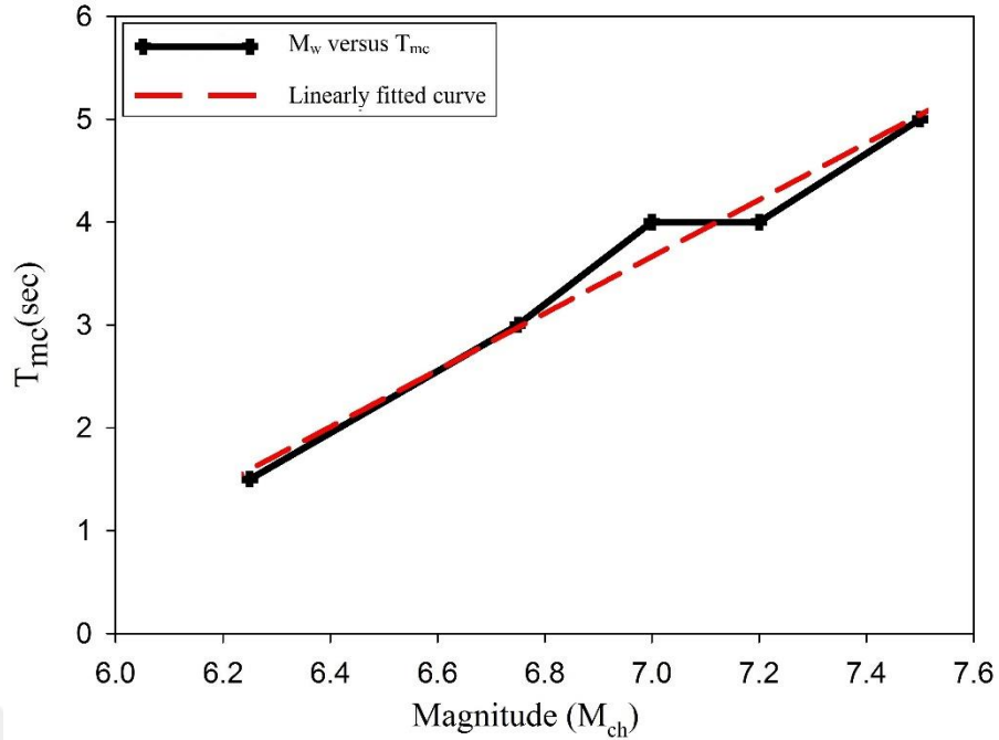
Figure 5.12 Relationship between characteristic magnitude and the spectral period ( T_{mc} ) at which the maximum directivity amplification occur. Dashed red line is the fit to the actual trend given in black
