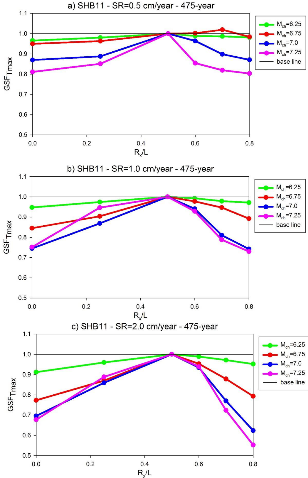
Figure 5.16 Observed geometric scale factors for AMP_{Tmax} - 475-year return period and \dot{s} = 0.5\text{cm/year} , \dot{s} = 1.0\text{cm/year} and \dot{s} = 2.0\text{cm/year} (SHB11)
