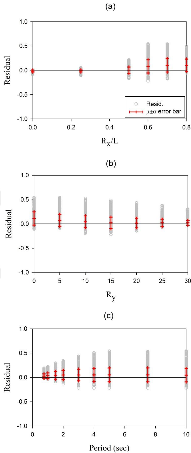
Figure 5.31 Residuals of PSHA and estimated amplification factors for CHS13 model, for the 475-year return period
