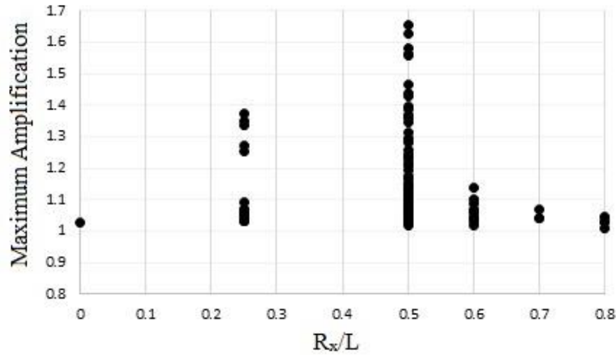
Figure 5.3 Maximum amplification values and location of the sites which experience the maximum value
