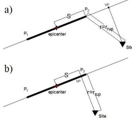
Figure A.6 Geometrical calculations for Shahi and Baker (2011) model
