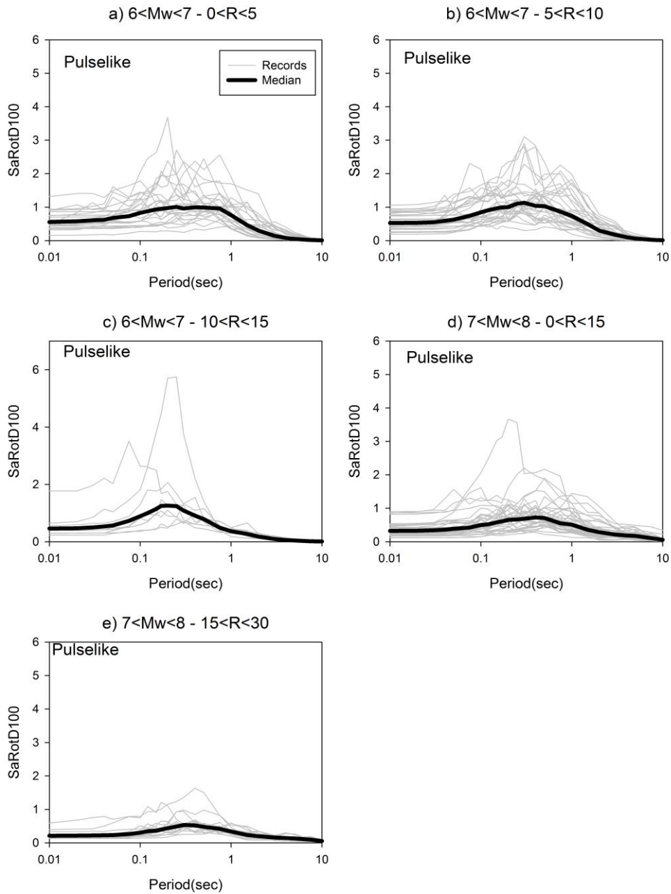
Figure 4.8 SaRotD100_{directivity} (from pulselike records) spectral amplitudes of individual ground motions of the bins given in Table 4.2
