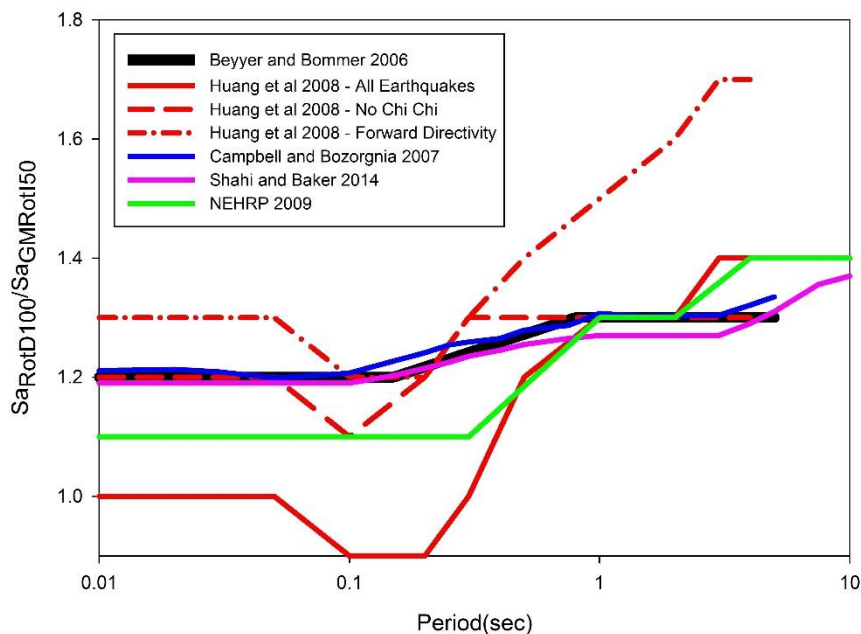
Figure 4.7 Comparison of different scaling (conversion) models proposed for Sa_{RotD100}/Sa_{GMRotI50} ratio
