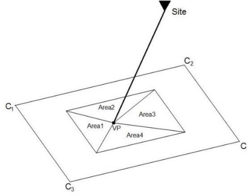
Figure A.3 Calculation of direct point for the case that closest point is located inside the rupture area
