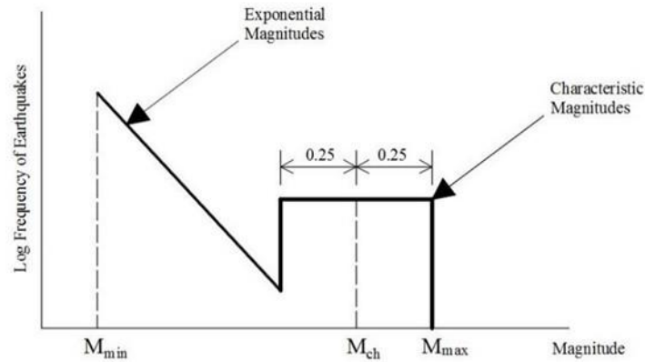
Figure 3.7 The Youngs and Coppersmith (1985) stochastic model to describe the earthquake recurrence in PSHA runs. The minimum magnitude, M_{min} , is always considered as M_w 5 in the probabilistic earthquake scenarios. The characteristic magnitude, M_{ch} , is determined from the mean M_w estimated from the empirical M_w vs. RA relationship in (Wells and Coppersmith 1994).
