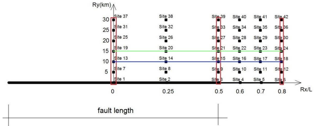
Figure 5.1 Spatial distribution of sites around the fictitious fault and the sites located in the boundary region enclosed by red rectangles
