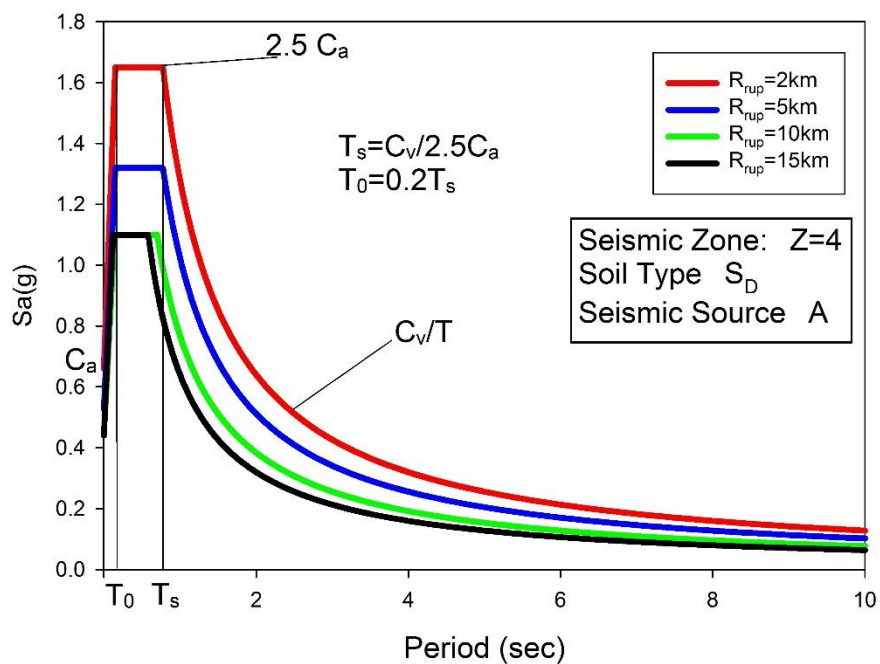
Figure 2.6 UBC 97 design spectrum calculated for seismic zone 4, soil type S_D and seismic source type A for closest distances 2, 5, 10 and 15km.
