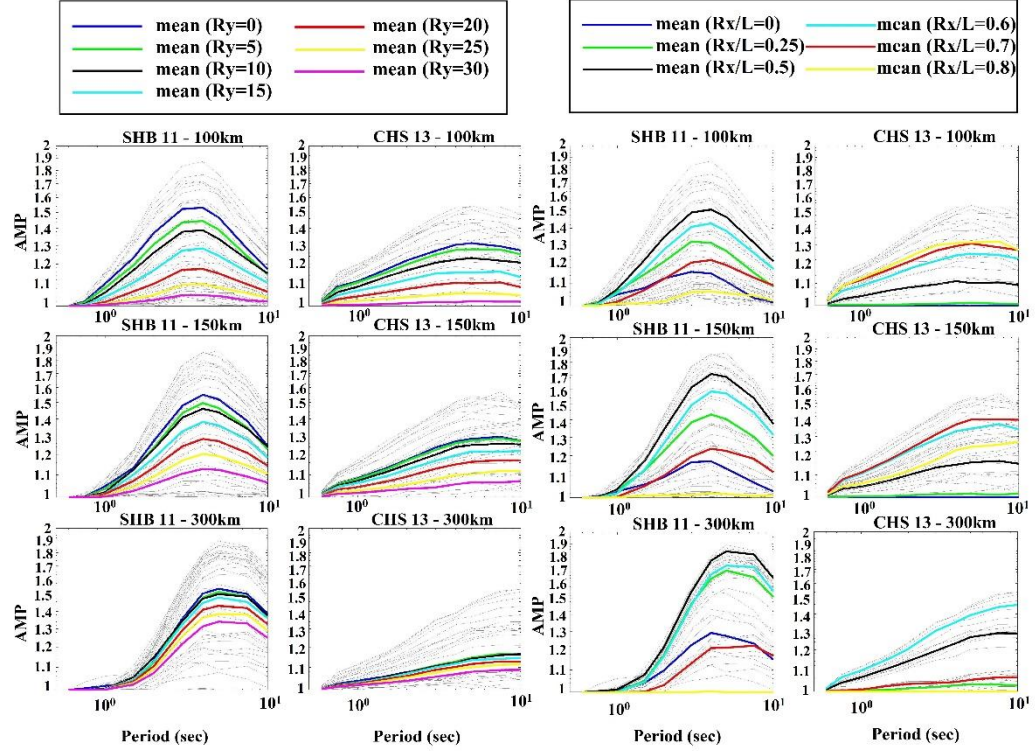
Figure 3.12 Period-dependent 2475-year forward-directivity spectral amplifications estimated by SHB11 and CHS13 for PSHA scenarios of fault lengths L = 100\text{km} (top row), L = 150\text{km} (middle row) and L = 300\text{km} (bottom row) having \dot{s}_{total} = 2.0\text{cm/year} . The first two columns show mean spectral amplifications of SHB11 (first column) and CHS13 (second column) for sites located at a constant R_y and the last two columns show mean spectral amplifications of SHB11 (third column) and CHS13 (fourth column) for sites located at a constant R_x/L
