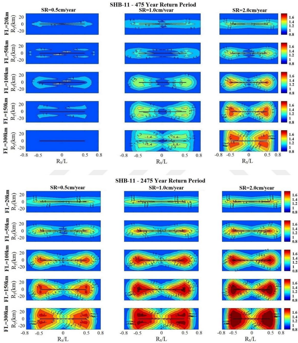
Figure 3.13 The spatial distribution of the forward-directivity spectral amplifications by SHB11 in terms of the return period, slip rate and the fault length (thus the characteristic earthquake magnitude)
