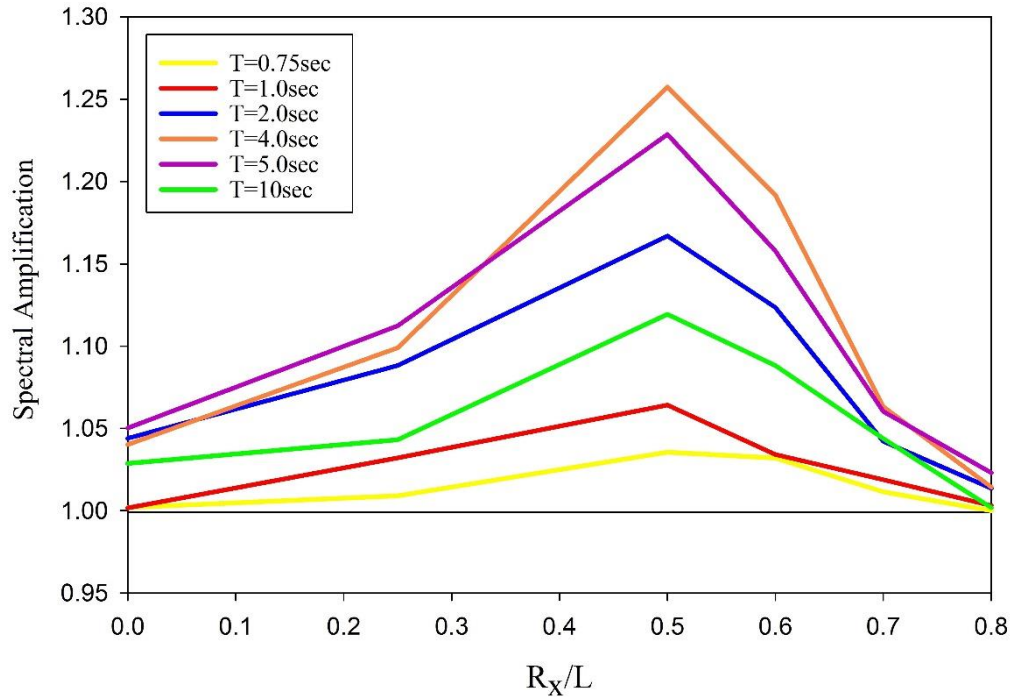
Figure 5.2 Bilinear trend for directivity-dominated spectral amplifications along fault strike, R_x/L , direction for a suit of spectral periods ( FL = 100\text{km} , \dot{s} = 1.0\text{cm/year} , R_y=15\text{km} )
