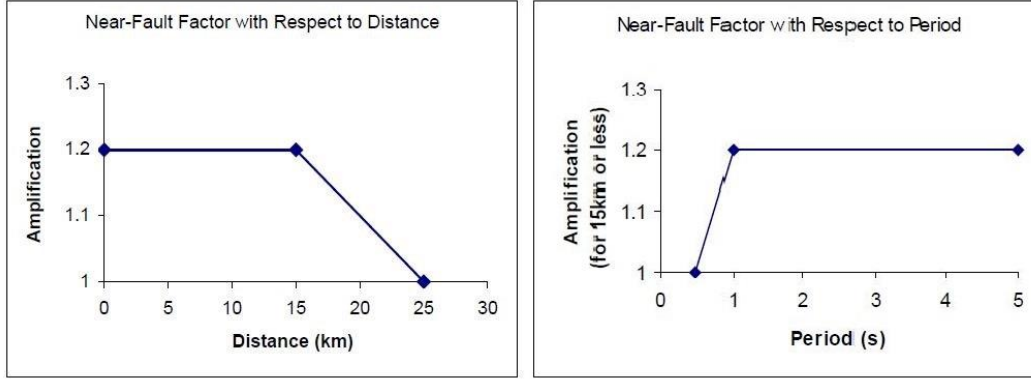
Figure 2.7 Near-Fault adjustment factor as a function of distance and spectral period (CALTRANS 2013).
