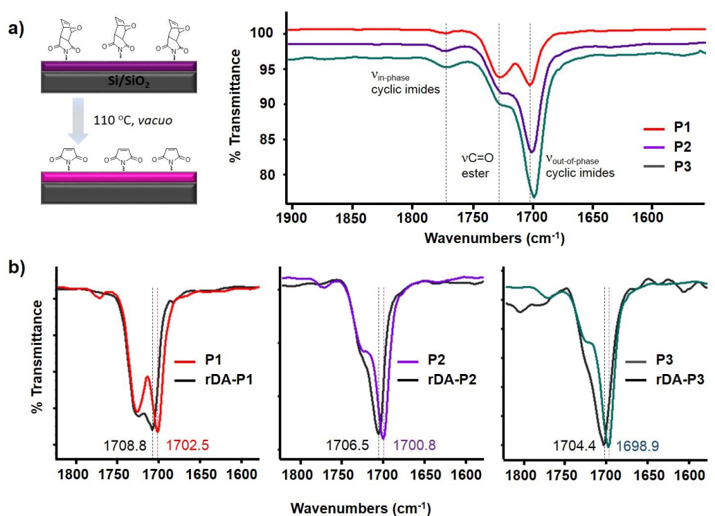
Figure 4.5. a) FTIR spectra in the 1905–1555 cm -1 spectral range for copolymers P1, P2 and P3 on Si/SiO 2 surface. b) FTIR spectra in the 1820–1580 cm -1 spectral range for copolymers (P1, P2 and P3) and activated copolymers rDA-P1, rDA-P2 and rDA-P3.
