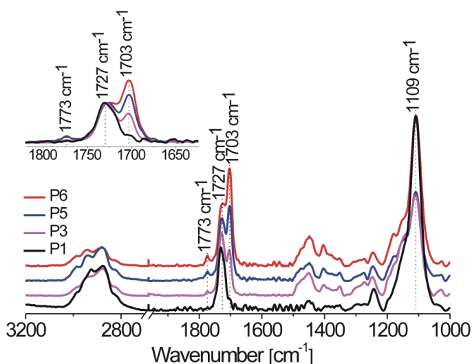
Figure 6.5. ATR-FTIR spectra of polymer brushes P1 ( d = 57 \text{ nm} ), P3 ( d = 39 \text{ nm} ), P5 ( d = 38 \text{ nm} ) and P6 ( d = 41 \text{ nm} ). All spectra were normalized with respect to the carbonyl at 1727 \text{ cm}^{-1} . Insert represents details of the 1820 - 1625 \text{ cm}^{-1} region.
