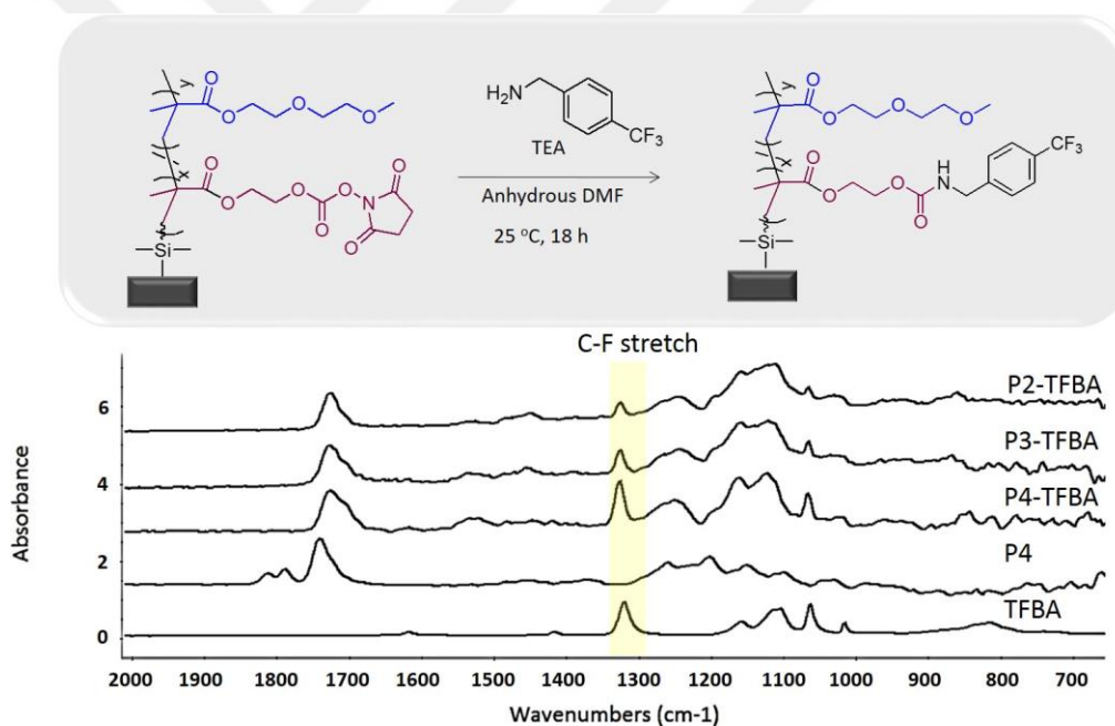
Figure 7.8. a) Scheme of 4-(trifluoromethyl)benzylamine (TFBA) attachment to P2, P3 and P4. b) ATR-FTIR spectra of TFBA immobilized polymer brushes P2, P3 P4 as well as bare P4 and TBFA for comperasion.
