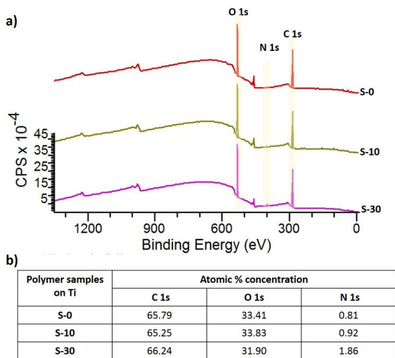
Figure 5.6. XPS survey spectra and relative concentrations of C, O and N of polymeric coatings.
