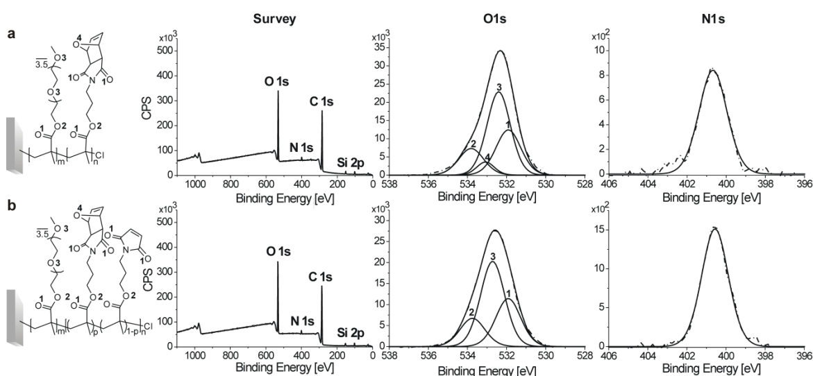
Figure 6.6. XPS survey scans as well as \text{O}1\text{s} and \text{N}1\text{s} high resolution spectra of copolymer brush P6 (a) before and (b) after retro Diels-Alder reaction.
