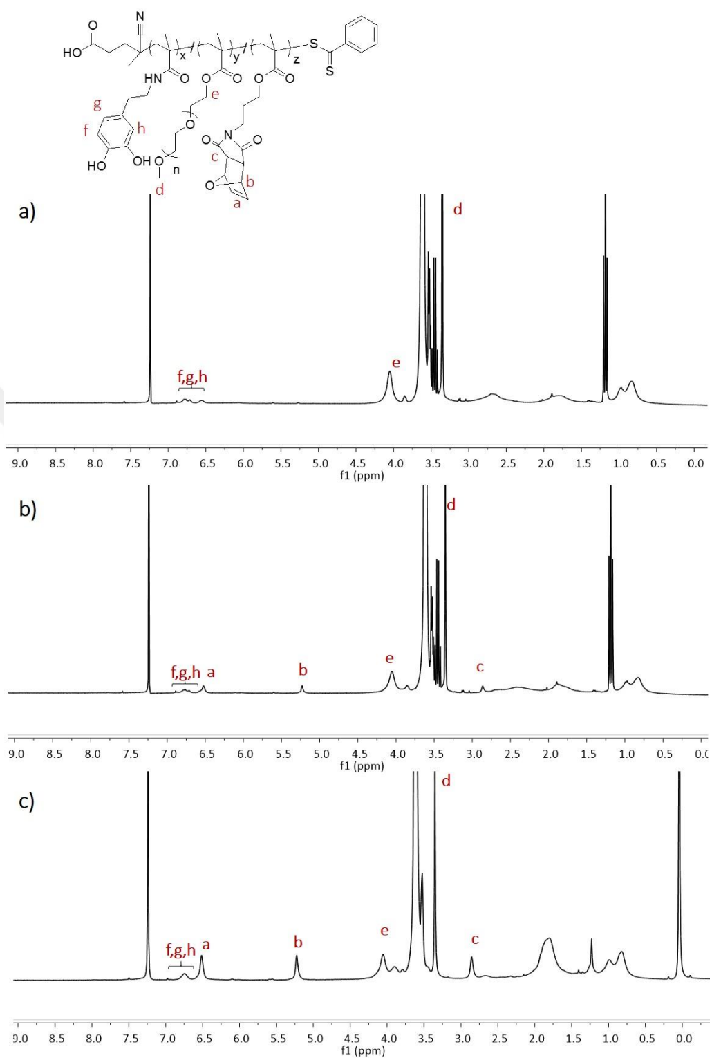
Figure 5.3. ^1\text{H} NMR spectra of the polymers a) P-0, b) P-10 and c) P-30 (Peaks at 1.18 and 3.46 ppm belong to ether)
