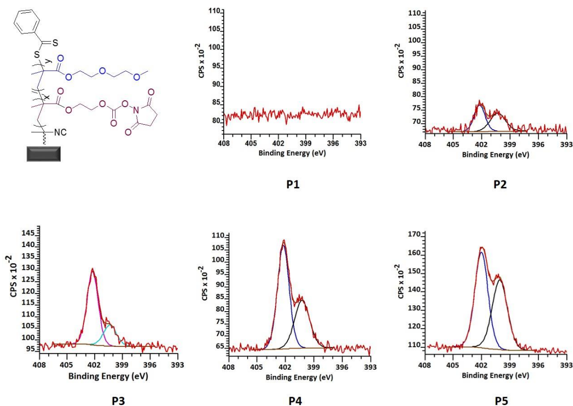
Figure 7.6. High resolution XPS elemental scans of N1s peaks of P1-P5.
