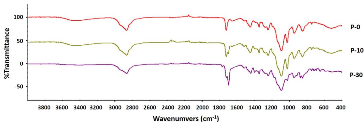
Figure 5.4. ATR-FTIR spectra of the copolymers a) P-0, b) P-10 and c) P-30.
