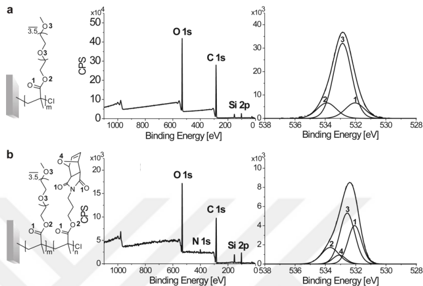
Figure 6.4. XPS survey spectra and high resolution \text{O} 1s elemental scans of: (a) a PEGMEMA homopolymer brush ( d = 102 \text{ nm} ) and (b) a P[PEGMEMA 50 -co-FuMaMA 50 ] copolymer brush ( d = 36 \text{ nm} ).
