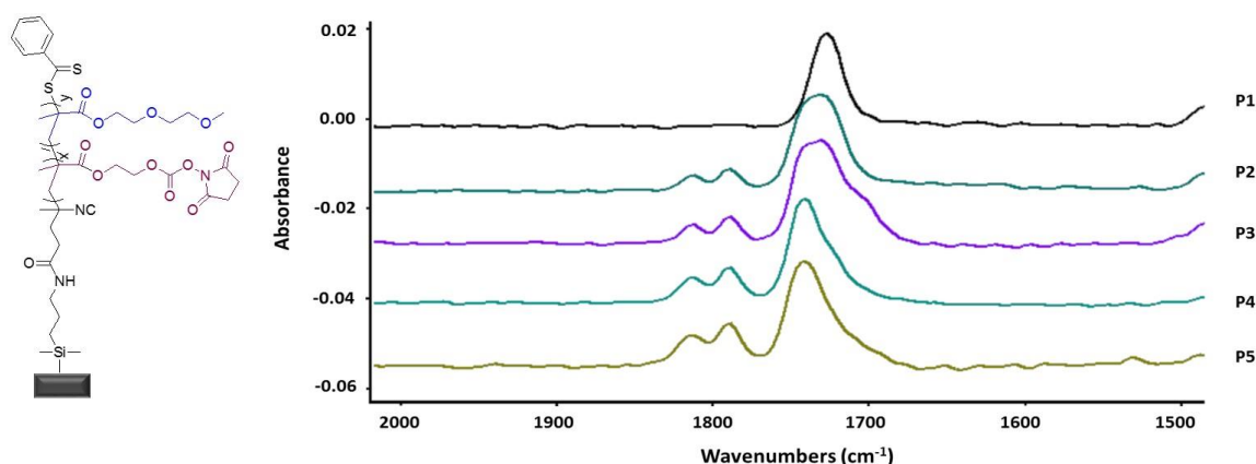
Figure 7.3. ATR-FTIR spectra of polymer brushes P1-P5.
