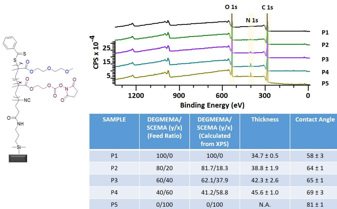
Figure 7.4. Survey spectra of polymer brush P1-P5 and calculated monomer incorporation from XPS based on N/C ratio.
