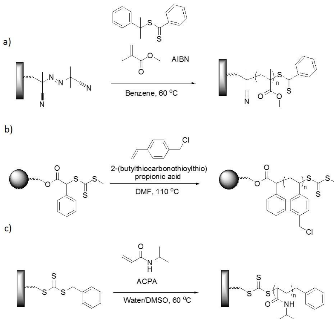
Figure 1.6. Three main methods for fabrication of polymer brushes via Surface RAFT polymerization a) using initiator modified surfaces [26] b) R-group approach [38] and c) Z-group approach [39]. Adapted from [21].
