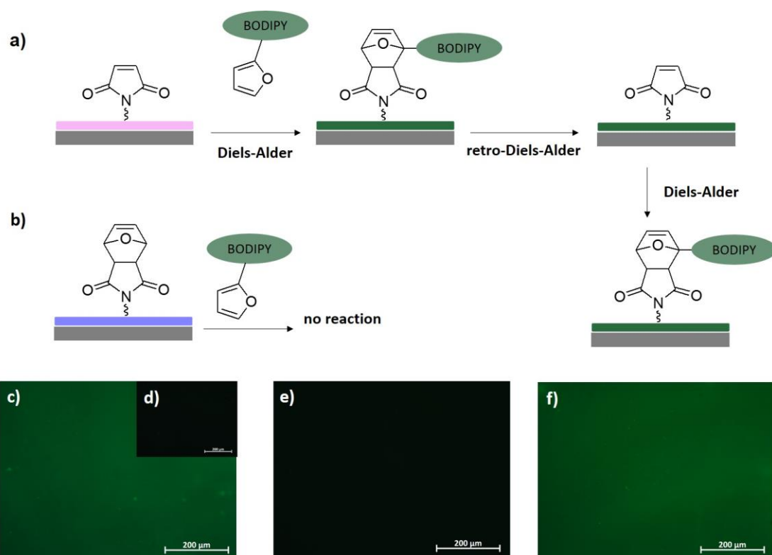
Figure 8.8. (a) BODIPY-furan reversible conjugation sequence, (b) control reaction. Fluorescence microscopy images of (c) dye conjugated hydrogel, (d) control experiment, (e) hydrogel after dye de-conjugation and (f) hydrogel after dye re-conjugation.
