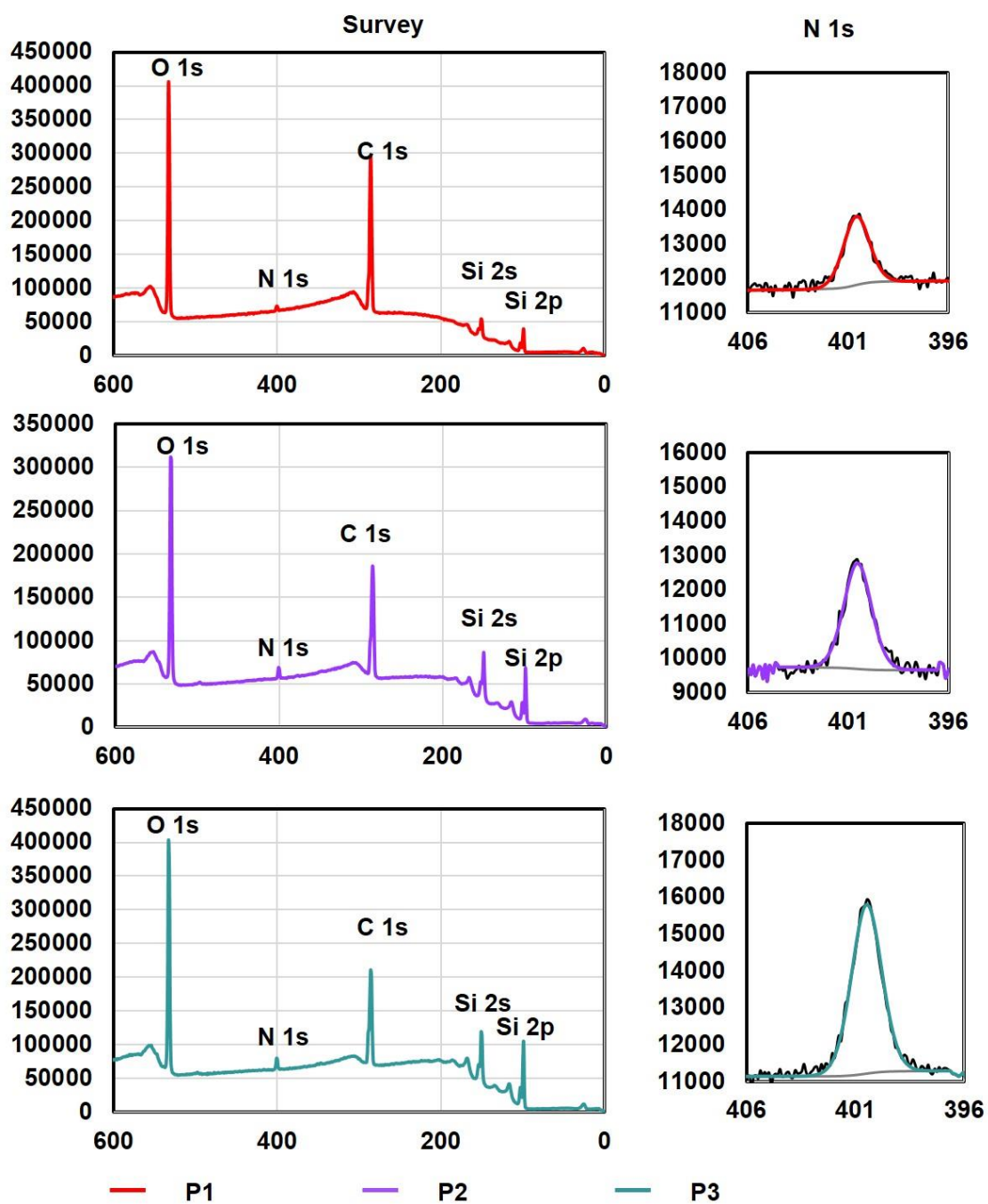
Figure 4.4. Fabricating polymeric layer on the substrates (a) and N1s peaks from XPS multiplex scans, of copolymer P1, P2 and P3 coated surfaces on Si/SiO 2 .
