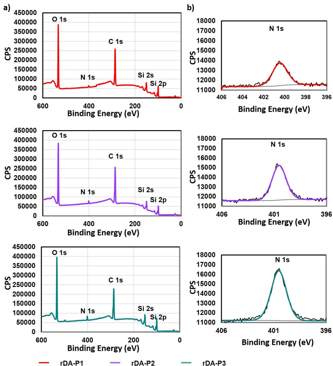
Figure 4.6. a) XPS survey spectra of rDA-P1, rDA-P2 and rDA-P3 surfaces, b) high-resolution XPS spectra for N 1s.
