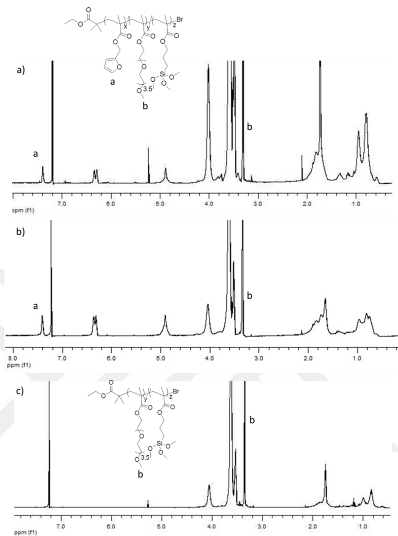
Figure 3.3. ^1\text{H} NMR spectra of copolymers: (a) P1, (b) P2 and (c) P3
