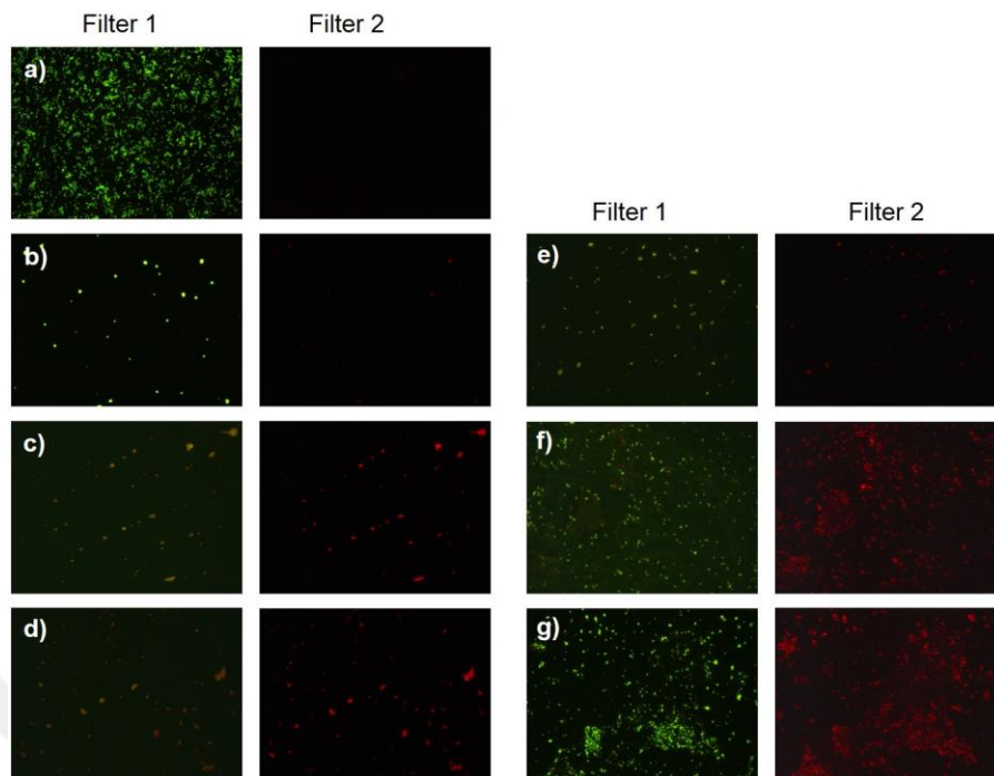
Figure 5.10. Fluorescence microscopy images of (a) bare titanium (b) S-0 (c) S-10 (d) S-30 (e) S-0-E6 (f) S-10-E6 (g) S-30-E6 on titanium surfaces by live/dead bacteria staining after incubation with P. aeruginosa .
