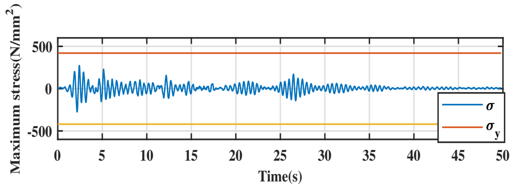
Figure 3.22. Maximum stresses
