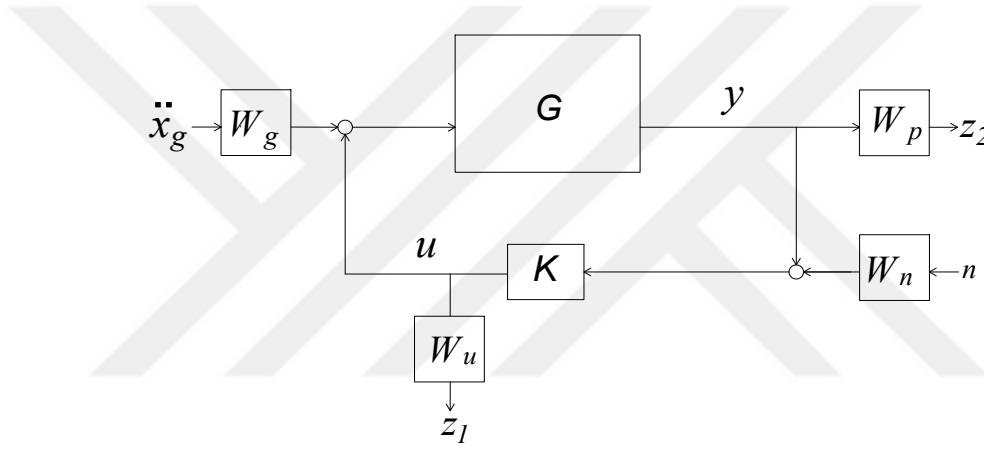
Figure 3.24. The generalized plant for a seismically excited nominal civil structure
