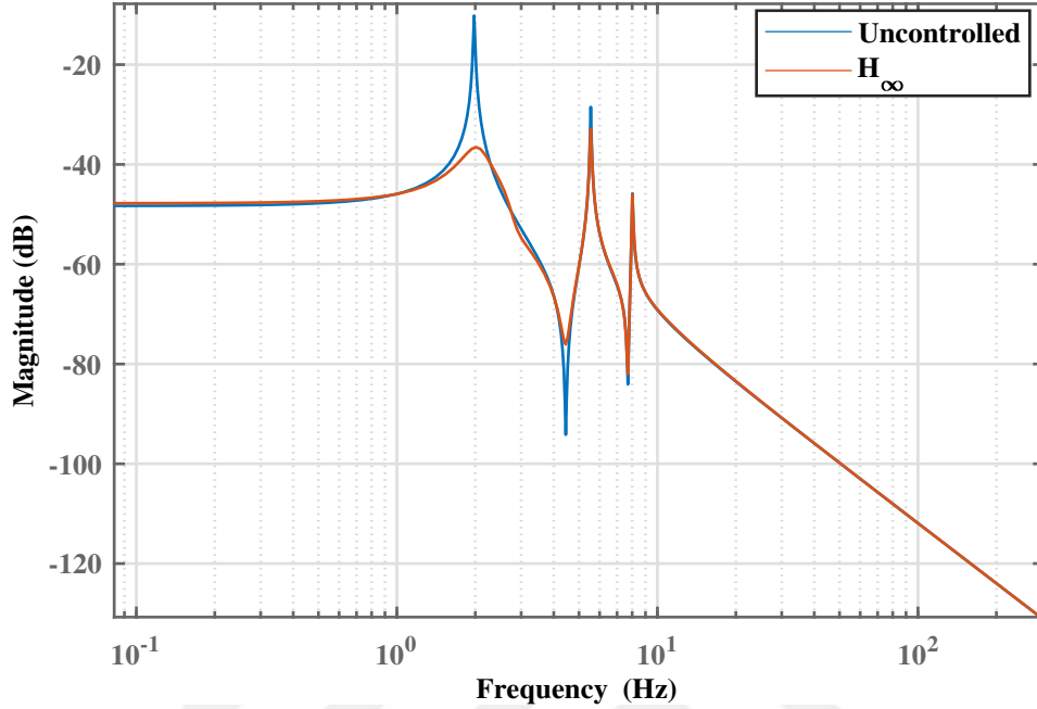
Figure 3.27. The bode diagram of H_\infty -controlled structure
