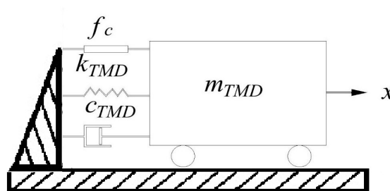
Figure 2.11. An active+passive hybrid controller setup
