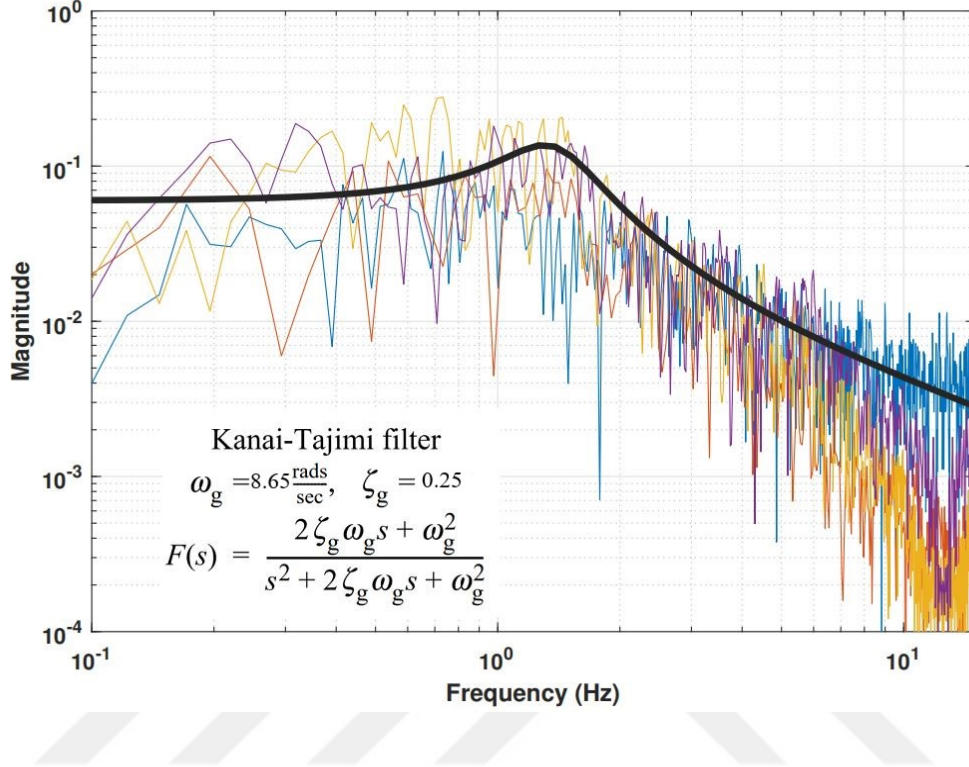
Figure 3.25. The designed Kanai-Tajimi filter
