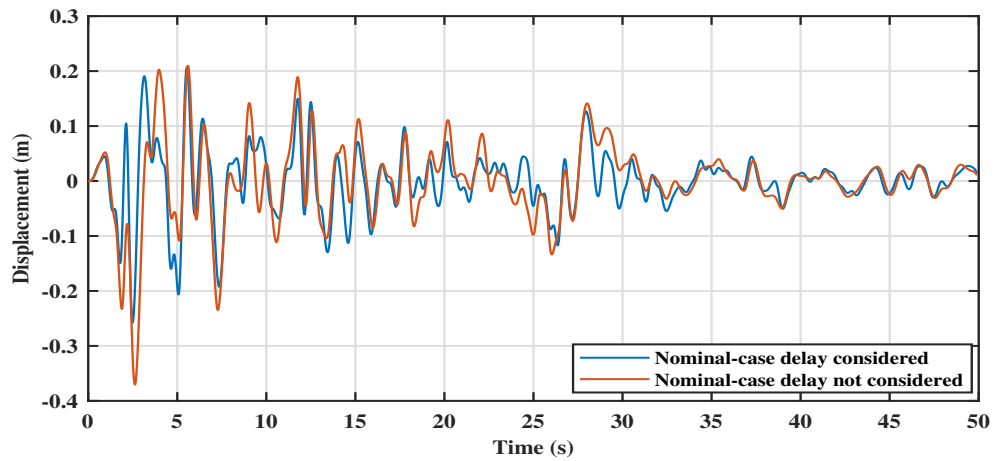
Figure 5.13. Delay effects
