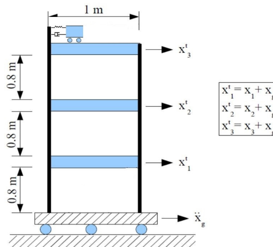
Figure 3.35. The TMD-installed structure
