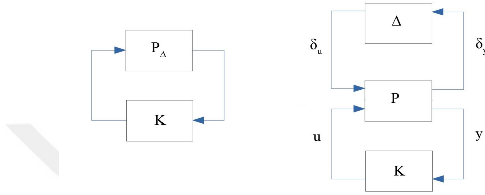
Figure 4.7. Robust stability
