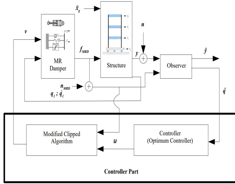
Figure 3.8. MRD setup
