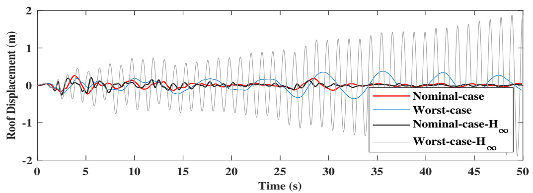
Figure 5.17. The responses of the structures subjected to the El Centro
