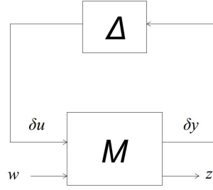
Figure 4.1. Standard M-Δ Configuration
