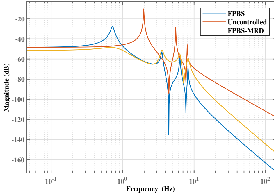
Figure 3.41. The Bode diagram of FPBS+MRD/Actuator-installed structure
