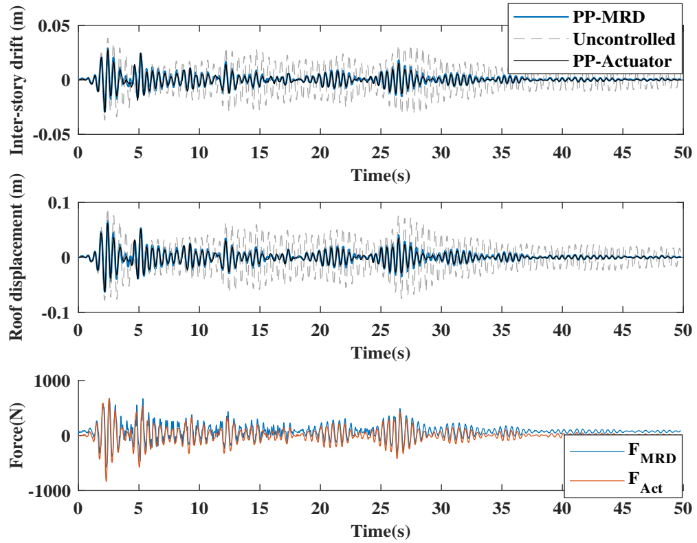
Figure 3.21. Responses of the PP-controlled structure
