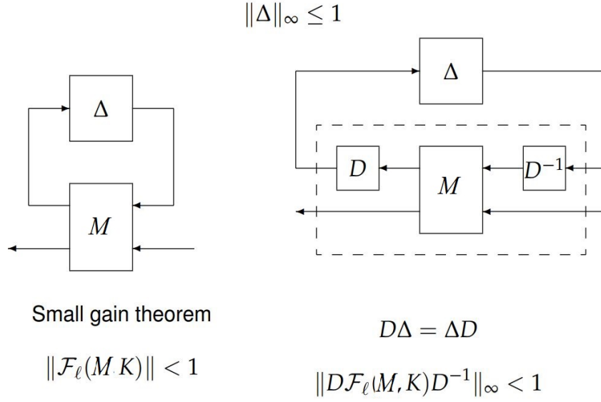
Figure 4.12. D Scaling (Source: Helmerson (2017))
