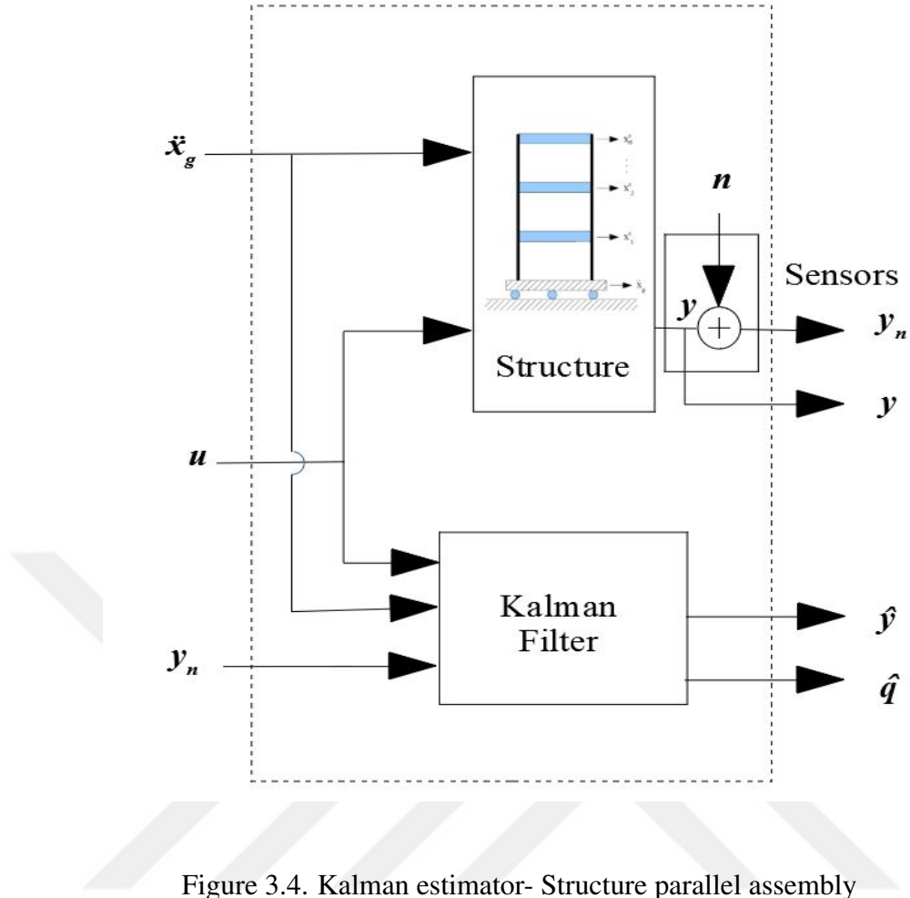
Figure 3.4. Kalman estimator- Structure parallel assembly
