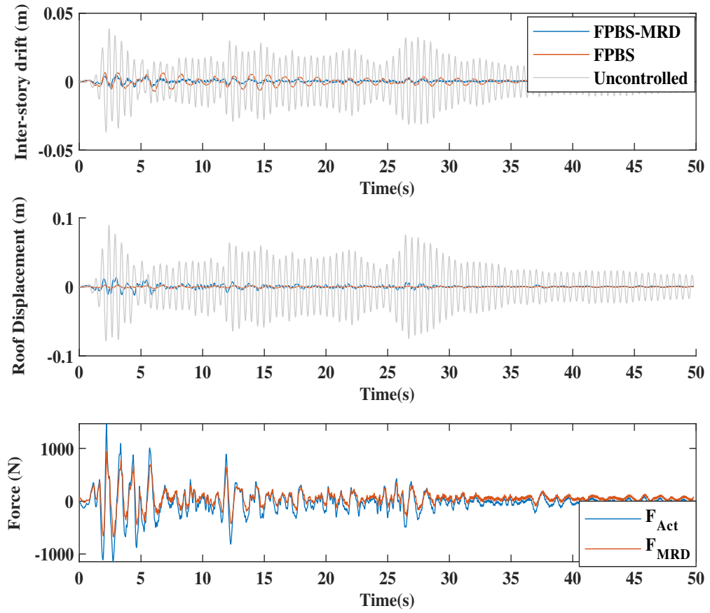
Figure 3.40. Responses of the FPBS+MRD-installed structure
