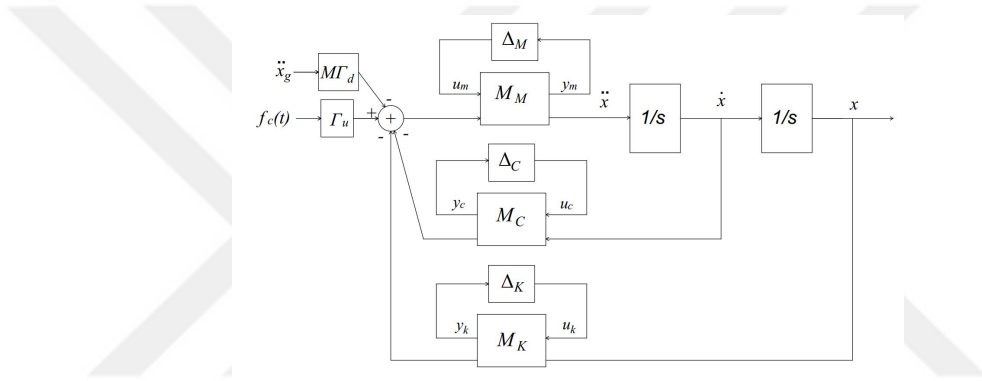
Figure 4.3. Block diagram of the controlled civil structure system with uncertainties
