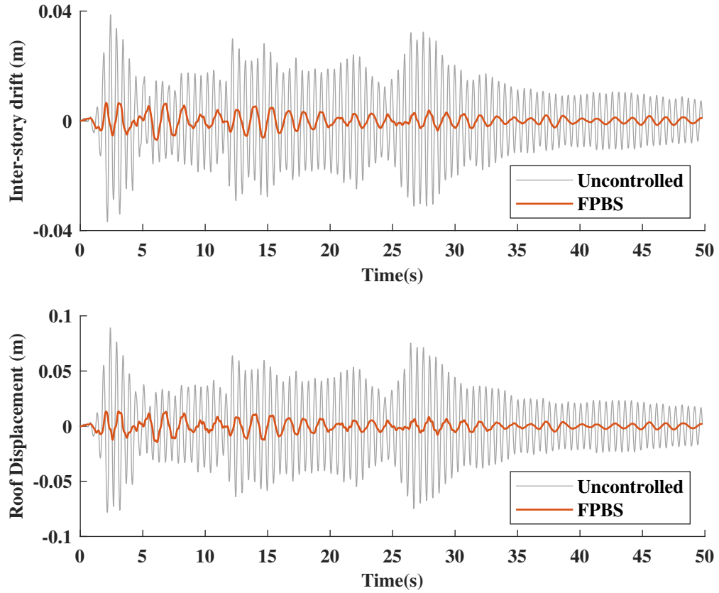
Figure 3.34. Responses of the FPBS-installed structure
