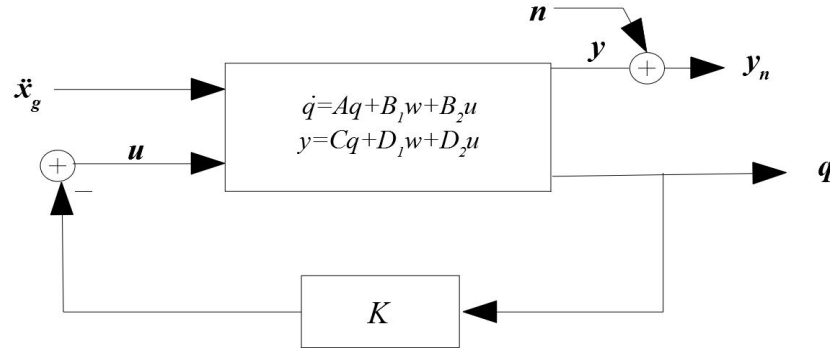
Figure 3.15. State-space feedback proportional control
