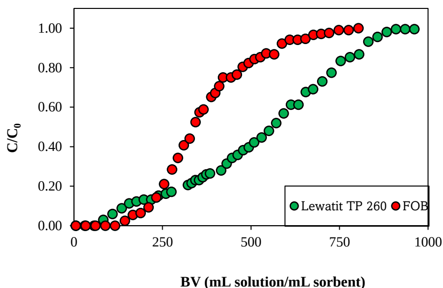
Figure 31. Breakthrough curves of \text{Li}^+ sorption on FOB and Lewatit TP 260
