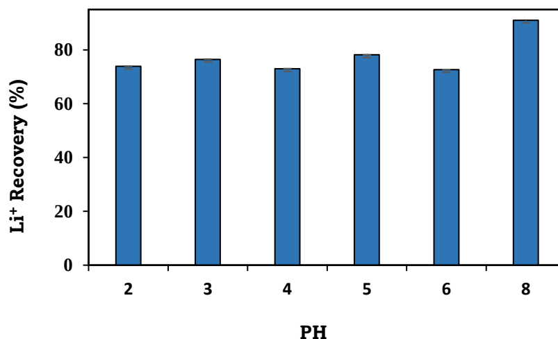
Figure 21. Effect of pH on lithium adsorption onto functionalized olive branches (Temp =30 °C, Adsorbent dosage 12 g/L, C_o = 10g/L, speed=180 rpm, pH = (2-8), Time =24 hr)
