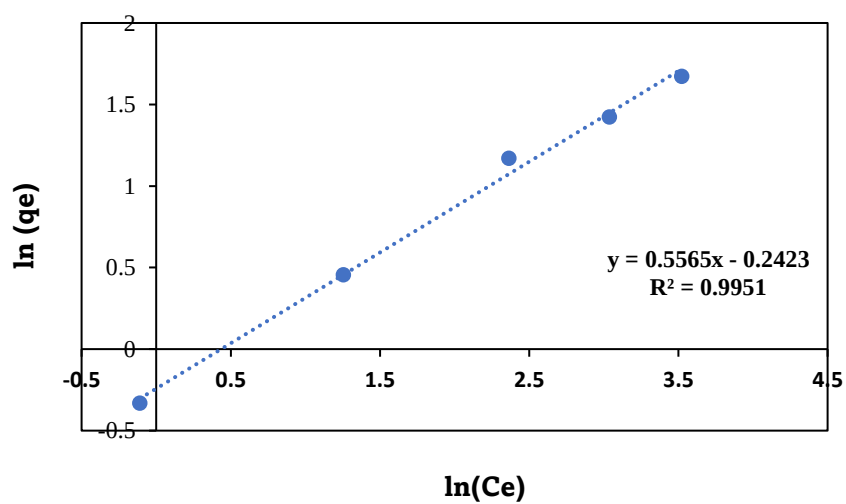
Figure B2. Freundlich model curve of FOB at 40 °C
