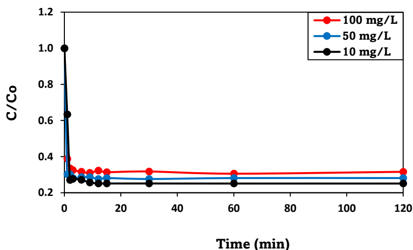
Figure 29. Adsorption kinetics at constant adsorbent dosage (12 g/L) with varying \text{Li}^+ concentration (Temp =25 °C, C_0 = (10-100 mg/L, Time = (0-120) min
