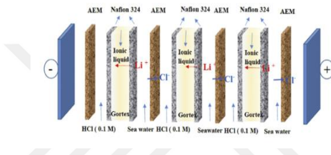
Figure 5. A set up for lithium extraction from seawater by electrodesialysis (Gmar and Chagnes 2019)
