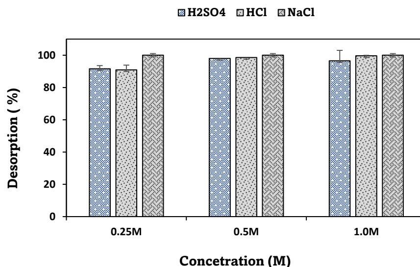
Figure 26. Desorption of \text{Li}^+ from Phosphorylated Olive Branches (FOB) (Temp =25 °C, Adsorbent dosage 12 g/L, \text{Co} = 100 mg/L saturated FOB, speed=180 rpm, pH = 8, Time =24 hr)
