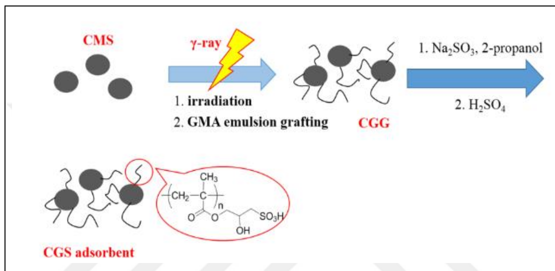
Figure 7. Shows step-by-step functionalization of cellulose by sulphuration (Source: C. Xu et al. 2020)
