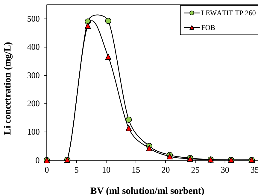
Figure 32. Elution curves of \text{Li}^+ sorption from FOB and Lewatit TP 260
