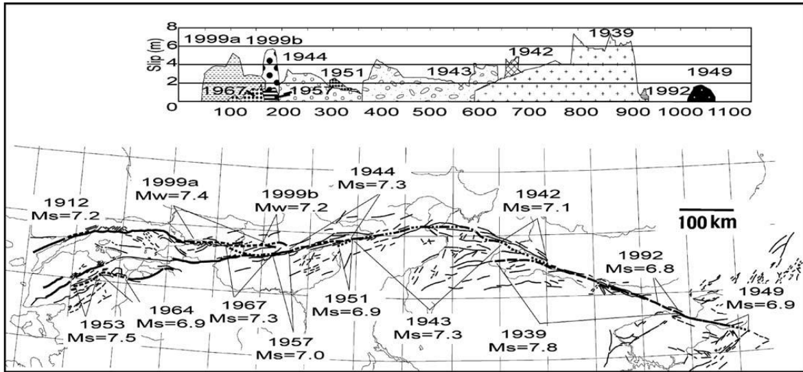
Figure 3.2. From the Figure 3 of study by Şengör et al. (2005) “Earthquakes and related fault displacements along the NAF since the December 26/27, 1939, Erzincan earthquake.”
