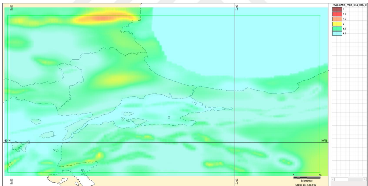
Figure 6.42. Fault source model \pm 1\sigma/\pm 1\sigma SA ( T=1.0 s) ratio, 2475 years RP
