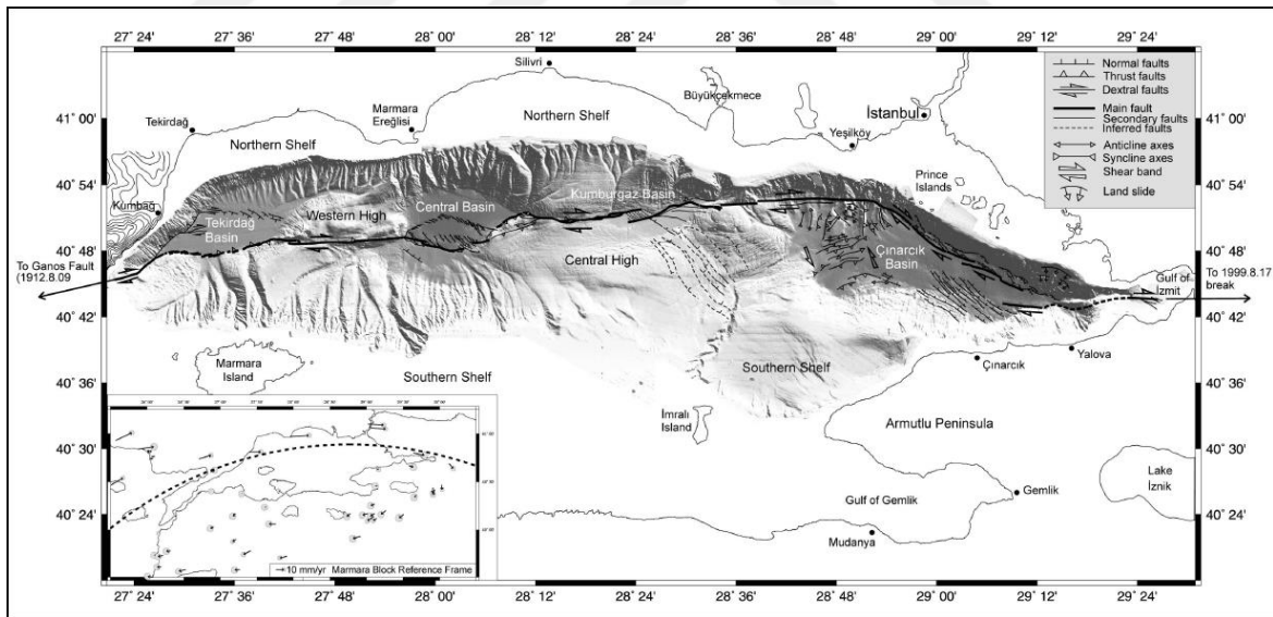
Figure 3.4. “Bathymetric map of the Marmara Sea” (Figure from the study by Le Pichon et al., 2001)
