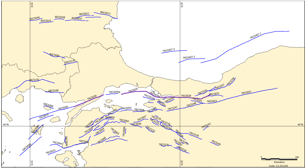
Figure 5.24. TRCS035, TRCS035, TRCS028 and TRCS036 fault sources
