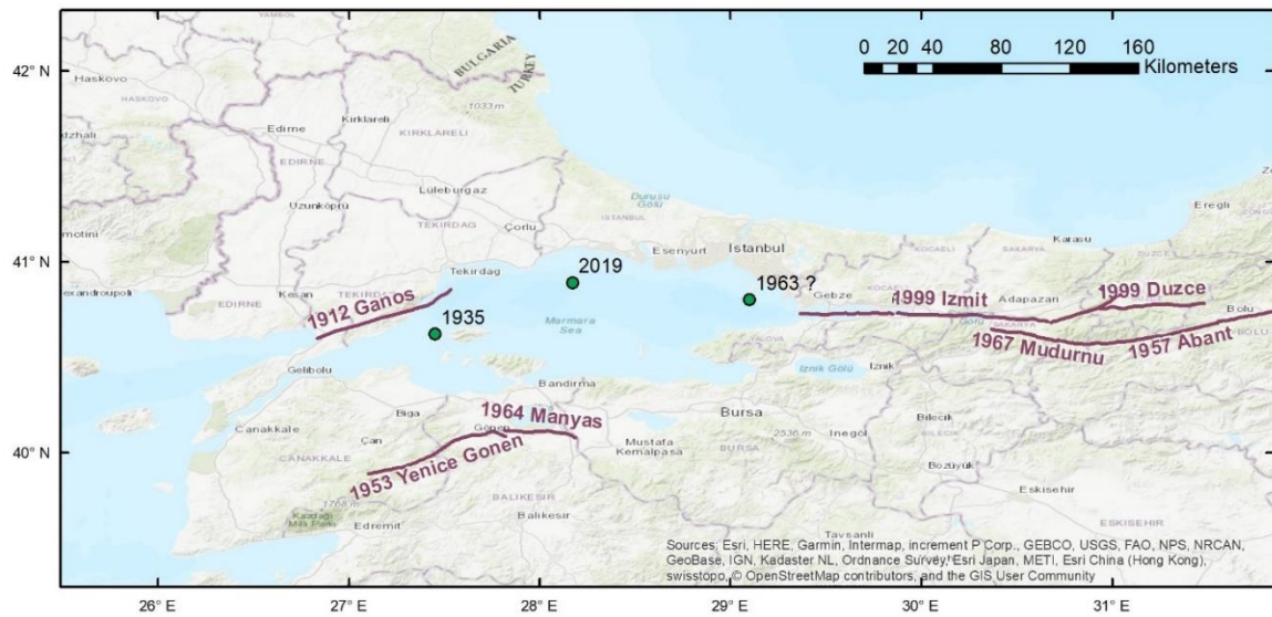
Figure 3.5. Major earthquakes of the 20th century in the Marmara region (Şeşetyan et al., 2019)
