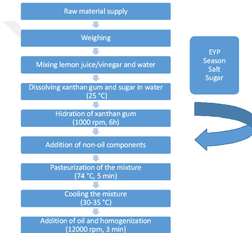
Figure 2. 4 Salad dressing production flow chart 3
