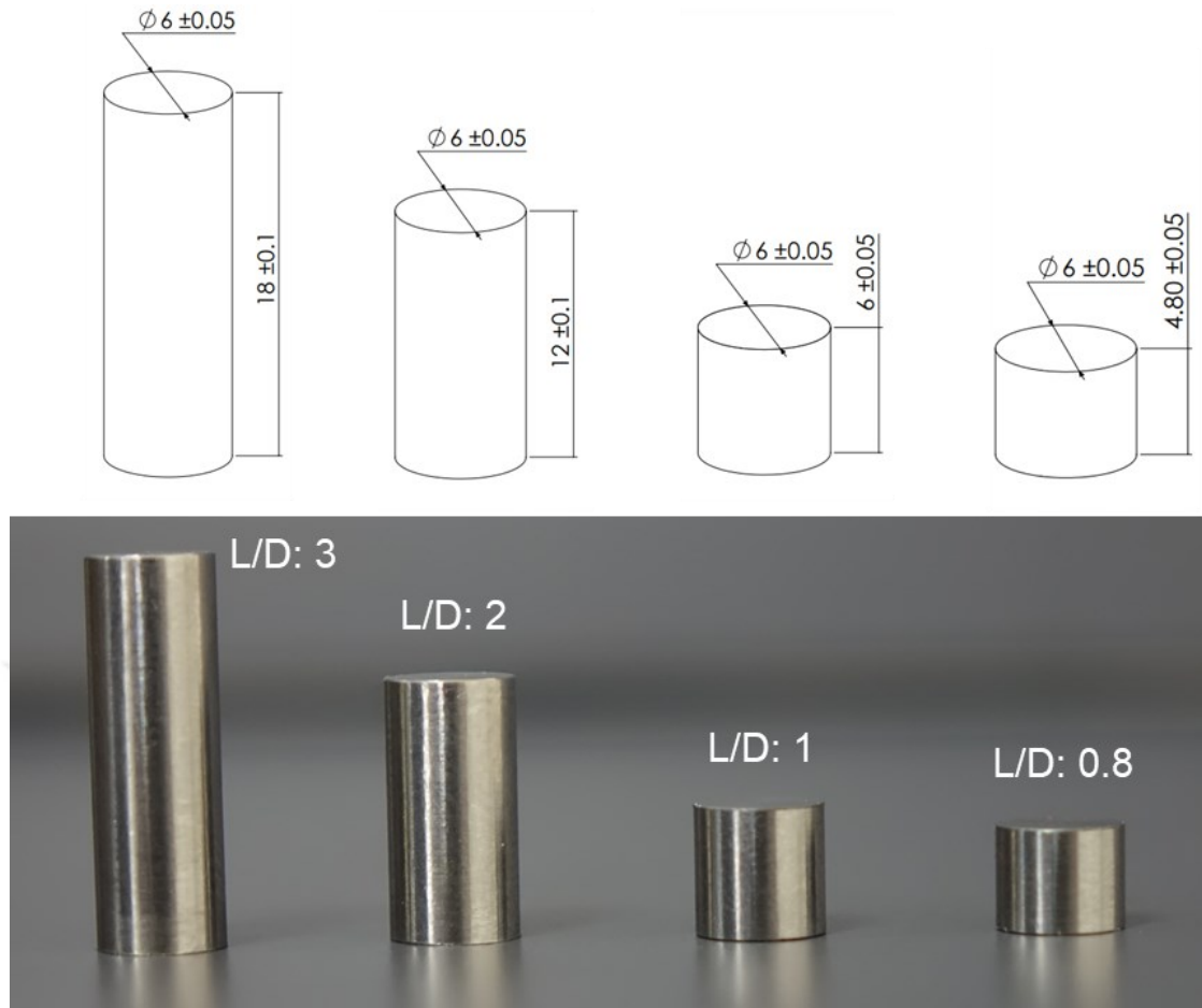
Figure 4.5. Compression test specimens used in quasi-static and dynamic tests and technical drawings of the specimens.
