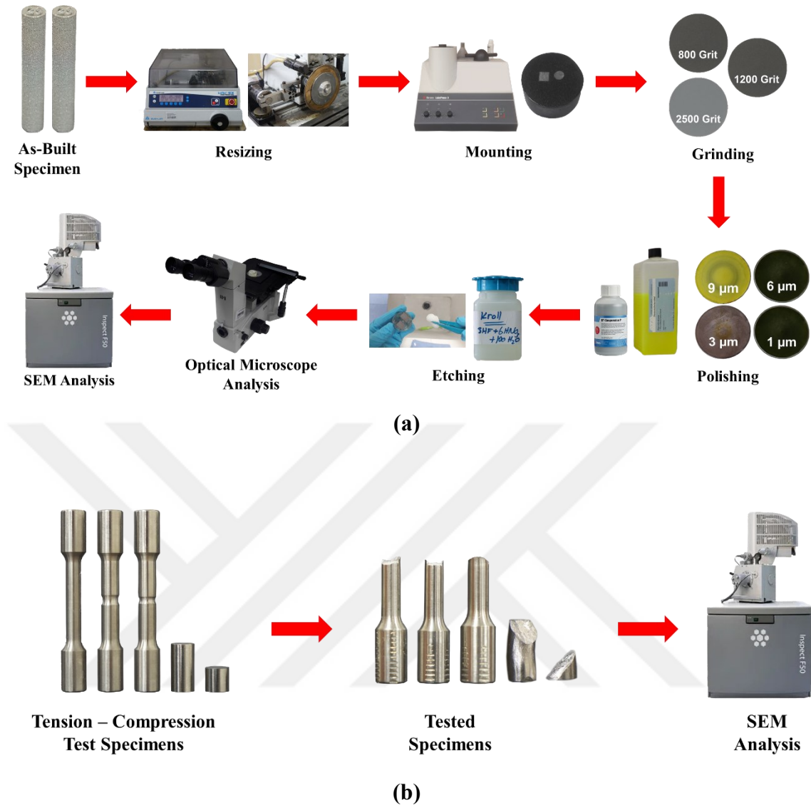
Figure 4.6. Procedures in metallographic analysis (a) as-built examination, (b) fracture analysis for tested specimens.
