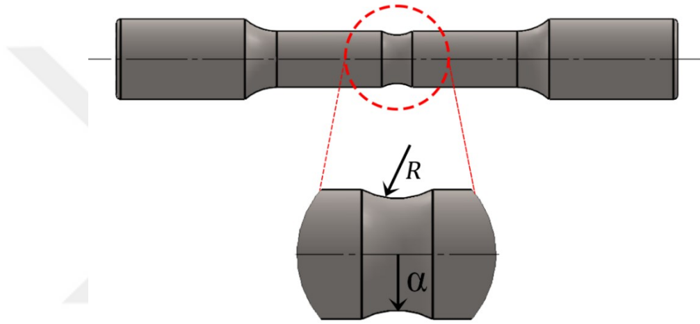
Figure 3.7. A notched tension specimen and the exploded view of the notch region.
