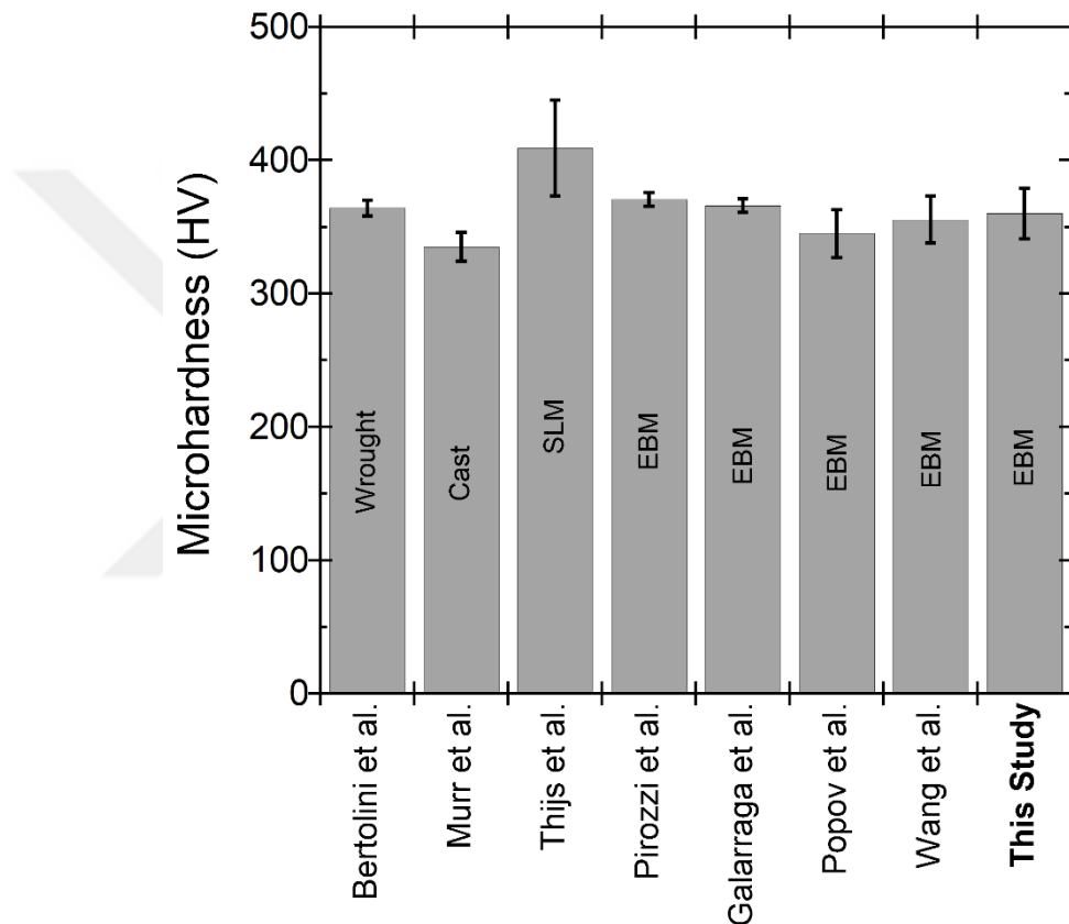
Figure 7.7. Microhardness results of Ti64 alloy taken from literature based on manufacturing methods.
