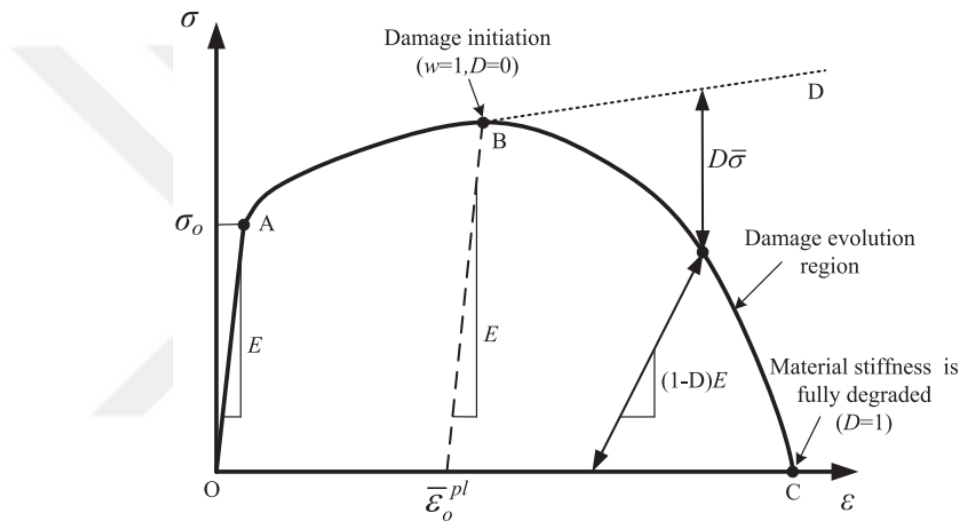
Figure 3.5. Strain to failure history curve of most metallic materials.
