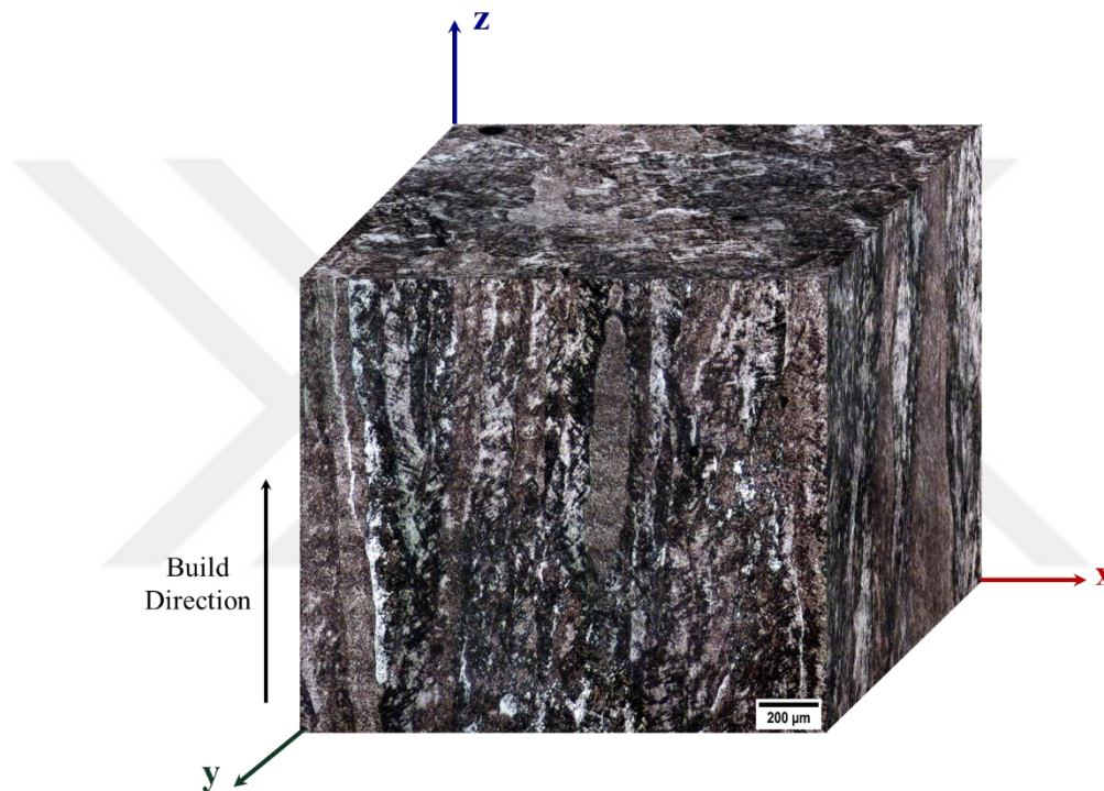
Figure 5.4. Combination of microstructural views with regards to all three axes relative to build direction.
