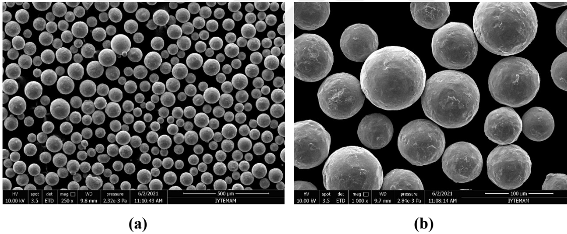
Figure 4.1. Magnified view of Ti64 ELI powder (a) at 250x magnification and (b) at 1000x magnification.
