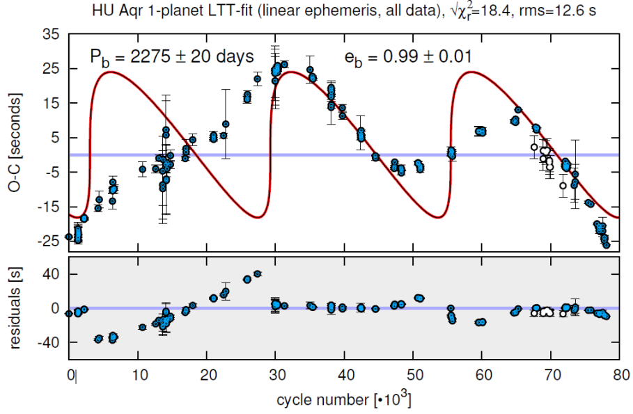
Figure 5.1. Synthetic curve of the 1-planet LTT model with linear ephemeris to all available data, including the very recent egress times collected by the OPTIMA photometer, as well as PIRATE, TCS and MONET/N telescopes. Open circles are for measurements in Qian et al. (2011). [Taken from Gozdziewski & Nasiroglu et al. (2012)]
