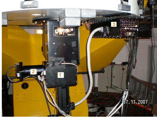
Figure 3.2. A photograph of OPTIMA-Burst mounted on the 1.3 m Cassegrain focus telescope of the Skinakas Observatory. The target acquisition optics (filters, target imaging and fiber pick-up) is located in box no. 1 and the CCD camera is mounted externally box no. 2. APD photon counters are located in box no. 3 connected to the telescope
