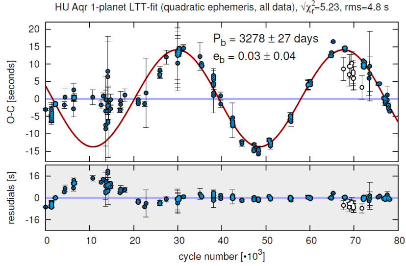
Figure 5.2. Synthetic curve of the 1-planet LTT model with quadratic ephemeris to all available data, gathered in this work, including the very recent mid-eclipse times collected by the OPTIMA photometer, as well as PIRATE, TCS and MONET/N telescopes with orbital parameters given in Table 5.1. (Fit I). The white filled circles mark the Qian et al. (2011) measurements. [Taken from Goździewski & Nasiroglu et al. (2012)]
