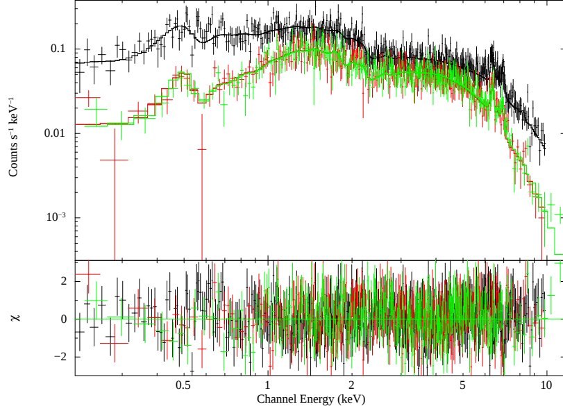
Figure 4.26. The composite model ( \text{phabs} \times \text{pcfabs} \times (\text{mekal} + \text{bbody} + \text{gaussian}) \times \text{constant} ) fitted to the spectrum of the EPIC-pn (black) and MOS (green and red) data in the 0.2–10 keV energy band. The bottom panel shows the residuals
