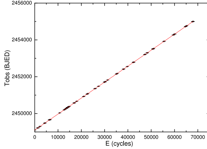
Figure 4.7. Entire observed egress times of HU Aqr and the least-squares linear fit ( f(x) = a + bx , solid line)
