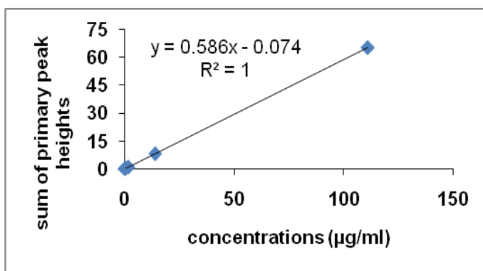
Figure B.10: Calibration curve for oleuropein.
