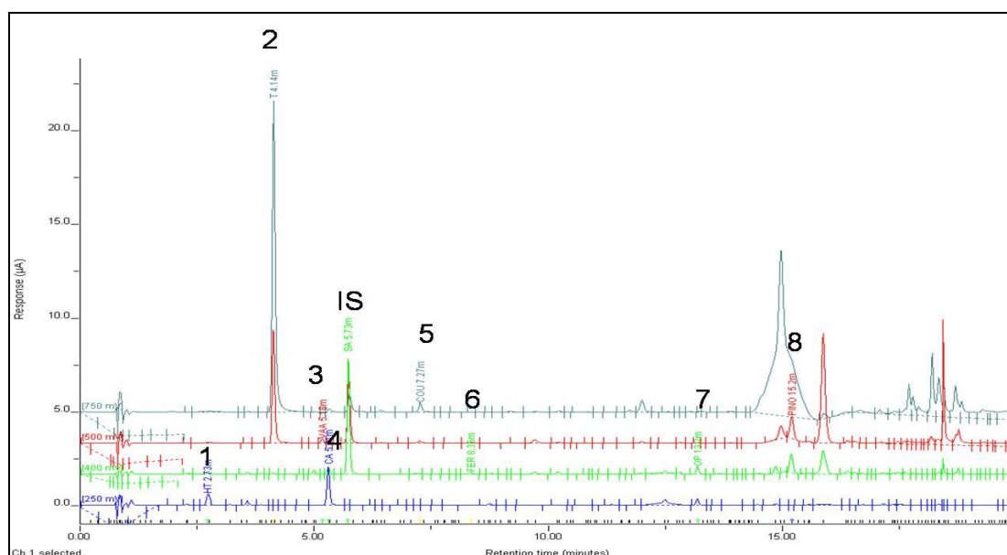
Figure A.2: Representative chromatogram of the olive oil extract1) hydroxytyrosol 2) tyrosol 3) caffeic acid 4) vanillic acid 5) ferulic acid 6) p-coumaric acid 7) oleuropein 8) pinoresinol IS: internal standard.
