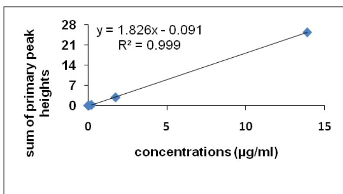
Figure B.9: Calibration curve for ferulic acid.
