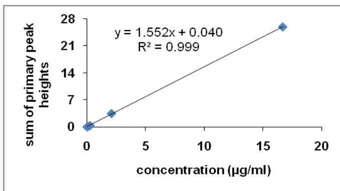
Figure B.11: Calibration curve for pinoresinol.
